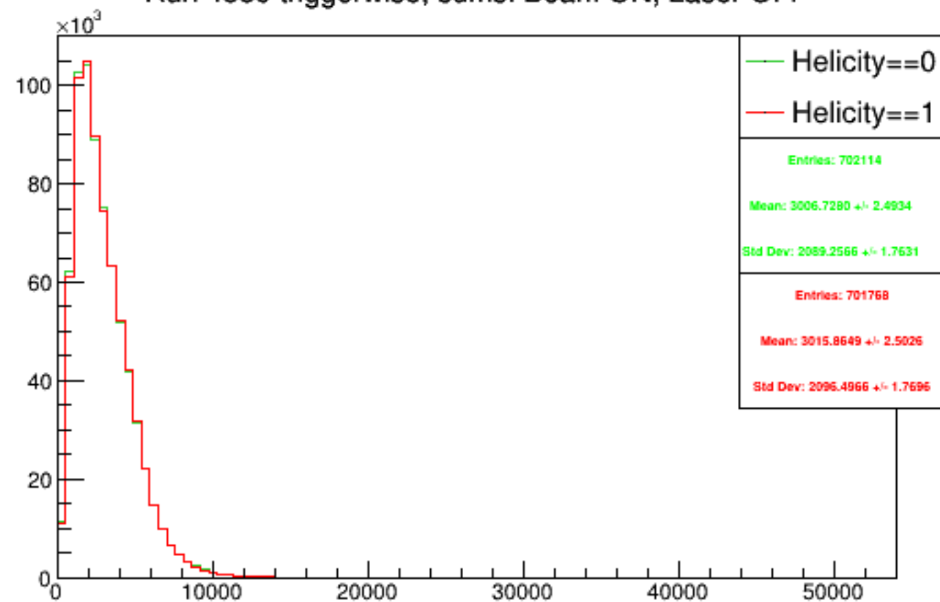
Run 4589 triggerwise, sums: Beam ON, Laser OFF
