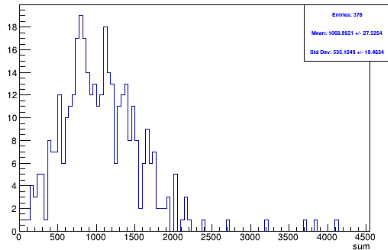
Run 4589 triggerwise, sums: Beam OFF
