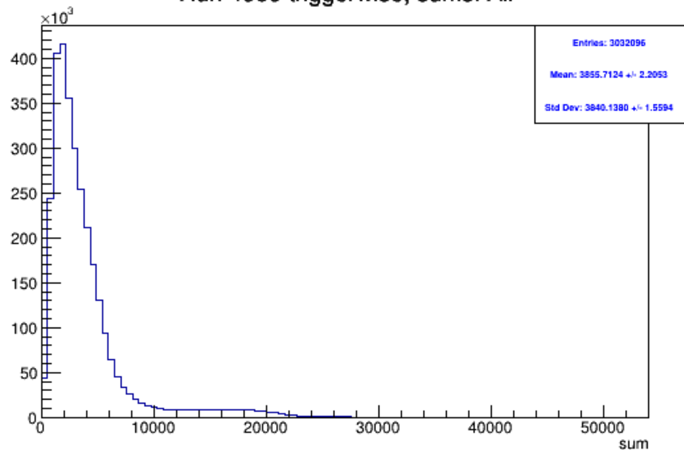
Run 4589 triggerwise, sums: All
