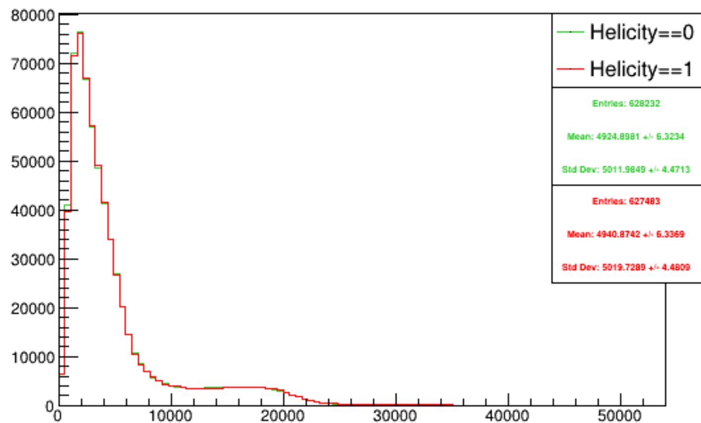
Run 4589 triggerwise, sums: Beam ON, Laser ON
