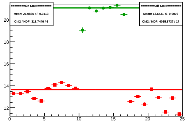
Cycle 4591.17: Multiplet Sums
