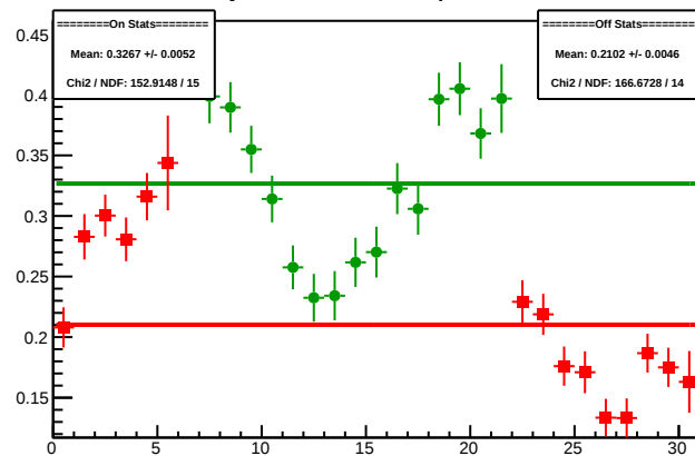
Cycle 4591.6: Multiplet Diffs
