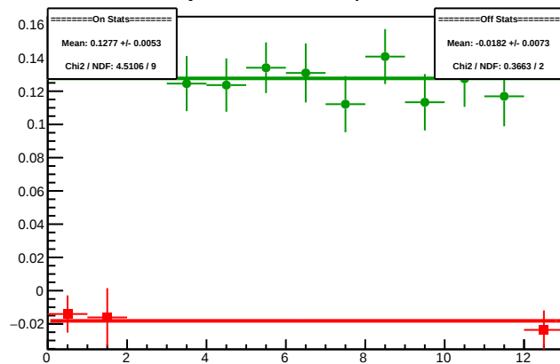
Cycle 4591.1: Multiplet Diffs
