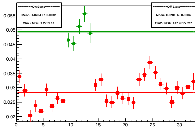
Cycle 4591.13: Multiplet Asyms
