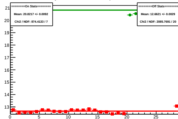
Cycle 4591.4: Multiplet Sums
