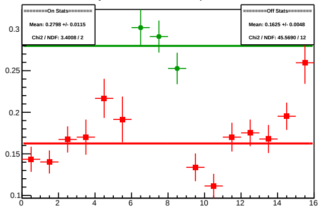
Cycle 4591.19: Multiplet Diffs
