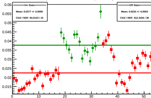
Cycle 4591.14: Multiplet Asyms
