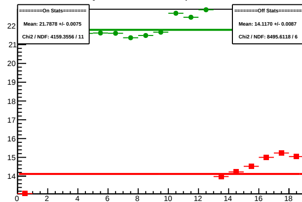
Cycle 4591.5: Multiplet Sums
