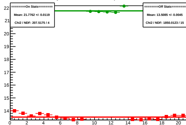
Cycle 4591.8: Multiplet Sums
