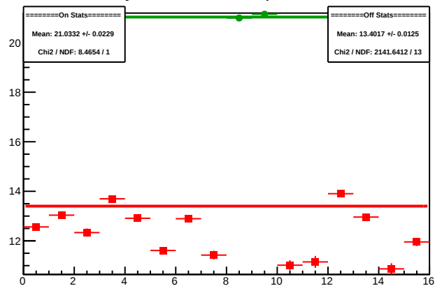
Cycle 4591.18: Multiplet Sums
