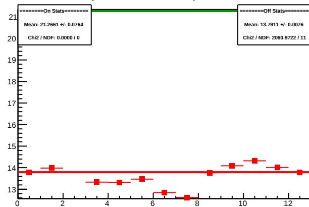
Cycle 4591.16: Multiplet Sums
