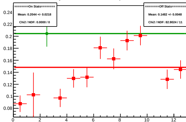
Cycle 4591.16: Multiplet Diffs
