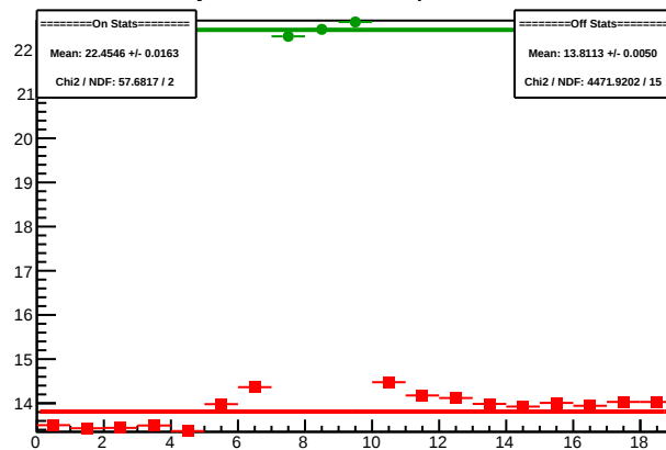
Cycle 4591.12: Multiplet Sums
