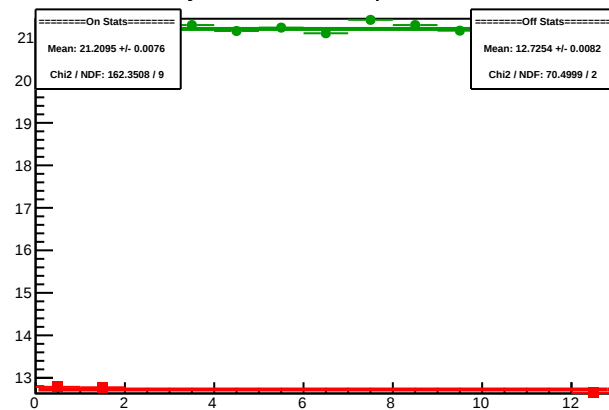
Cycle 4591.1: Multiplet Sums
