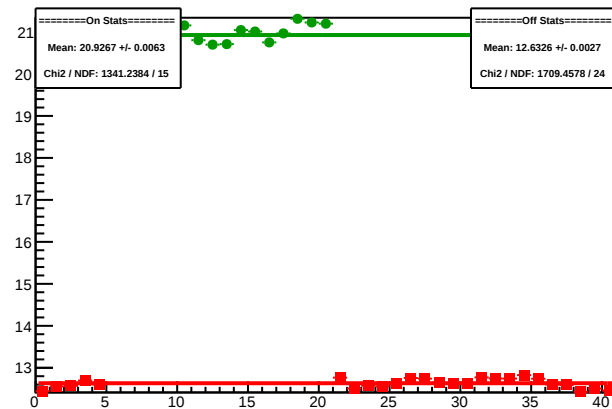
Cycle 4591.3: Multiplet Sums
