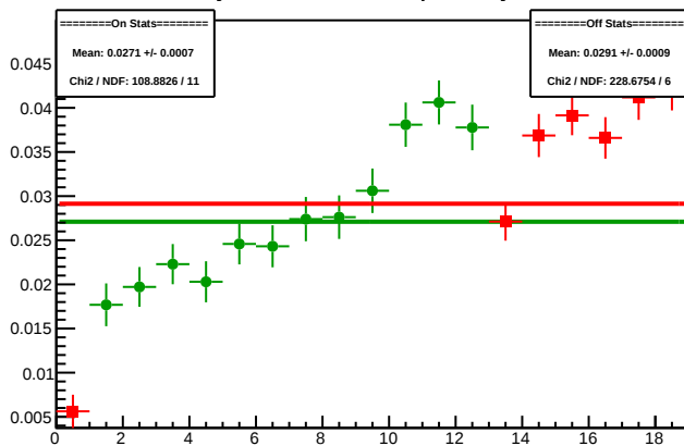
Cycle 4591.5: Multiplet Asyms
