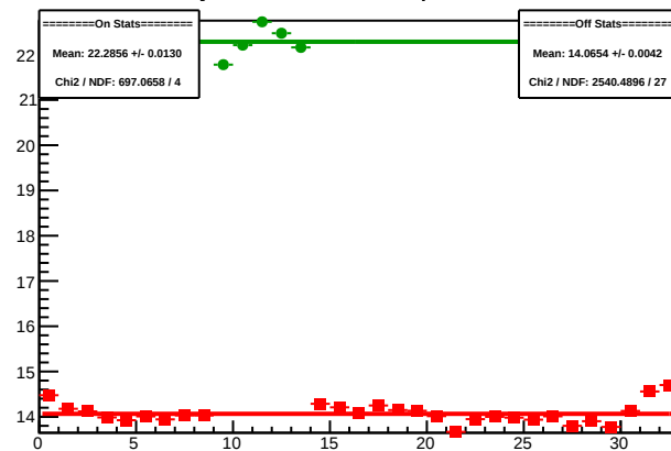
Cycle 4591.13: Multiplet Sums
