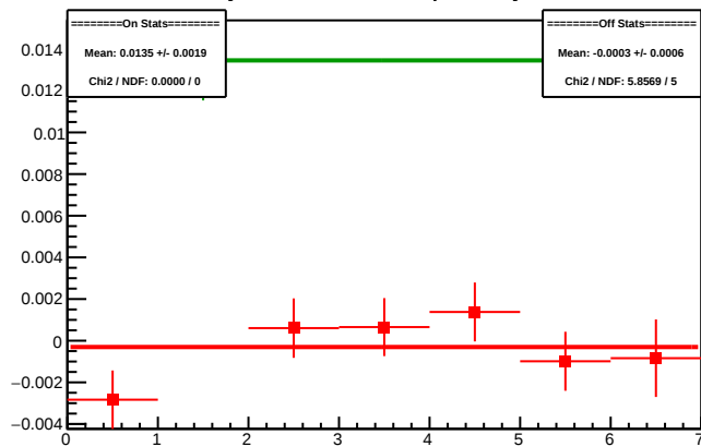
Cycle 4591.2: Multiplet Asyms
