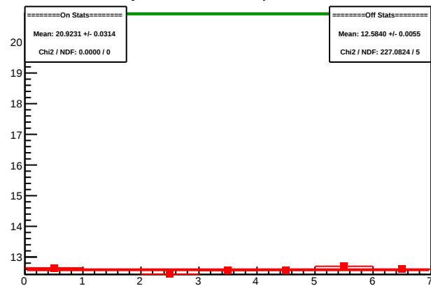
Cycle 4591.2: Multiplet Sums
