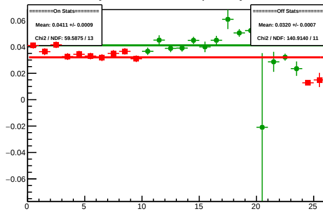
Cycle 4591.15: Multiplet Asyms
