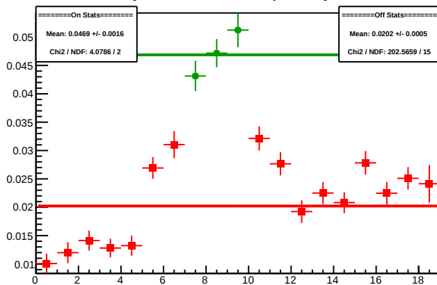
Cycle 4591.12: Multiplet Asyms
