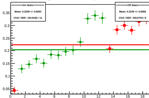
Cycle 4591.5: Multiplet Diffs
