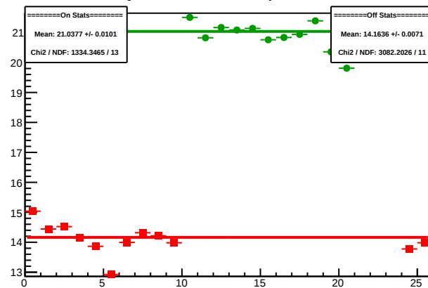
Cycle 4591.15: Multiplet Sums
