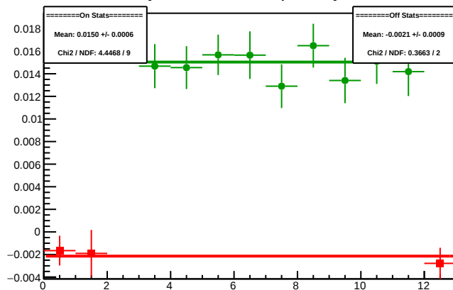
Cycle 4591.1: Multiplet Asyms
