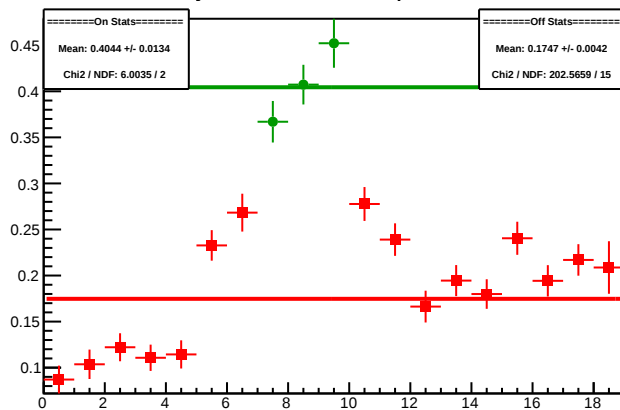
Cycle 4591.12: Multiplet Diffs
