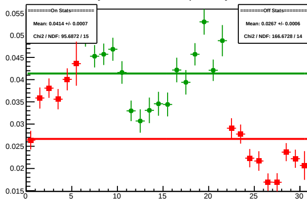
Cycle 4591.6: Multiplet Asyms
