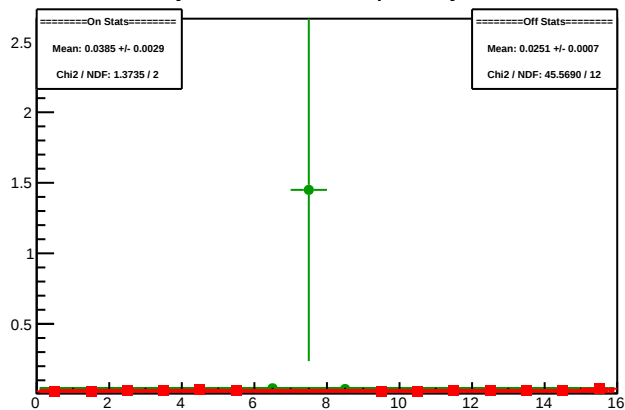
Cycle 4591.19: Multiplet Asyms
