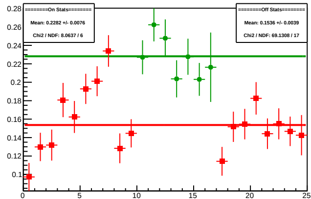
Cycle 4591.17: Multiplet Diffs
