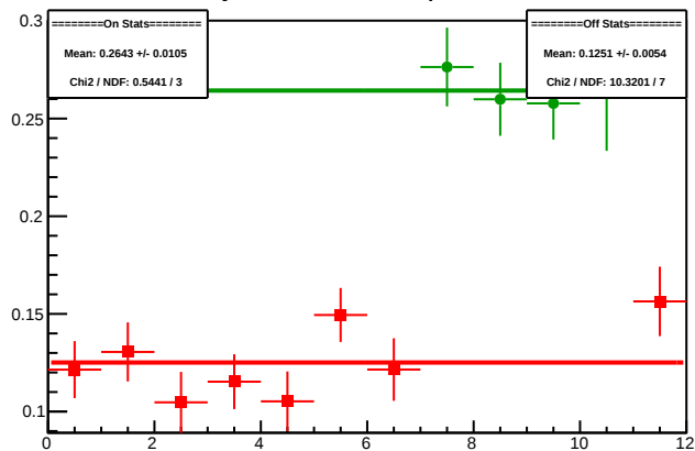
Cycle 4591.9: Multiplet Diffs
