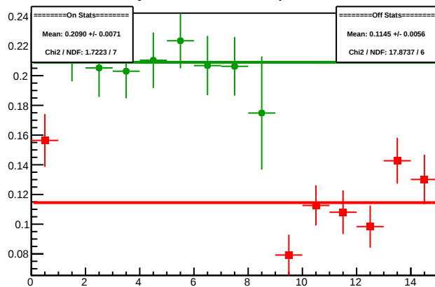
Cycle 4591.10: Multiplet Diffs
