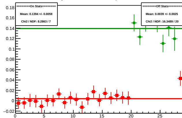
Cycle 4591.4: Multiplet Diffs
