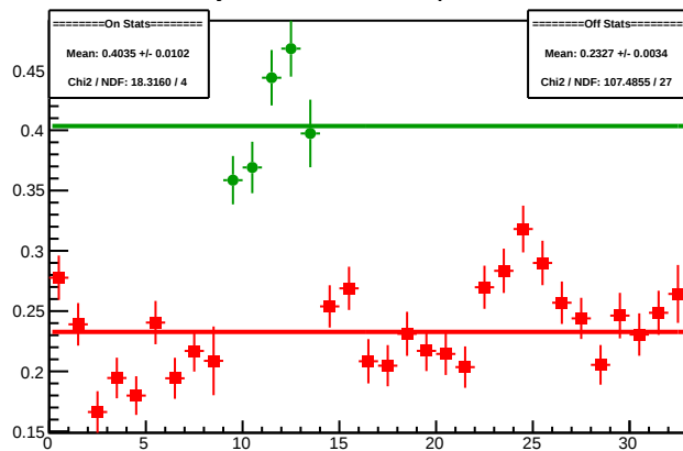
Cycle 4591.13: Multiplet Diffs
