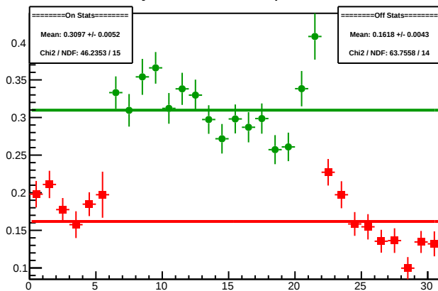
Cycle 4591.7: Multiplet Diffs
