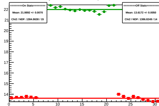
Cycle 4591.7: Multiplet Sums
