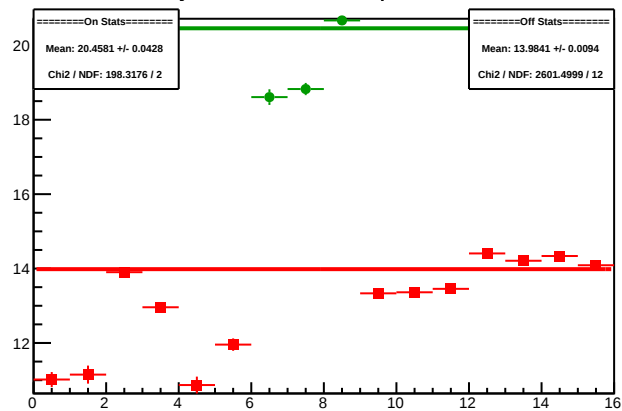
Cycle 4591.19: Multiplet Sums
