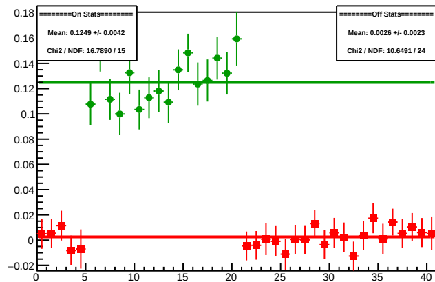
Cycle 4591.3: Multiplet Diffs
