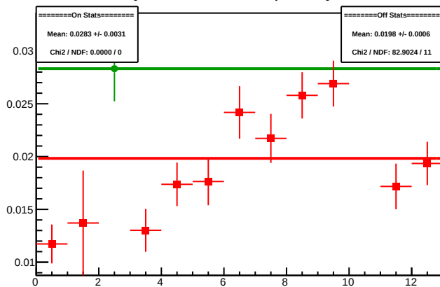
Cycle 4591.16: Multiplet Asyms
