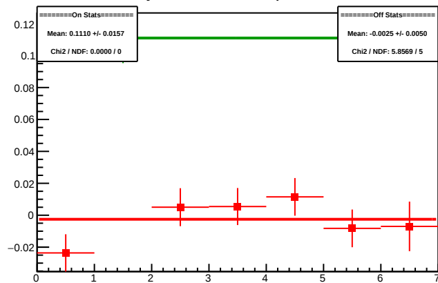
Cycle 4591.2: Multiplet Diffs
