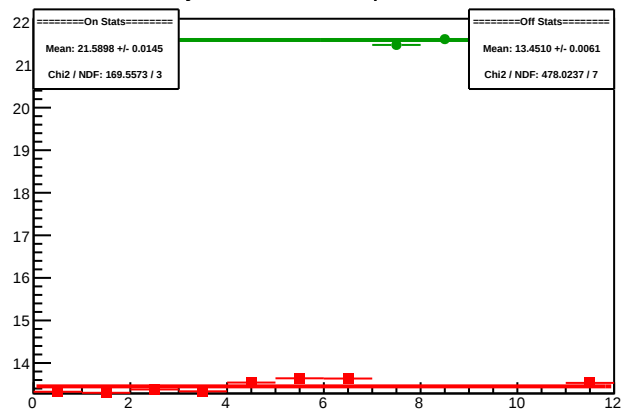
Cycle 4591.9: Multiplet Sums
