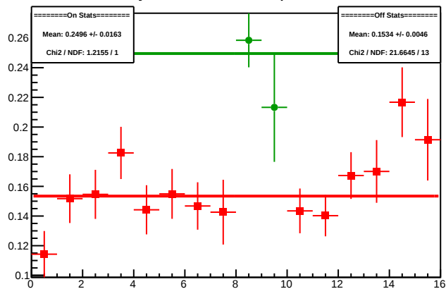
Cycle 4591.18: Multiplet Diffs
