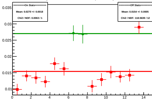
Cycle 4591.11: Multiplet Asyms
