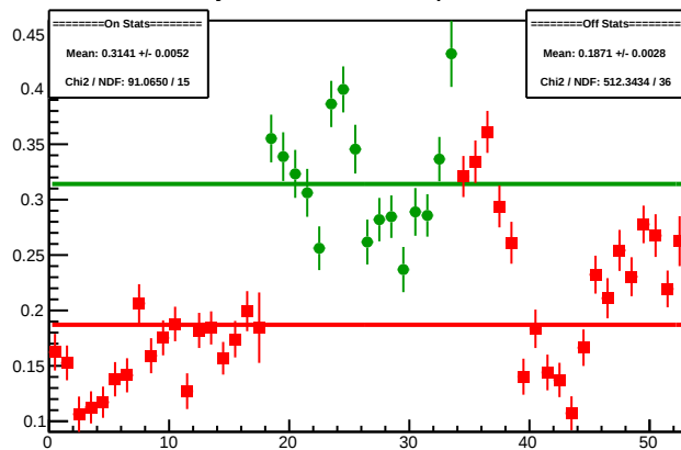
Cycle 4591.14: Multiplet Diffs
