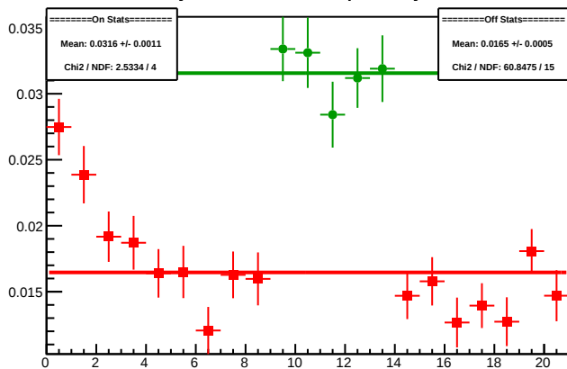
Cycle 4591.8: Multiplet Asyms
