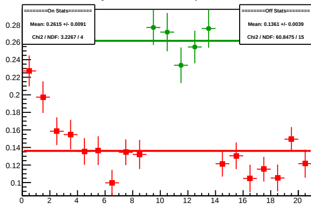
Cycle 4591.8: Multiplet Diffs
