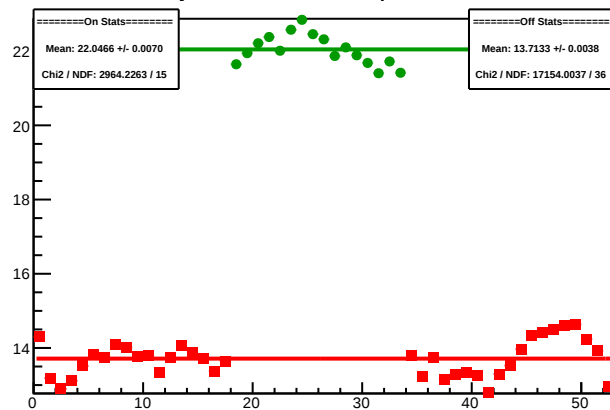
Cycle 4591.14: Multiplet Sums
