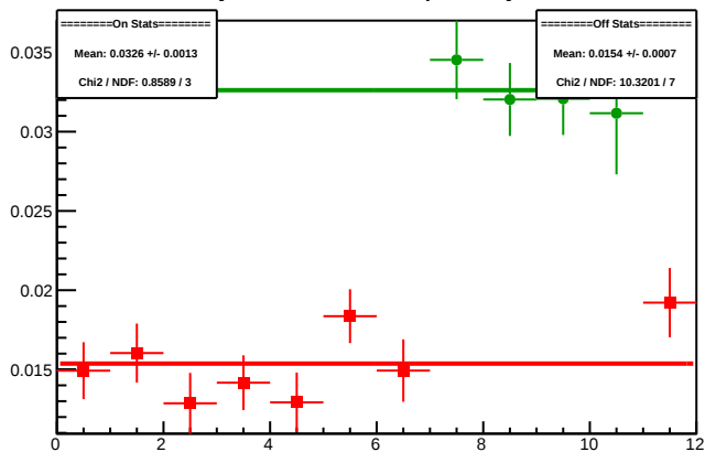
Cycle 4591.9: Multiplet Asyms
