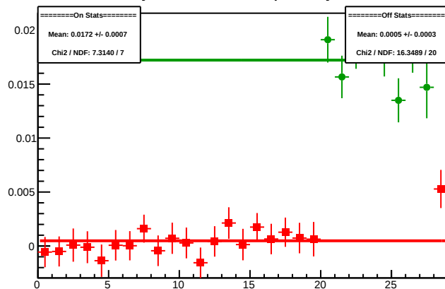
Cycle 4591.4: Multiplet Asyms
