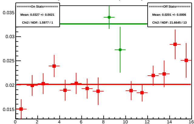
Cycle 4591.18: Multiplet Asyms
