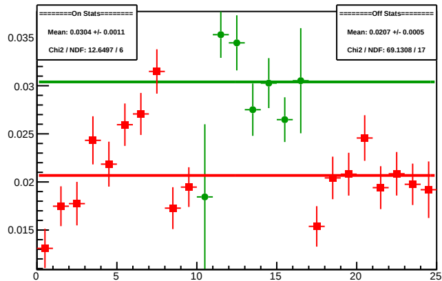
Cycle 4591.17: Multiplet Asyms
