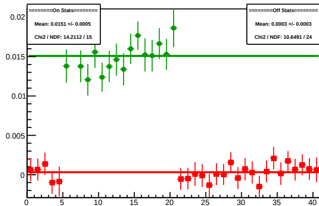
Cycle 4591.3: Multiplet Asyms
