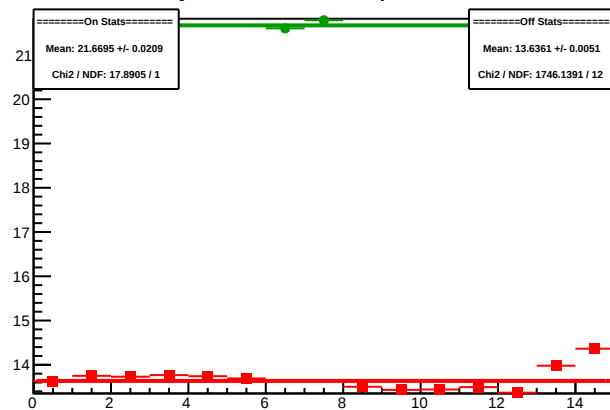
Cycle 4591.11: Multiplet Sums
