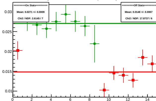
Cycle 4591.10: Multiplet Asyms
