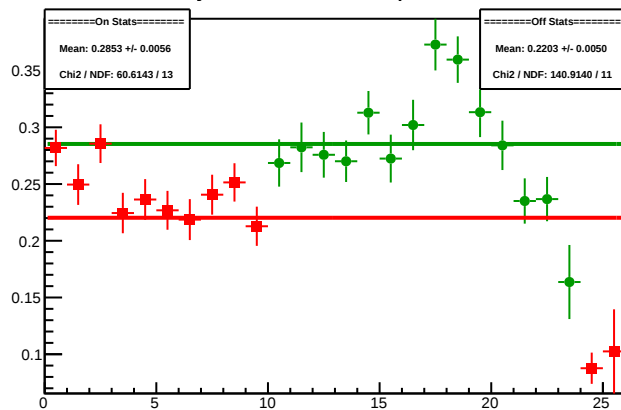
Cycle 4591.15: Multiplet Diffs
