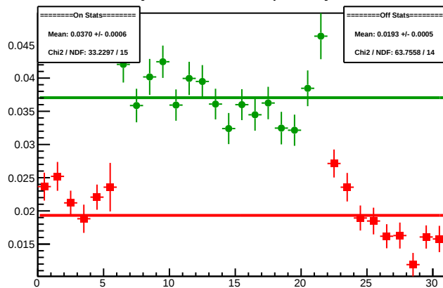
Cycle 4591.7: Multiplet Asyms
