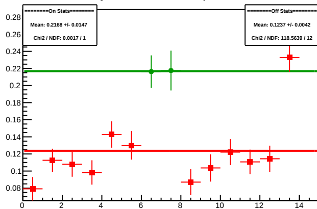
Cycle 4591.11: Multiplet Diffs
