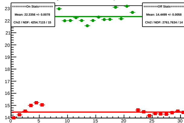
Cycle 4591.6: Multiplet Sums
