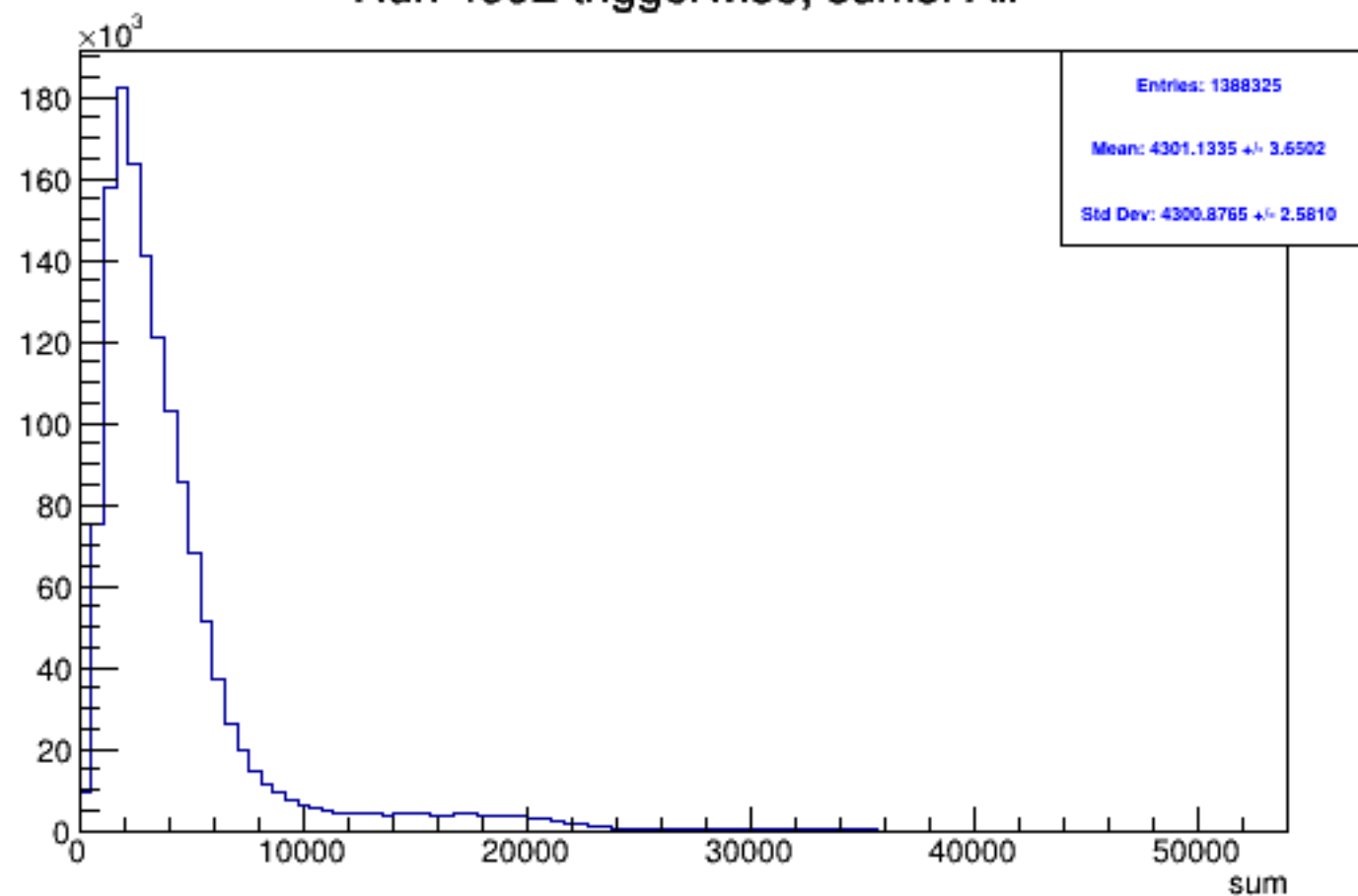
Run 4592 triggerwise, sums: All
