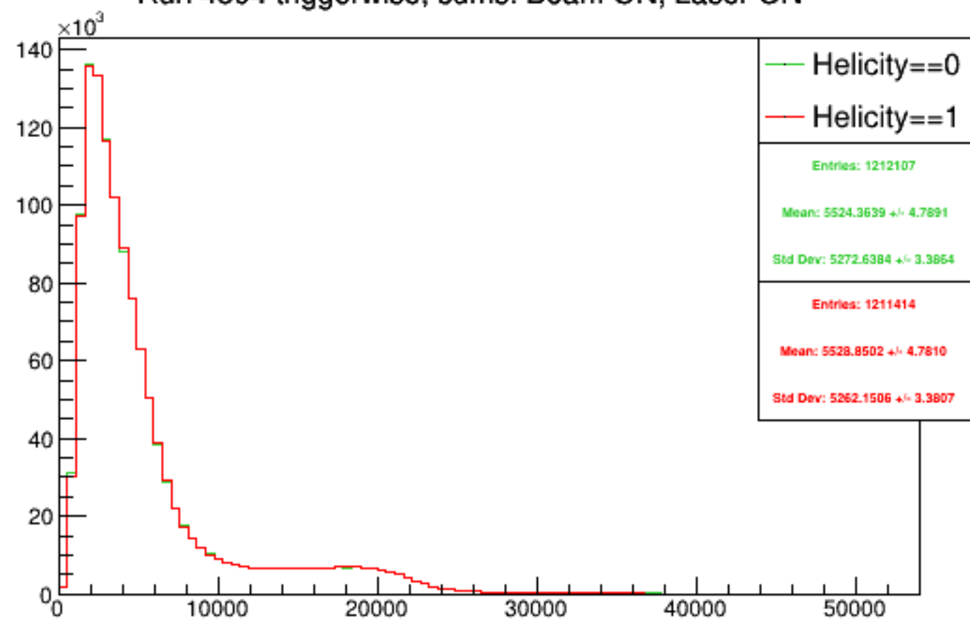
Run 4594 triggerwise, sums: Beam ON, Laser ON
