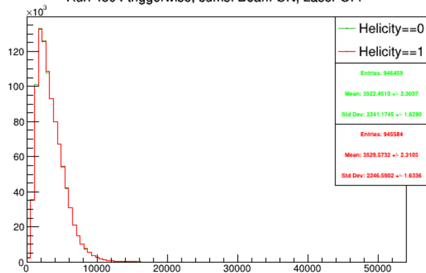
Run 4594 triggerwise, sums: Beam ON, Laser OFF
