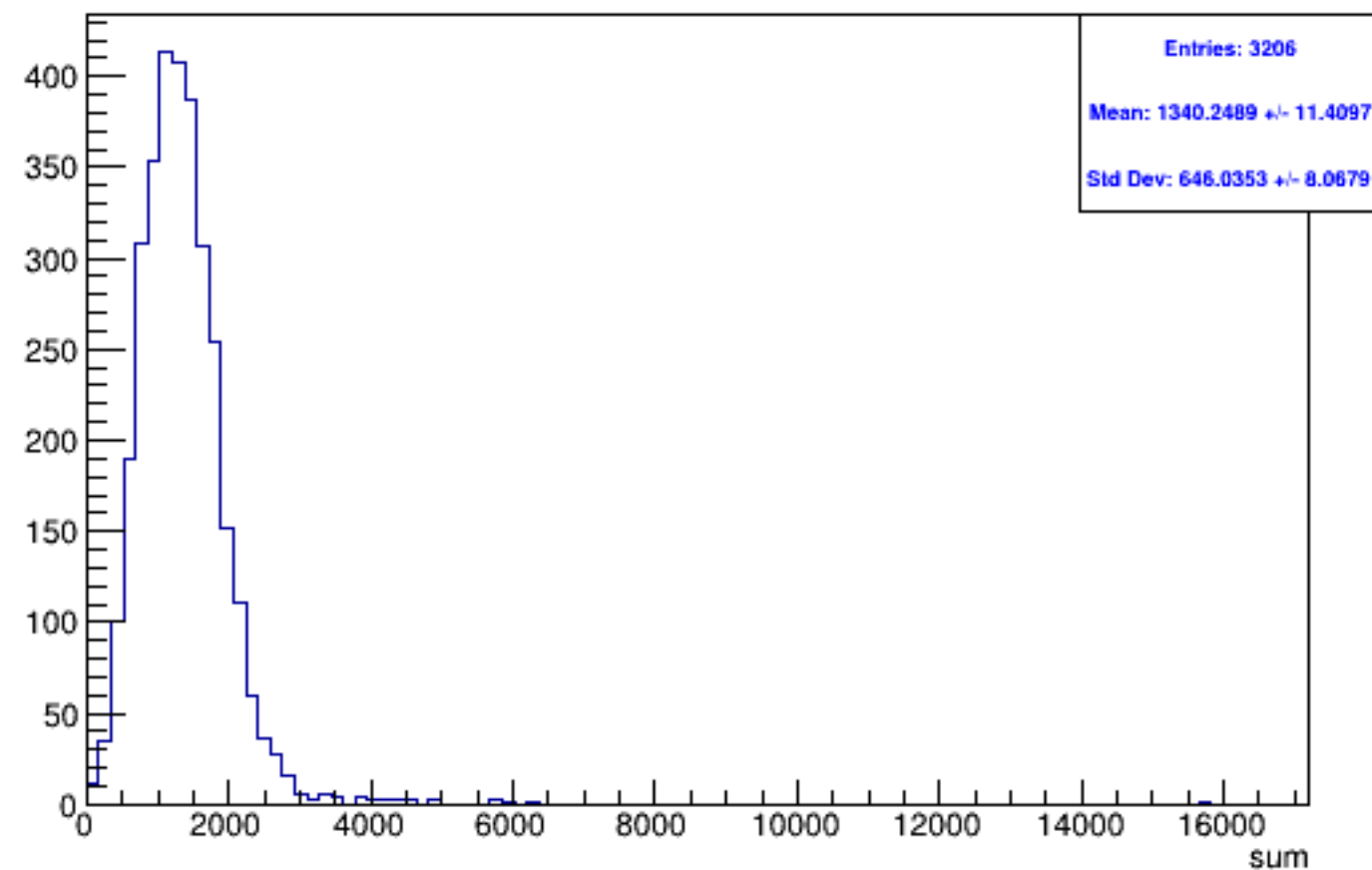
Run 4594 triggerwise, sums: Beam OFF
