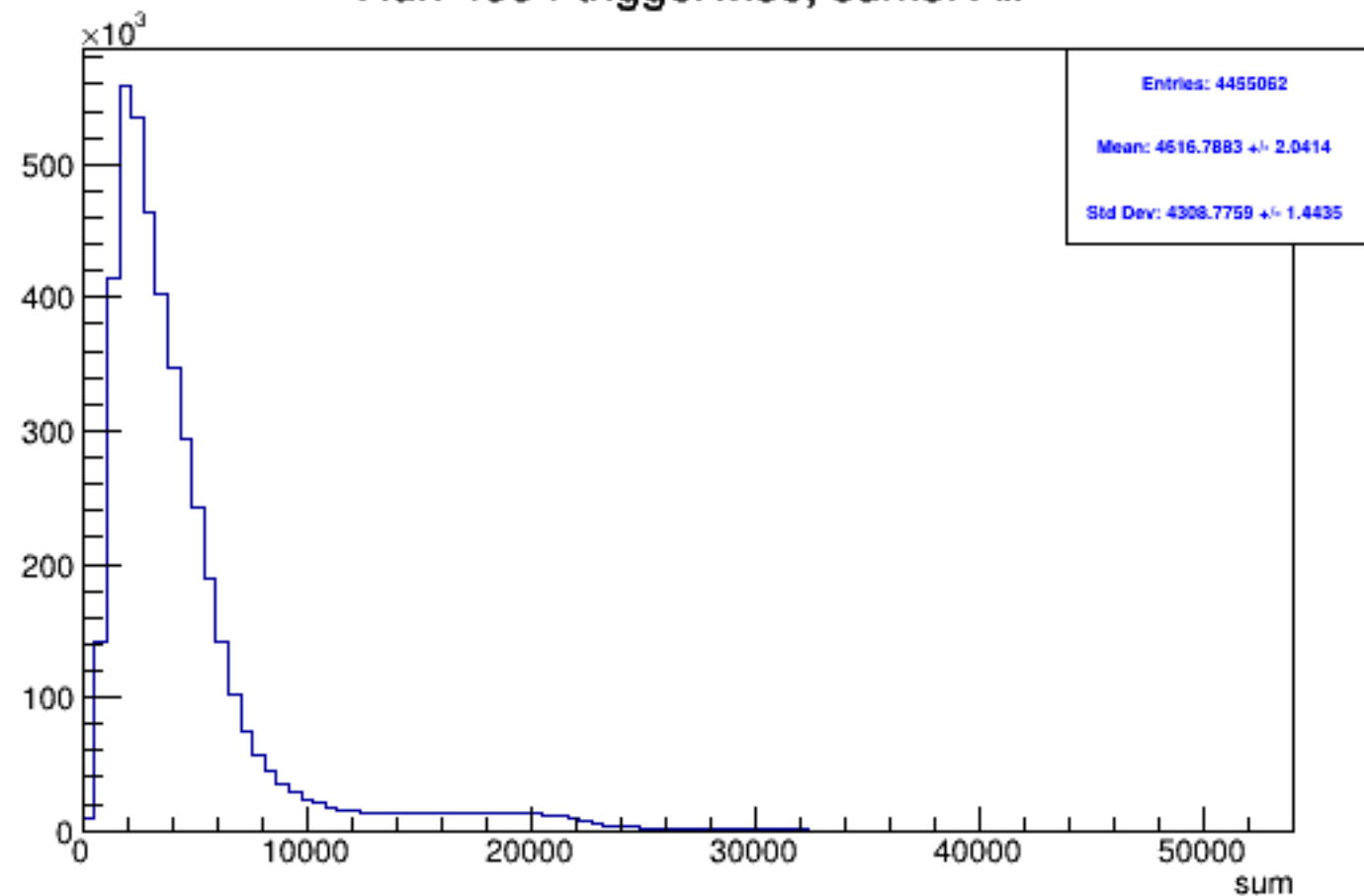
Run 4594 triggerwise, sums: All
