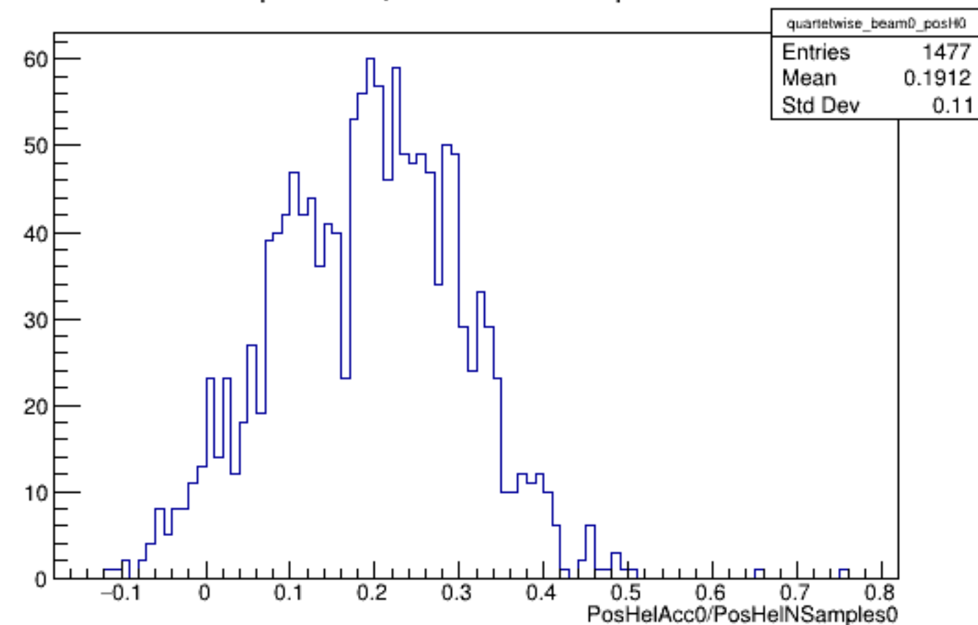
Run 4599 quartetwise, PosHelAcc0/NSamples0: Beam OFF
