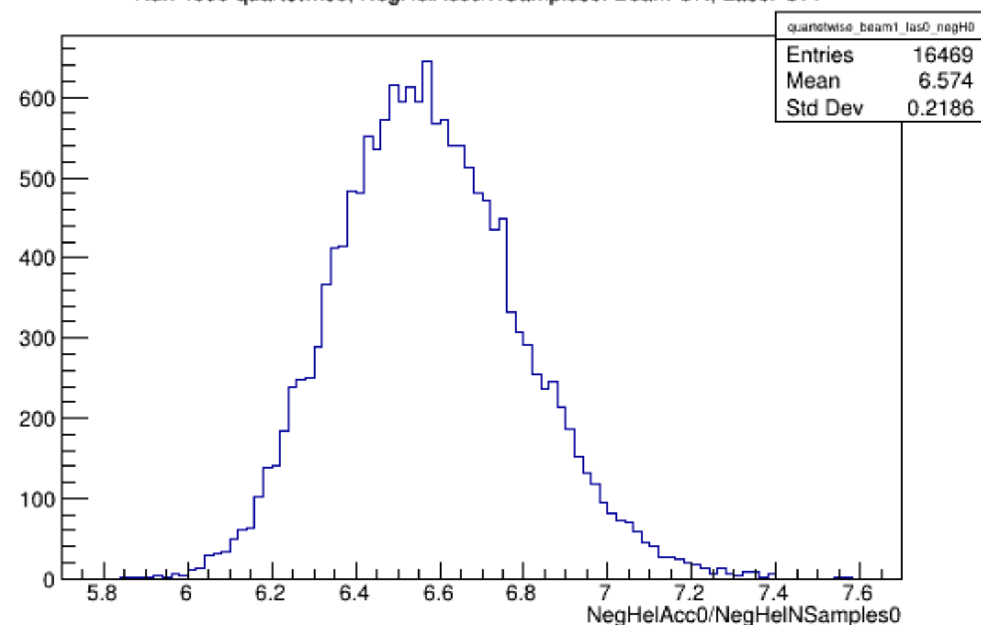
Run 4599 quartetwise, NegHelAcc0/NSamples0: Beam ON, Laser OFF
