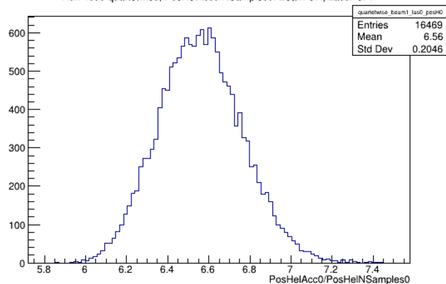
Run 4599 quartetwise, PosHelAcc0/NSamples0: Beam ON, Laser OFF
