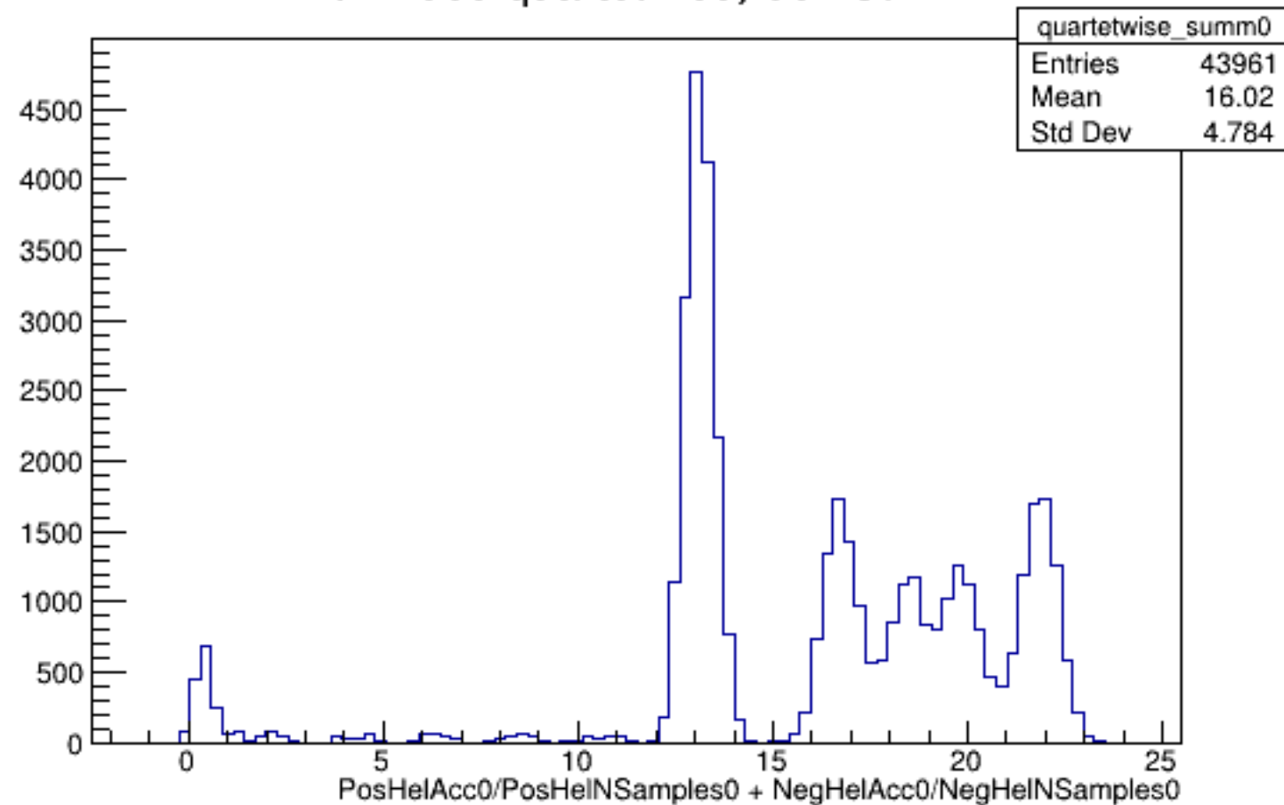
Run 4599 quartetwise, Sums0: All
