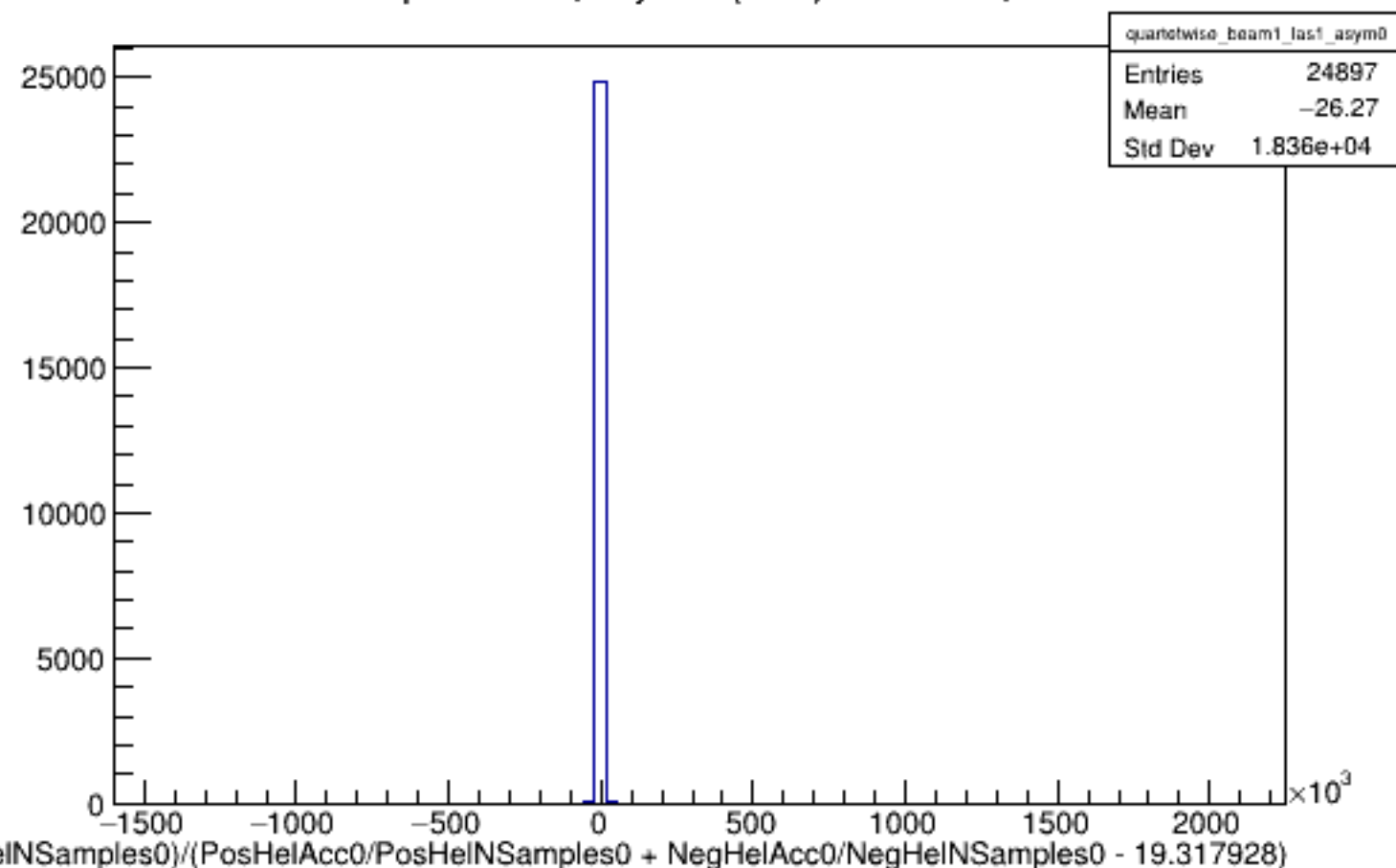
Run 4599 quartetwise, Asyms0 (Raw): Beam ON, Laser ON
