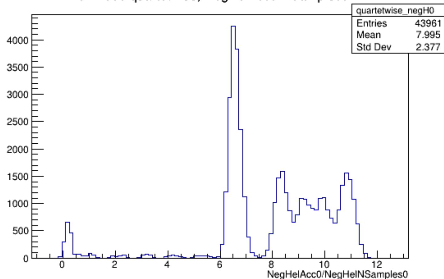
Run 4599 quartetwise, NegHelAcc0/NSamples0: All
