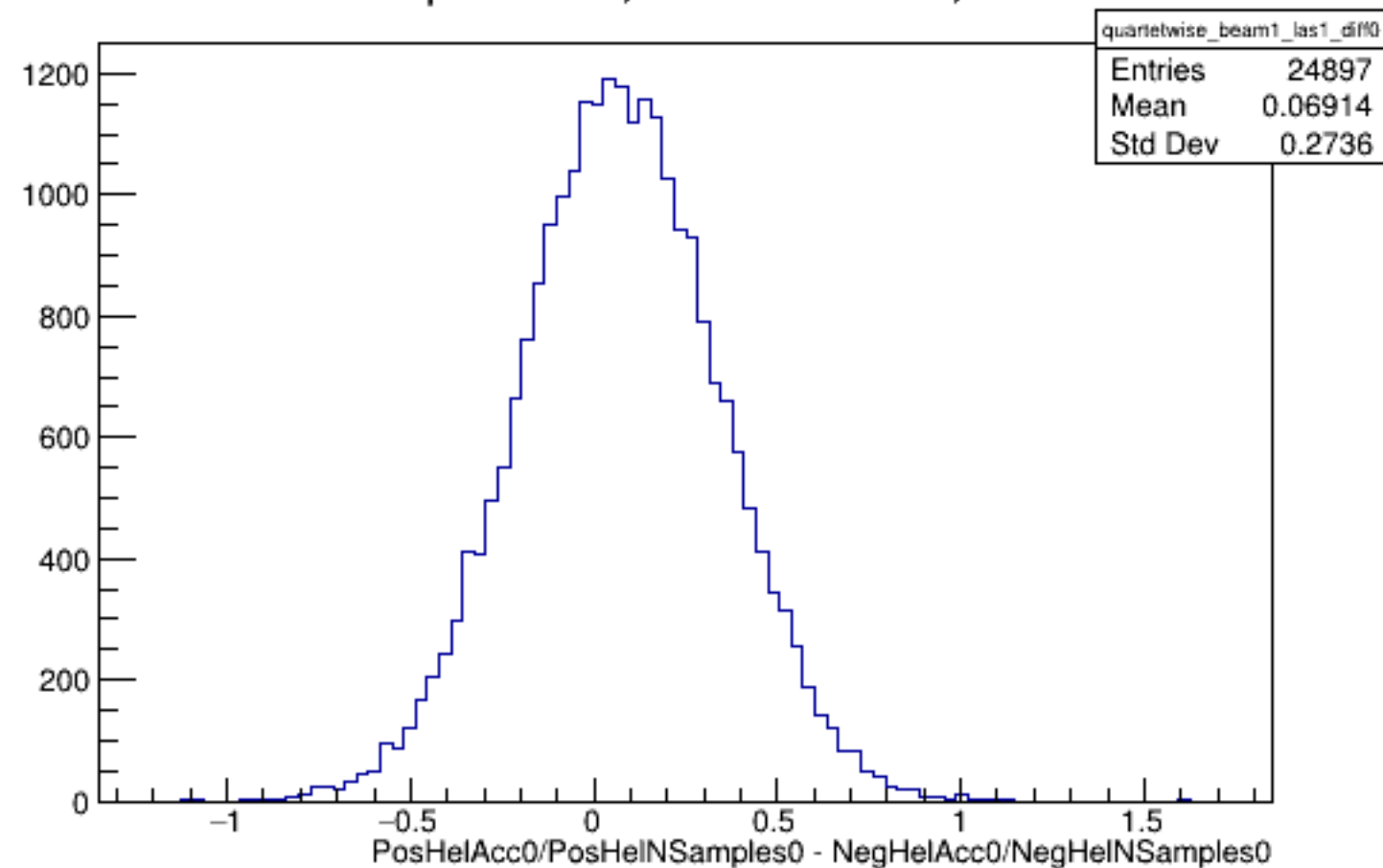
Run 4599 quartetwise, Diffs0: Beam ON, Laser ON
