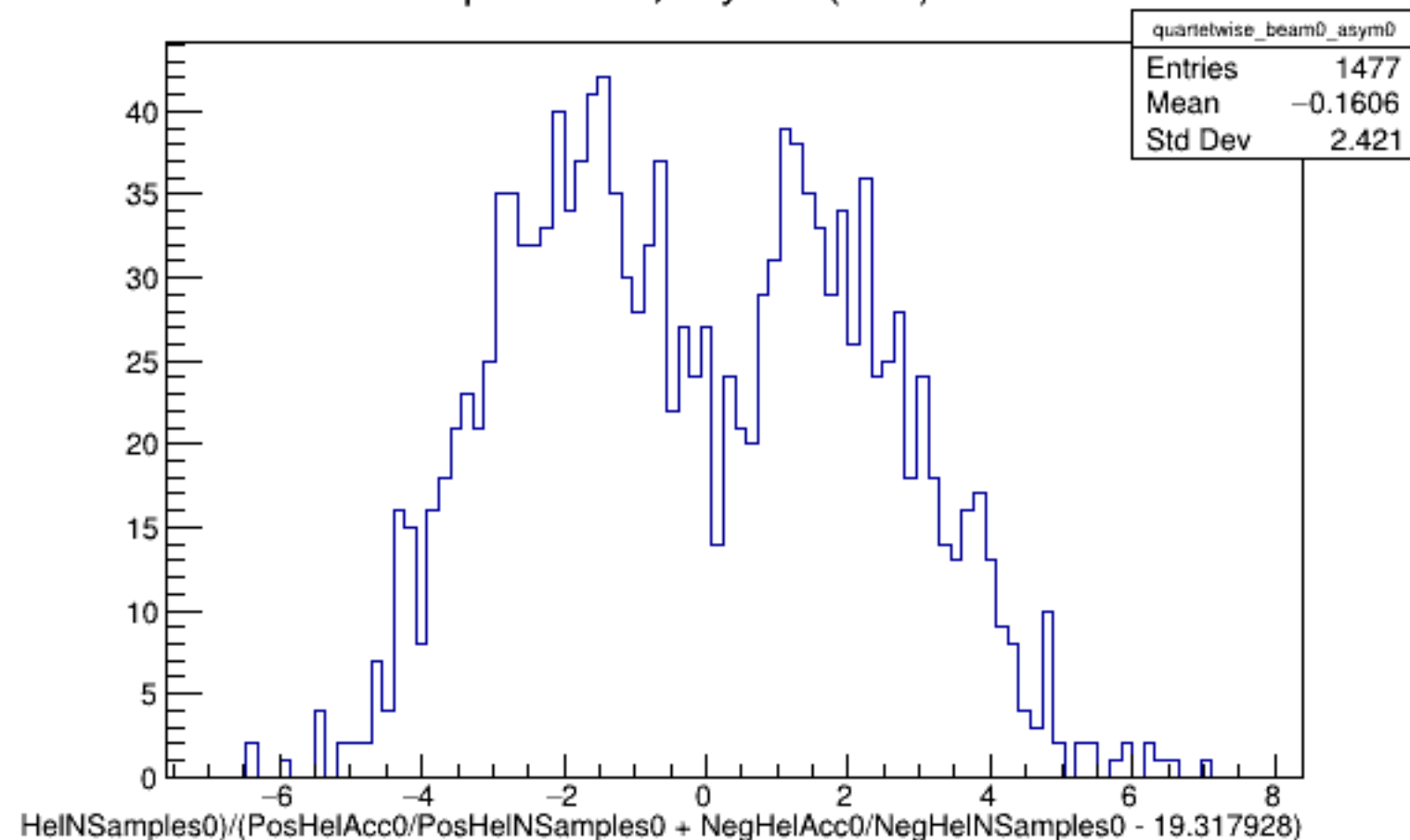
Run 4599 quartetwise, Asyms0 (Raw): Beam OFF
