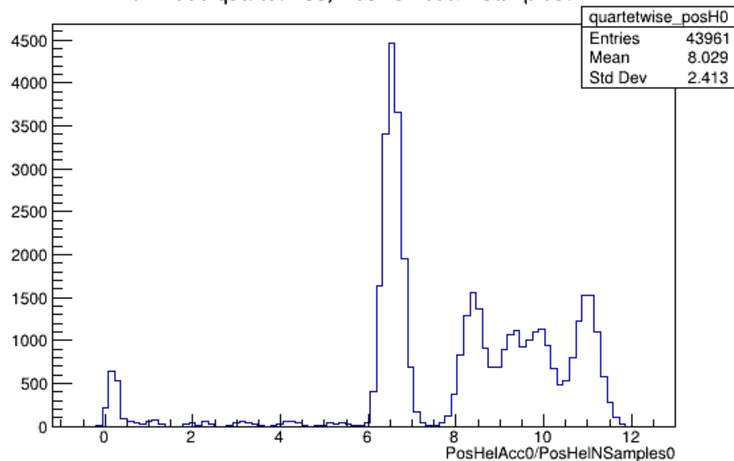
Run 4599 quartetwise, PosHelAcc0/NSamples0: All
