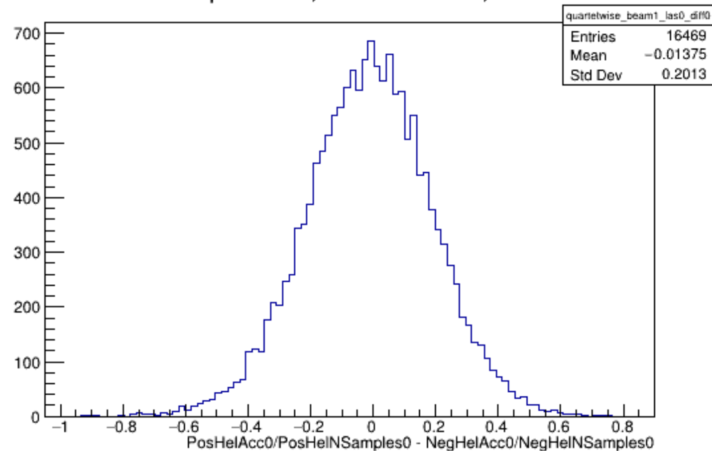
Run 4599 quartetwise, Diffs0: Beam ON, Laser OFF
