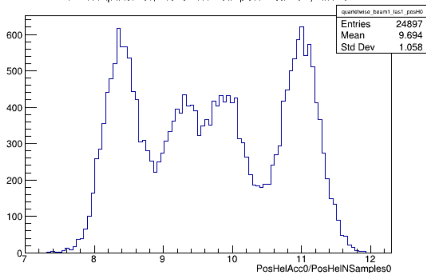
Run 4599 quartetwise, PosHelAcc0/NSamples0: Beam ON, Laser ON
