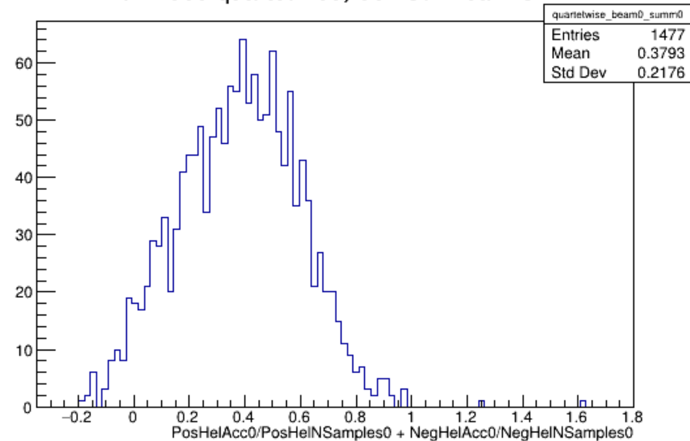
Run 4599 quartetwise, Sums0: Beam OFF
