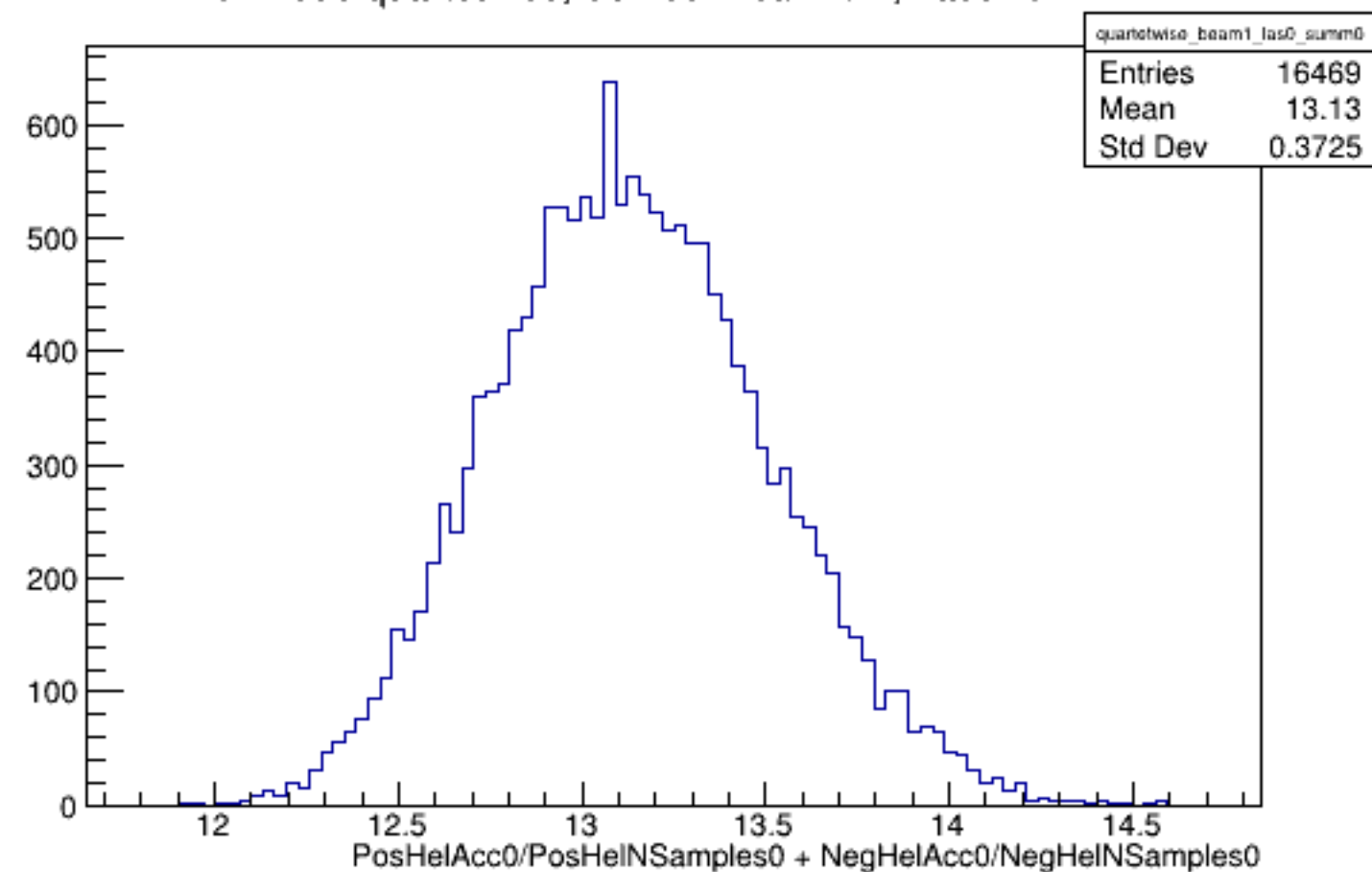
Run 4599 quartetwise, Sums0: Beam ON, Laser OFF
