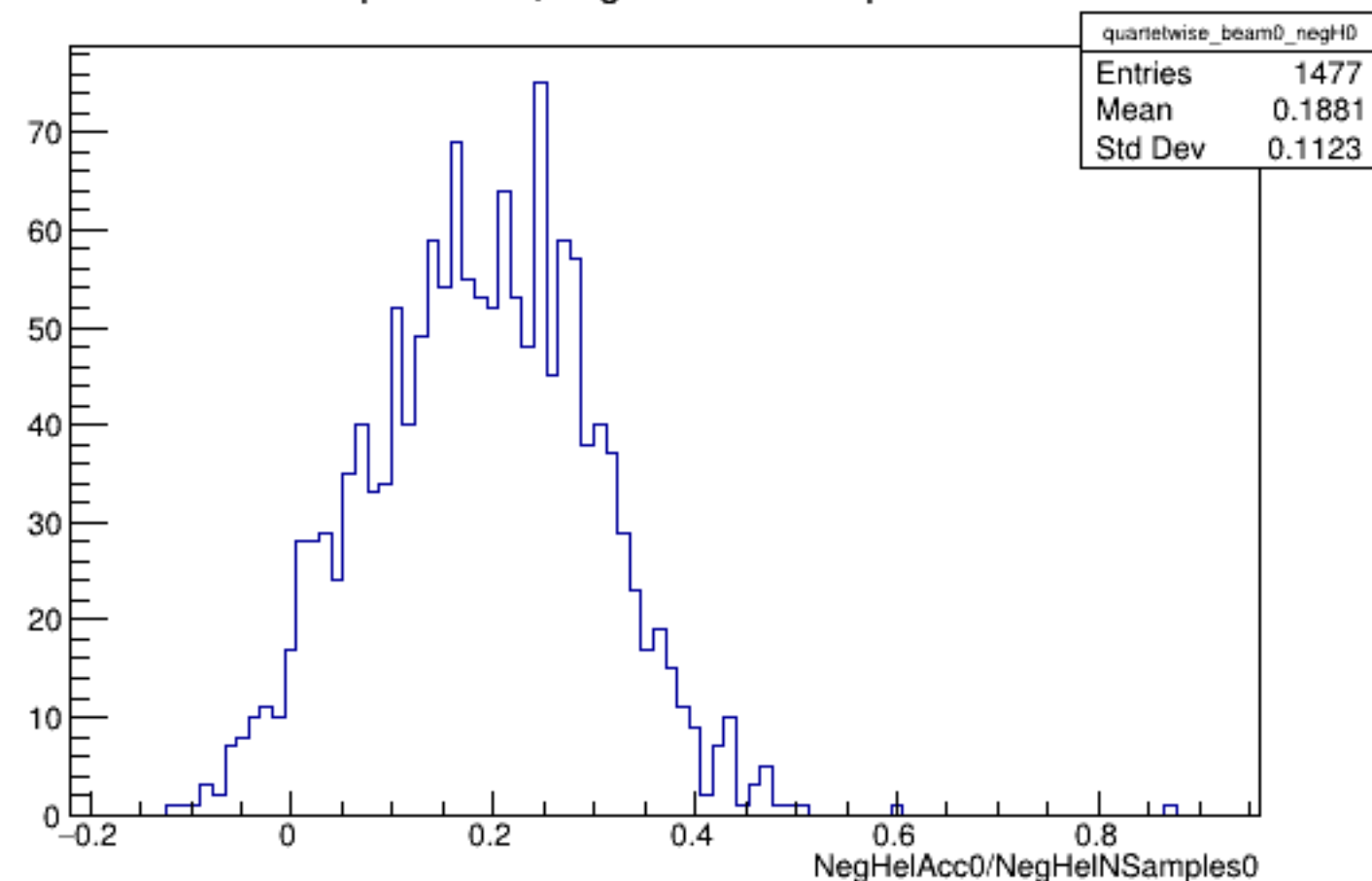
Run 4599 quartetwise, NegHelAcc0/NSamples0: Beam OFF
