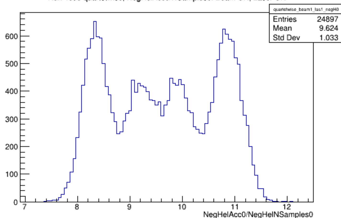
Run 4599 quartetwise, NegHelAcc0/NSamples0: Beam ON, Laser ON
