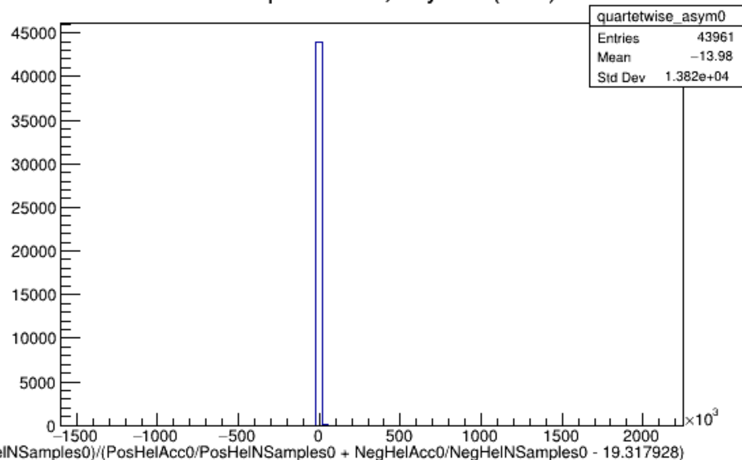
Run 4599 quartetwise, Asyms0 (Raw): All
