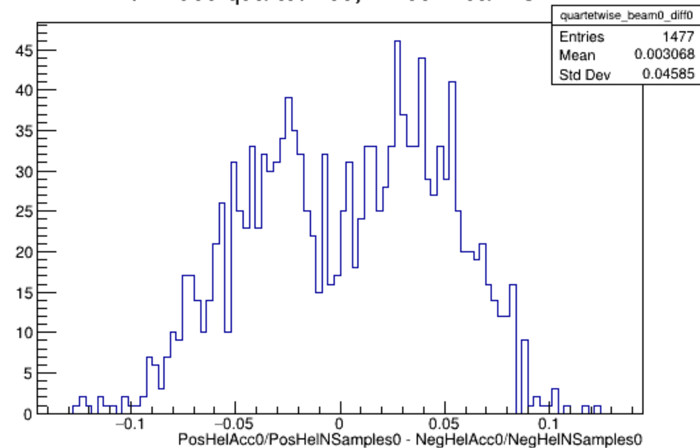
Run 4599 quartetwise, Diffs0: Beam OFF
