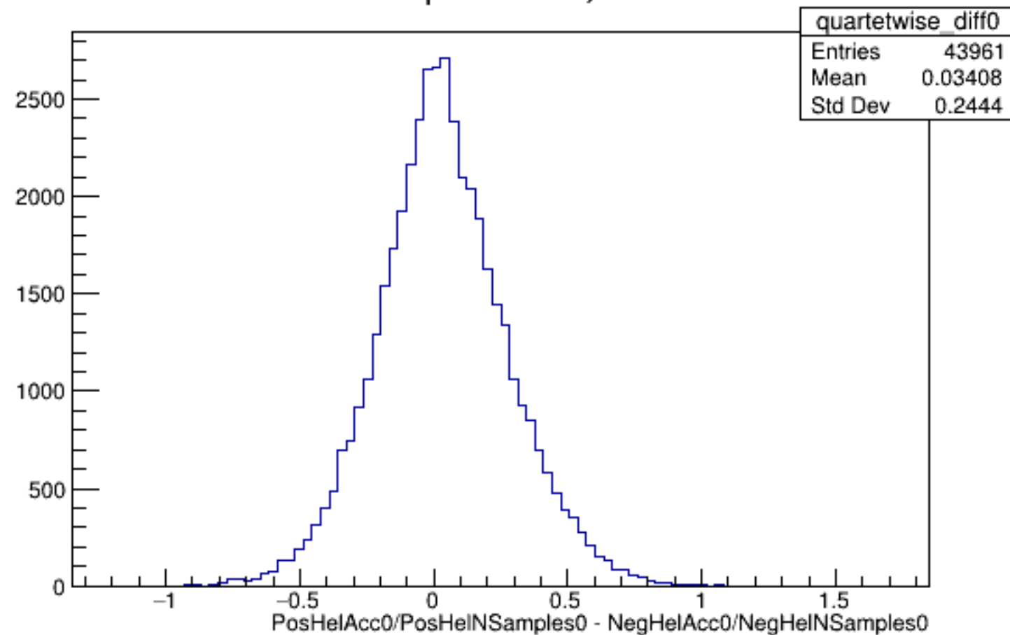
Run 4599 quartetwise, Diffs0: All
