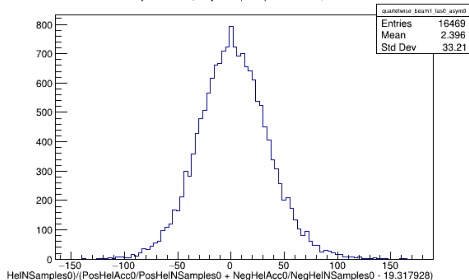
Run 4599 quartetwise, Asyms0 (Raw): Beam ON, Laser OFF
