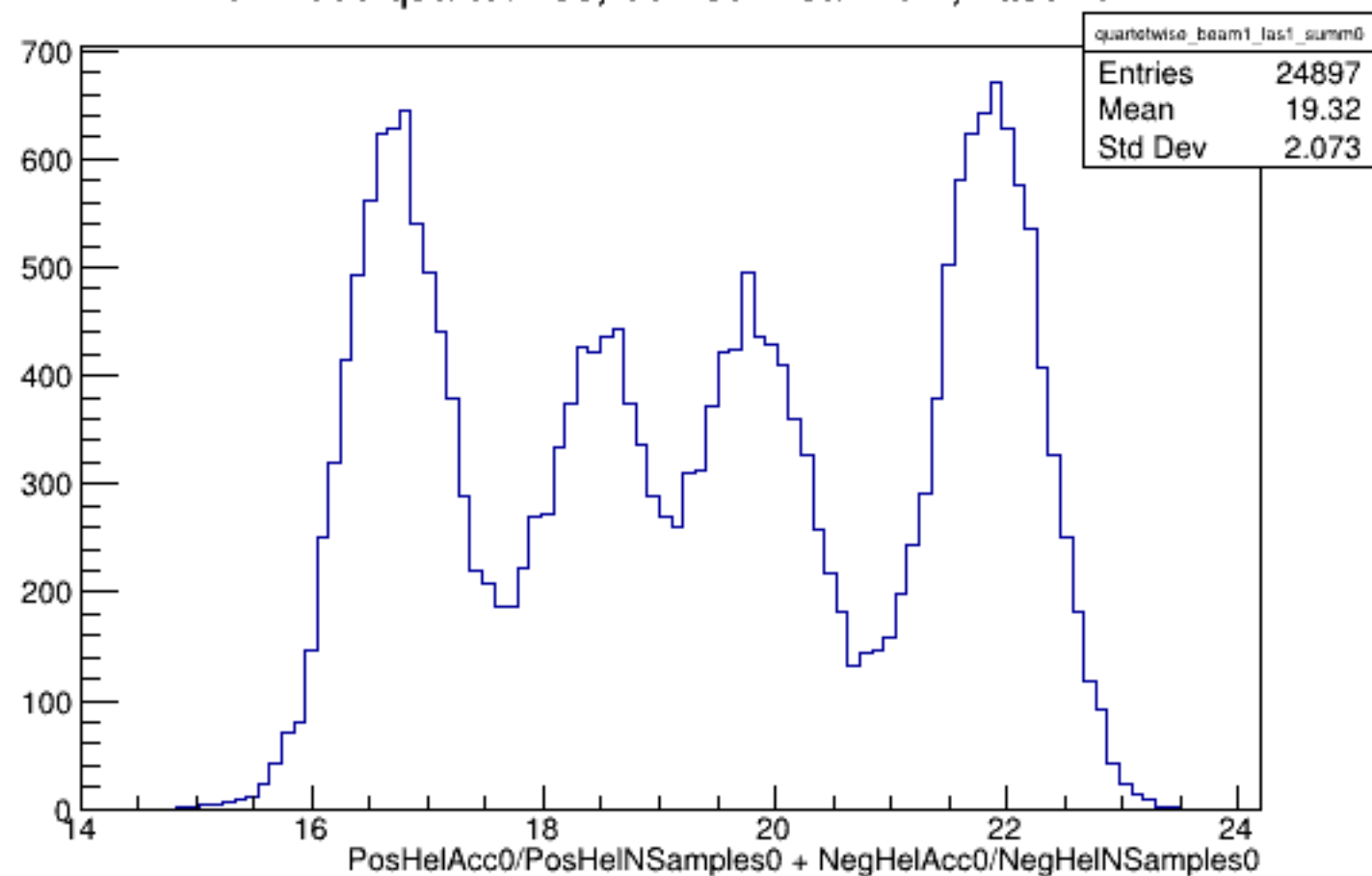
Run 4599 quartetwise, Sums0: Beam ON, Laser ON
