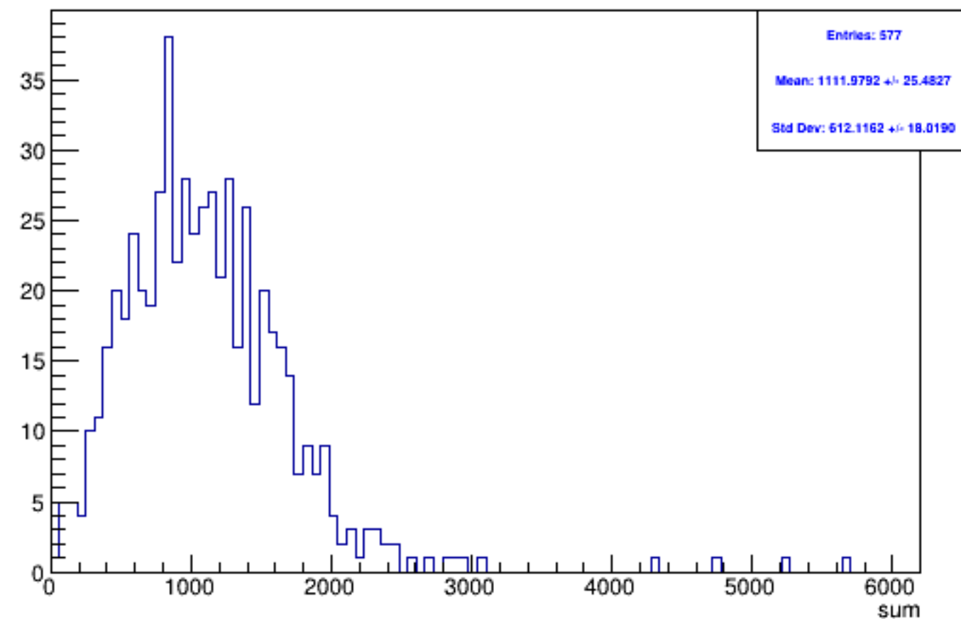
Run 4599 triggerwise, sums: Beam OFF
