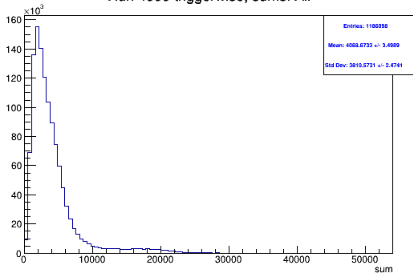
Run 4599 triggerwise, sums: All
