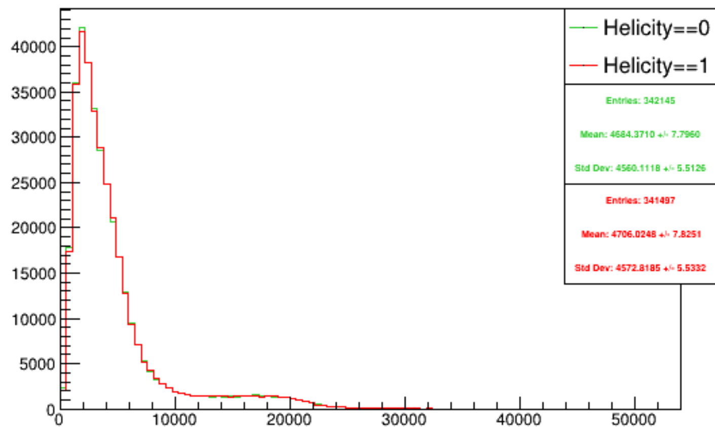
Run 4599 triggerwise, sums: Beam ON, Laser ON
