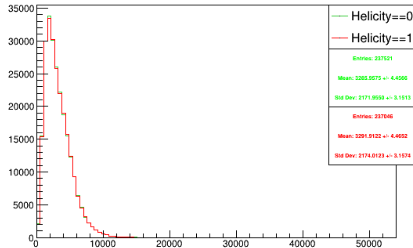
Run 4599 triggerwise, sums: Beam ON, Laser OFF
