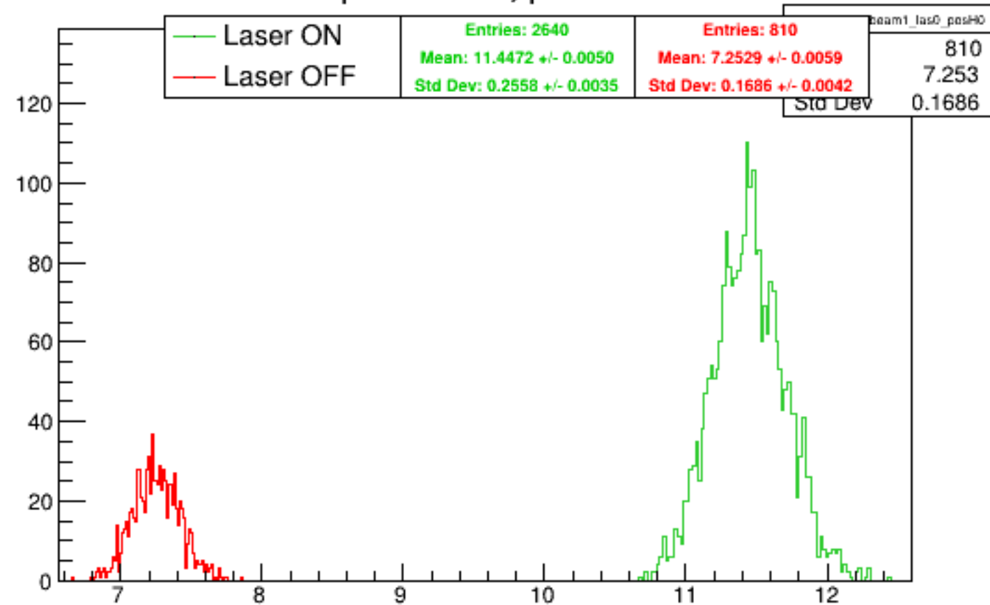
Run 4606 quartetwise, posH0: Beam ON
