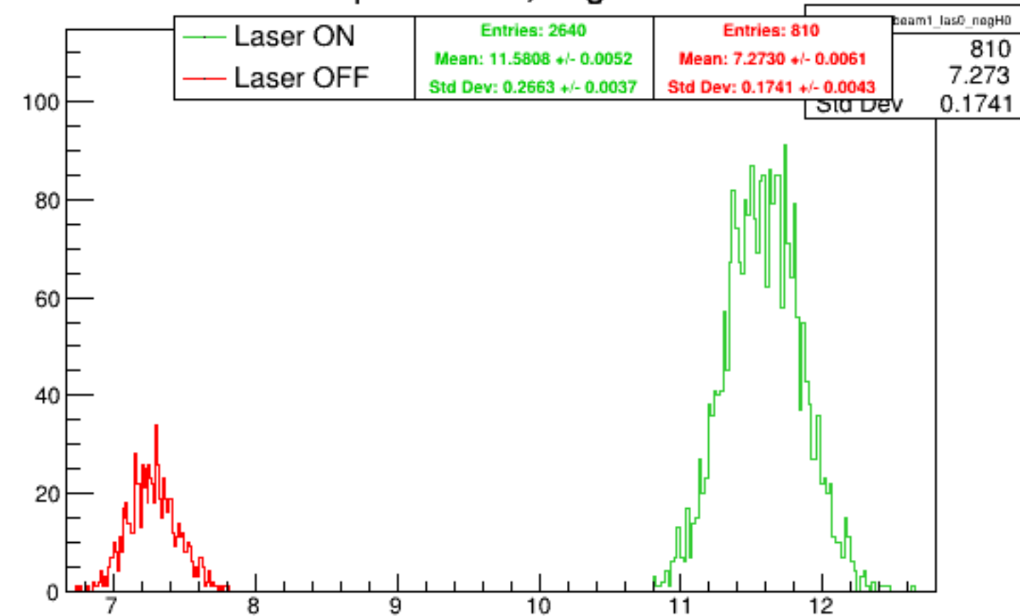
Run 4606 quartetwise, negH0: Beam ON
