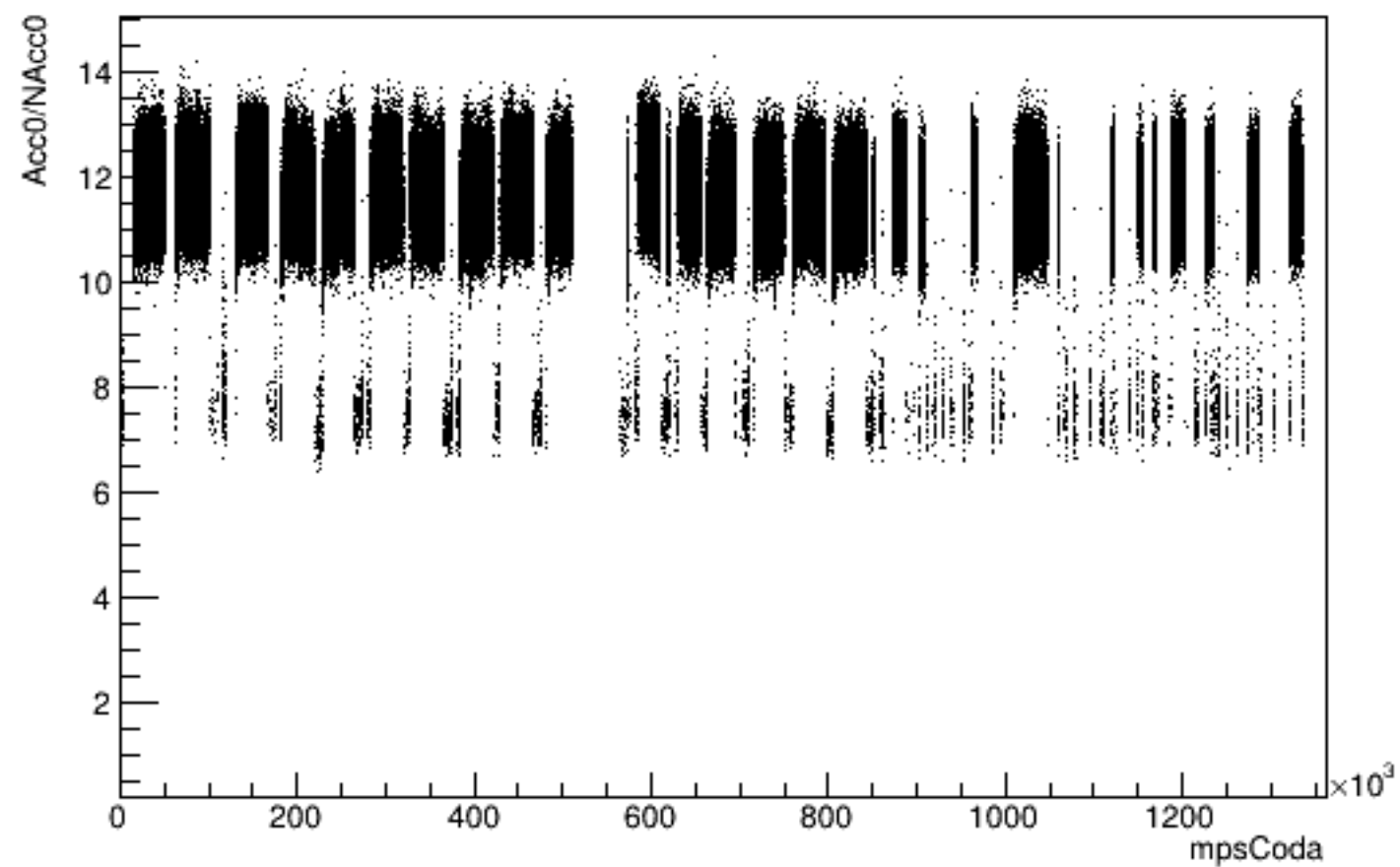
Run 4608 mpwise, Acc0/NAcc0:mpsCoda, beam ON, laser ON
