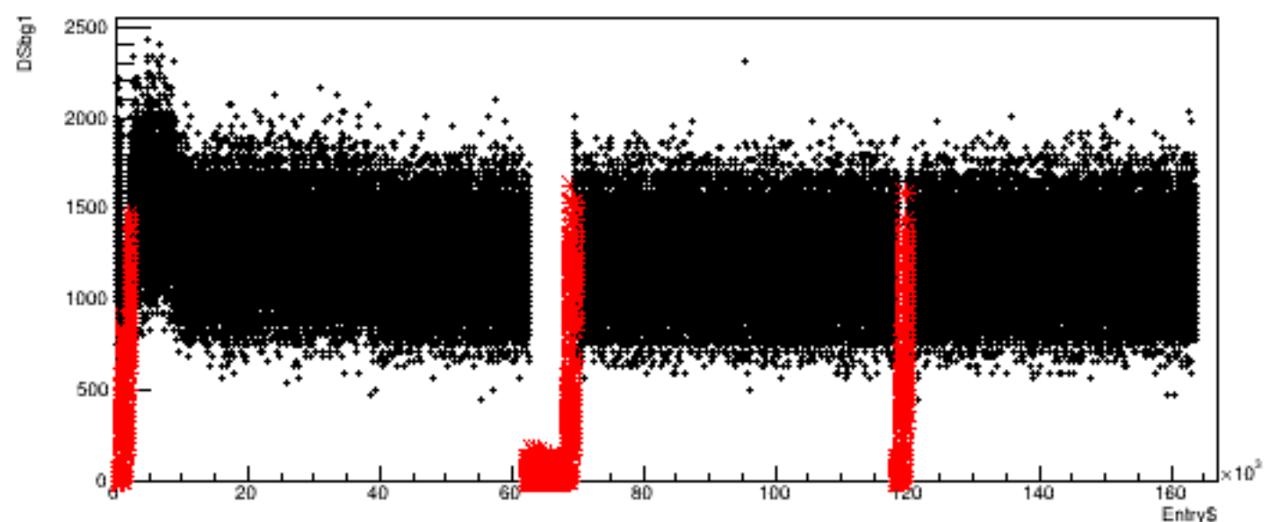
Run 4608, quartetwise: DSbg1 vs time
