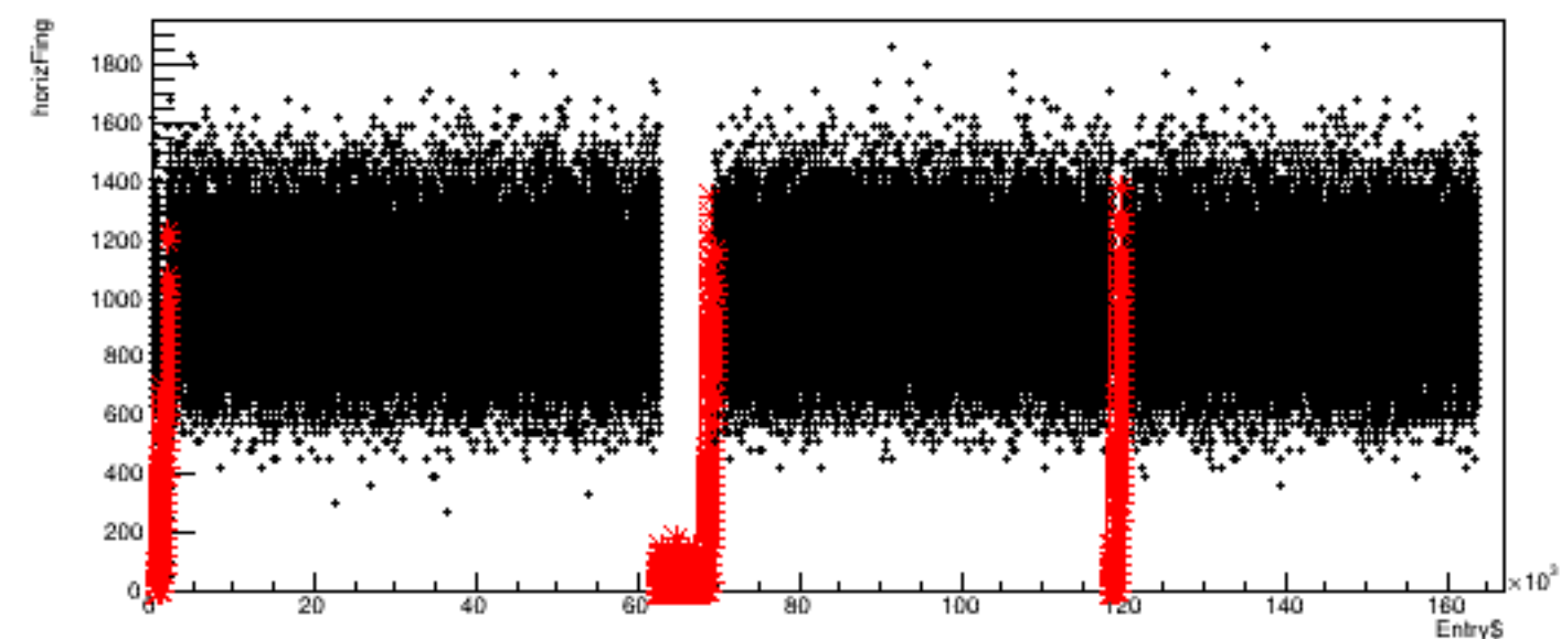
Run 4608, quartetwise: horizFing vs time
