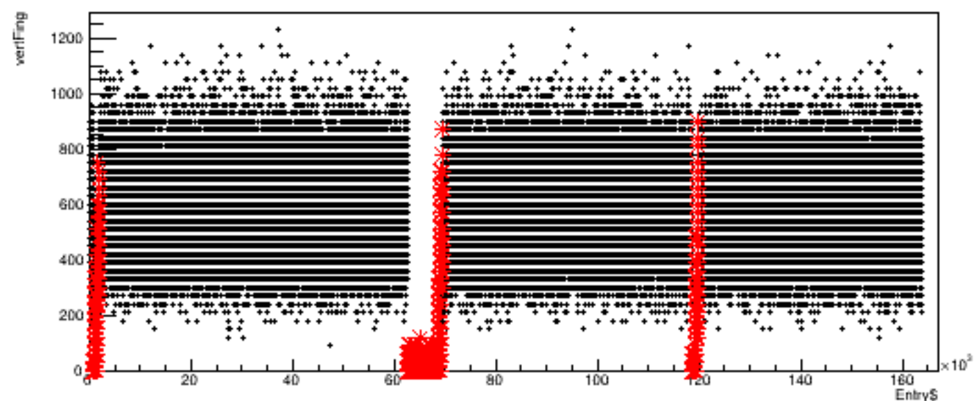
Run 4608, quartetwise: vertFing vs time
