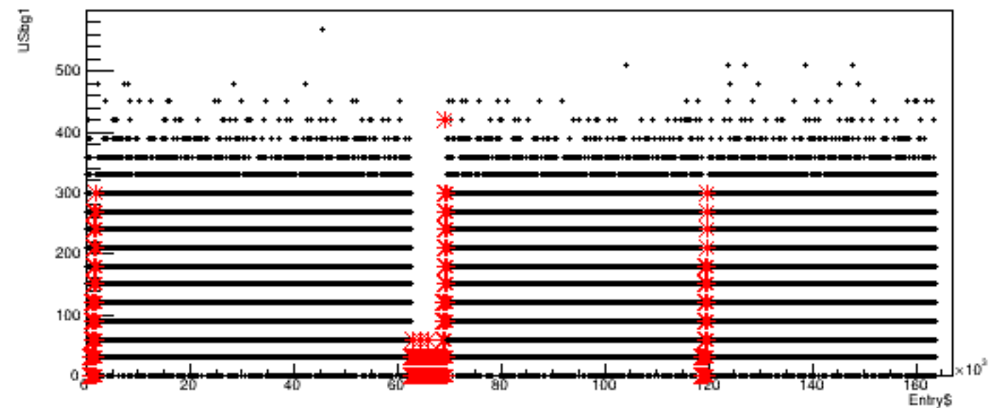
Run 4608, quartetwise: USbg1 vs time
