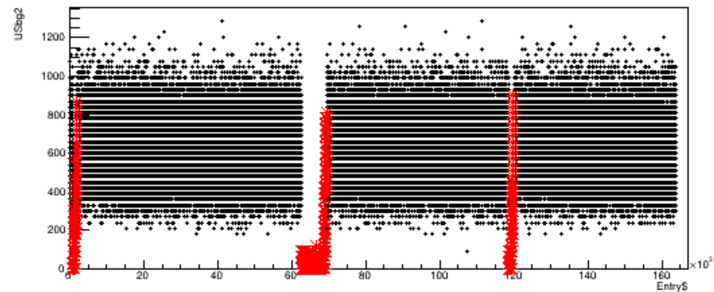
Run 4608, quartetwise: USbg2 vs time
