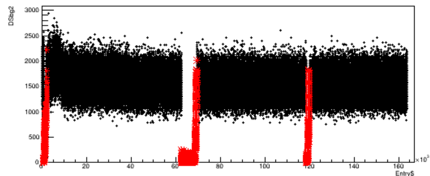
Run 4608, quartetwise: DSbg2 vs time
