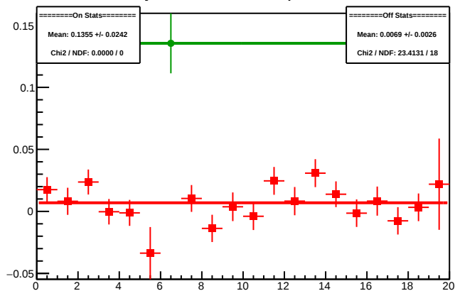
Cycle 4608.17: Multiplet Diffs
