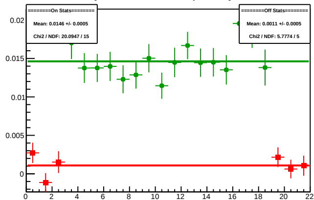
Cycle 4608.11: Multiplet Asyms
