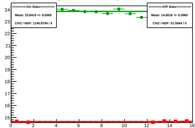
Cycle 4608.6: Multiplet Sums
