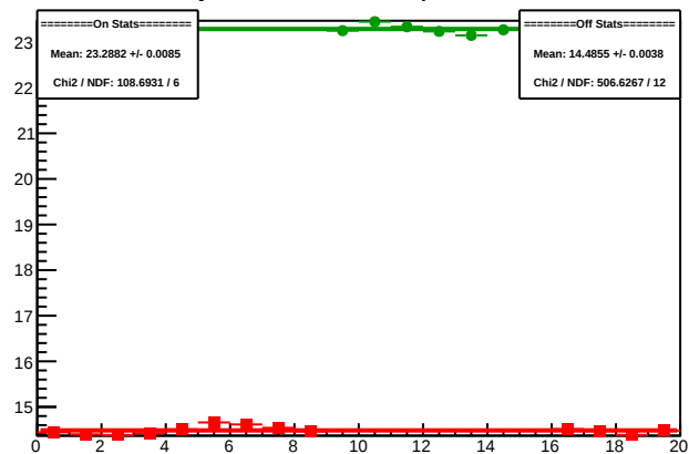
Cycle 4608.14: Multiplet Sums
