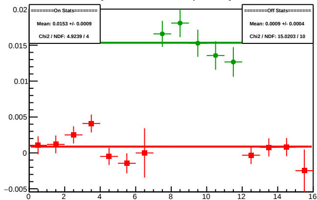
Cycle 4608.4: Multiplet Asyms
