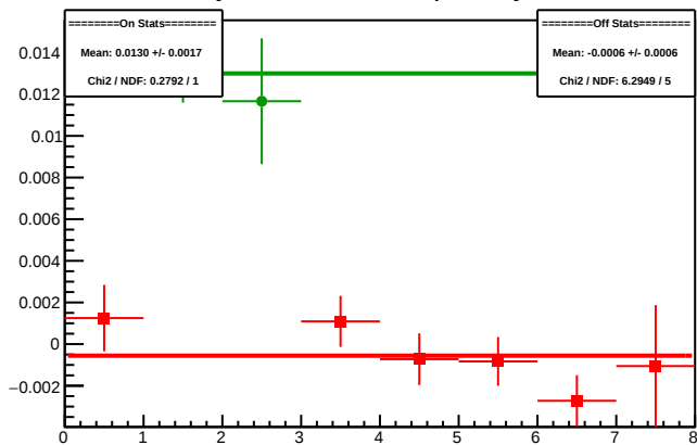
Cycle 4608.23: Multiplet Asyms
