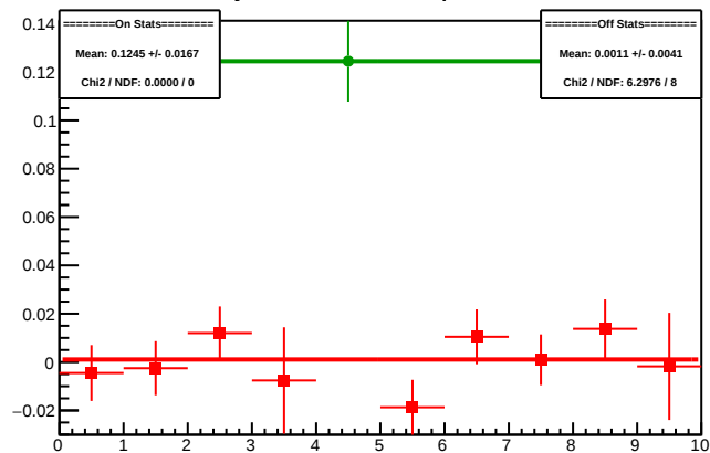
Cycle 4608.7: Multiplet Diffs
