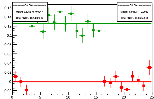
Cycle 4608.9: Multiplet Diffs
