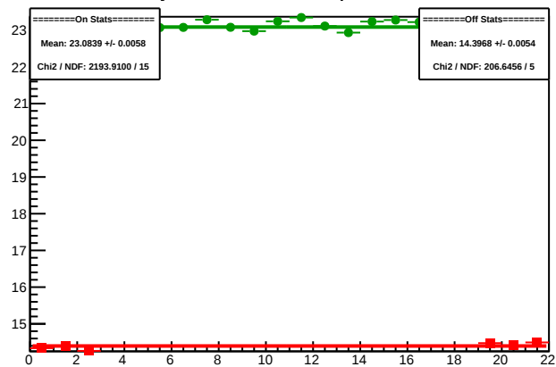
Cycle 4608.12: Multiplet Sums
