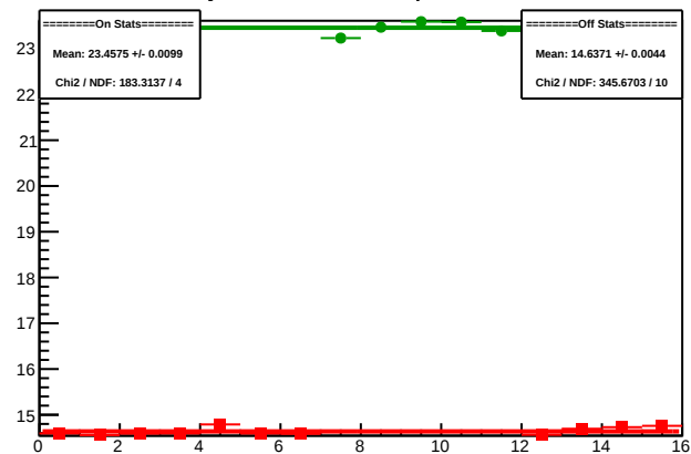
Cycle 4608.4: Multiplet Sums
