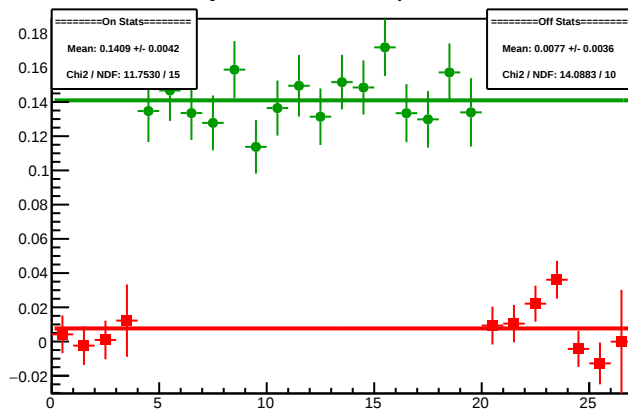
Cycle 4608.3: Multiplet Diffs
