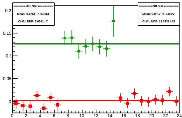
Cycle 4608.21: Multiplet Diff
