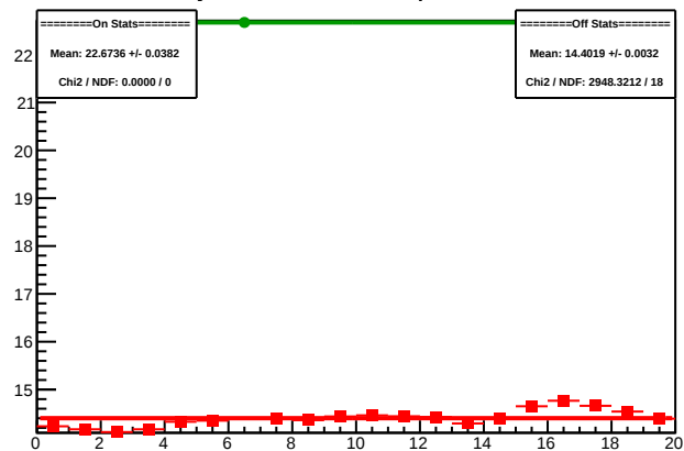
Cycle 4608.17: Multiplet Sums
