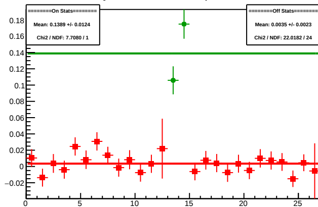
Cycle 4608.18: Multiplet Diffs
