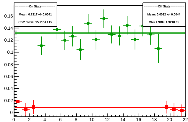
Cycle 4608.12: Multiplet Diffs
