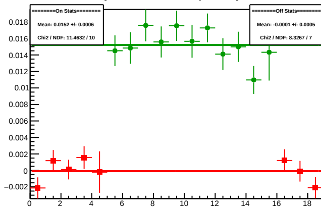
Cycle 4608.8: Multiplet Asyms
