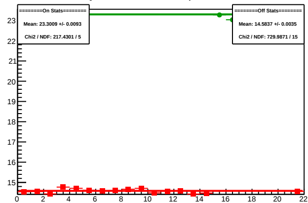
Cycle 4608.25: Multiplet Sums
