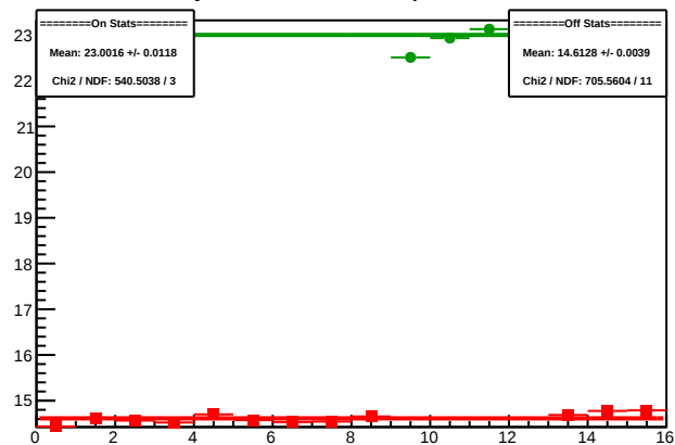
Cycle 4608.10: Multiplet Sums
