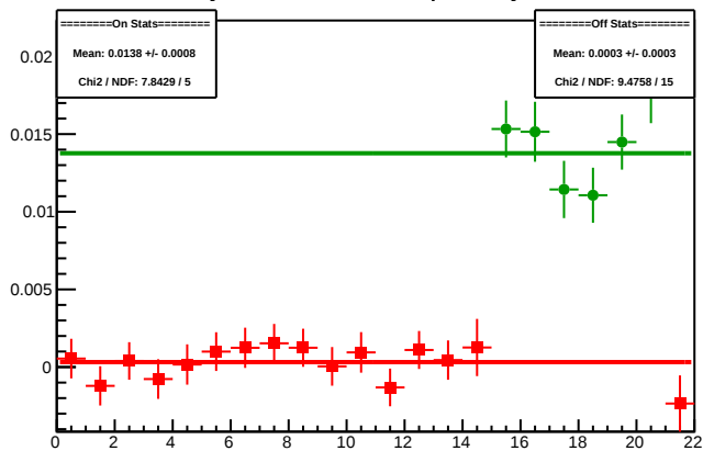
Cycle 4608.25: Multiplet Asyms
