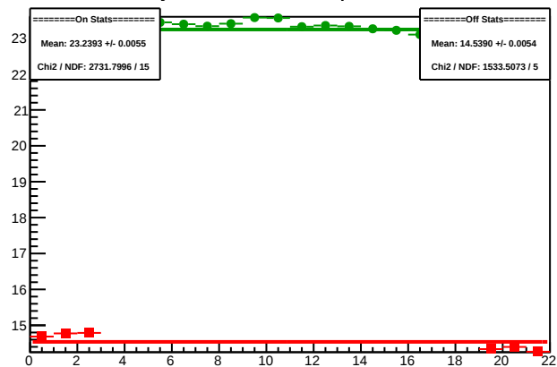
Cycle 4608.11: Multiplet Sums
