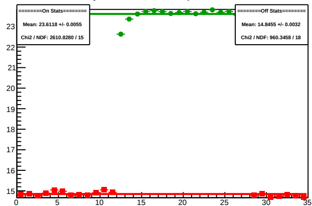
Cycle 4608.1: Multiplet Sums
