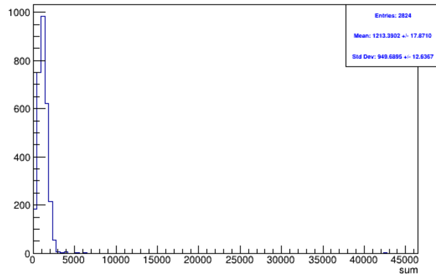
Run 4608 triggerwise, sums: Beam OFF
