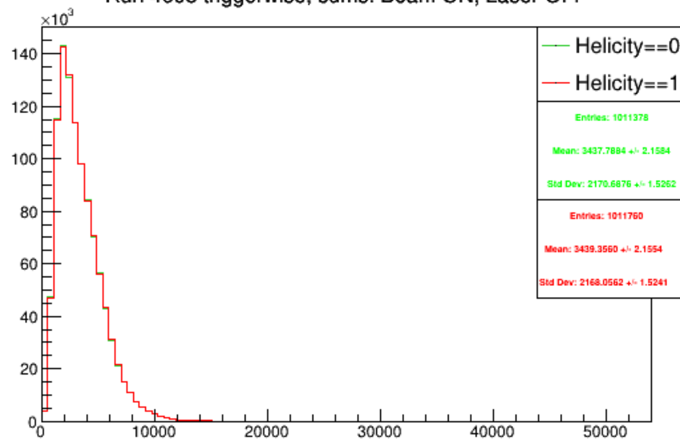
Run 4608 triggerwise, sums: Beam ON, Laser OFF
