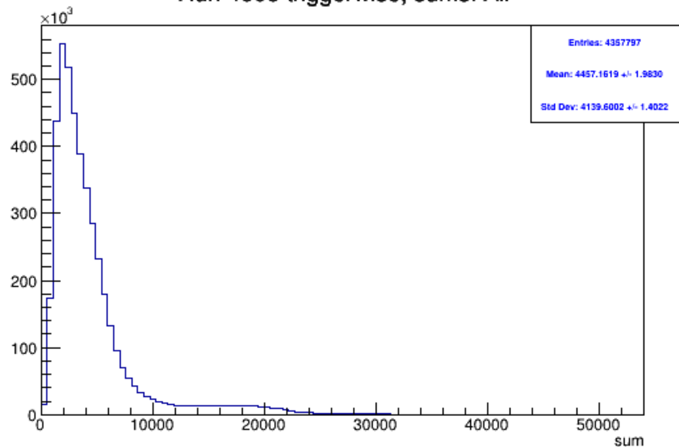
Run 4608 triggerwise, sums: All
