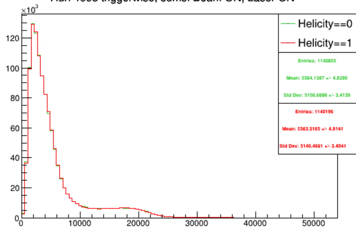
Run 4608 triggerwise, sums: Beam ON, Laser ON
