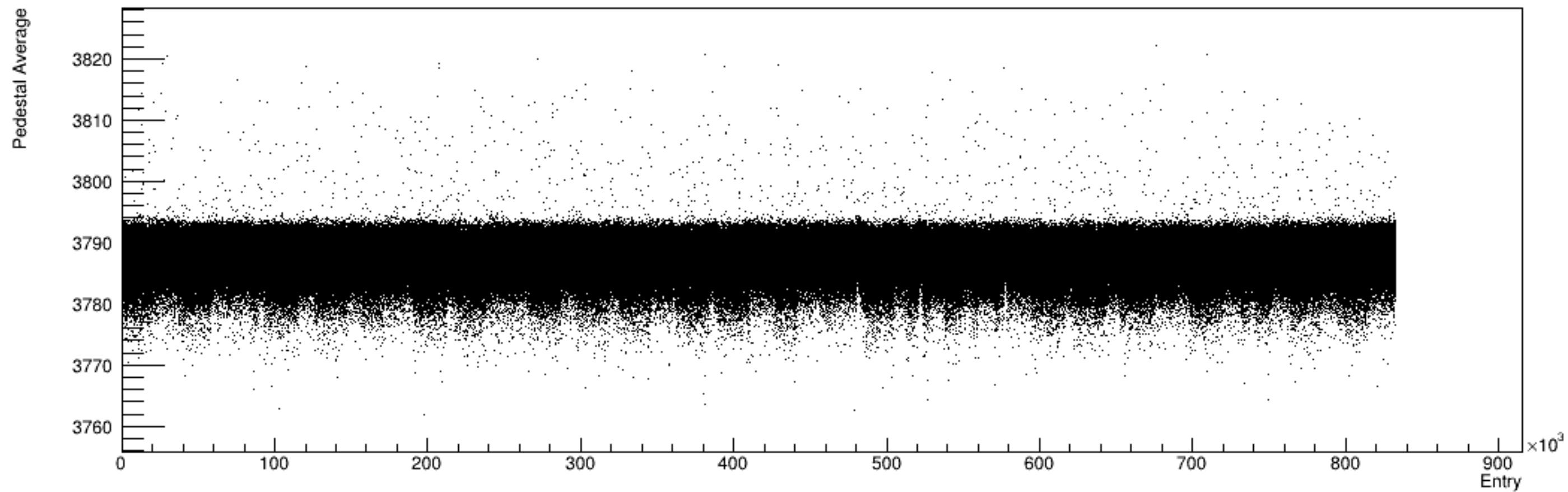
Run 4614, snapshots: Pedestal vs. Time
