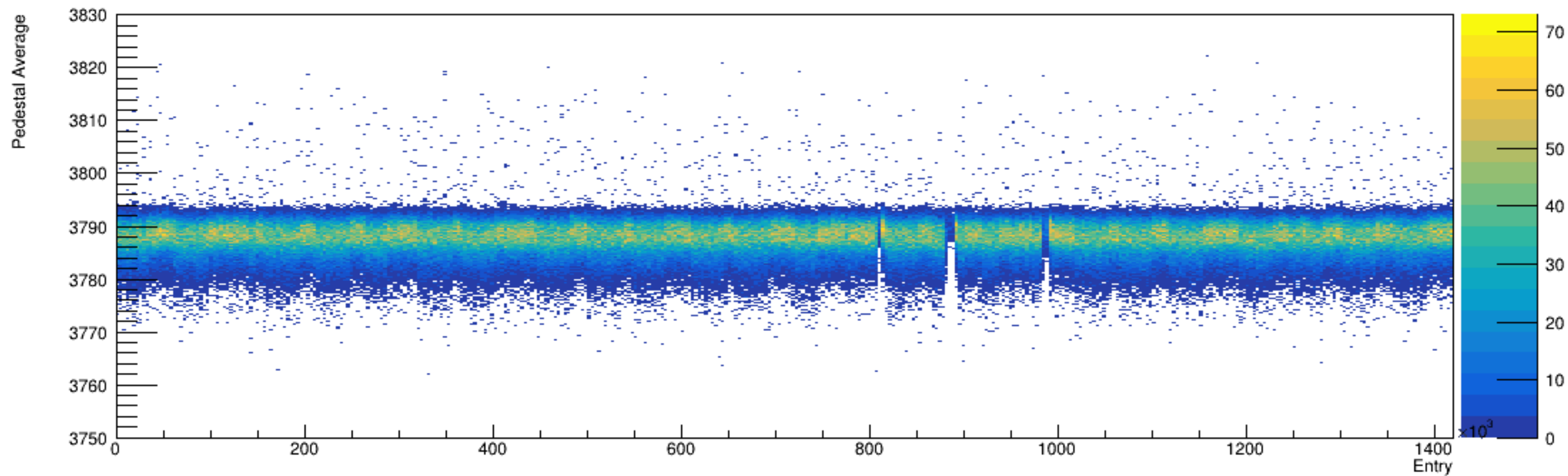
Run 4614, snapshots: Pedestal vs. Time
