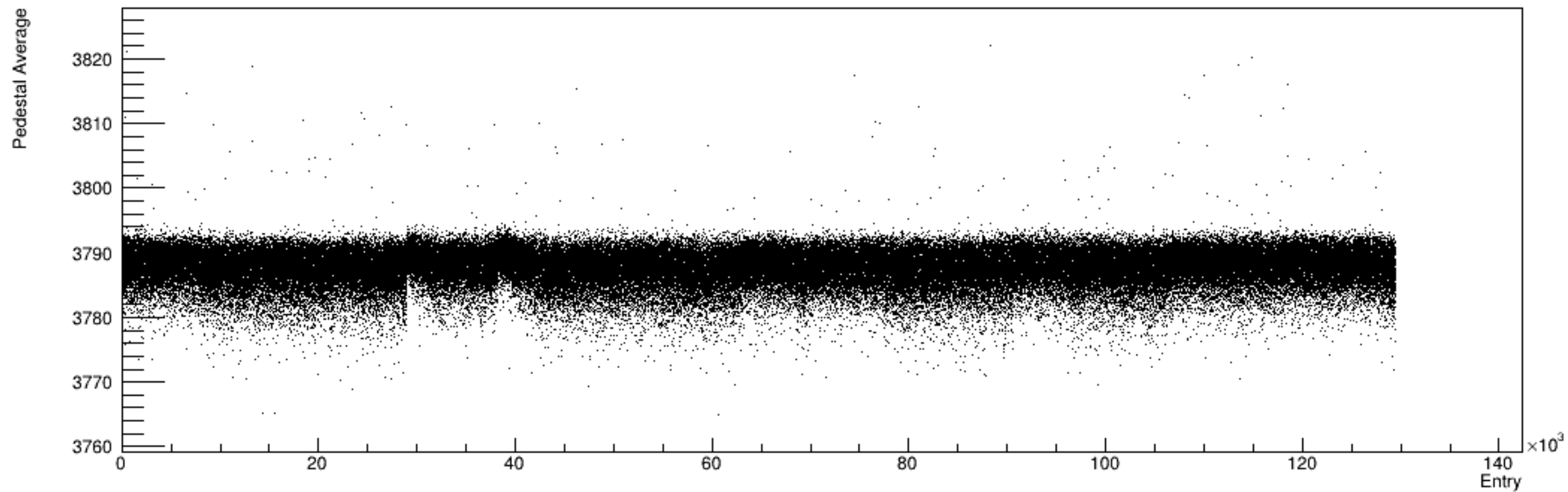
Run 4616, snapshots: Pedestal vs. Time
