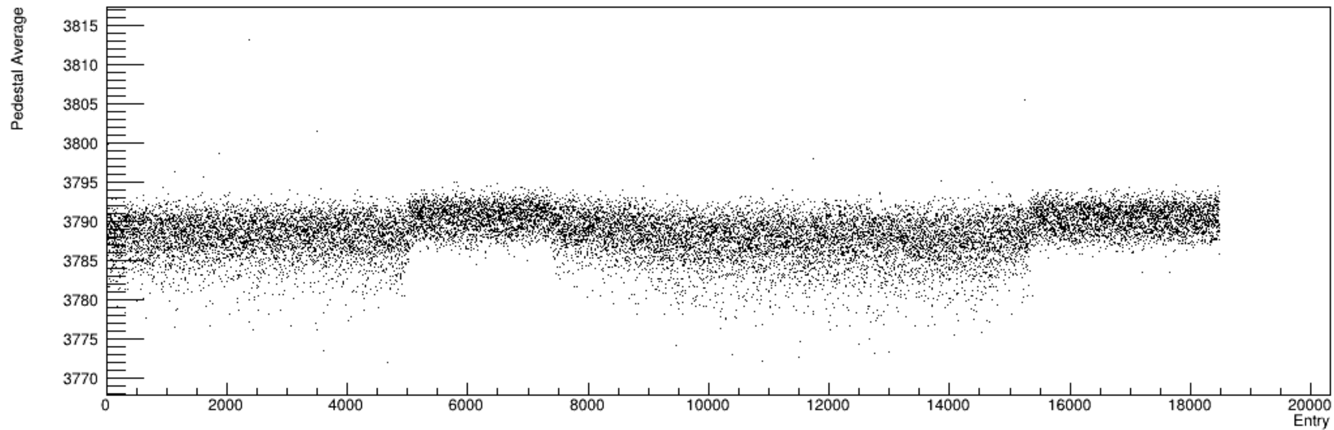
Run 4617, snapshots: Pedestal vs. Time
