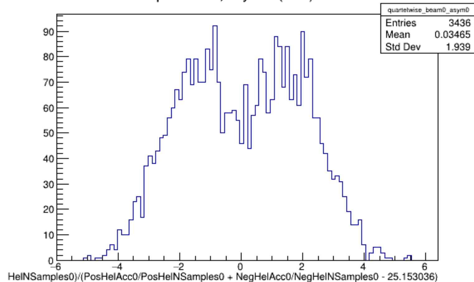
Run 4618 quartetwise, Asyms0 (Raw): Beam OFF
