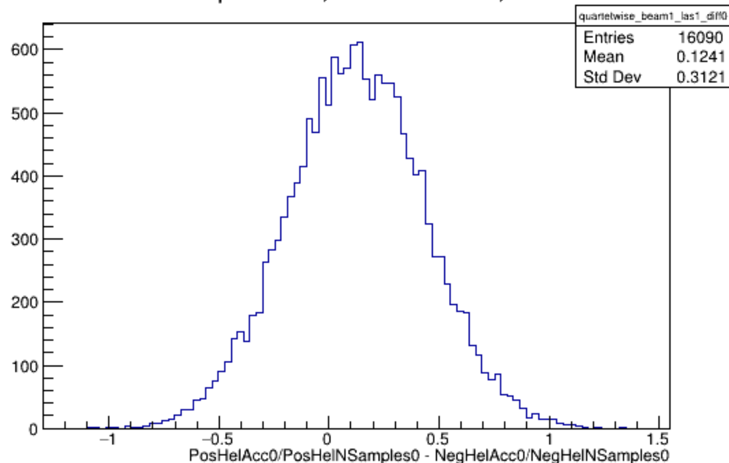
Run 4618 quartetwise, Diffs0: Beam ON, Laser ON
