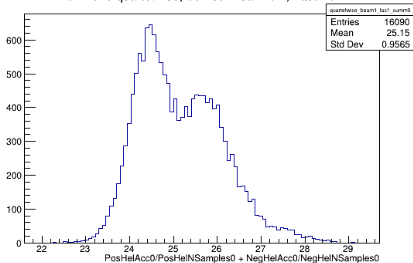
Run 4618 quartetwise, Sums0: Beam ON, Laser ON
