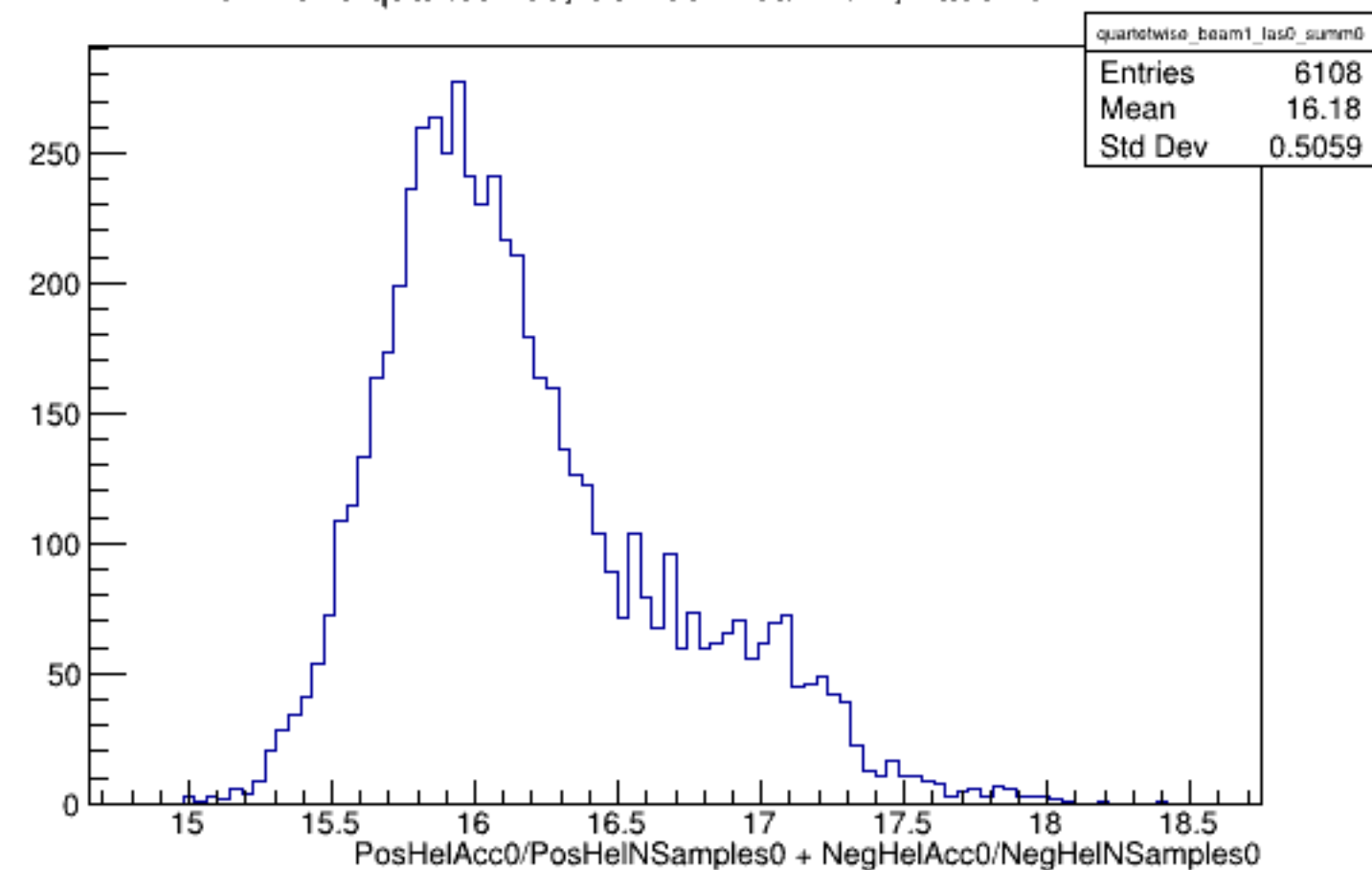
Run 4618 quartetwise, Sums0: Beam ON, Laser OFF
