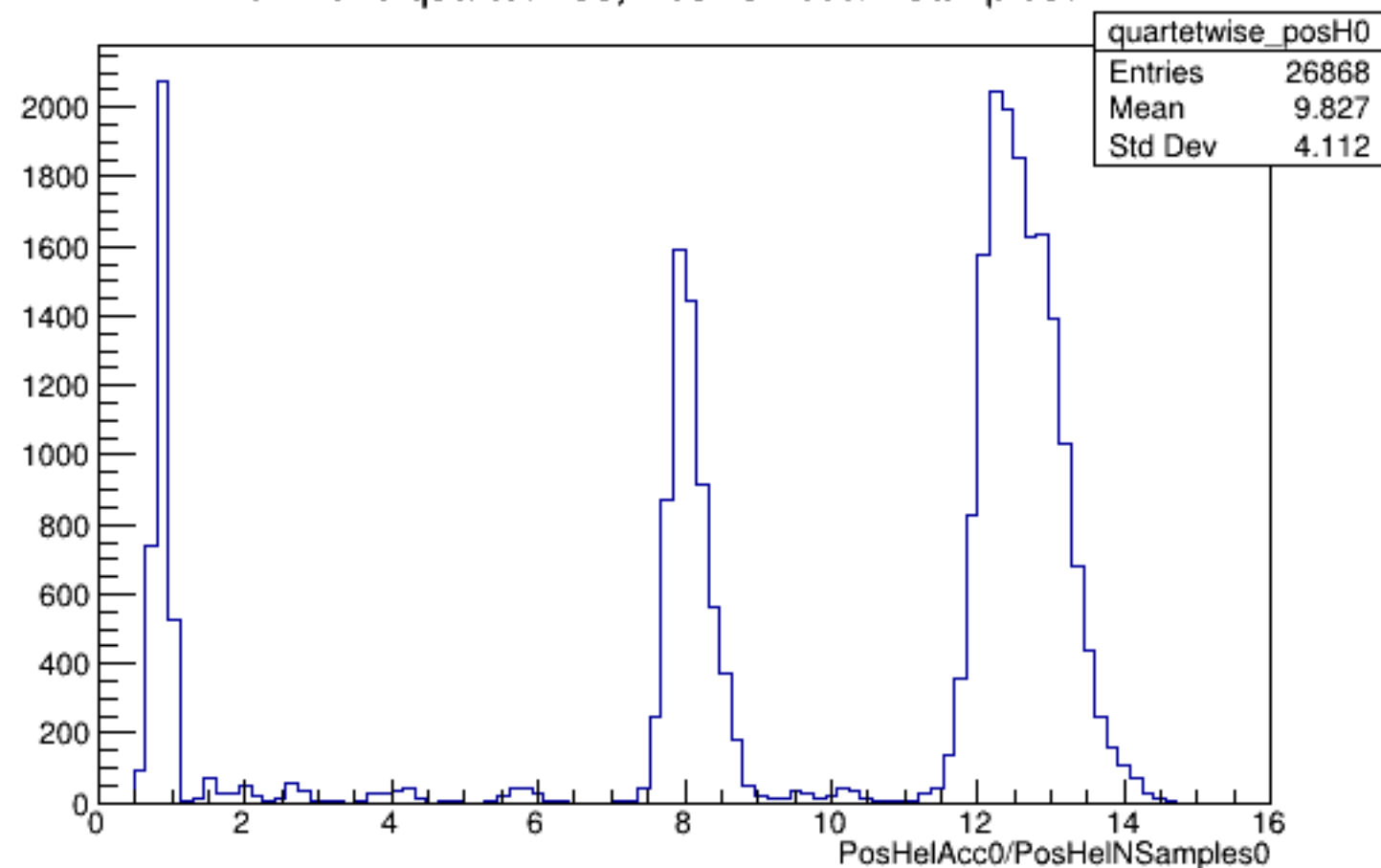
Run 4618 quartetwise, PosHelAcc0/NSamples0: All
