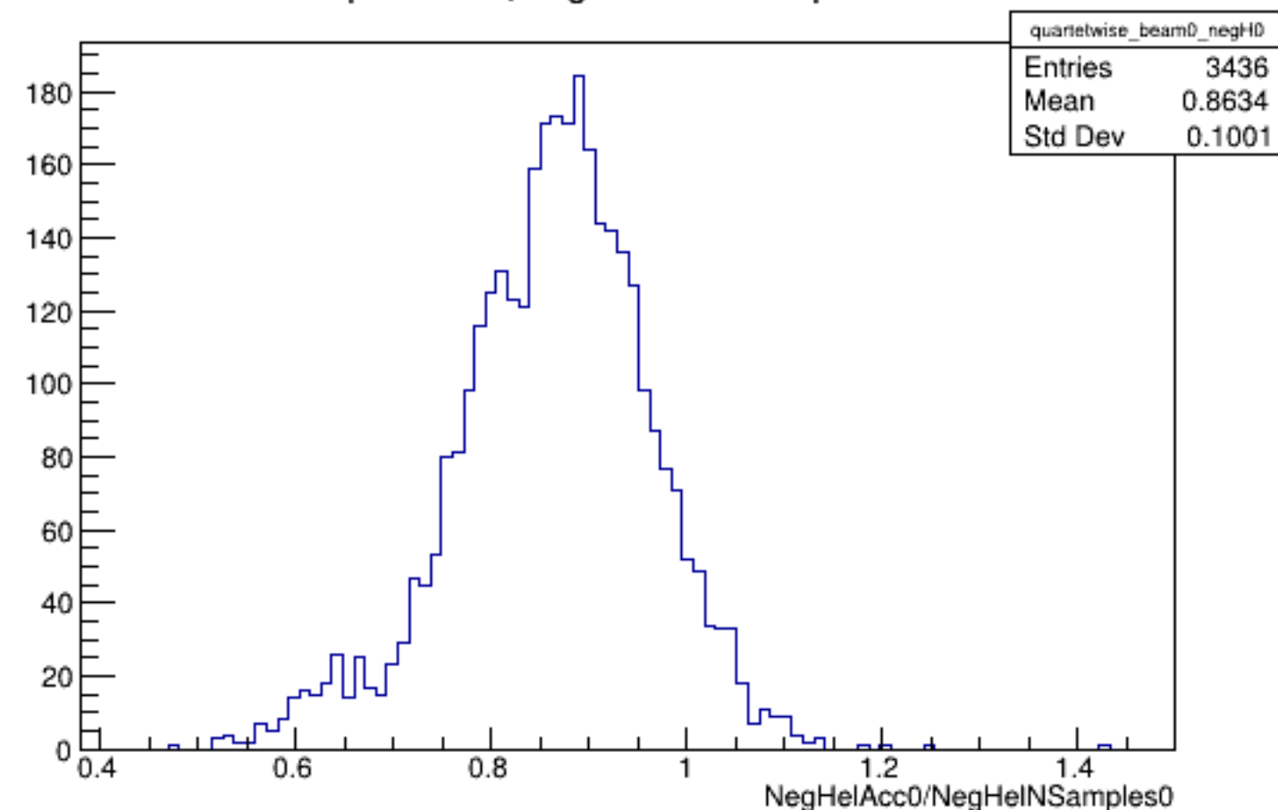
Run 4618 quartetwise, NegHelAcc0/NSamples0: Beam OFF
