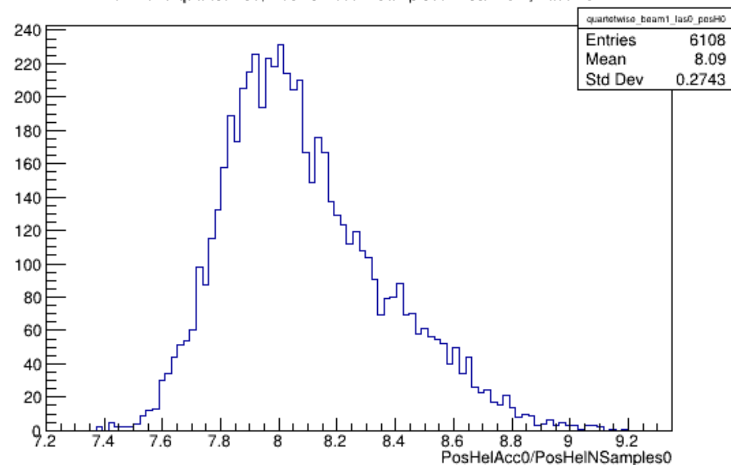
Run 4618 quartetwise, PosHelAcc0/NSamples0: Beam ON, Laser OFF
