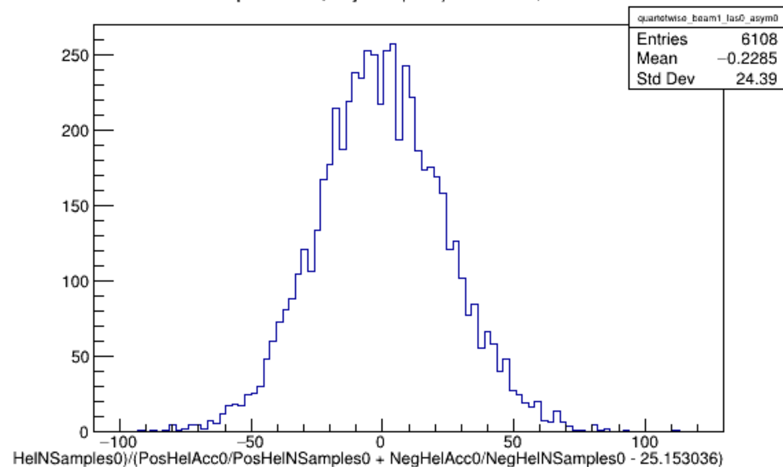
Run 4618 quartetwise, Asyms0 (Raw): Beam ON, Laser OFF
