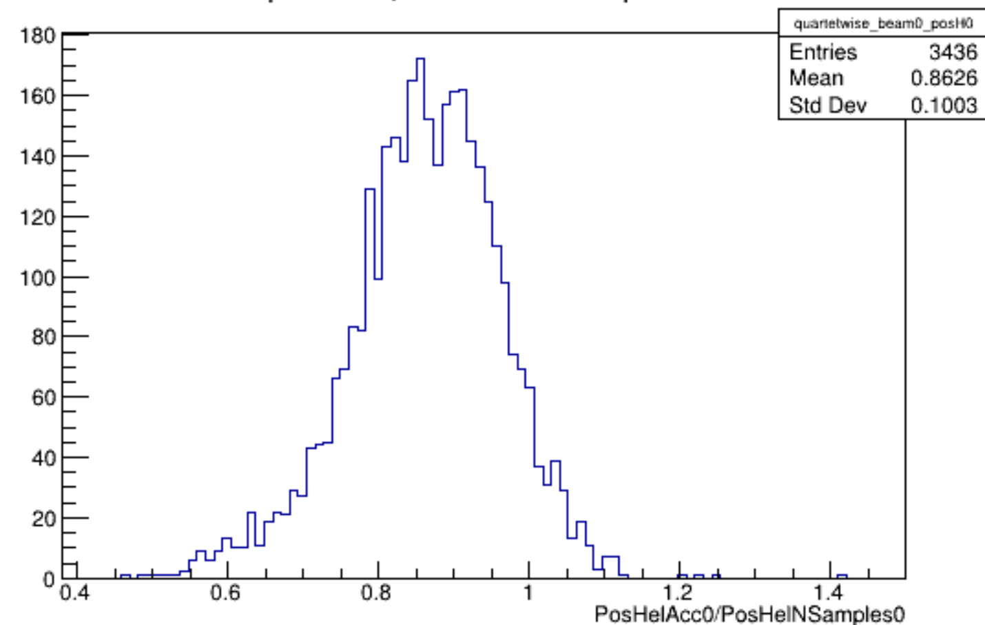
Run 4618 quartetwise, PosHelAcc0/NSamples0: Beam OFF
