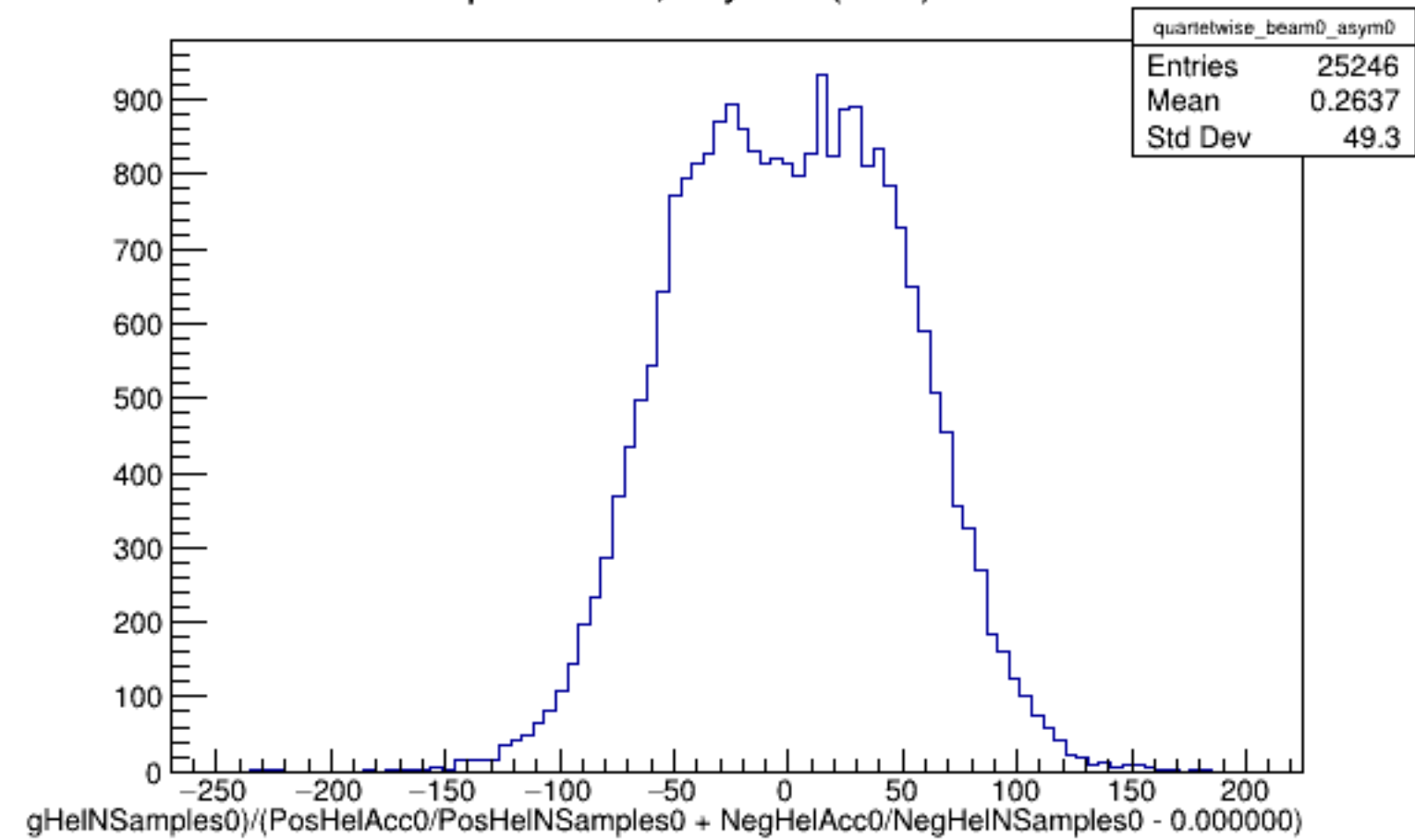
Run 4623 quartetwise, Asyms0 (Raw): Beam OFF
