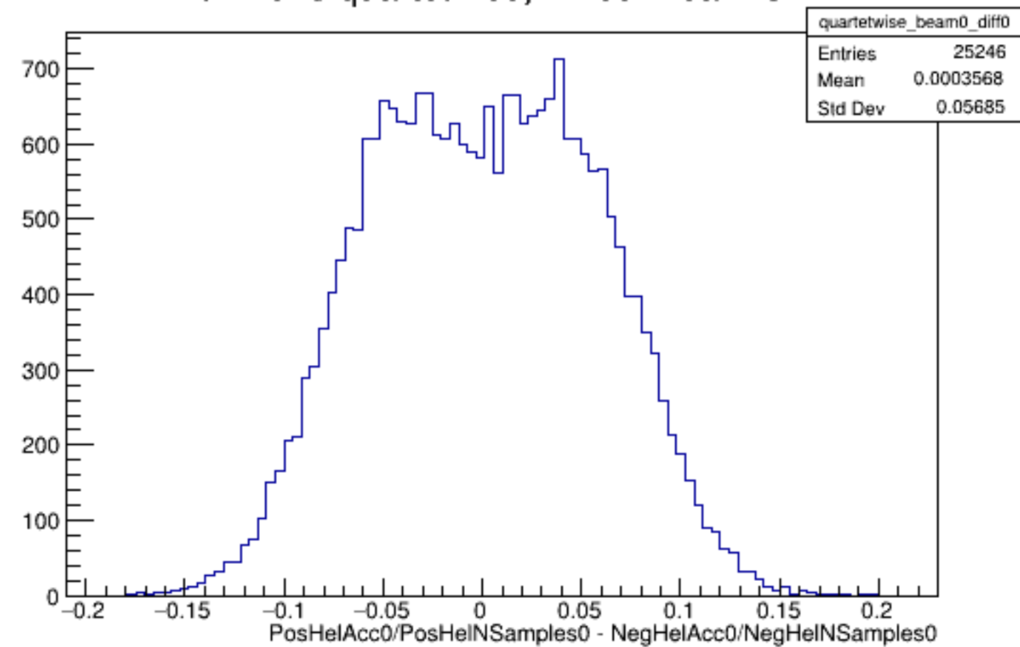
Run 4623 quartetwise, Diffs0: Beam OFF
