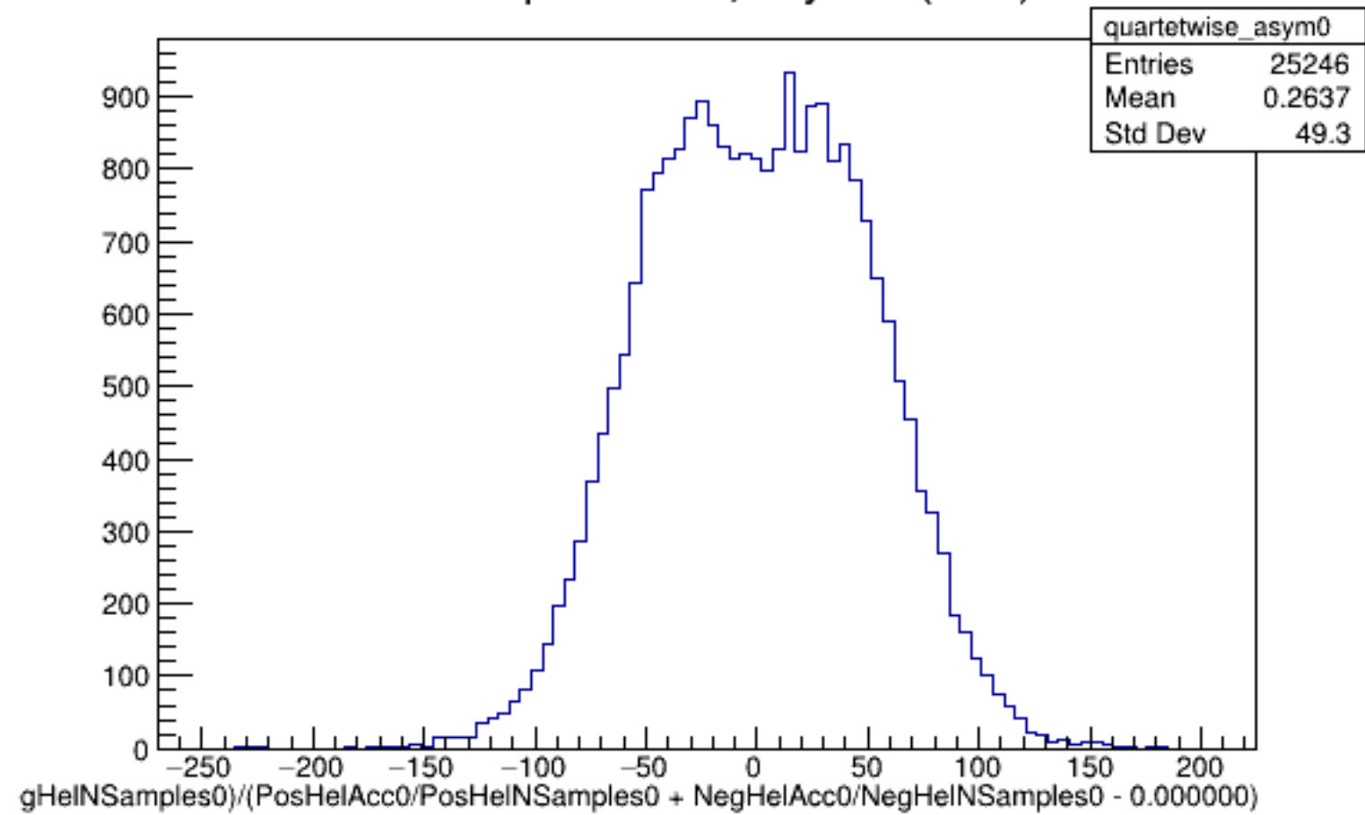
Run 4623 quartetwise, Asyms0 (Raw): All
