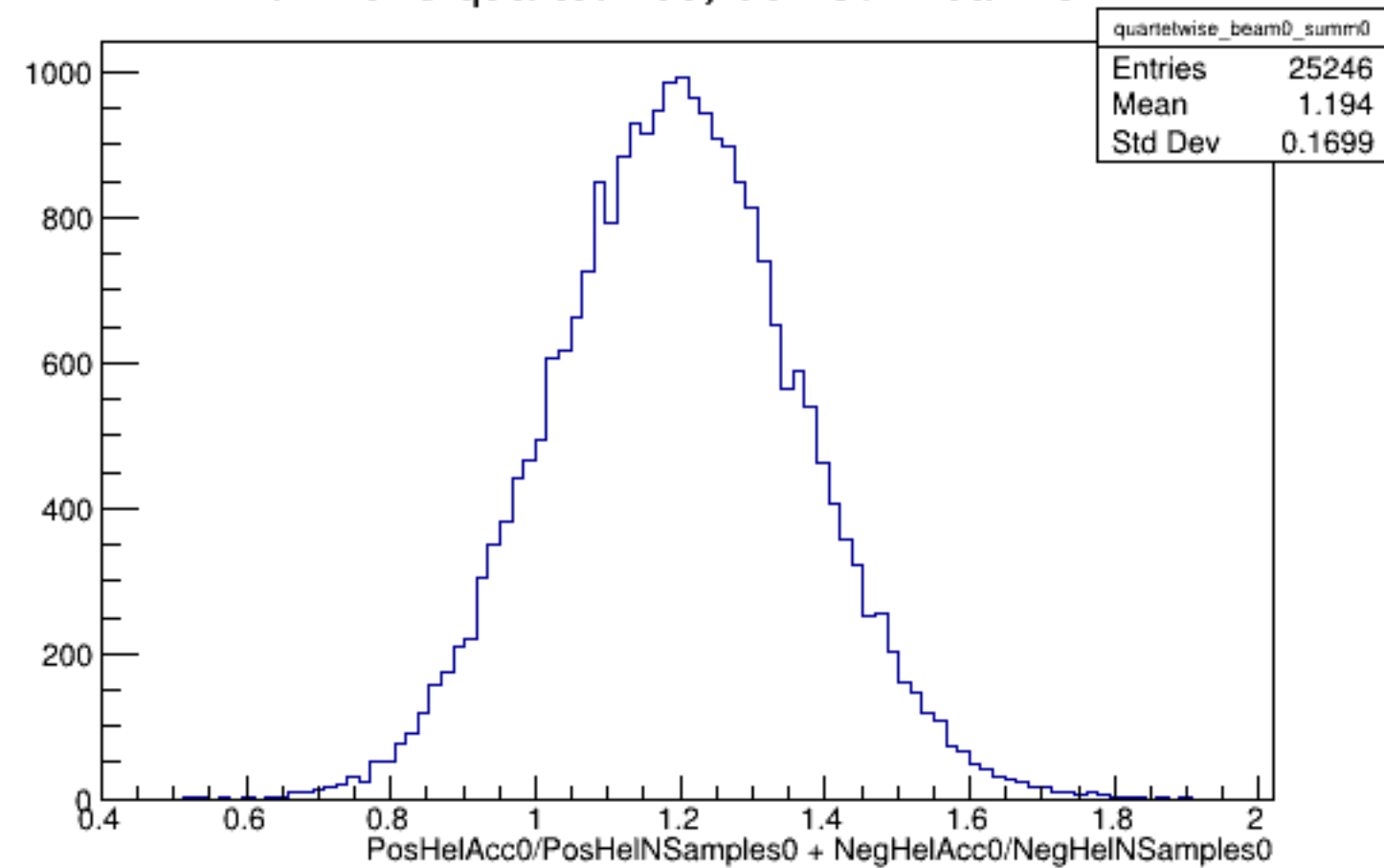
Run 4623 quartetwise, Sums0: Beam OFF
