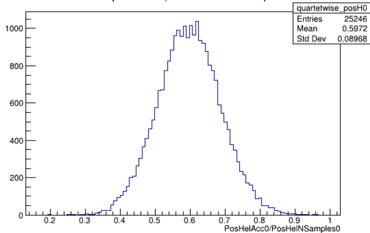
Run 4623 quartetwise, PosHelAcc0/NSamples0: All
