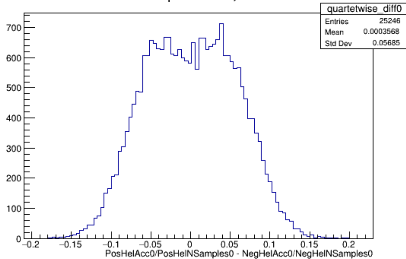
Run 4623 quartetwise, Diffs0: All
