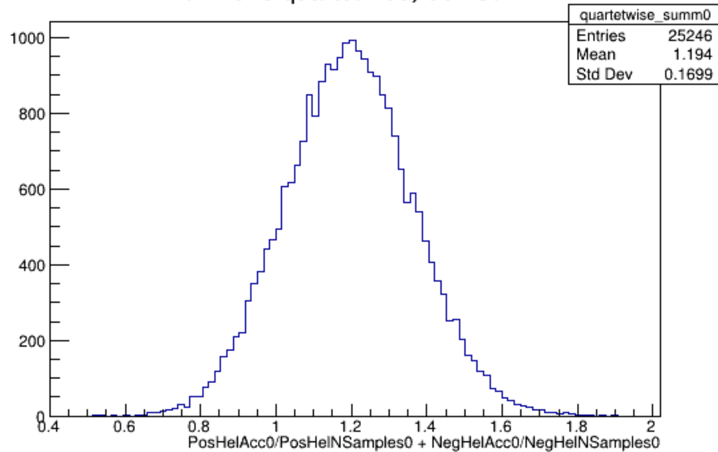
Run 4623 quartetwise, Sums0: All
