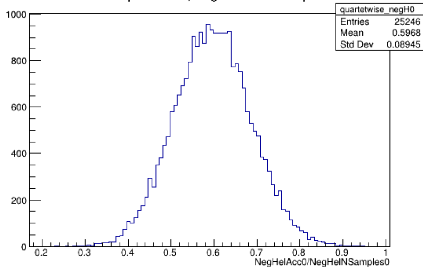
Run 4623 quartetwise, NegHelAcc0/NSamples0: All
