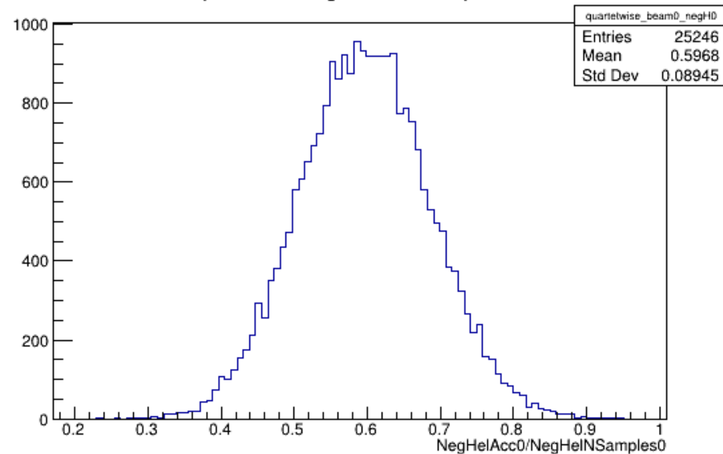
Run 4623 quartetwise, NegHelAcc0/NSamples0: Beam OFF
