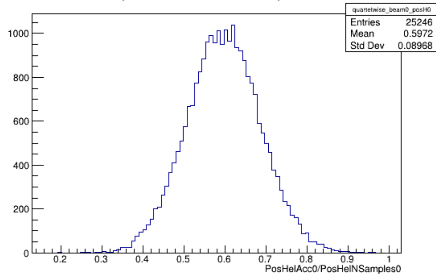
Run 4623 quartetwise, PosHelAcc0/NSamples0: Beam OFF
