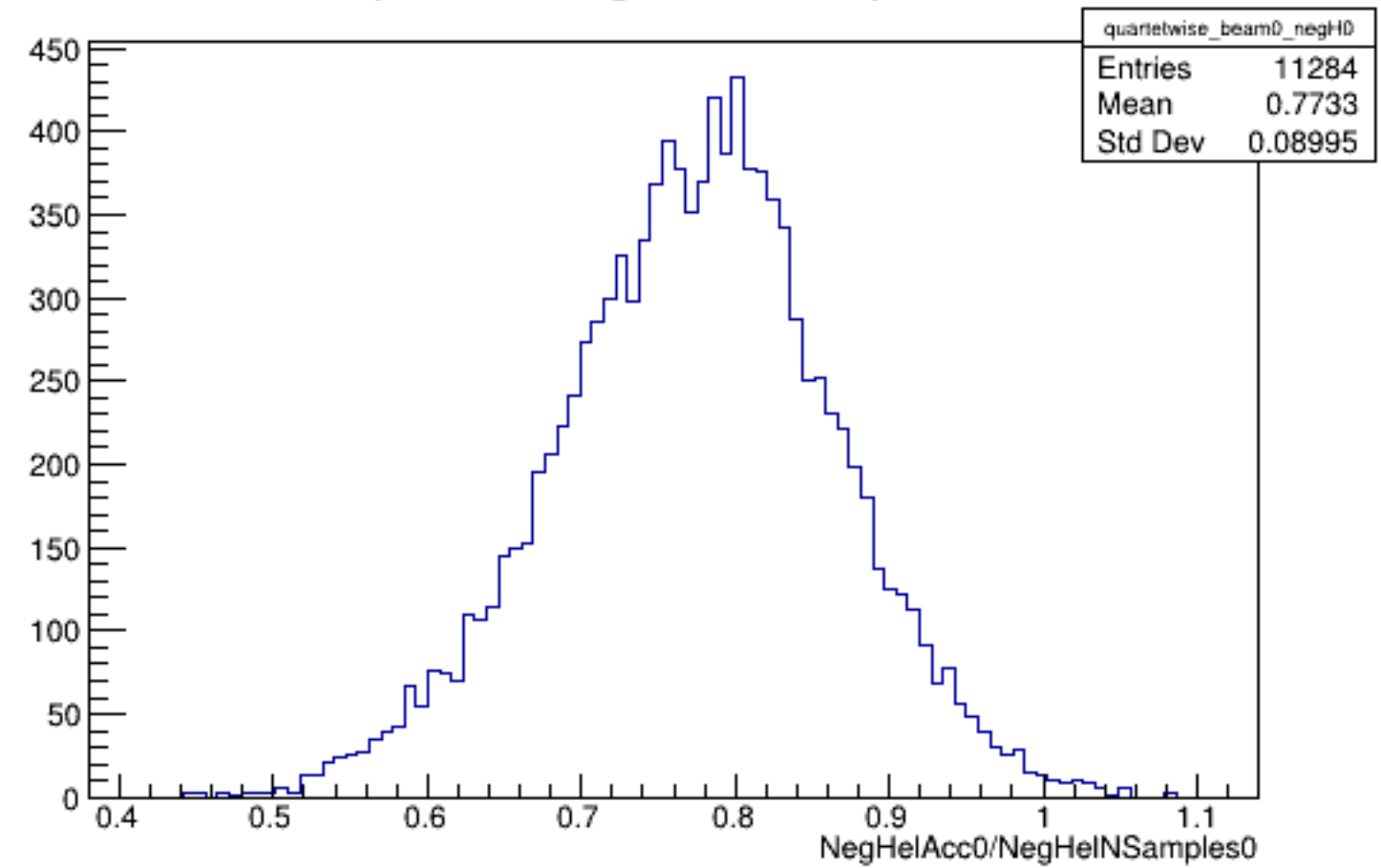
Run 4625 quartetwise, NegHelAcc0/NSamples0: Beam OFF
