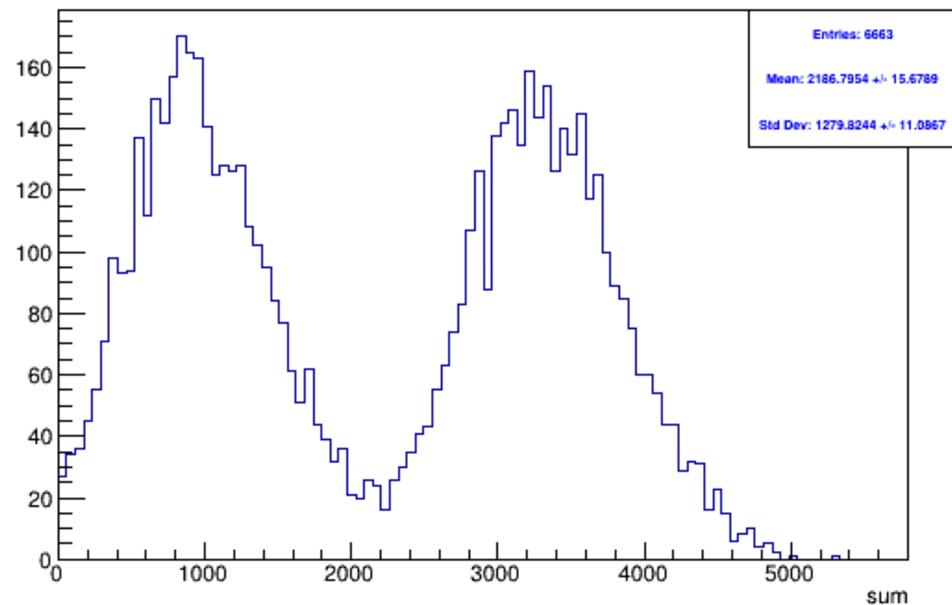
Run 4633 triggerwise, sums: Beam OFF
