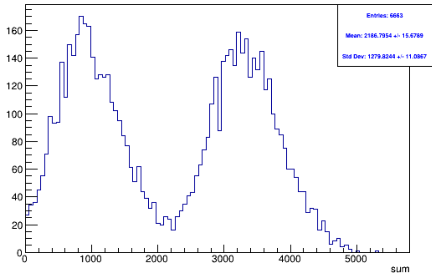
Run 4633 triggerwise, sums: All
