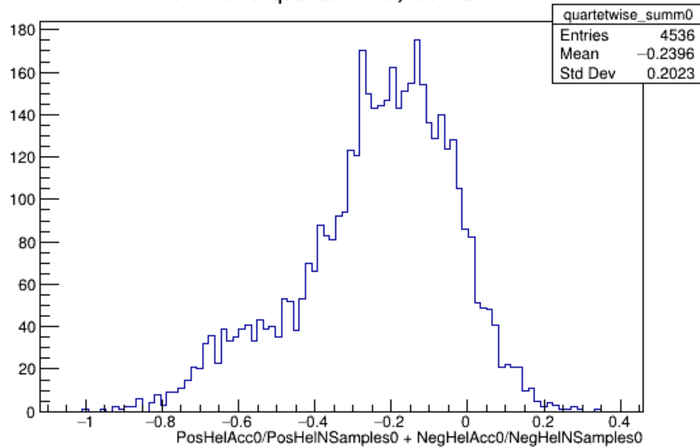
Run 4849 quartetwise, Sums0: All
