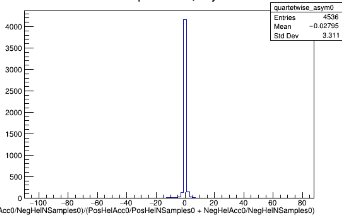
Run 4849 quartetwise, Asyms0: All
