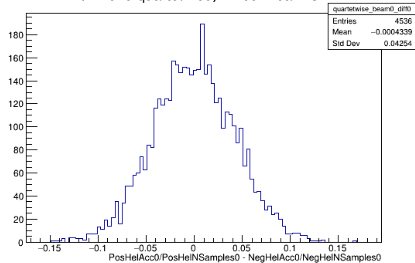
Run 4849 quartetwise, Diffs0: Beam OFF
