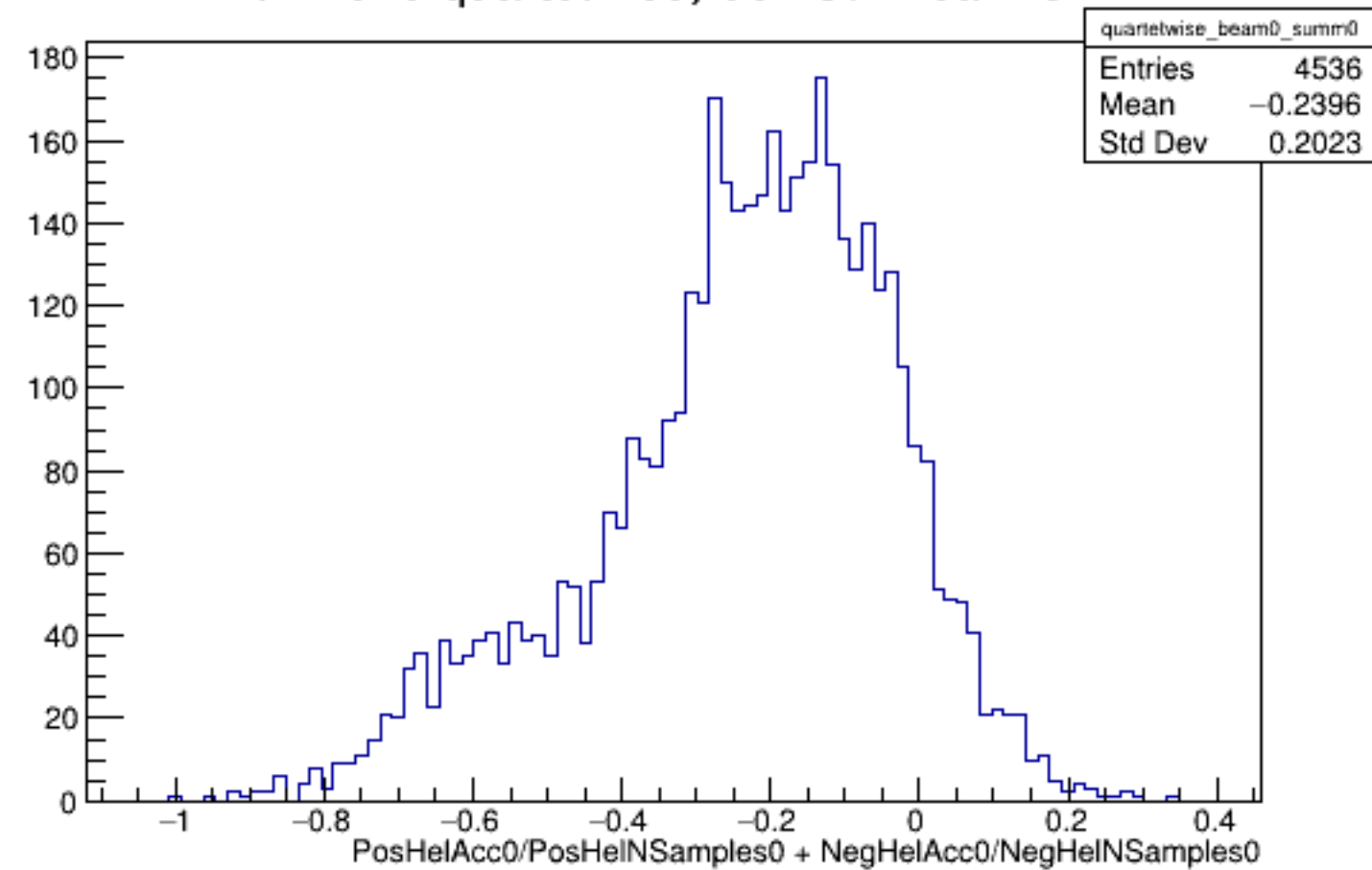
Run 4849 quartetwise, Sums0: Beam OFF
