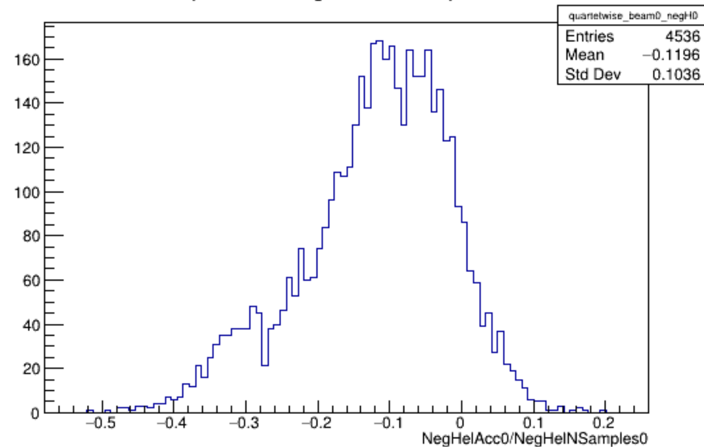
Run 4849 quartetwise, NegHelAcc0/NSamples0: Beam OFF
