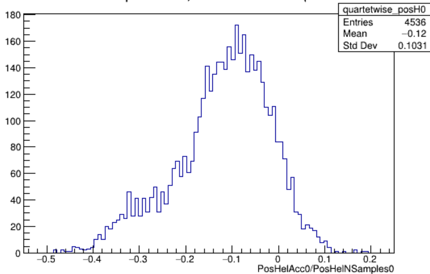
Run 4849 quartetwise, PosHelAcc0/NSamples0: All
