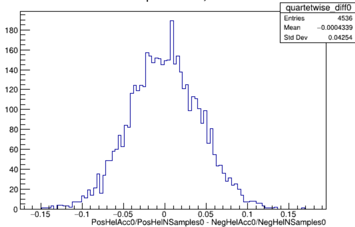
Run 4849 quartetwise, Diffs0: All
