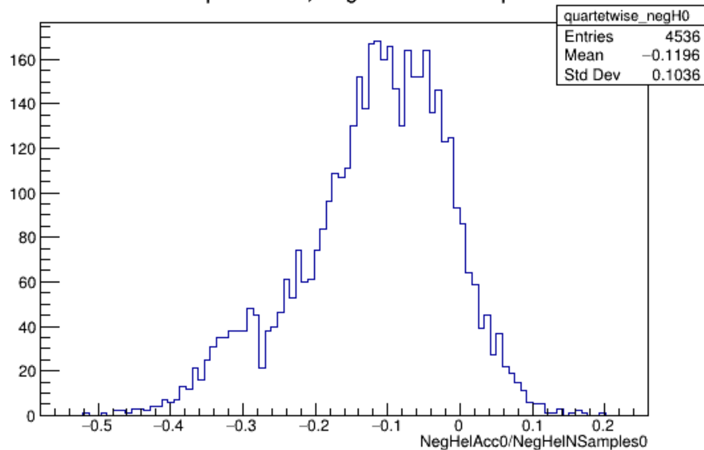
Run 4849 quartetwise, NegHelAcc0/NSamples0: All
