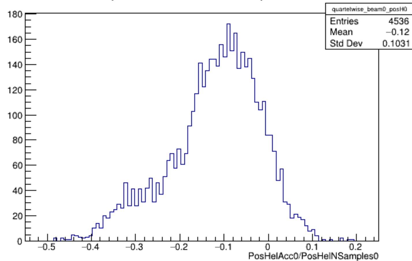
Run 4849 quartetwise, PosHelAcc0/NSamples0: Beam OFF
