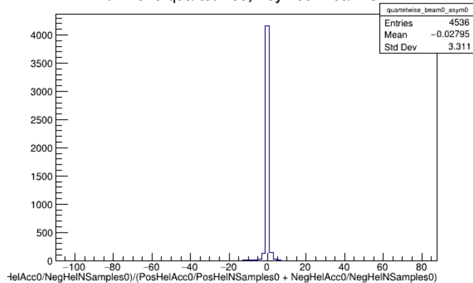
Run 4849 quartetwise, Asyms0: Beam OFF
