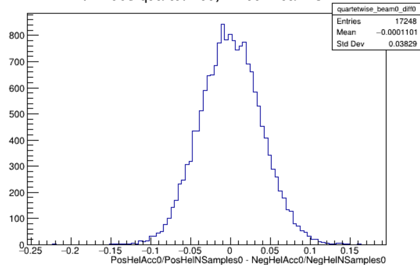
Run 4933 quartetwise, Diffs0: Beam OFF
