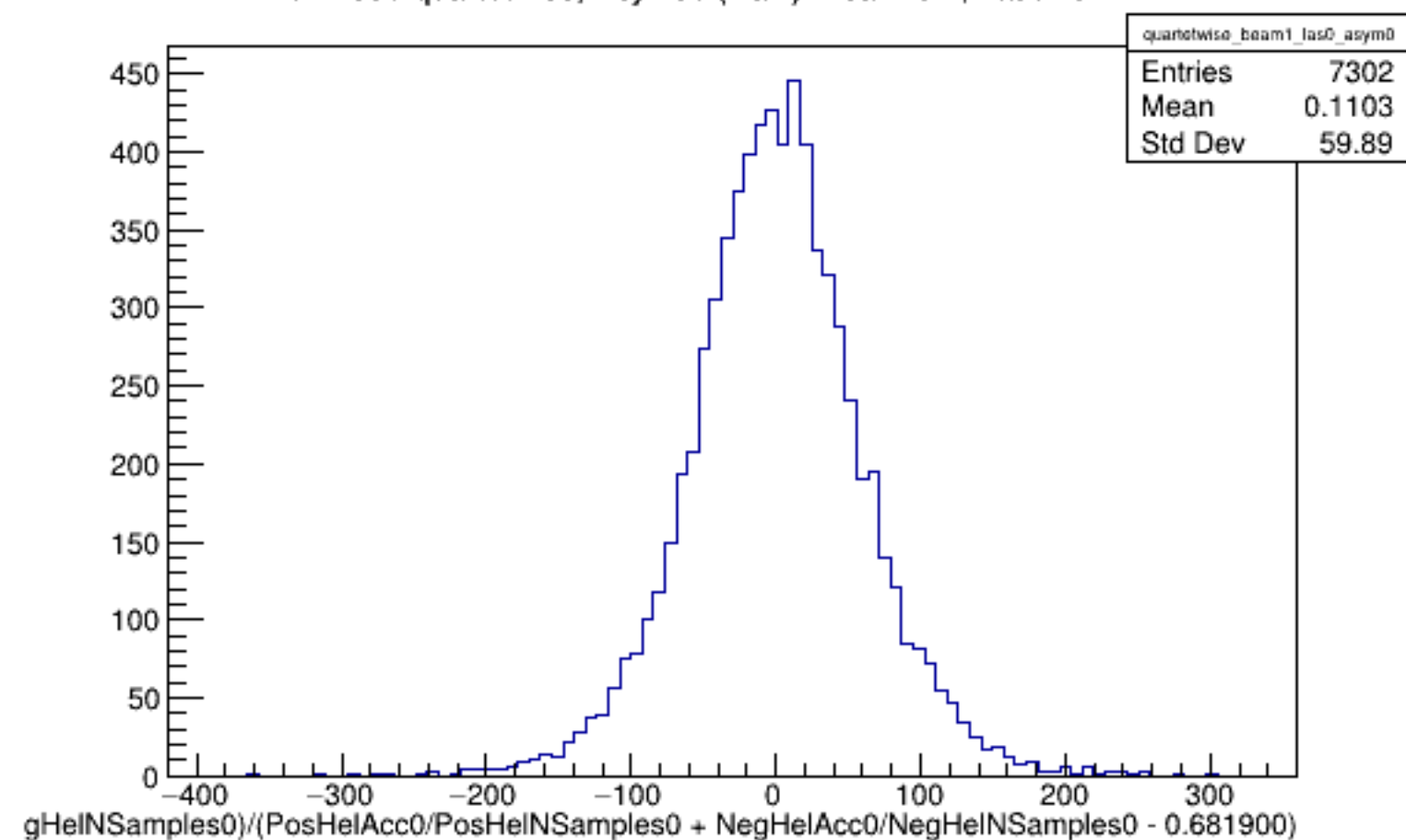
Run 4933 quartetwise, Asyms0 (Raw): Beam ON, Laser OFF
