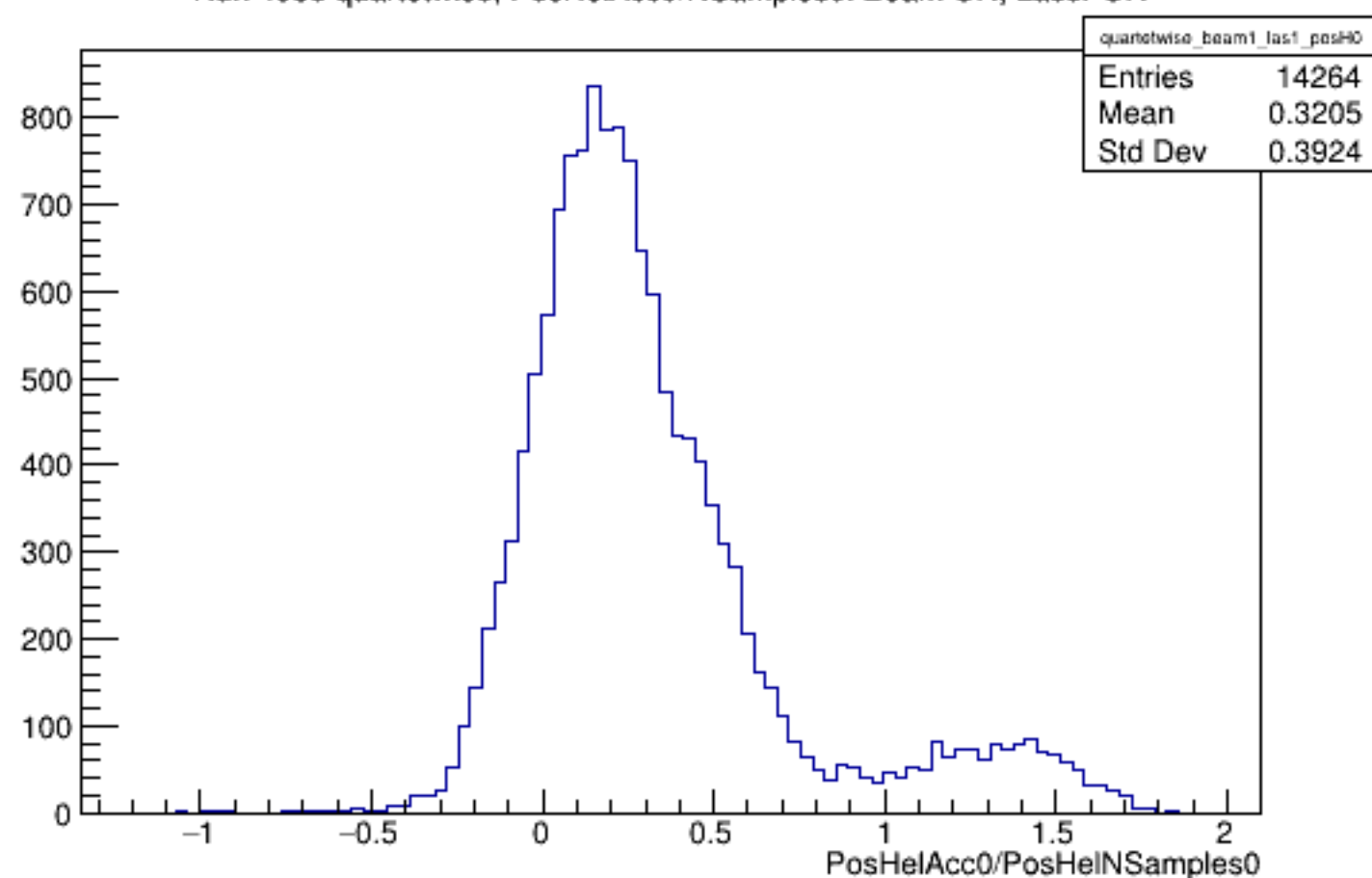
Run 4933 quartetwise, PosHelAcc0/NSamples0: Beam ON, Laser ON
