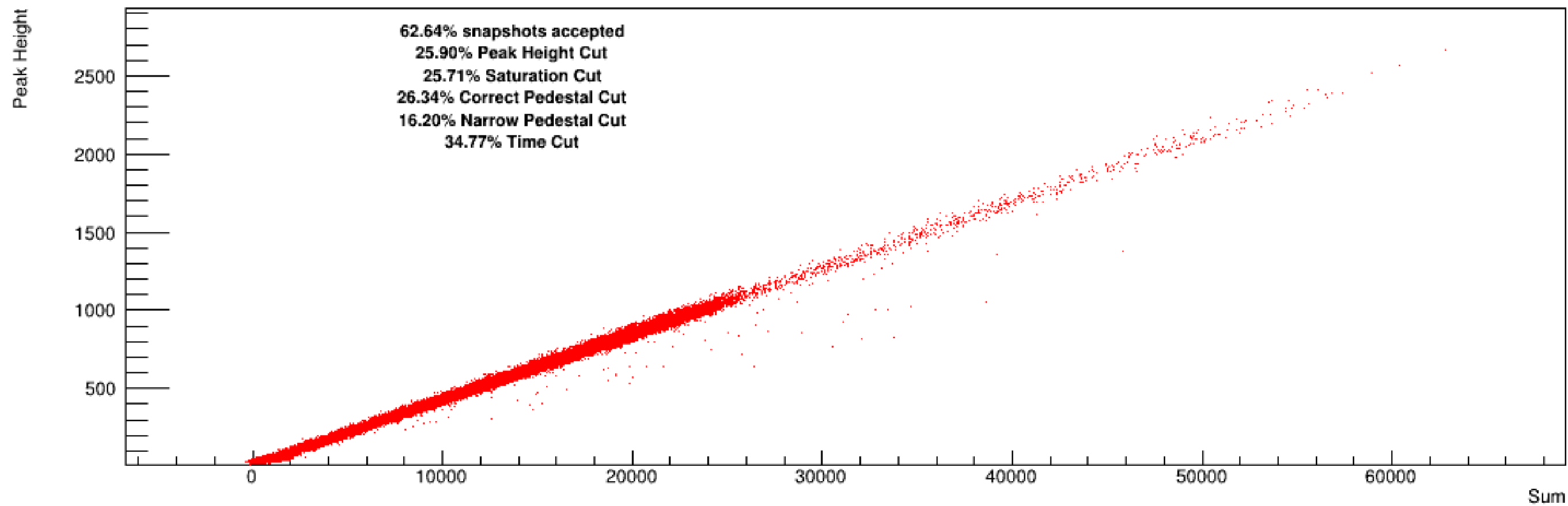
Run 4933, snapshots: Peak Height vs. Sum
