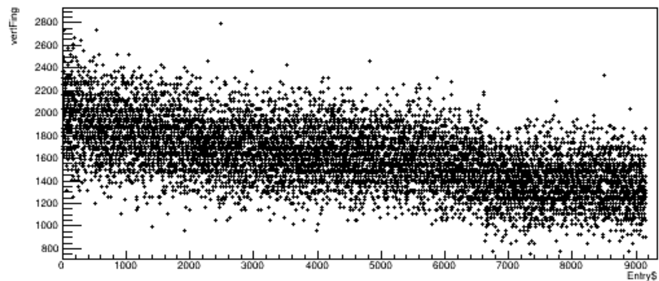
Run 4960, quartetwise: vertFing vs time
