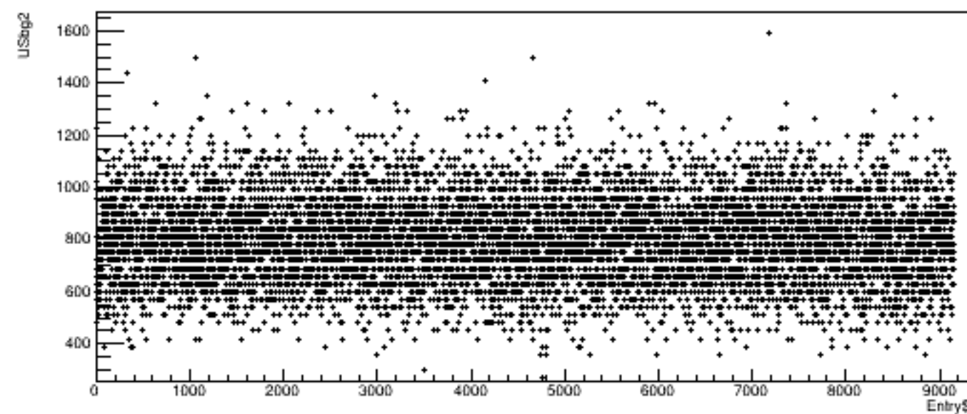
Run 4960, quartetwise: USbg2 vs time
