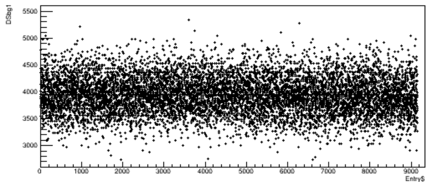
Run 4960, quartetwise: DSbg1 vs time
