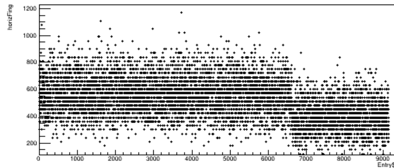
Run 4960, quartetwise: horizFing vs time
