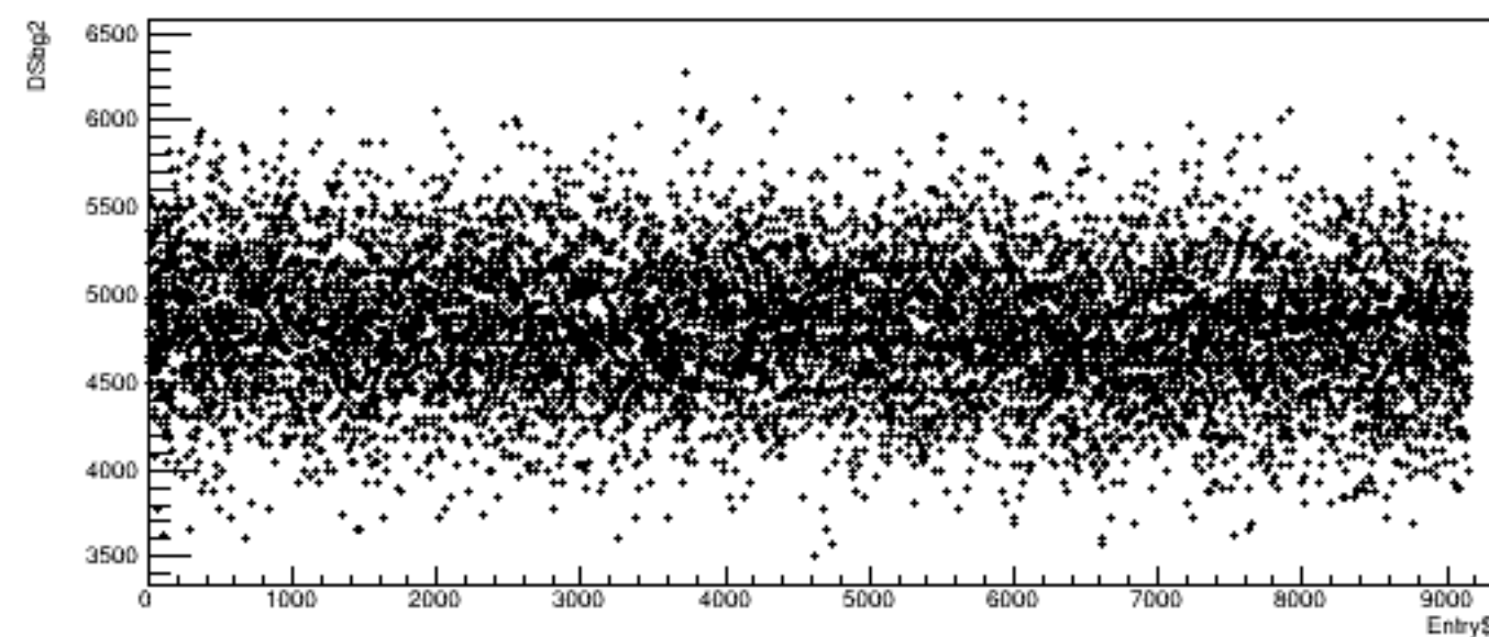
Run 4960, quartetwise: DSbg2 vs time
