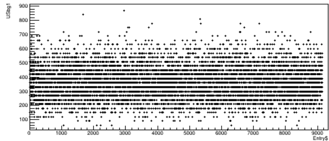
Run 4960, quartetwise: USbg1 vs time
