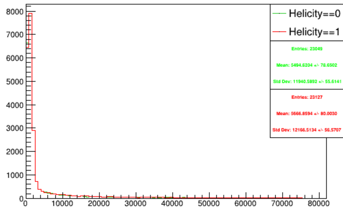
Run 4960 triggerwise, sums: Beam ON, Laser OFF
