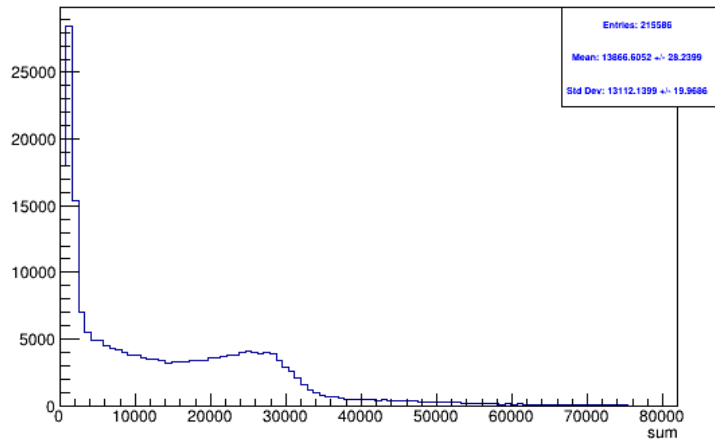
Run 4960 triggerwise, sums: All
