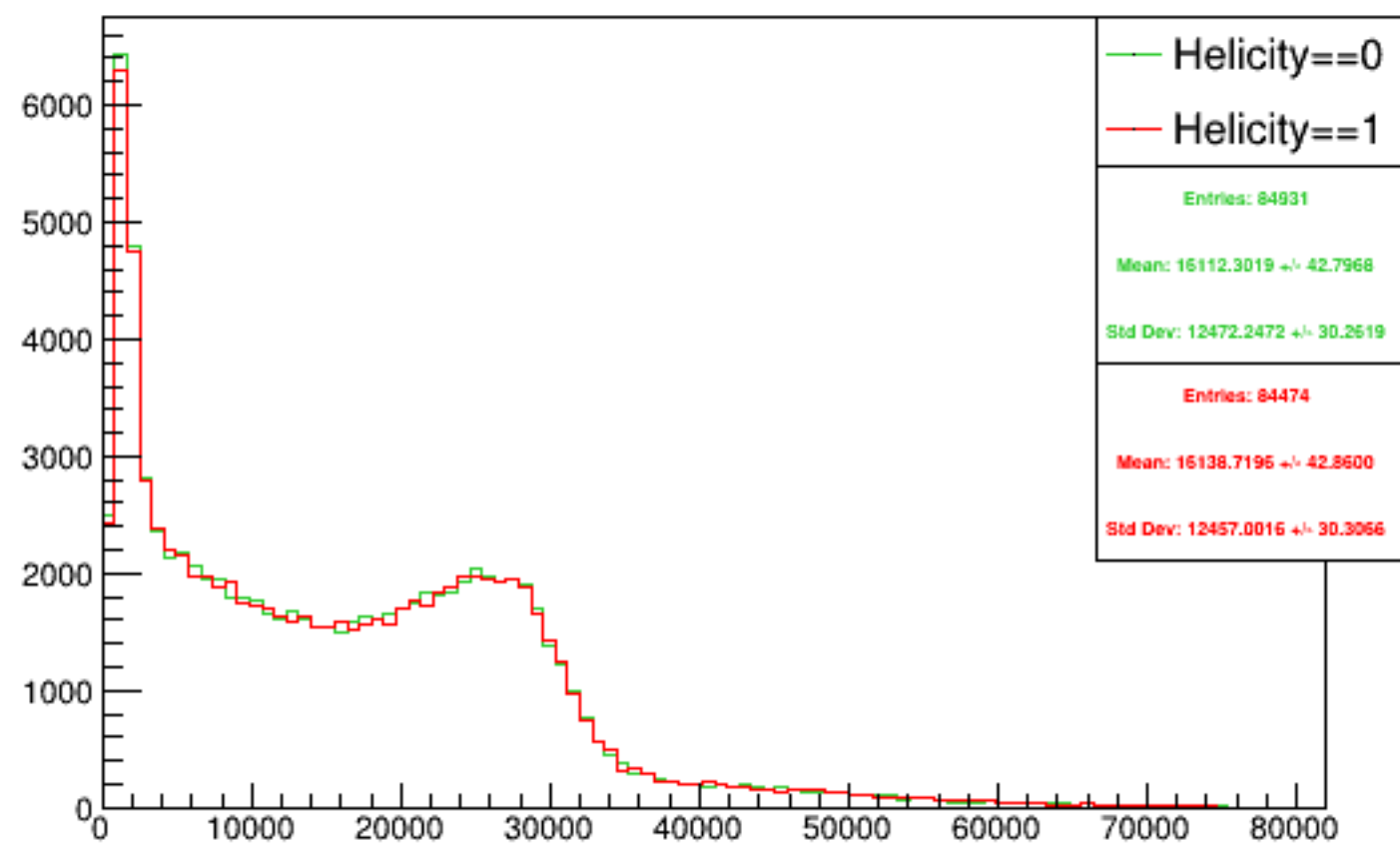
Run 4960 triggerwise, sums: Beam ON, Laser ON
