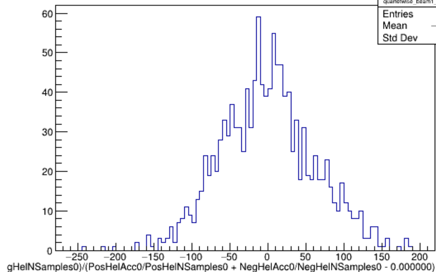
Run 4961 quartetwise, Asyms0 (Raw): Beam ON, Laser OFF
