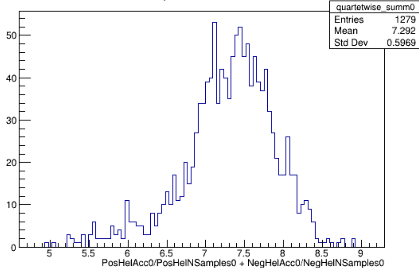
Run 4961 quartetwise, Sums0: All
