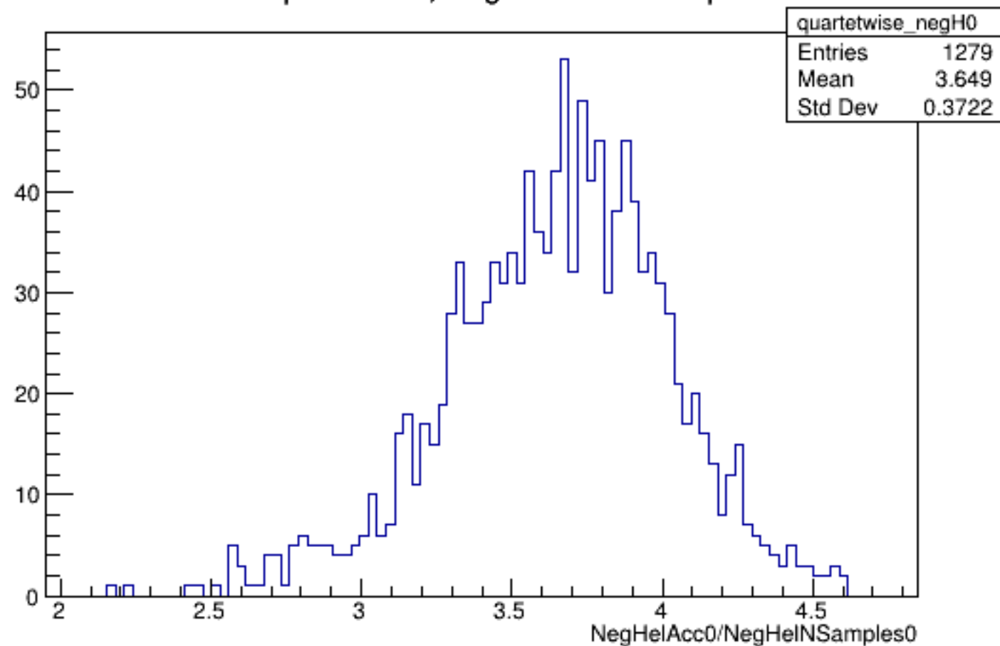
Run 4961 quartetwise, NegHelAcc0/NSamples0: All
