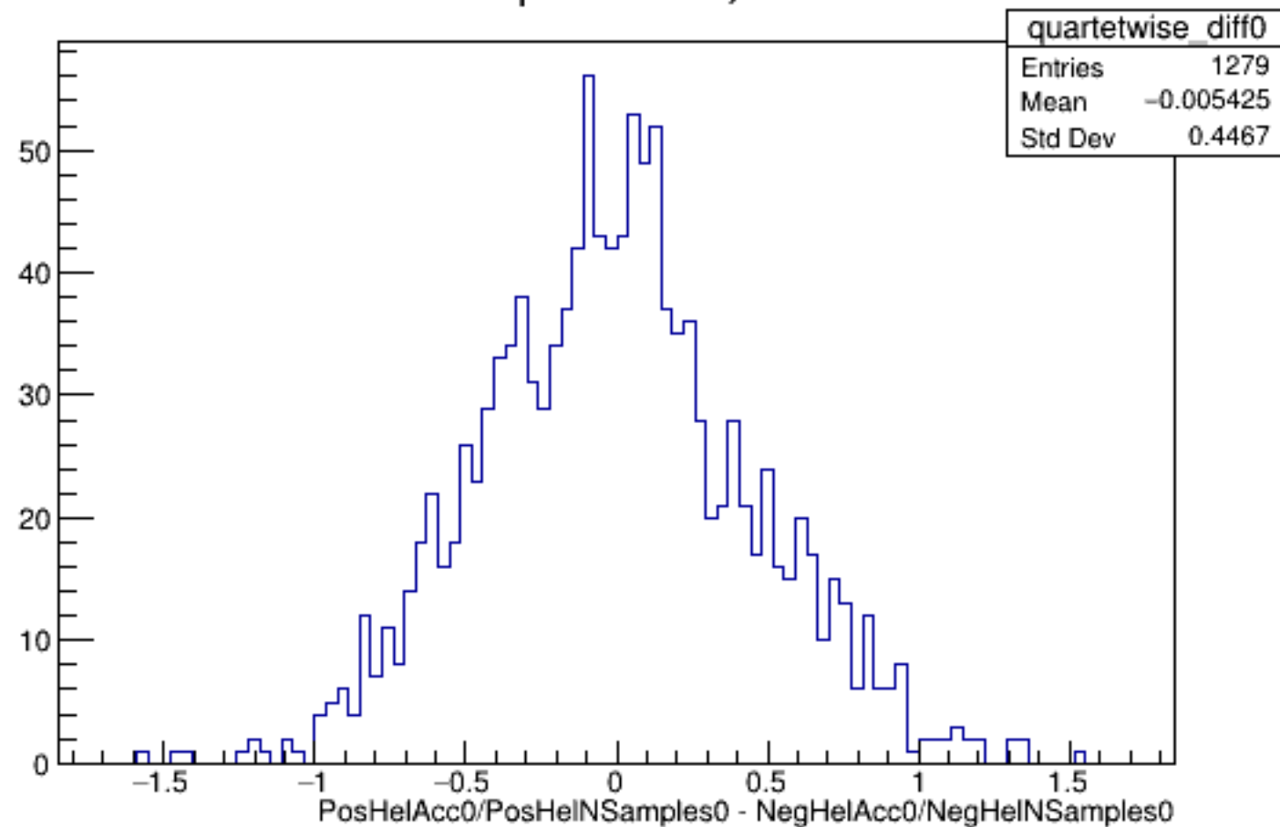
Run 4961 quartetwise, Diffs0: All
