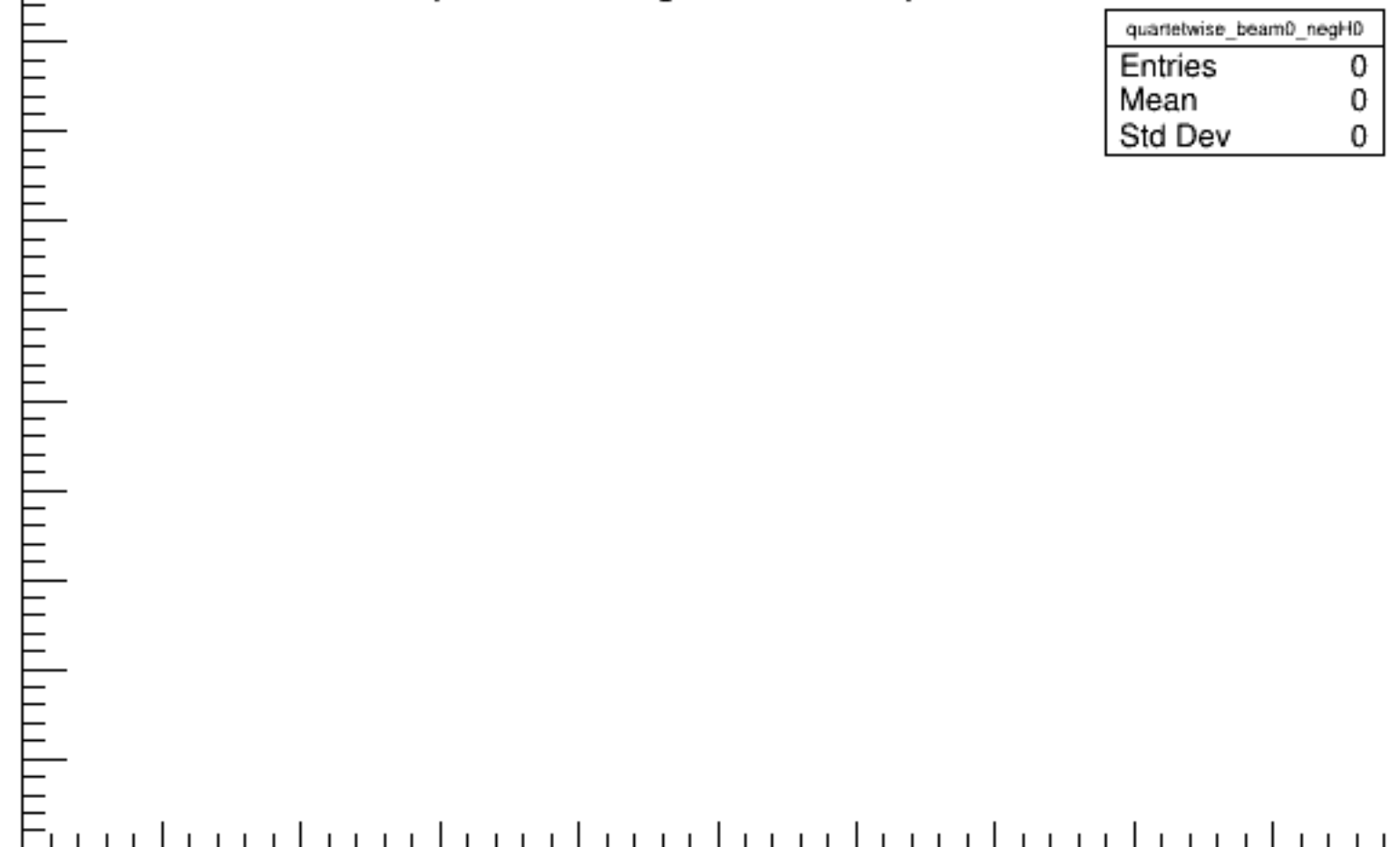
Run 4961 quartetwise, NegHelAcc0/NSamples0: Beam OFF
