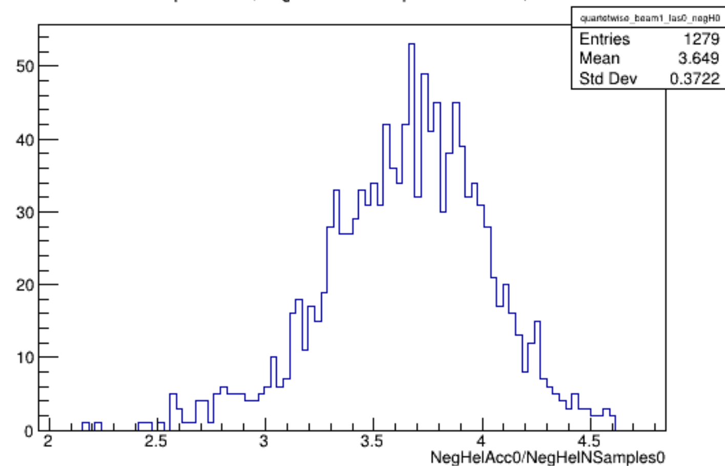
Run 4961 quartetwise, NegHelAcc0/NSamples0: Beam ON, Laser OFF
