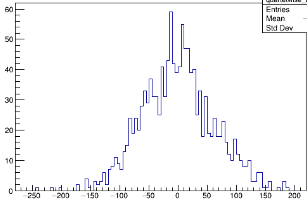
Run 4961 quartetwise, Asyms0 (Raw): All
