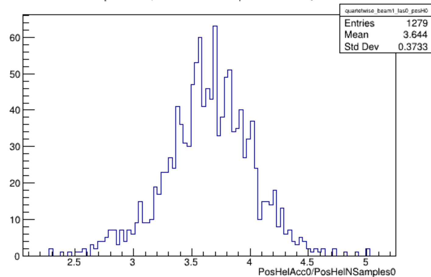
Run 4961 quartetwise, PosHelAcc0/NSamples0: Beam ON, Laser OFF
