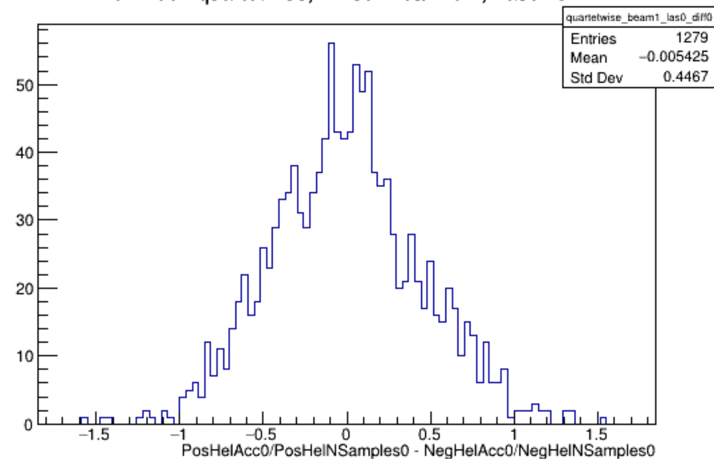
Run 4961 quartetwise, Diffs0: Beam ON, Laser OFF
