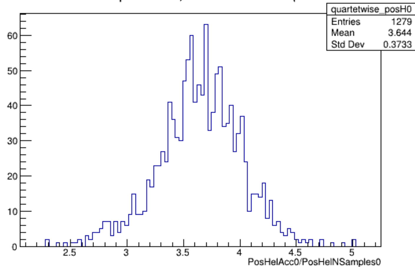
Run 4961 quartetwise, PosHelAcc0/NSamples0: All
