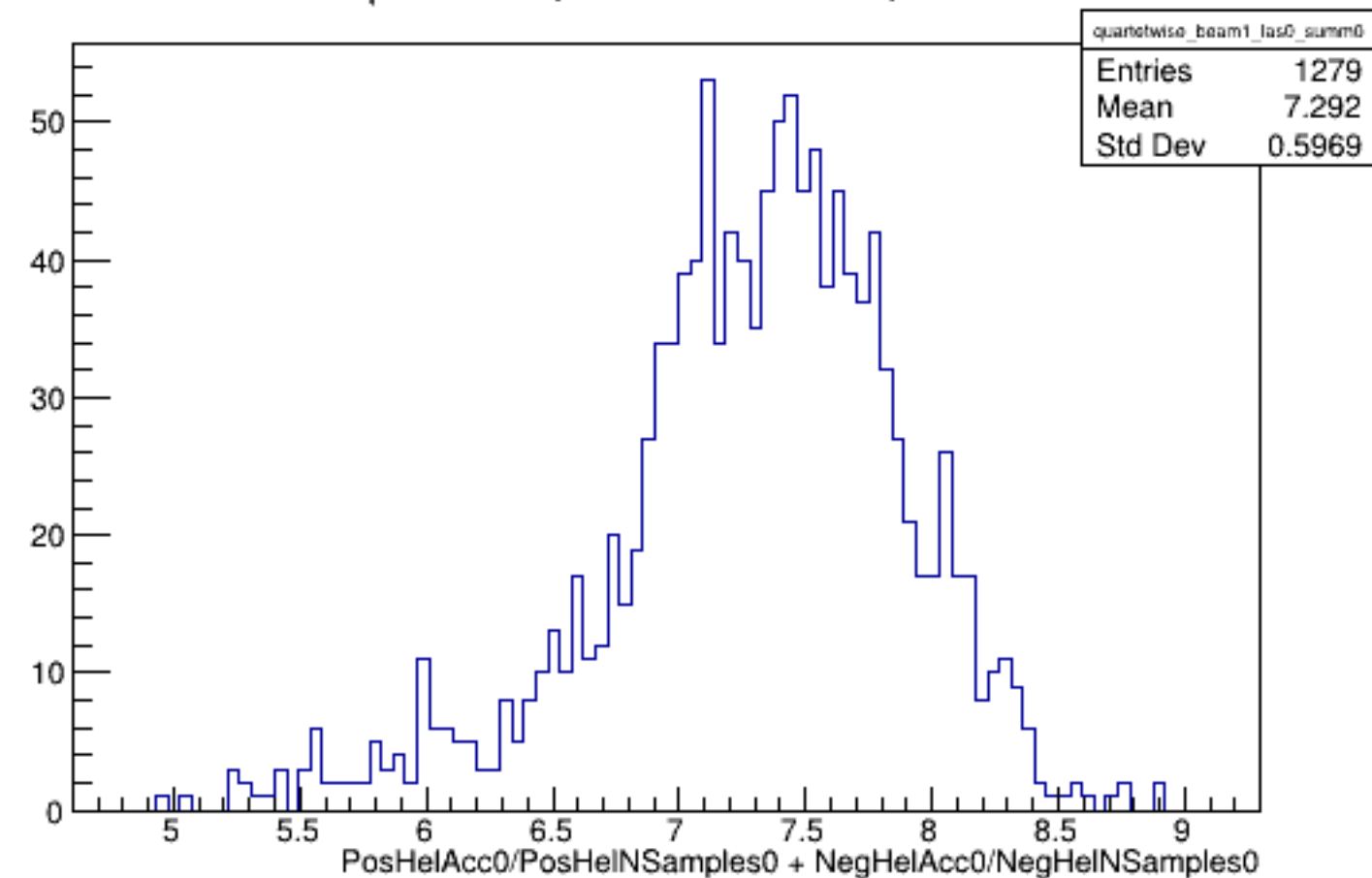
Run 4961 quartetwise, Sums0: Beam ON, Laser OFF
