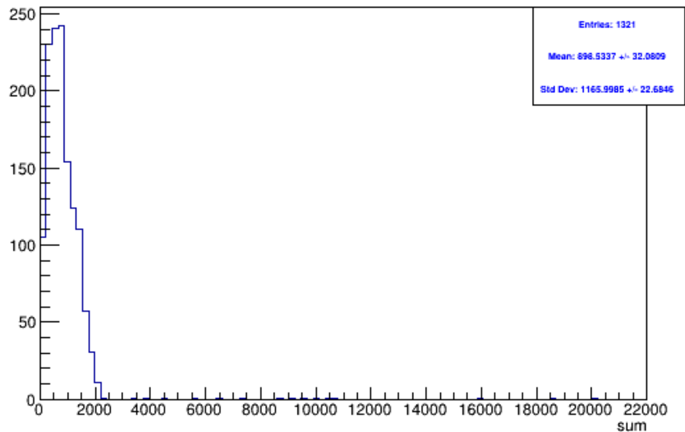
Run 4970 triggerwise, sums: All
