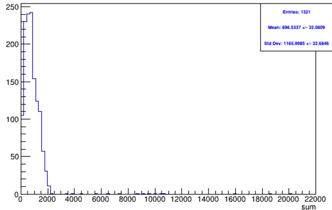
Run 4970 triggerwise, sums: Beam OFF
