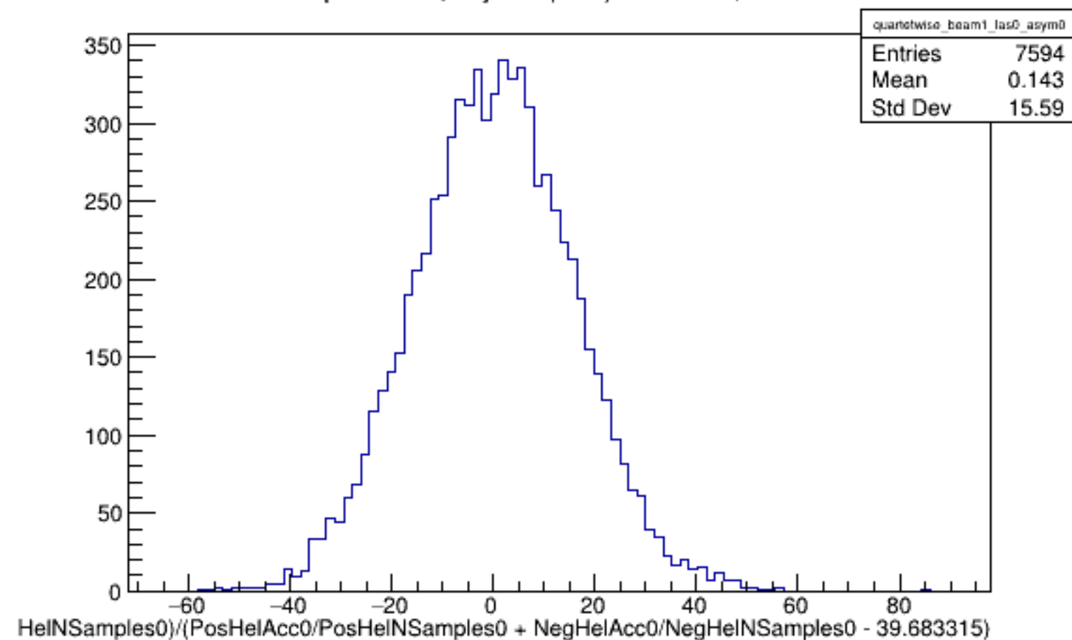
Run 4977 quartetwise, Asyms0 (Raw): Beam ON, Laser OFF
