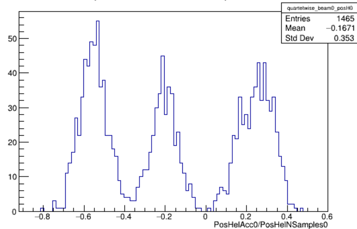
Run 4977 quartetwise, PosHelAcc0/NSamples0: Beam OFF
