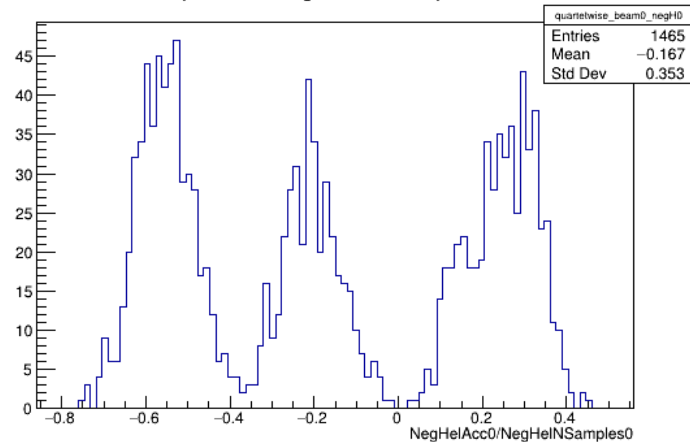
Run 4977 quartetwise, NegHelAcc0/NSamples0: Beam OFF
