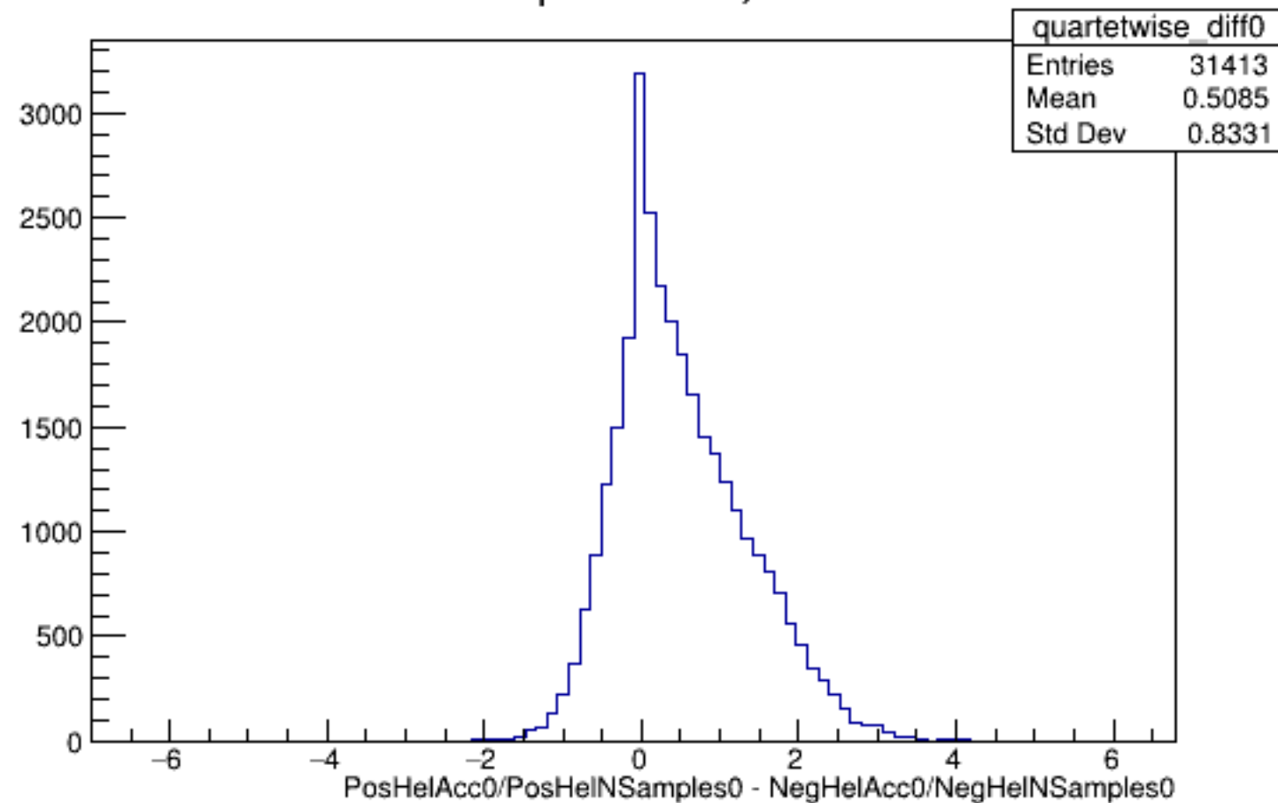
Run 4977 quartetwise, Diffs0: All
