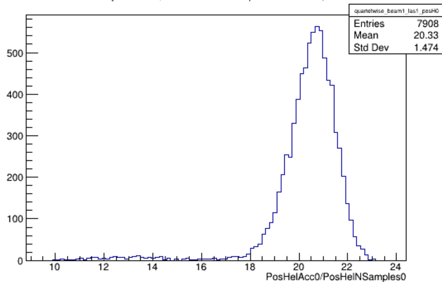
Run 4977 quartetwise, PosHelAcc0/NSamples0: Beam ON, Laser ON
