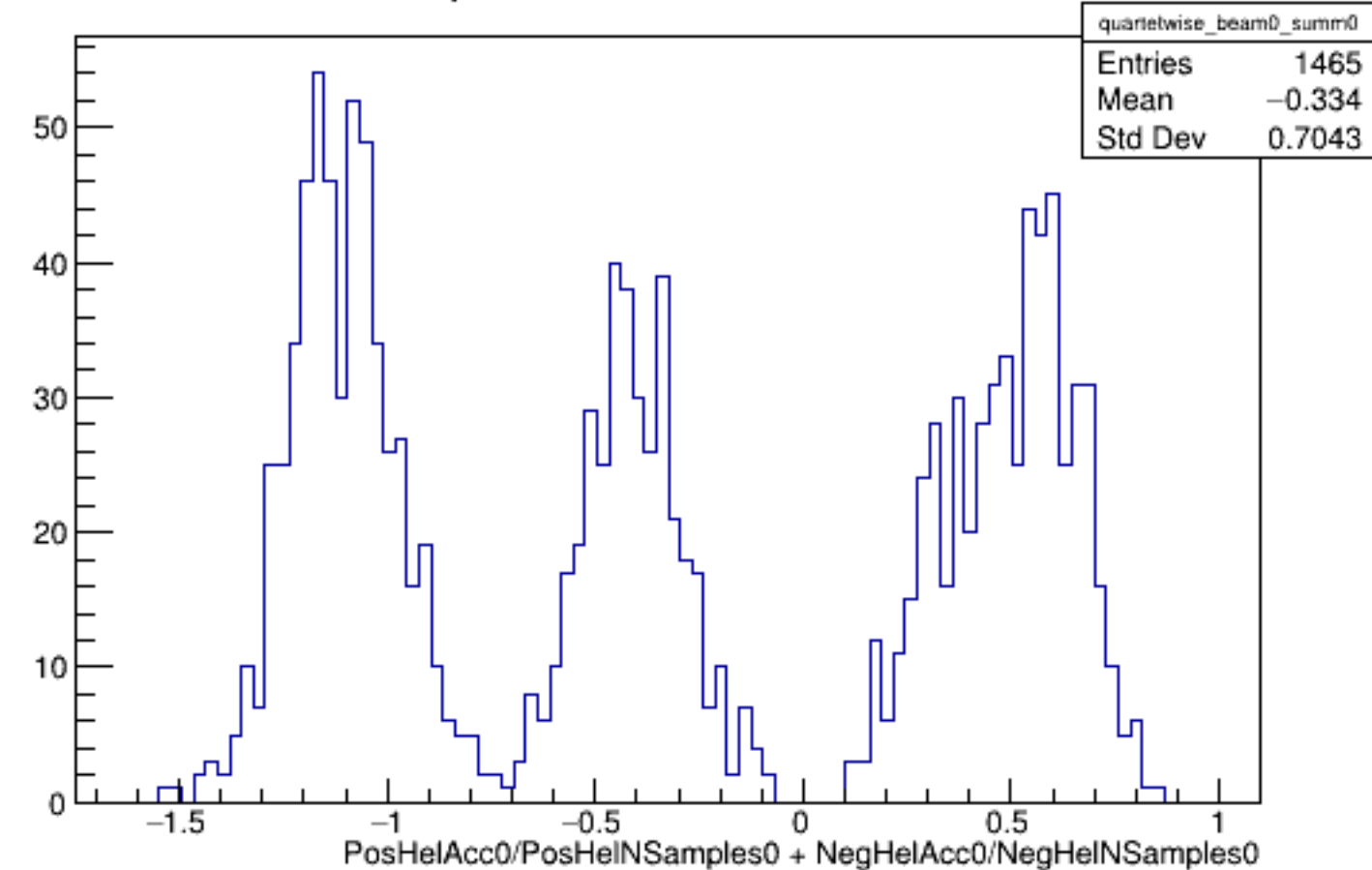
Run 4977 quartetwise, Sums0: Beam OFF
