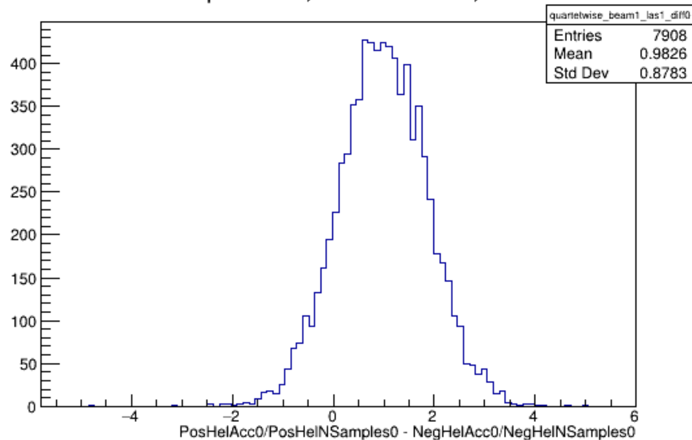
Run 4977 quartetwise, Diffs0: Beam ON, Laser ON
