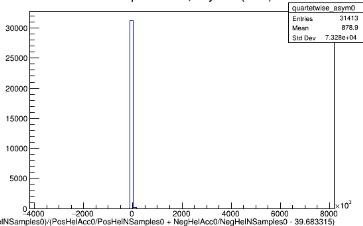
Run 4977 quartetwise, Asyms0 (Raw): All
