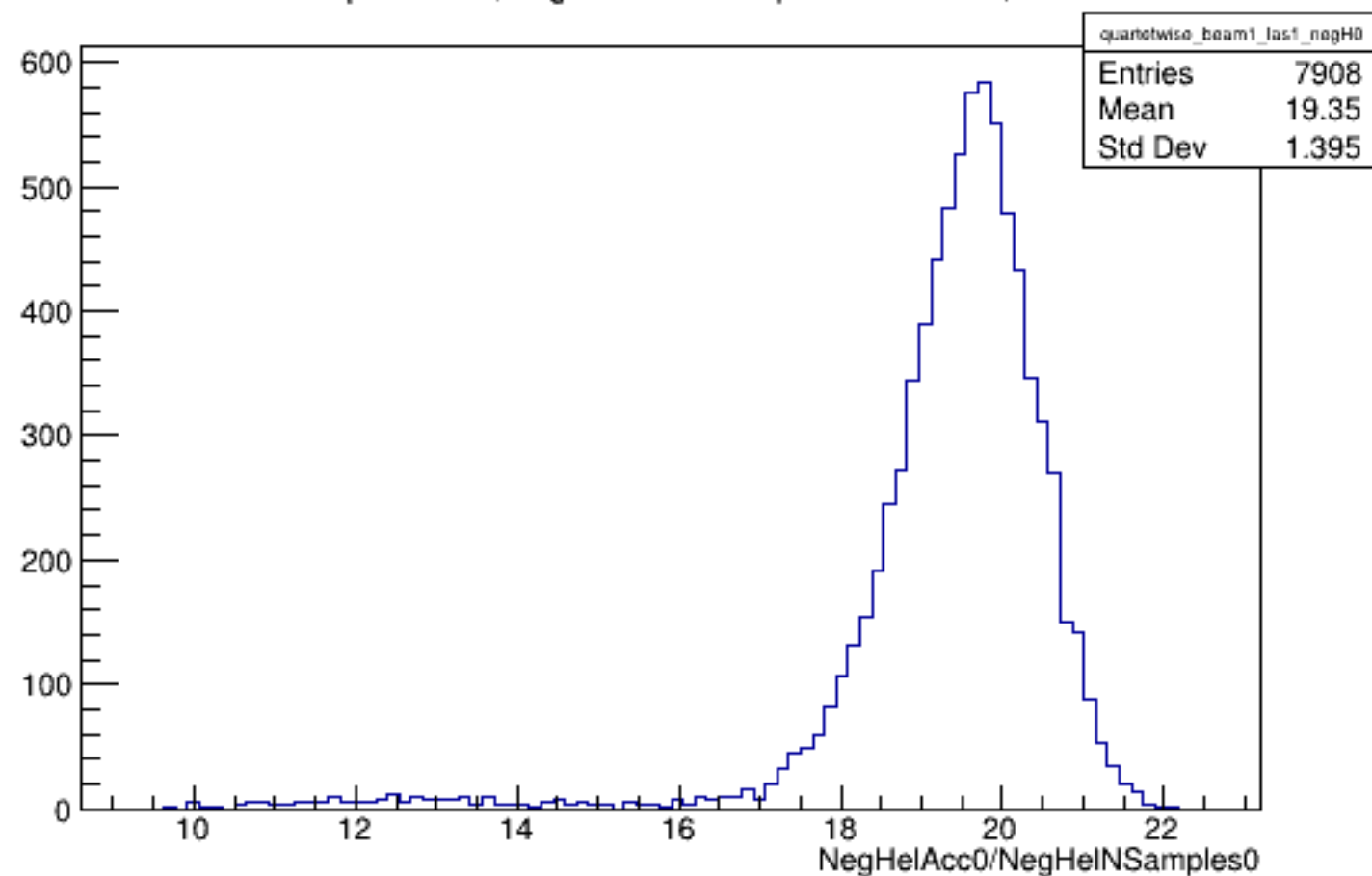
Run 4977 quartetwise, NegHelAcc0/NSamples0: Beam ON, Laser ON
