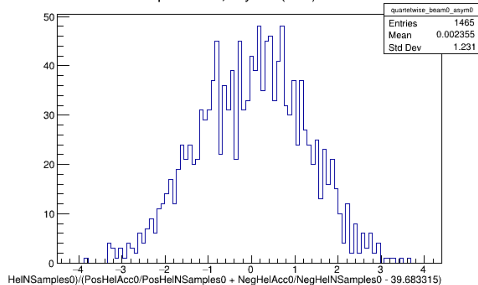
Run 4977 quartetwise, Asyms0 (Raw): Beam OFF
