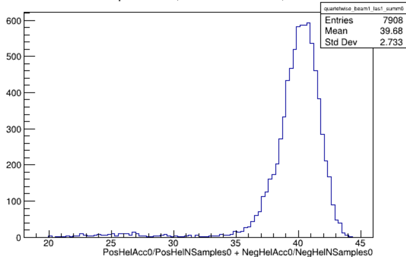
Run 4977 quartetwise, Sums0: Beam ON, Laser ON
