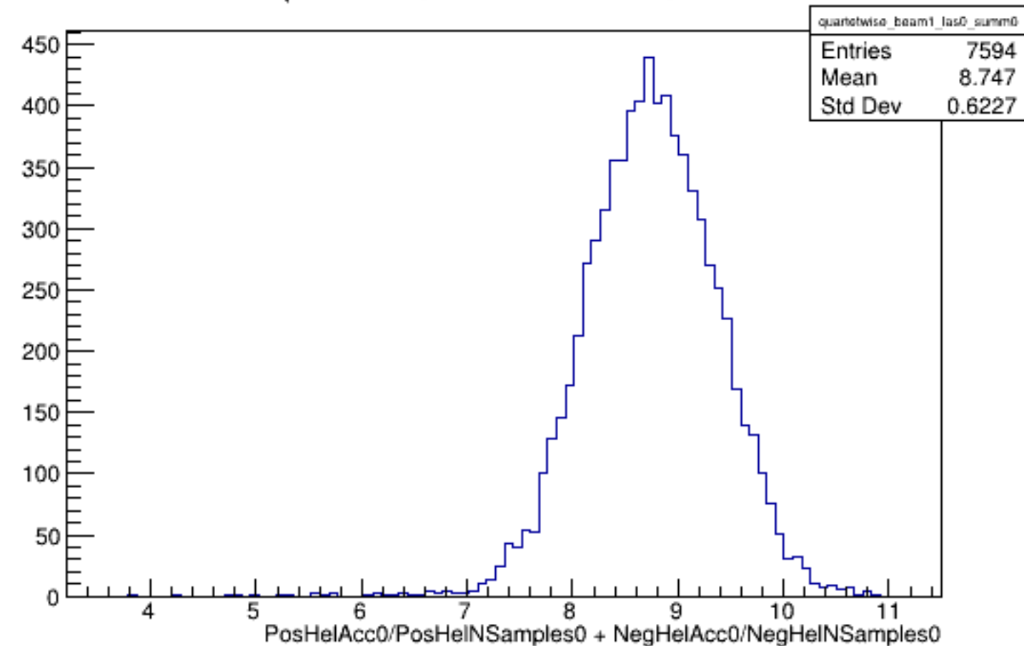
Run 4977 quartetwise, Sums0: Beam ON, Laser OFF
