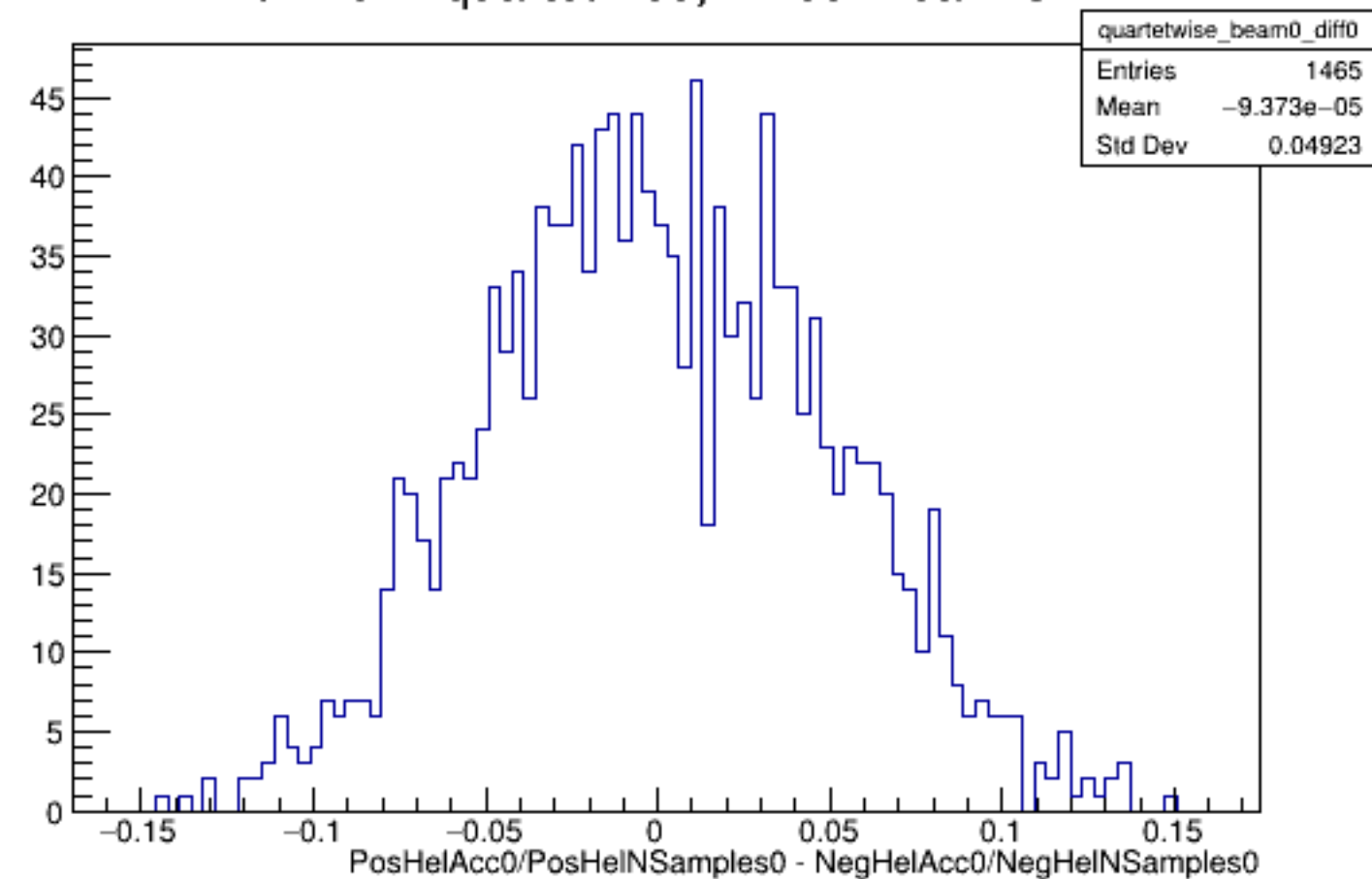
Run 4977 quartetwise, Diffs0: Beam OFF
