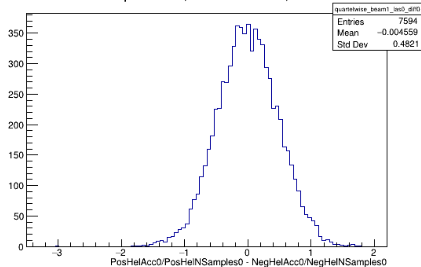
Run 4977 quartetwise, Diffs0: Beam ON, Laser OFF
