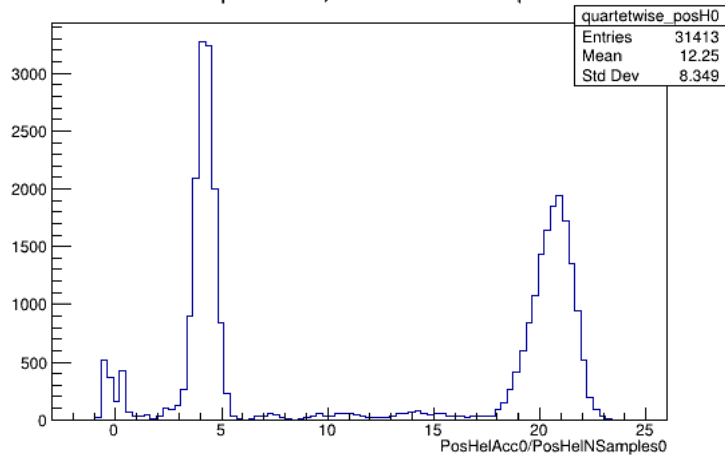
Run 4977 quartetwise, PosHelAcc0/NSamples0: All
