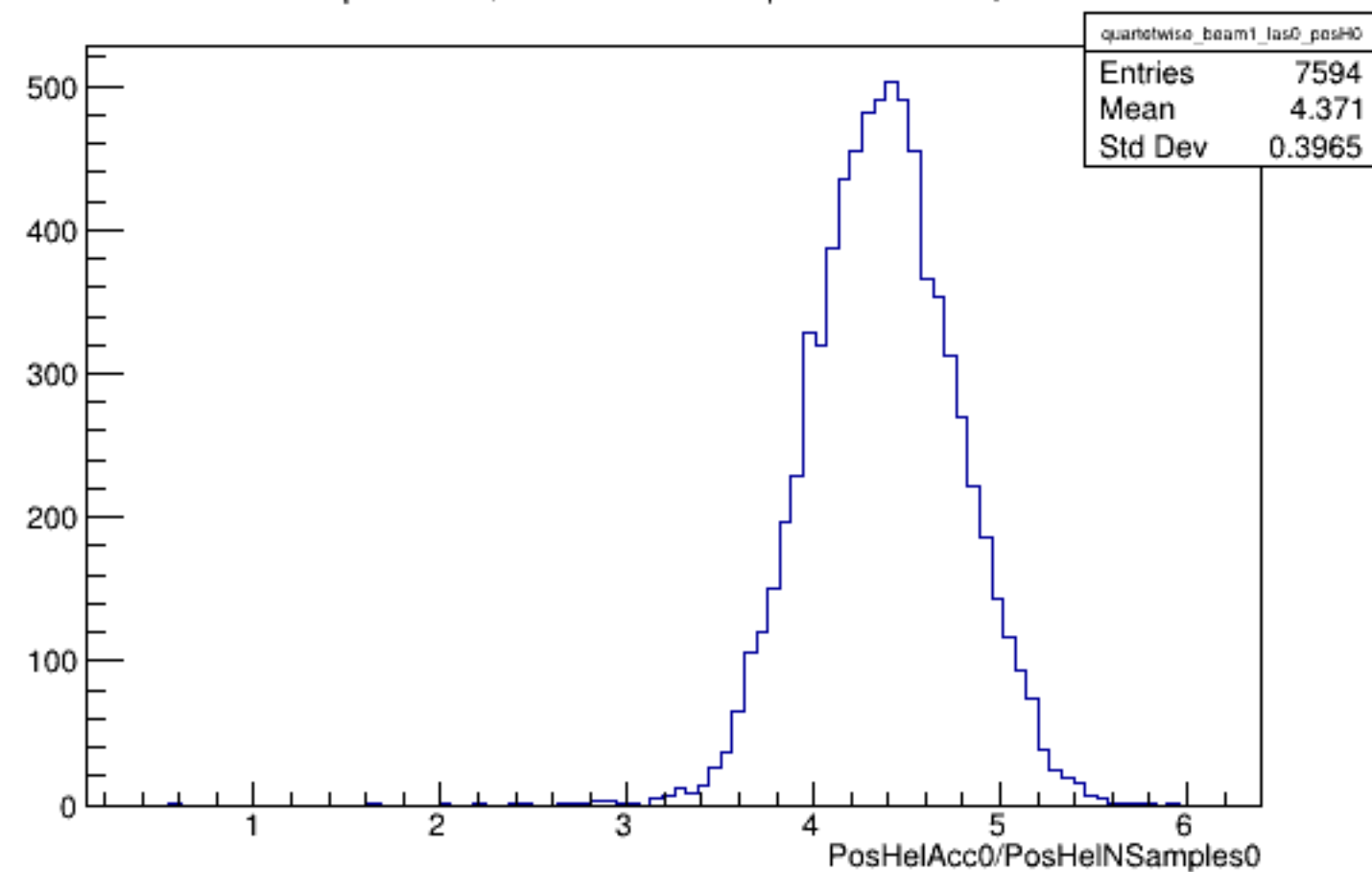
Run 4977 quartetwise, PosHelAcc0/NSamples0: Beam ON, Laser OFF
