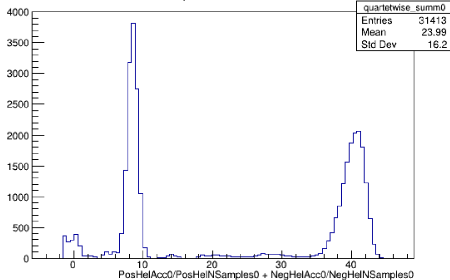
Run 4977 quartetwise, Sums0: All
