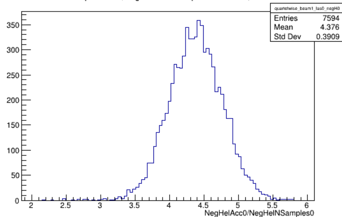
Run 4977 quartetwise, NegHelAcc0/NSamples0: Beam ON, Laser OFF
