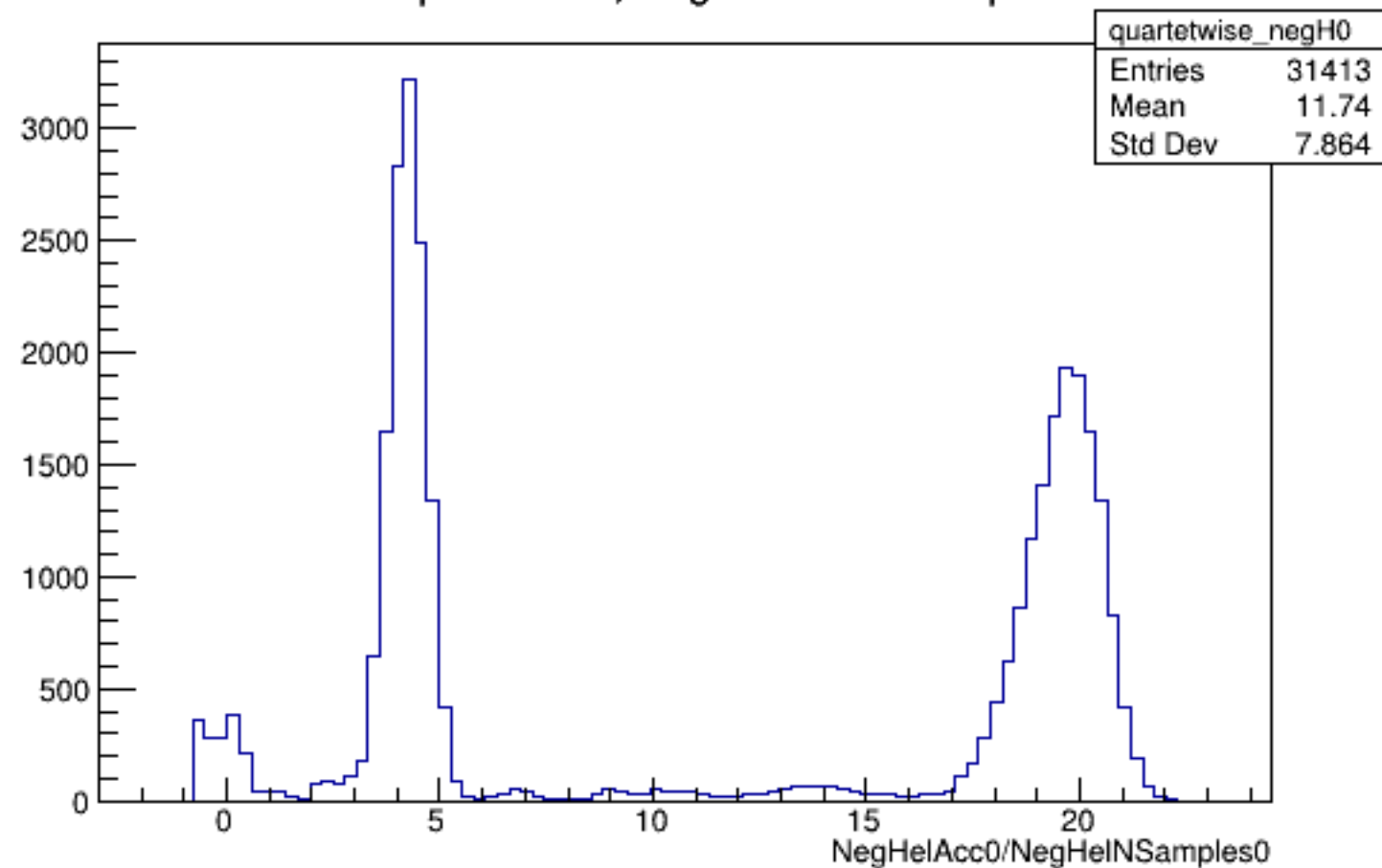
Run 4977 quartetwise, NegHelAcc0/NSamples0: All
