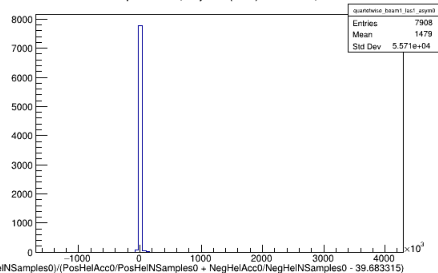
Run 4977 quartetwise, Asyms0 (Raw): Beam ON, Laser ON
