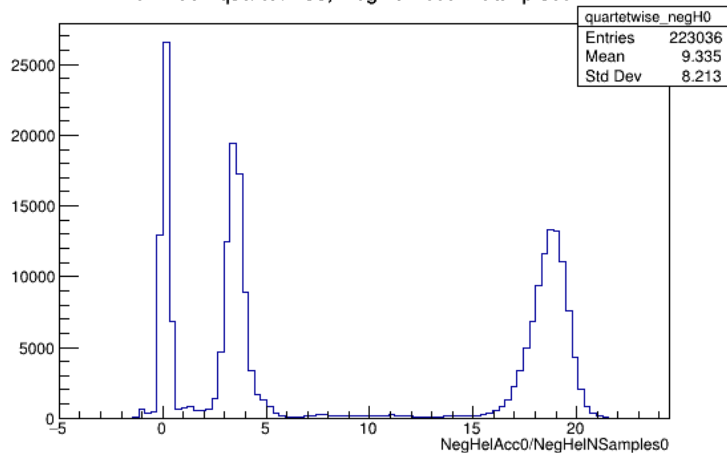
Run 4981 quartetwise, NegHelAcc0/NSamples0: All
