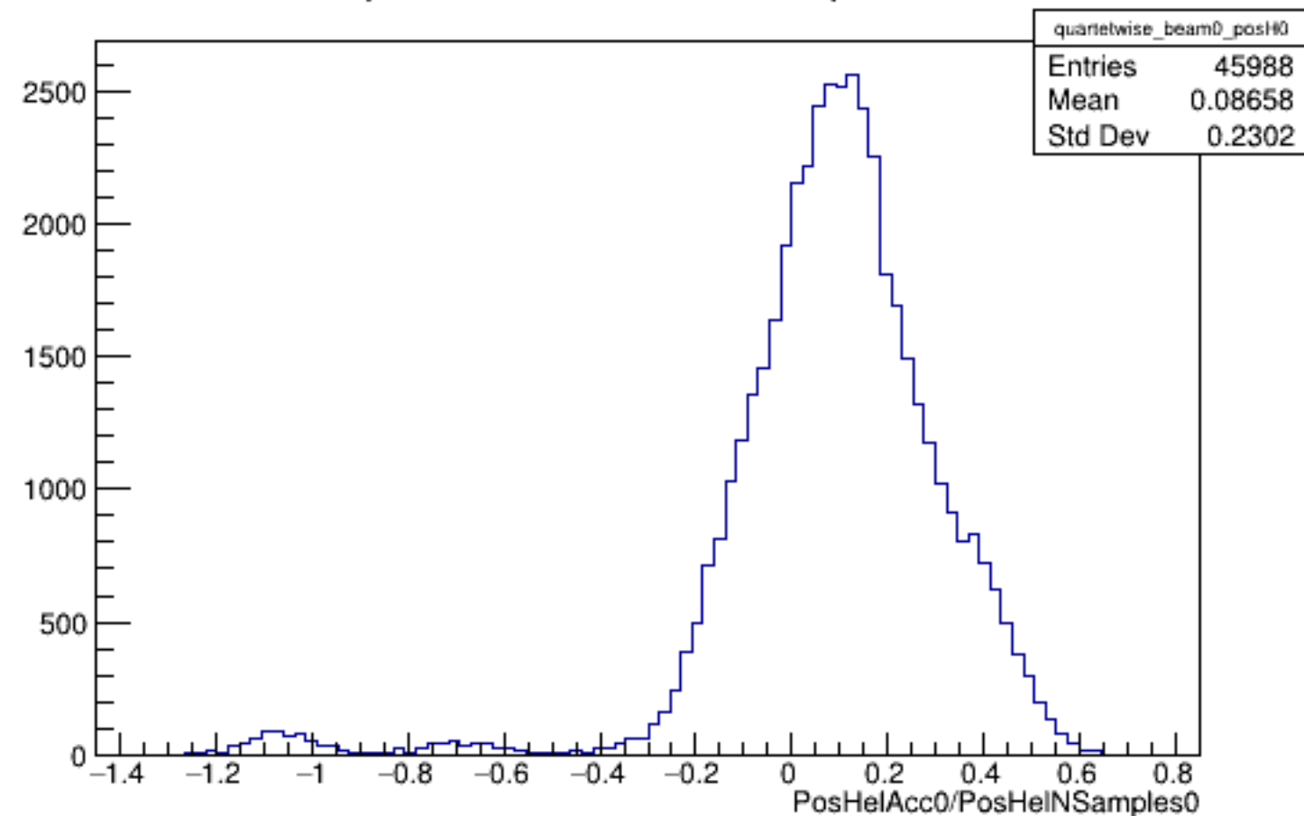
Run 4981 quartetwise, PosHelAcc0/NSamples0: Beam OFF
