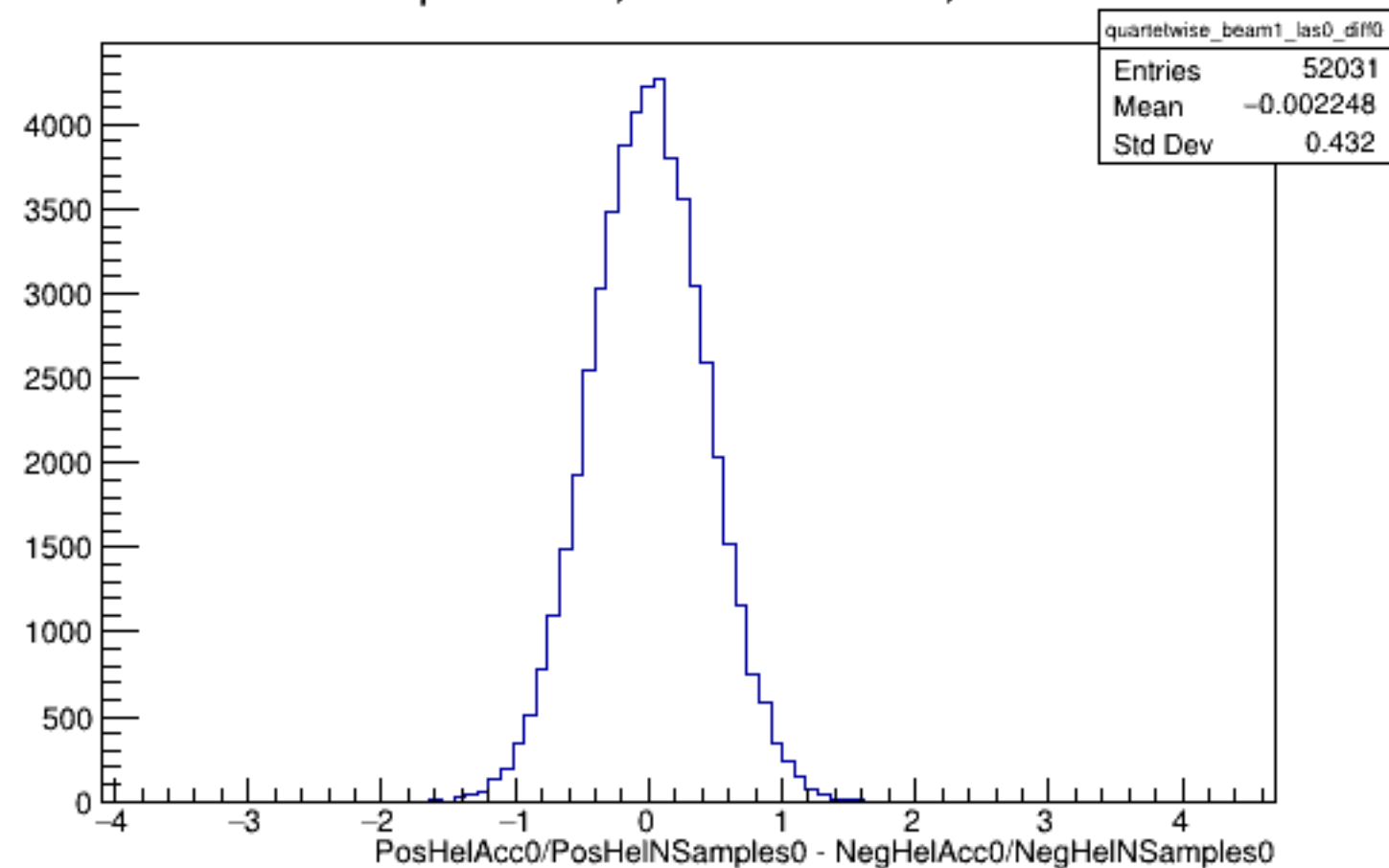
Run 4981 quartetwise, Diffs0: Beam ON, Laser OFF
