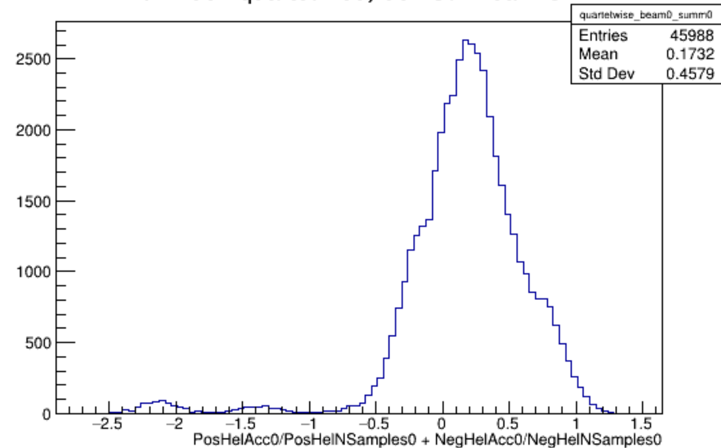
Run 4981 quartetwise, Sums0: Beam OFF
