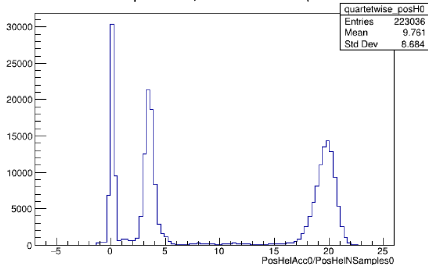
Run 4981 quartetwise, PosHelAcc0/NSamples0: All
