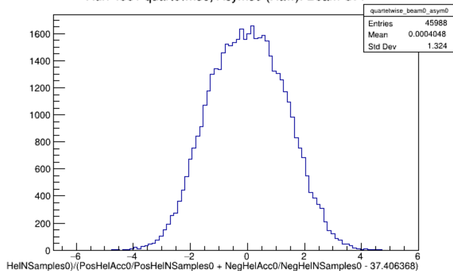
Run 4981 quartetwise, Asyms0 (Raw): Beam OFF
