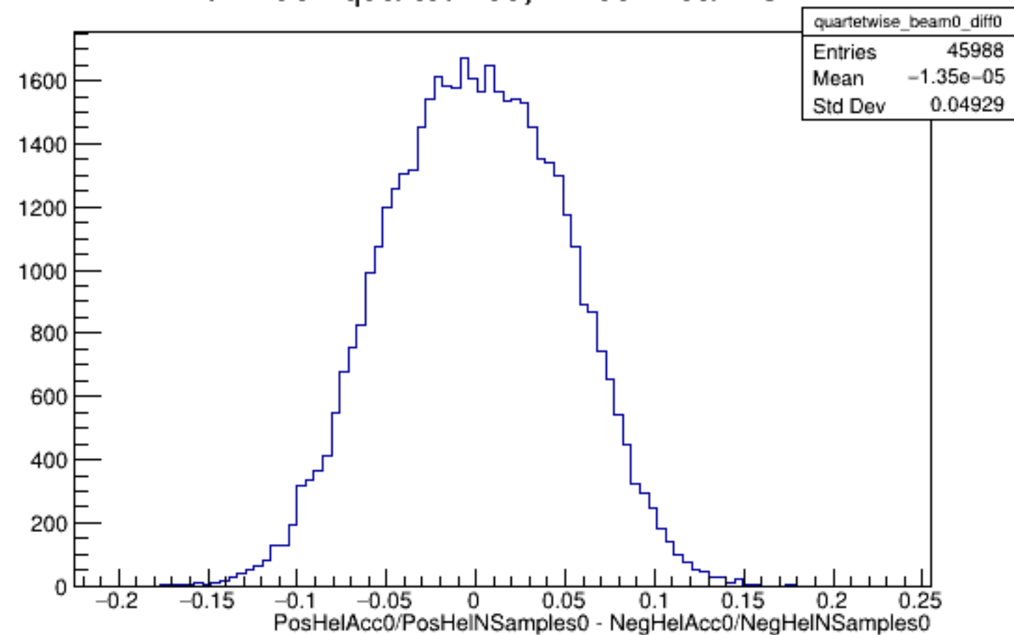
Run 4981 quartetwise, Diffs0: Beam OFF
