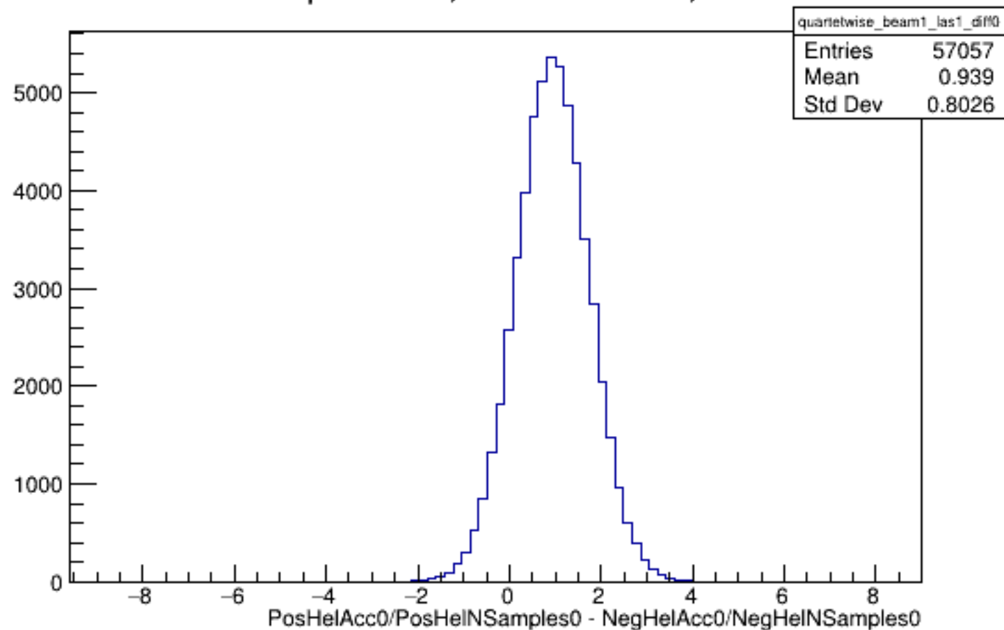
Run 4981 quartetwise, Diffs0: Beam ON, Laser ON
