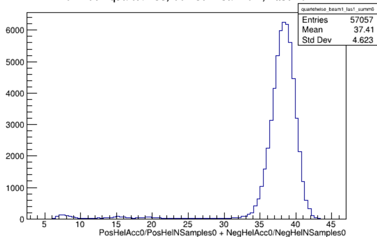
Run 4981 quartetwise, Sums0: Beam ON, Laser ON
