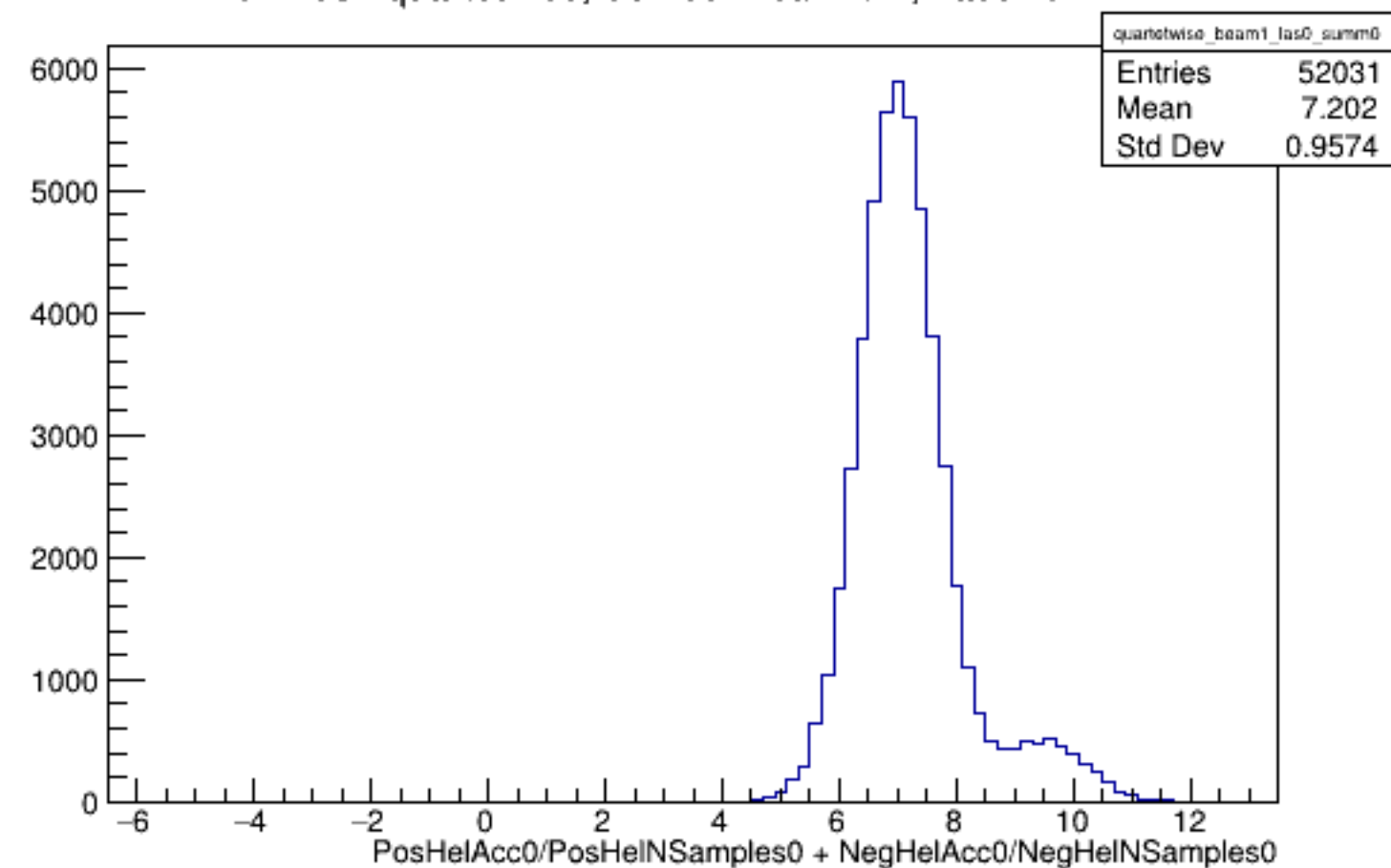
Run 4981 quartetwise, Sums0: Beam ON, Laser OFF
