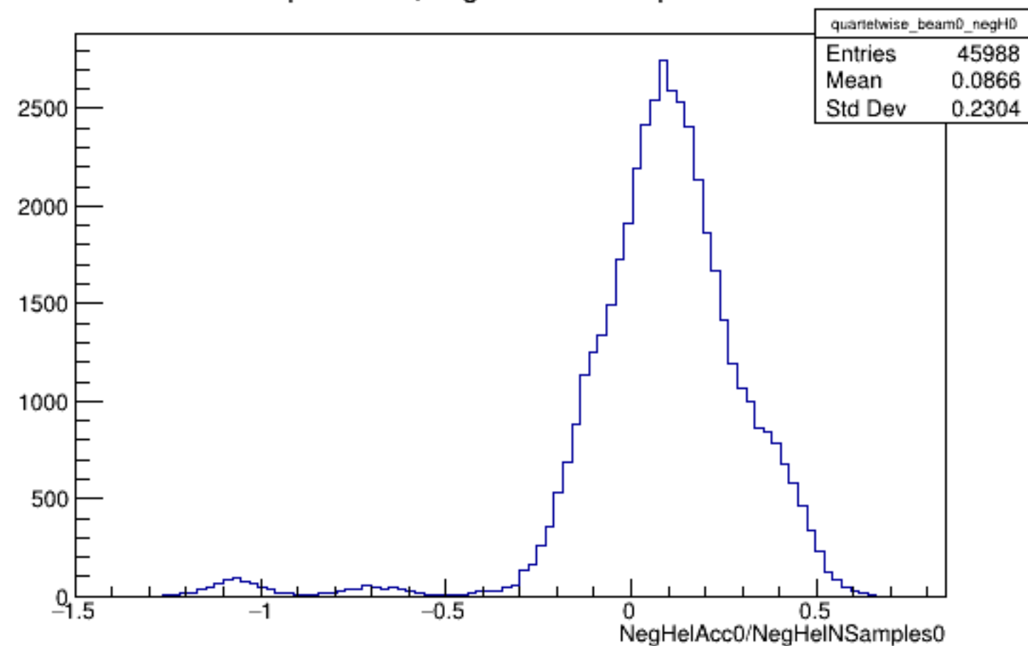
Run 4981 quartetwise, NegHelAcc0/NSamples0: Beam OFF
