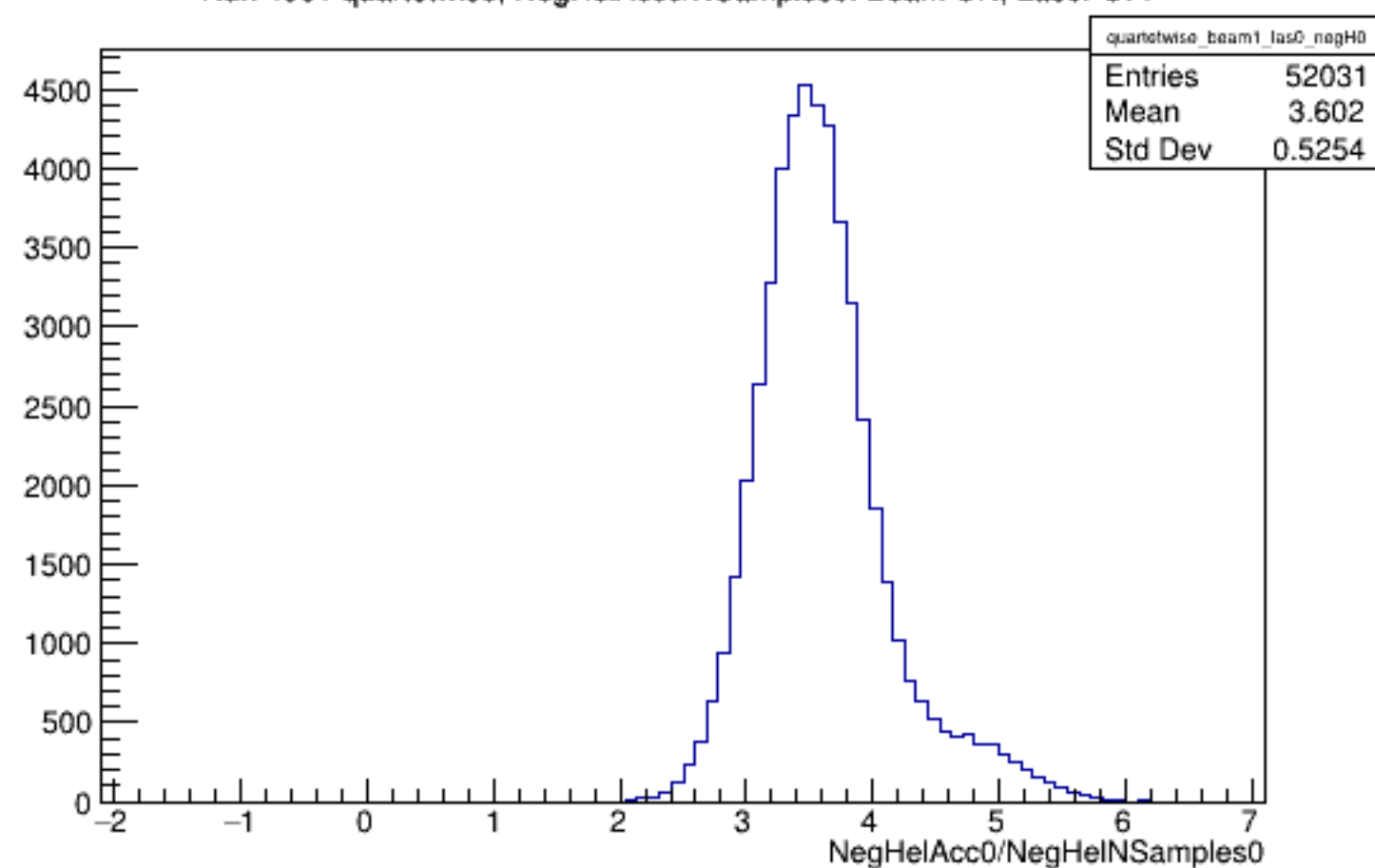
Run 4981 quartetwise, NegHelAcc0/NSamples0: Beam ON, Laser OFF
