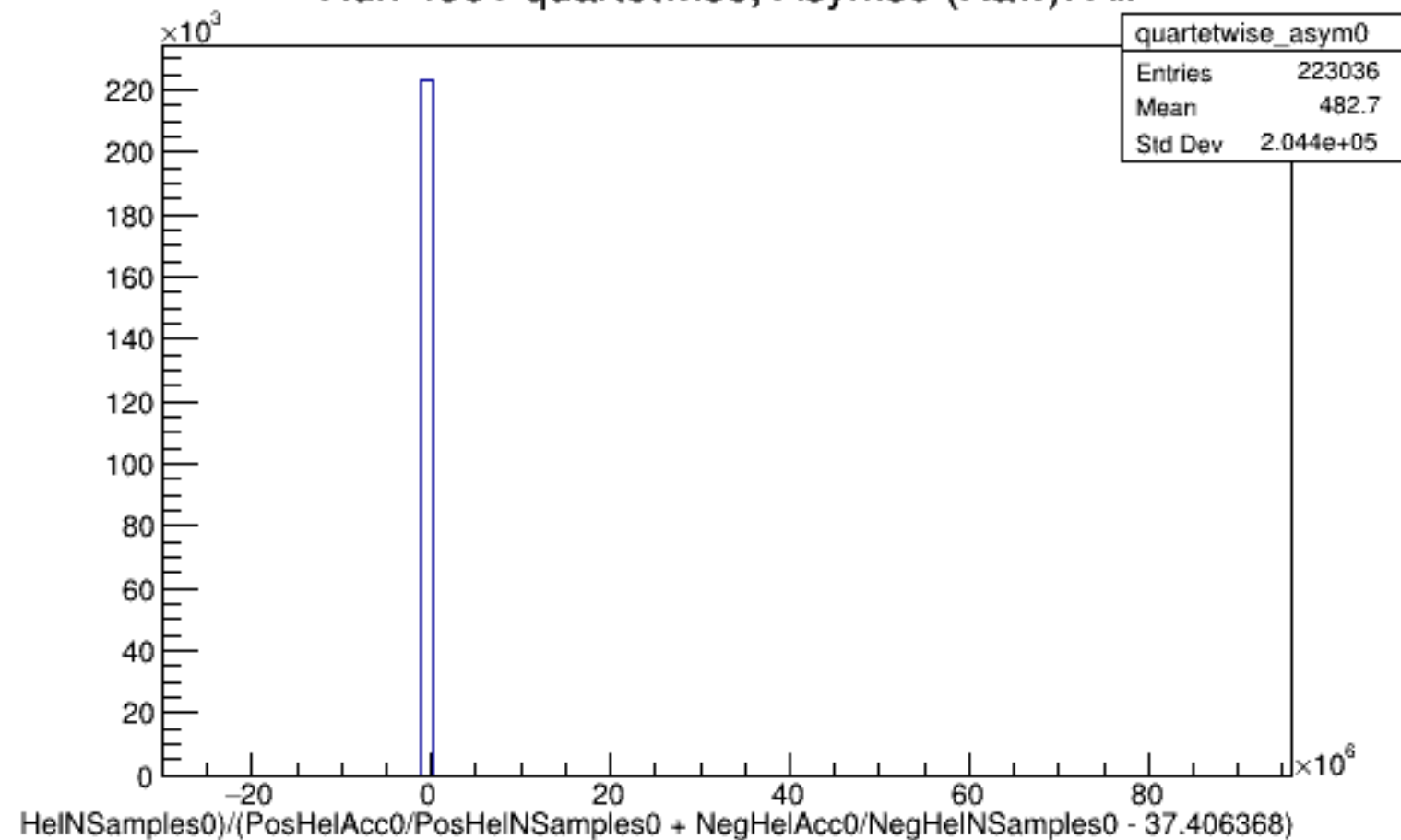
Run 4981 quartetwise, Asyms0 (Raw): All
