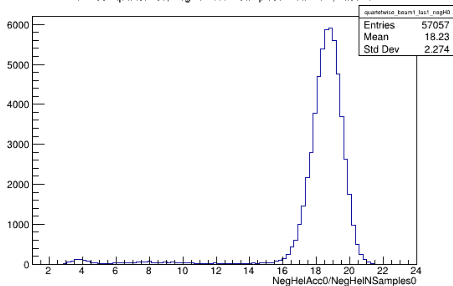
Run 4981 quartetwise, NegHelAcc0/NSamples0: Beam ON, Laser ON
