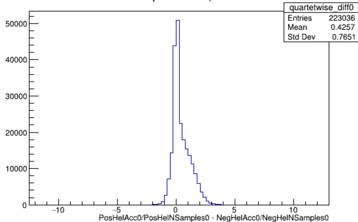
Run 4981 quartetwise, Diffs0: All
