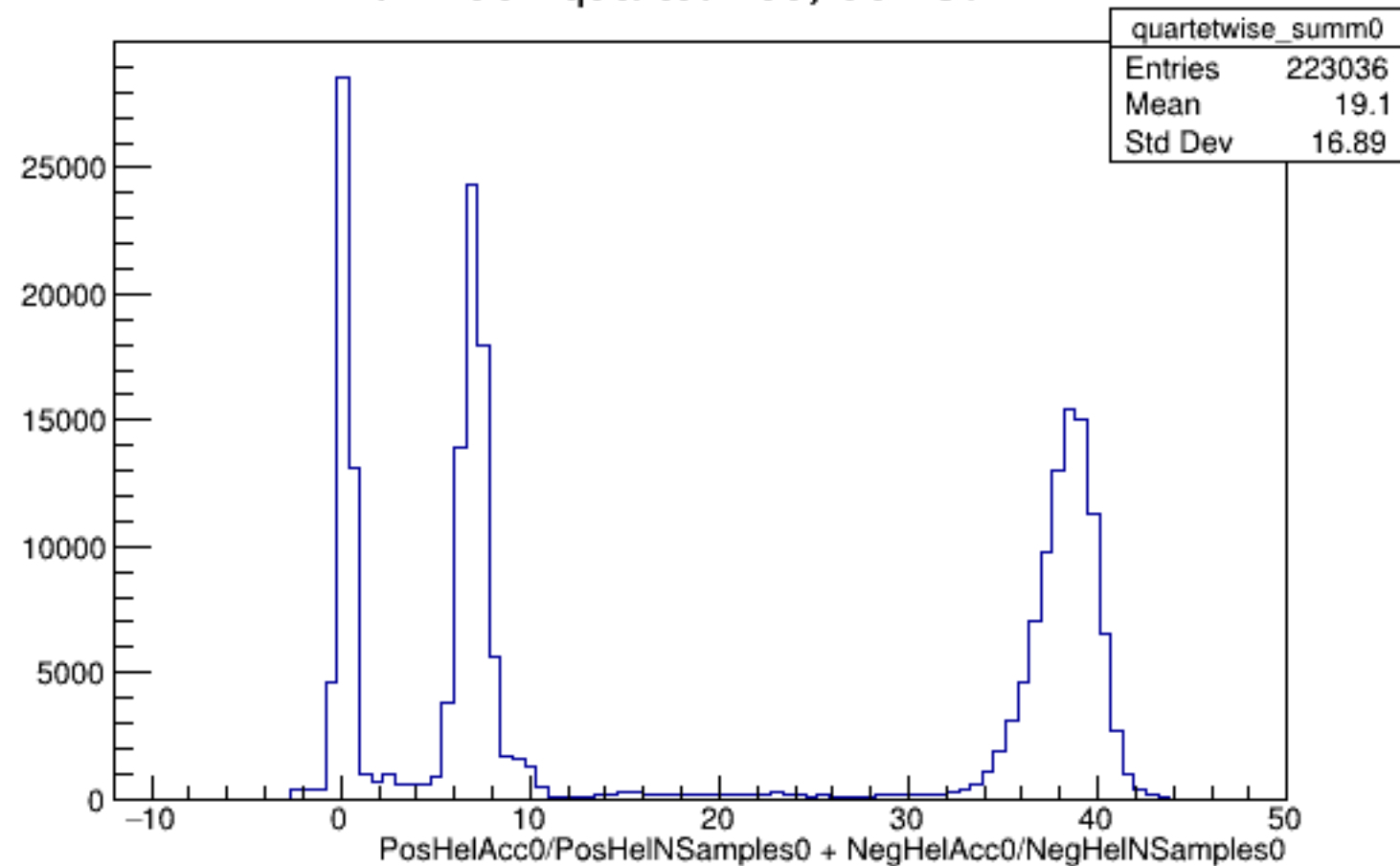
Run 4981 quartetwise, Sums0: All
