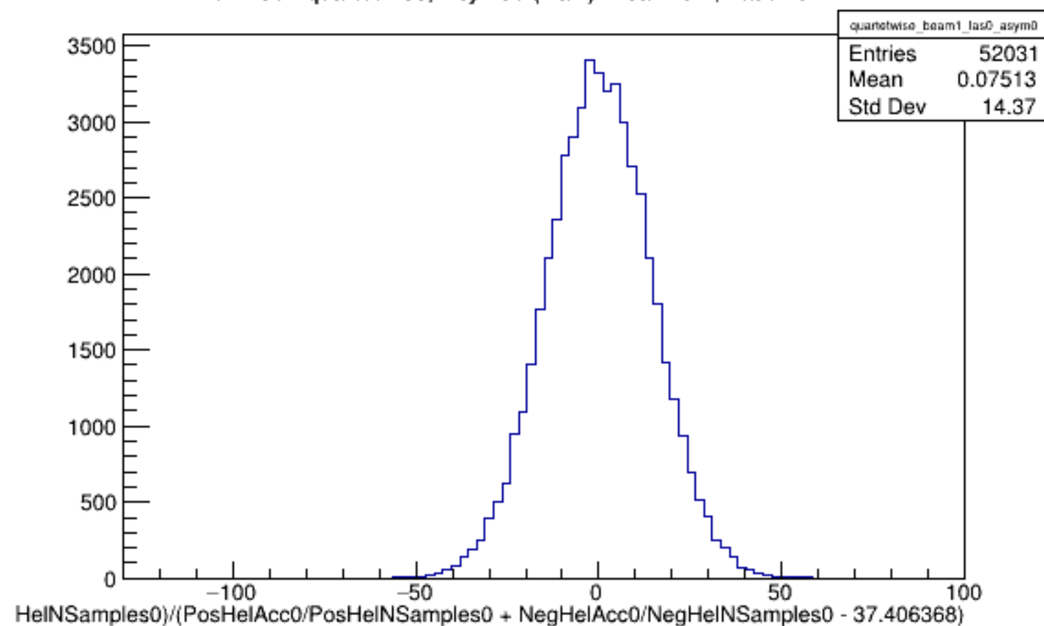
Run 4981 quartetwise, Asyms0 (Raw): Beam ON, Laser OFF
