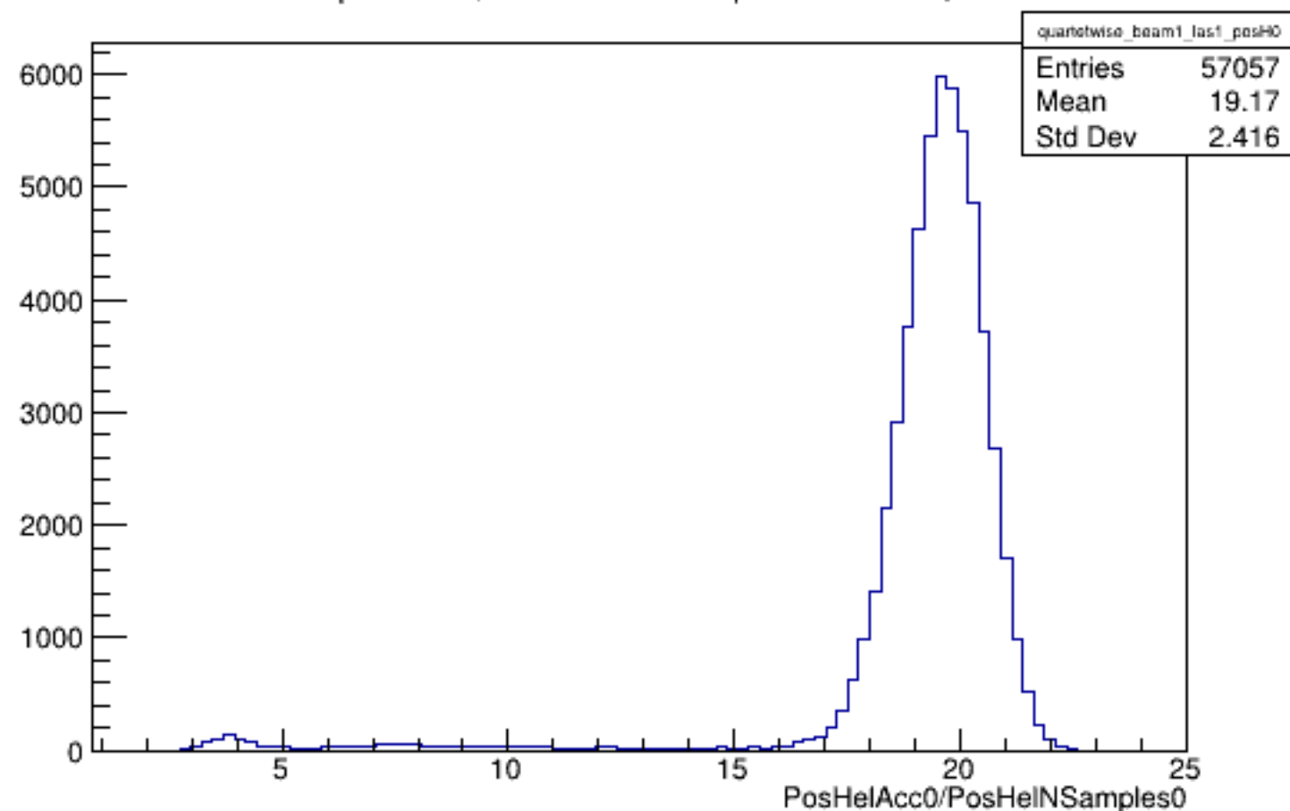
Run 4981 quartetwise, PosHelAcc0/NSamples0: Beam ON, Laser ON
