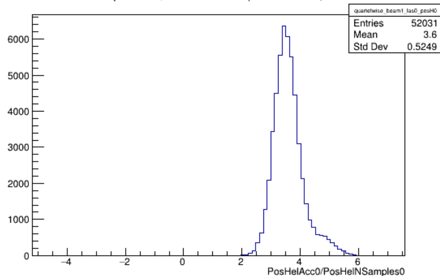
Run 4981 quartetwise, PosHelAcc0/NSamples0: Beam ON, Laser OFF
