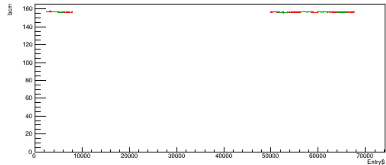
Run 4985 quartetwise, posH4 vs time
