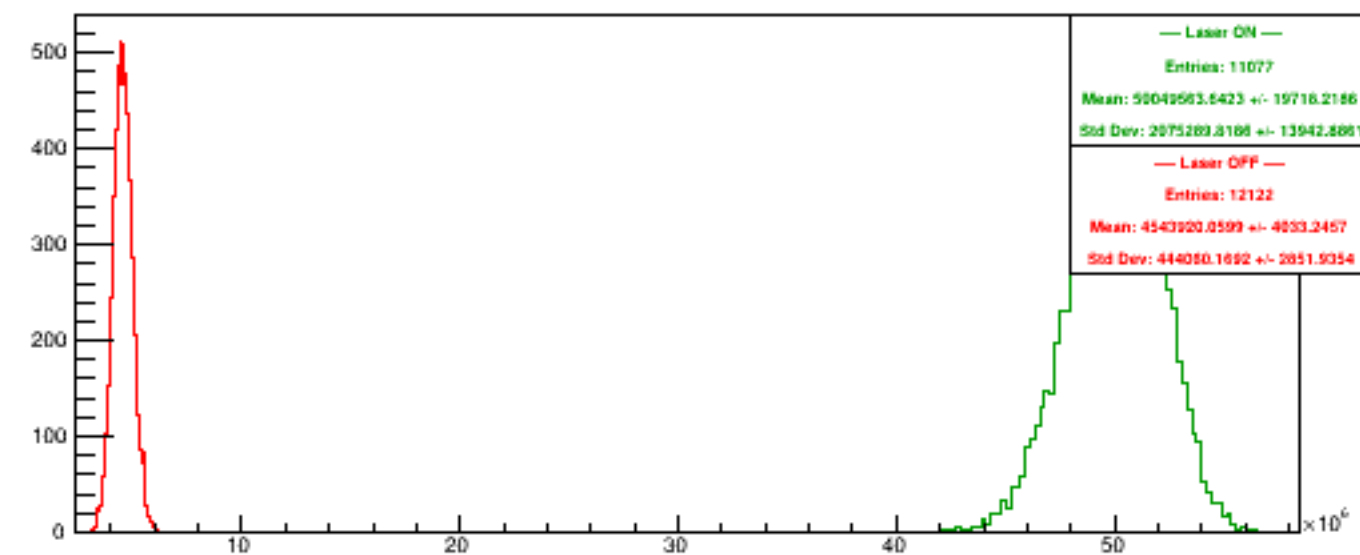
Run 4985 quartetwise, NegHelAcc4
