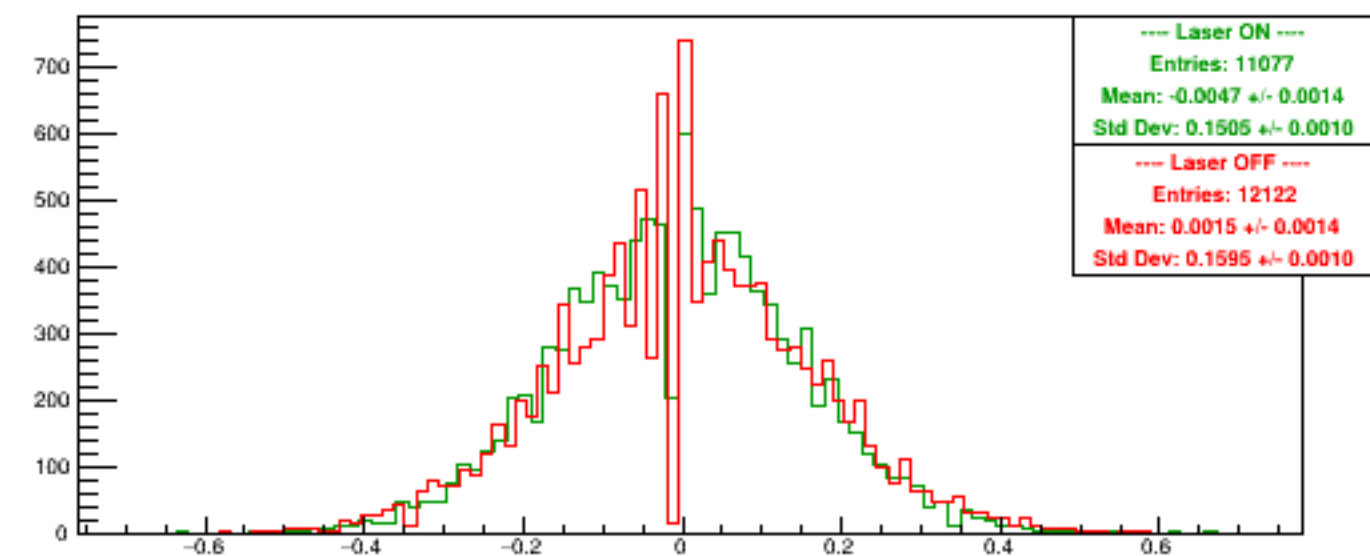
Run 4985 quartetwise, Asyms Horiz Finger
