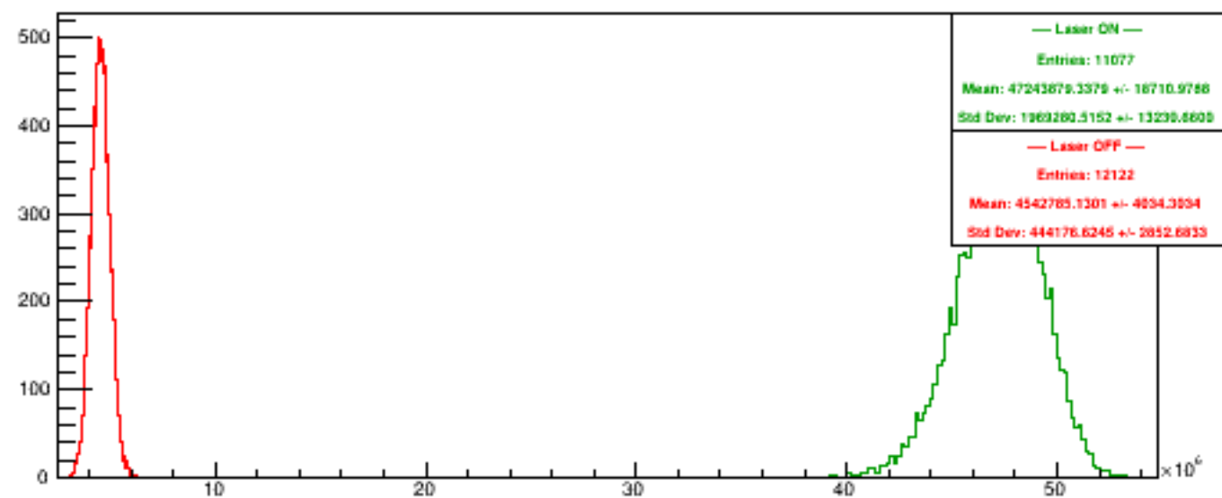
Run 4985 quartetwise, PosHelAcc4
