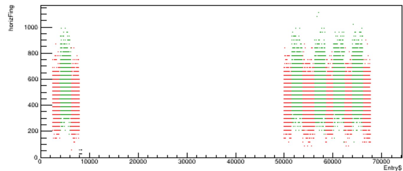
Run 4985 quartetwise, horizFing vs time
