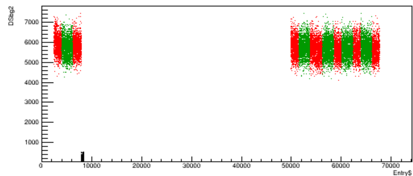
Run 4985 quartetwise, DSbg2 vs time
