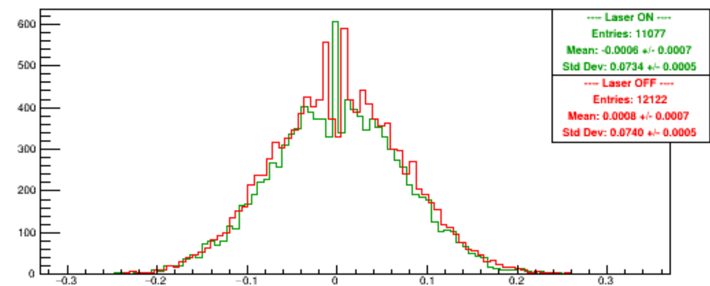
Run 4985 quartetwise, Asyms DSbg2
