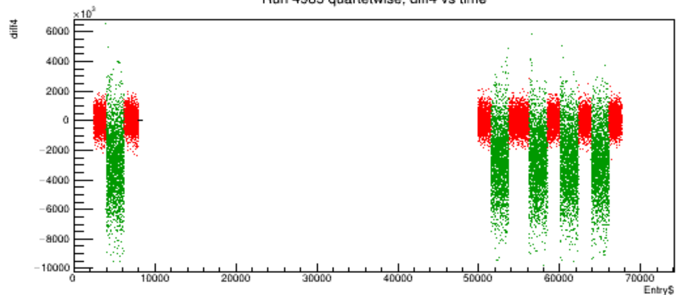
Run 4985 quartetwise, diff4 vs time
