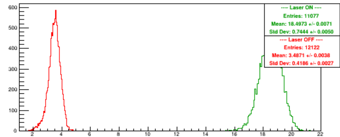
Run 4985 quartetwise, NegHelAcc0/NSamples0
