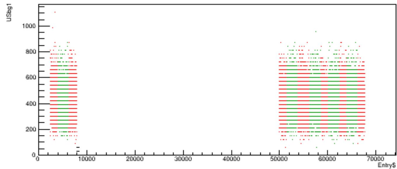
Run 4985 quartetwise, USbg1 vs time
