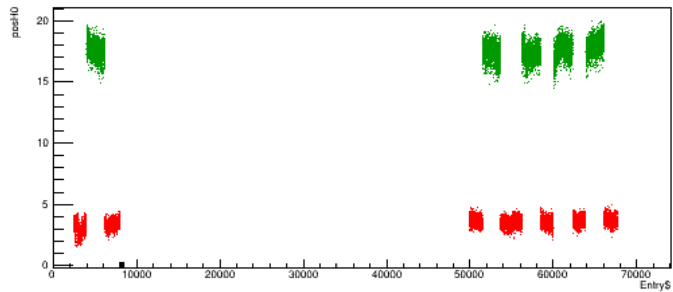
Run 4985 quartetwise, posH0 vs time
