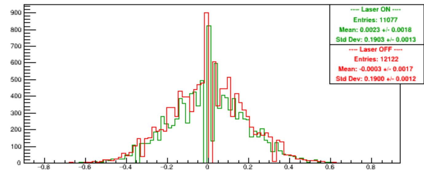
Run 4985 quartetwise, Asyms USbg2
