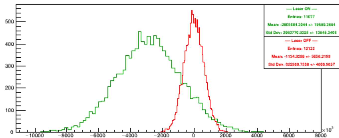
Run 4985 quartetwise, Diffs4
