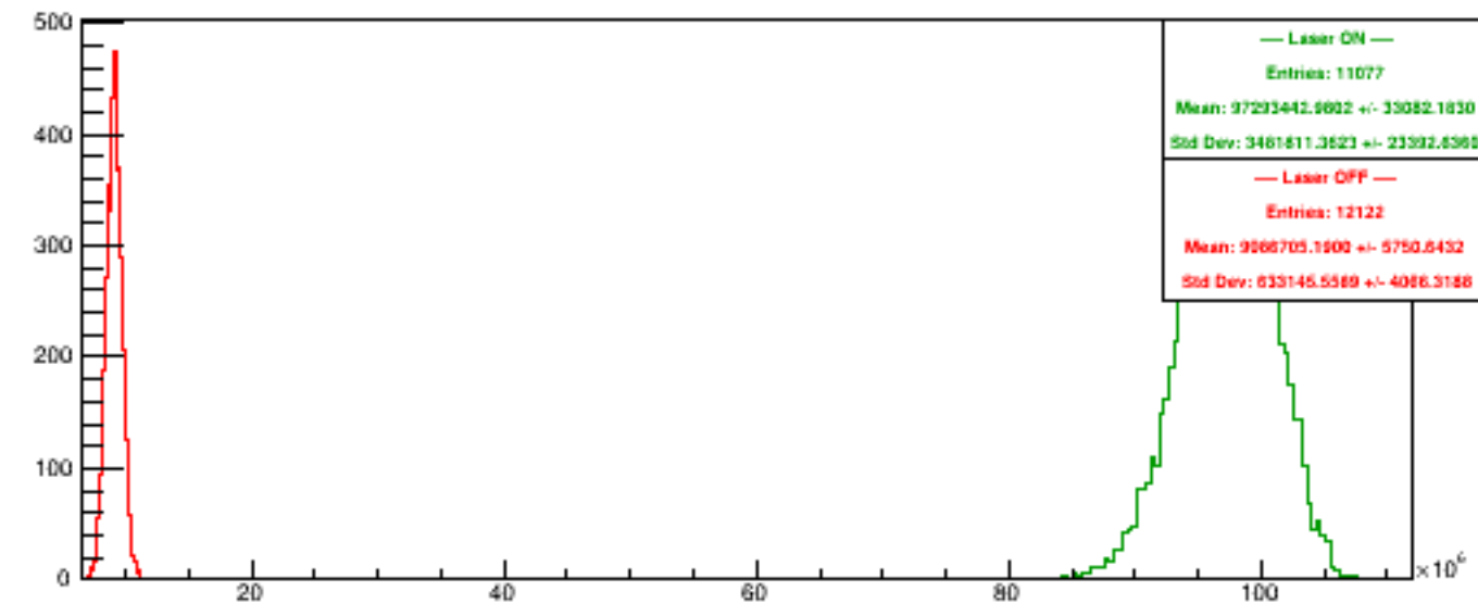
Run 4985 quartetwise, Sums4
