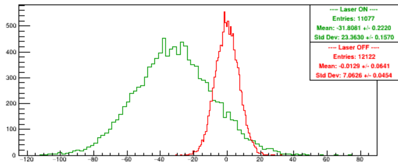
Run 4985 quartetwise, Asyms4
