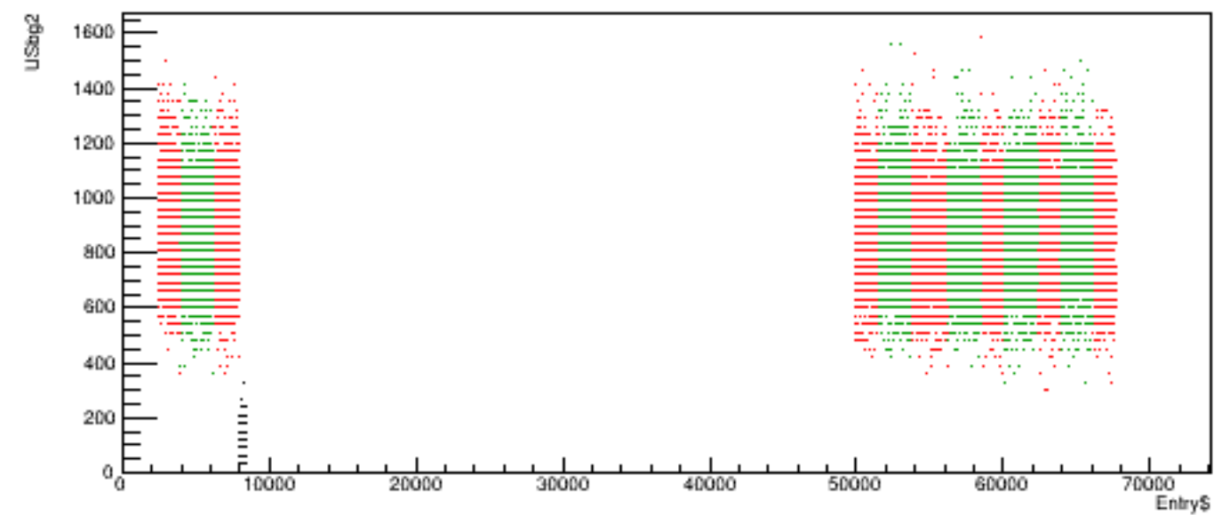
Run 4985 quartetwise, USbg2 vs time
