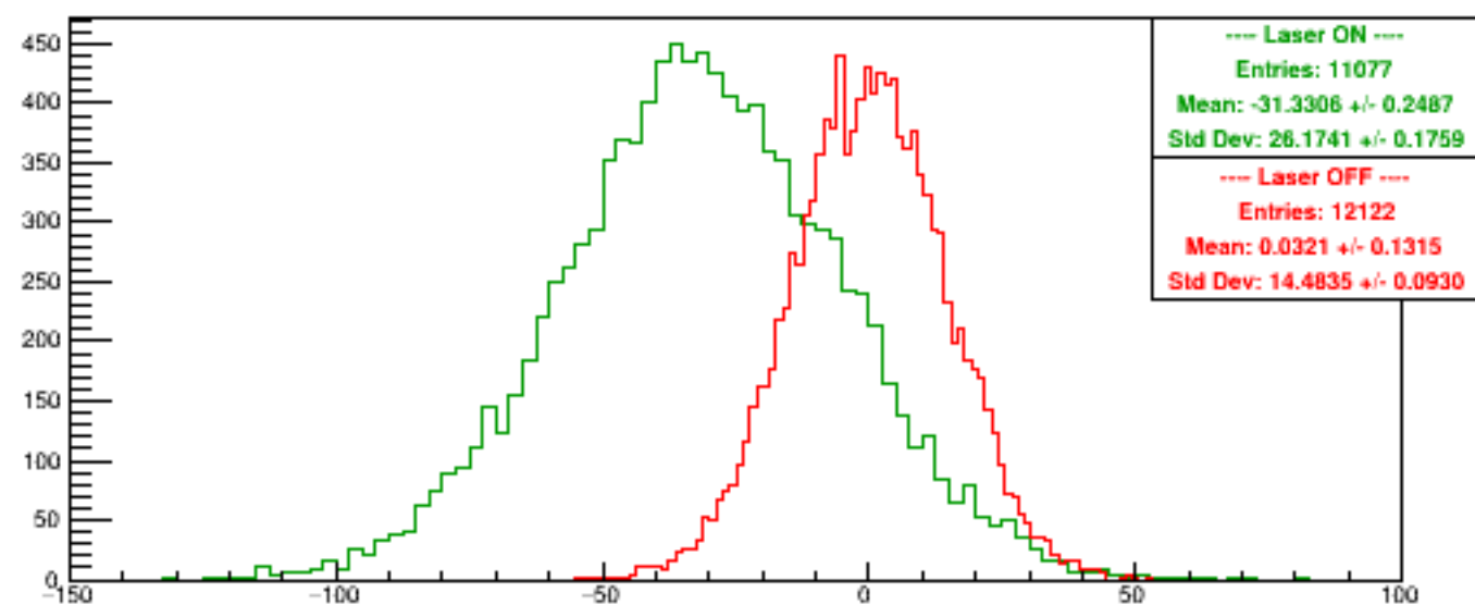
Run 4985 quartetwise, Asyms0
