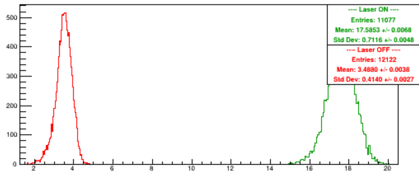
Run 4985 quartetwise, PosHelAcc0/NSamples0
