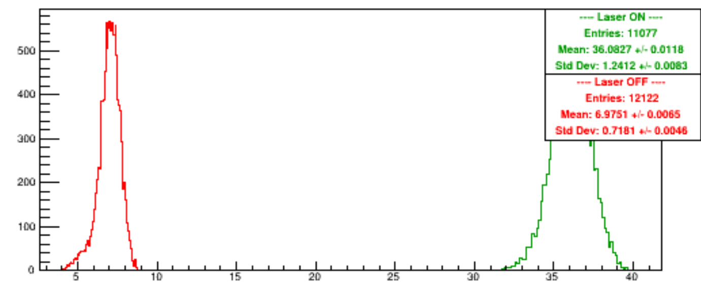
Run 4985 quartetwise, Sums0
