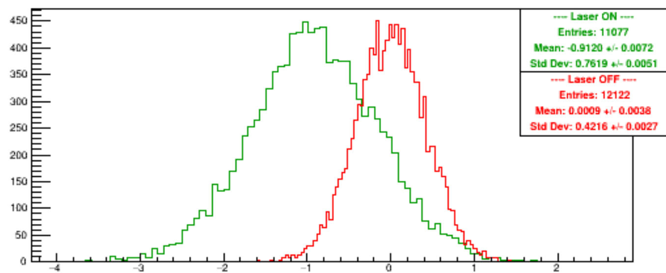
Run 4985 quartetwise, Diffs0
