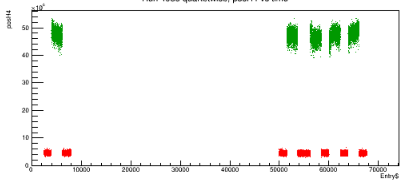
Run 4985 quartetwise, posH4 vs time
