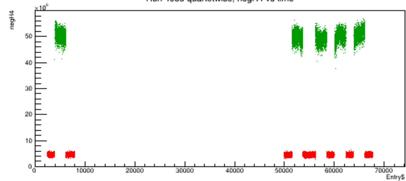
Run 4985 quartetwise, negH4 vs time
