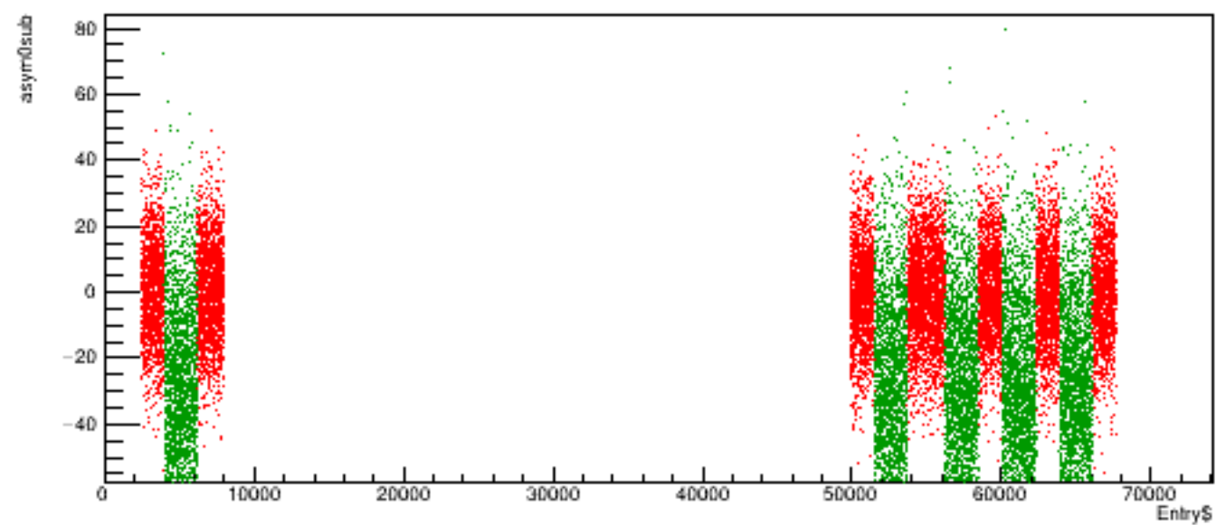
Run 4985 quartetwise, asym0sub vs time
