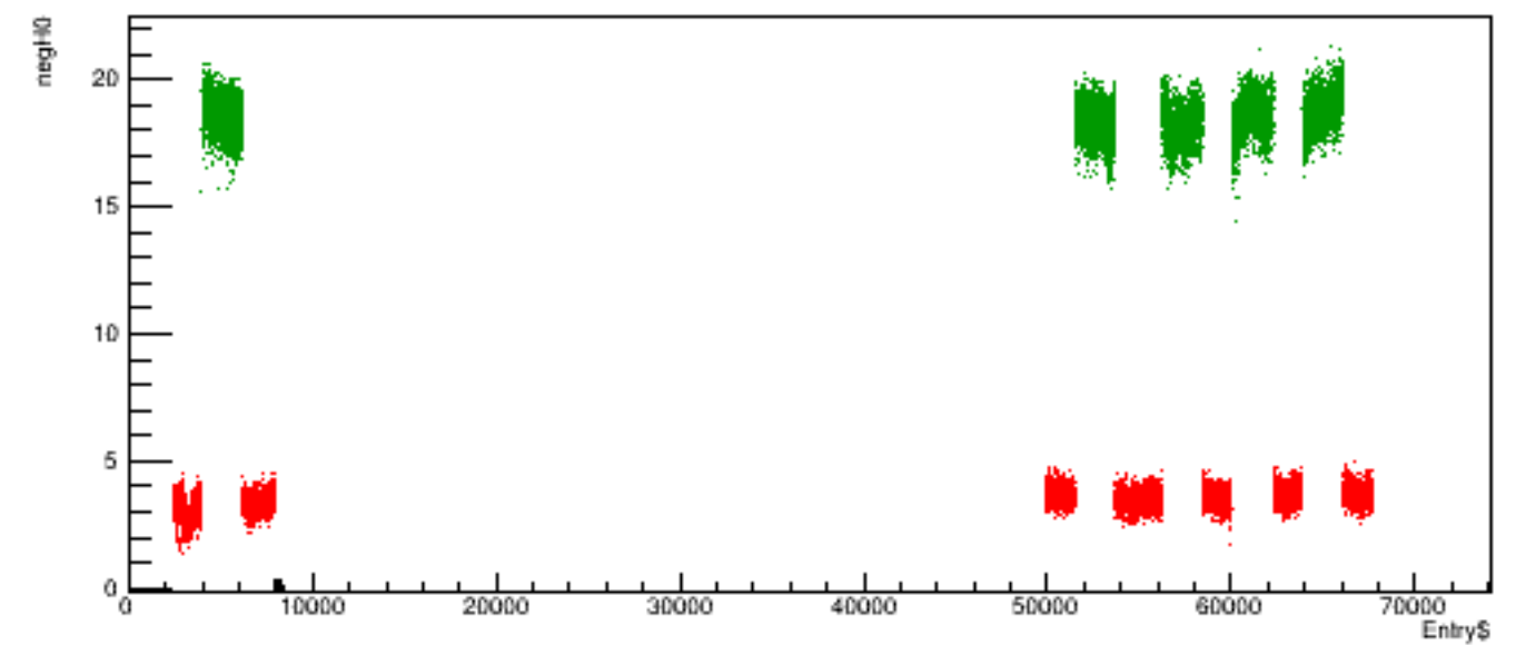
Run 4985 quartetwise, negH0 vs time
