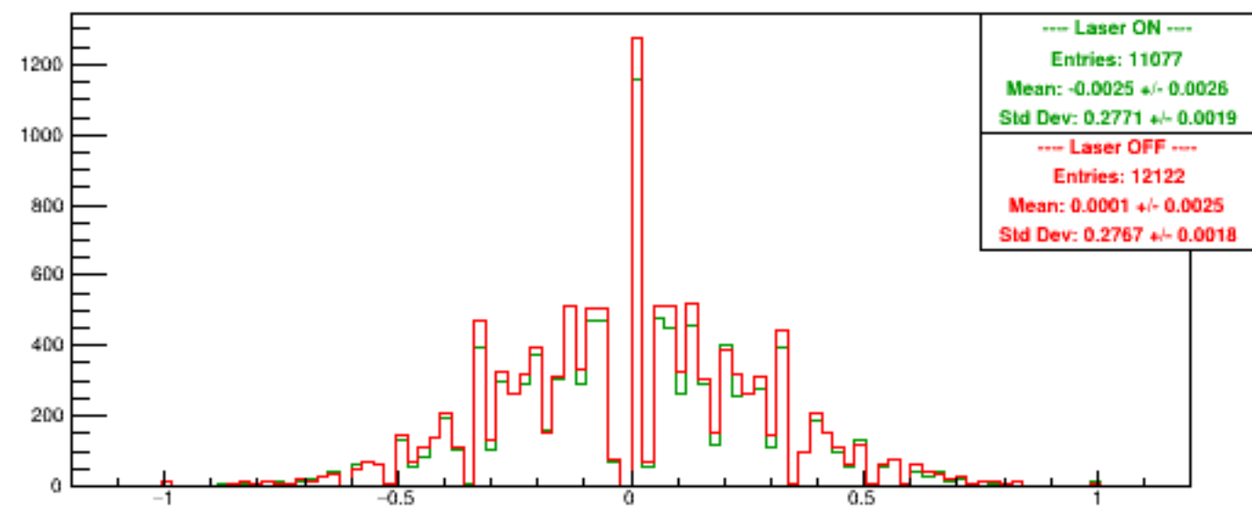
Run 4985 quartetwise, Asyms USbg1
