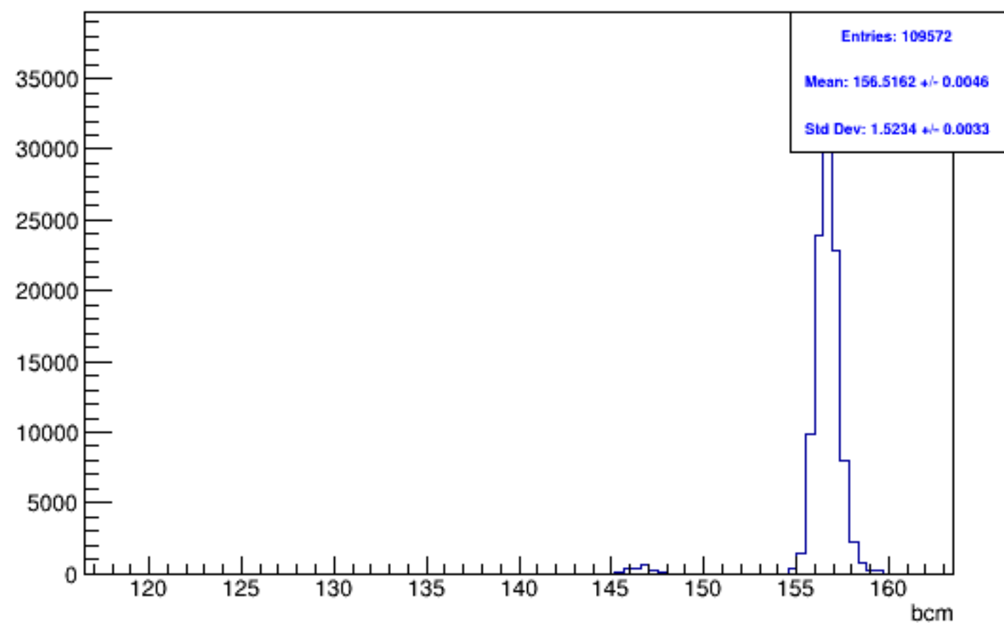
Run 4988, mpwise, BCM: Beam ON, Laser ON
