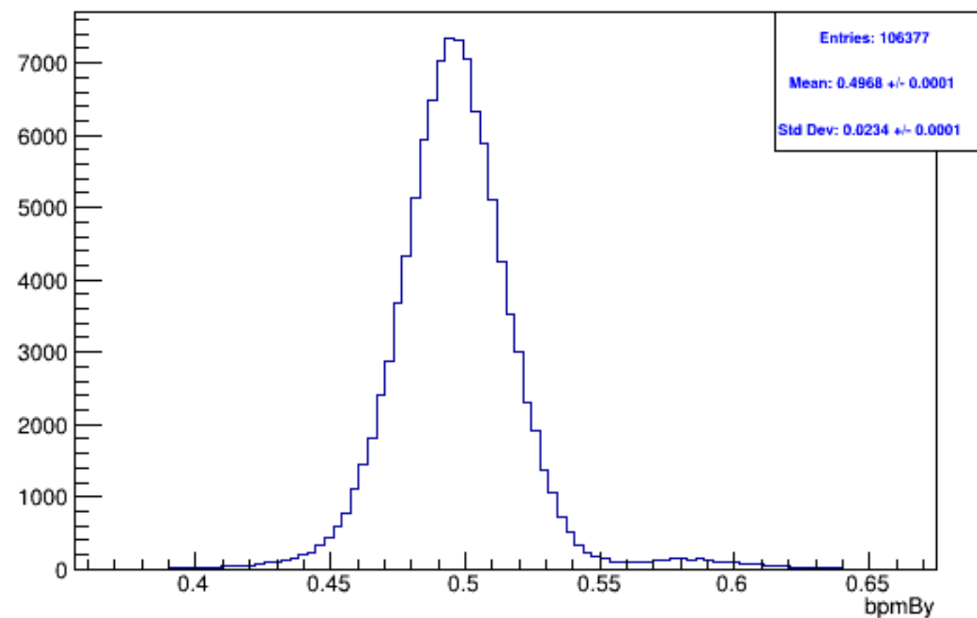
Run 4988, mpwise, bpmBy: Beam ON, Laser OFF
