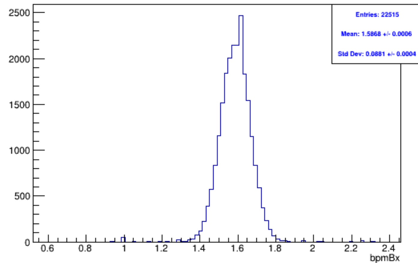
Run 4988 mpswise, bpmBx: Beam OFF
