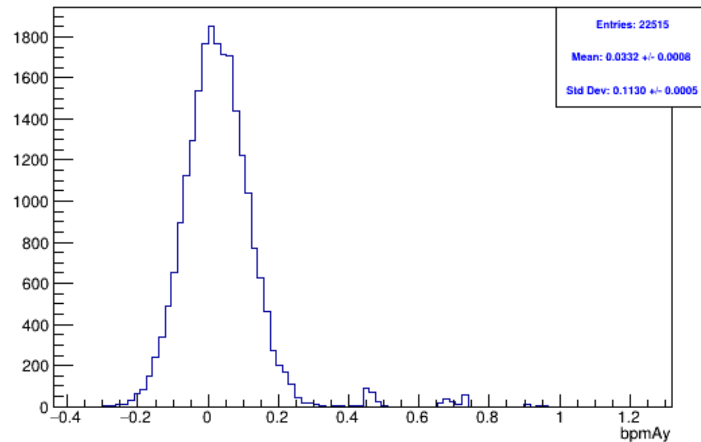
Run 4988 mpwise, bpmAy: Beam OFF
