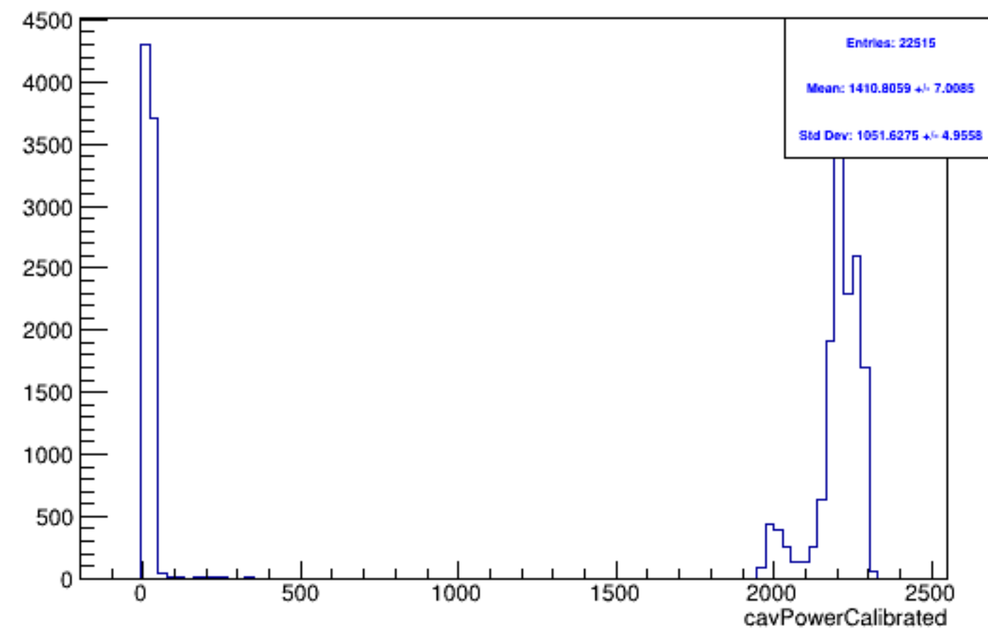
Run 4988 mpwise, lasPow: Beam OFF
