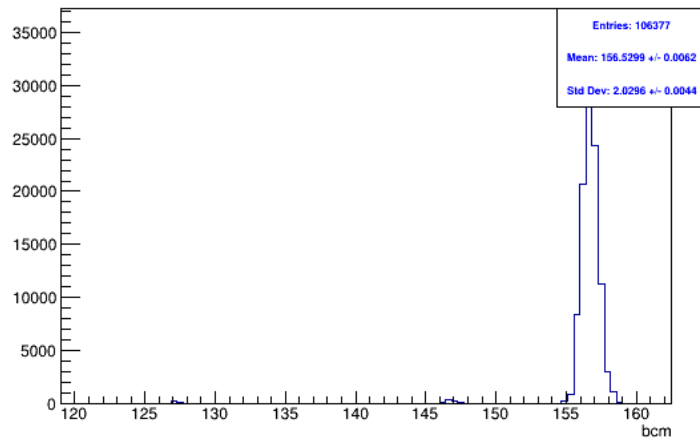
Run 4988, mpwise, BCM: Beam ON, Laser OFF
