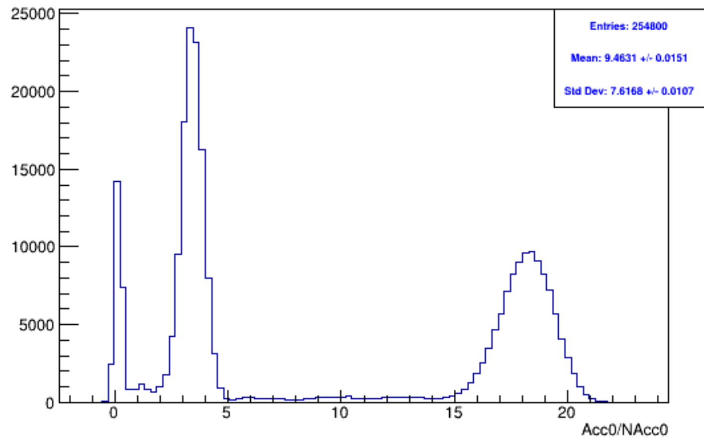
Run 4988 mpwise, acc0: All
