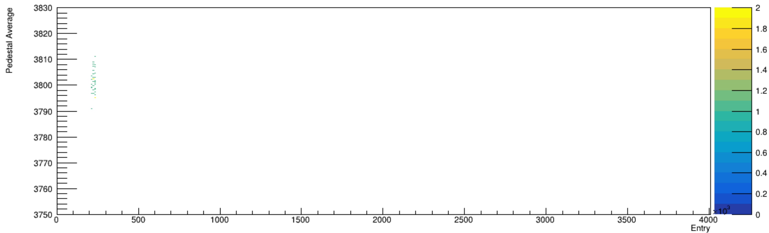
Run 5016, snapshots: Pedestal vs. Time
