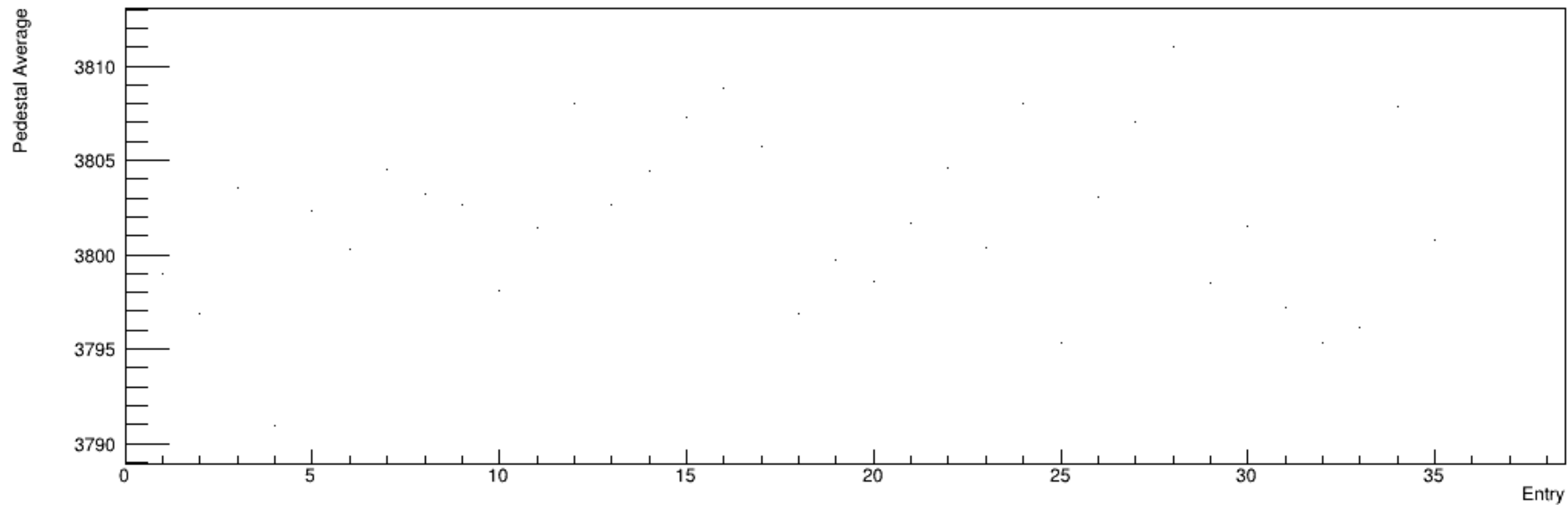
Run 5016, snapshots: Pedestal vs. Time
