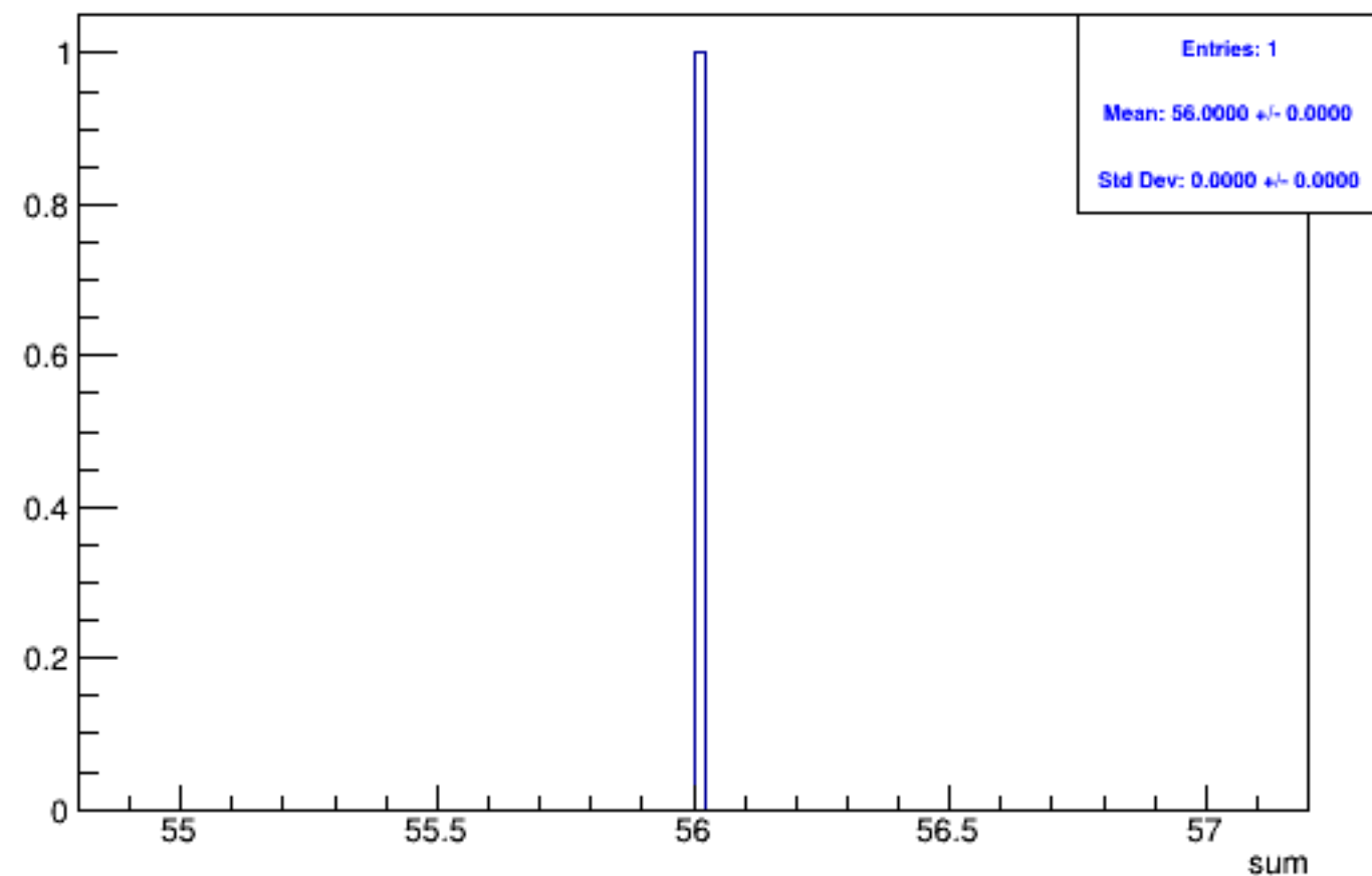
Run 5021 triggerwise, sums: Beam OFF
