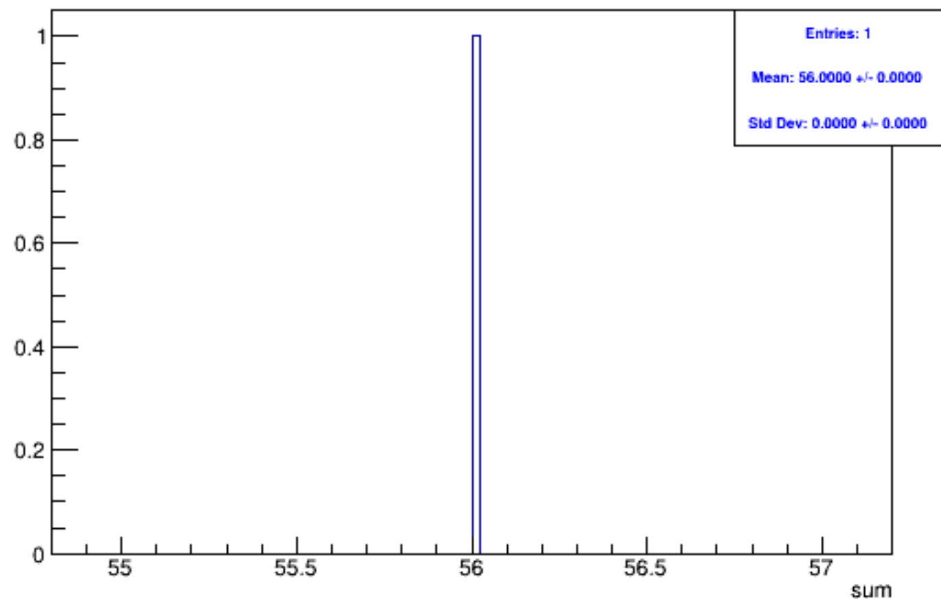
Run 5021 triggerwise, sums: All
