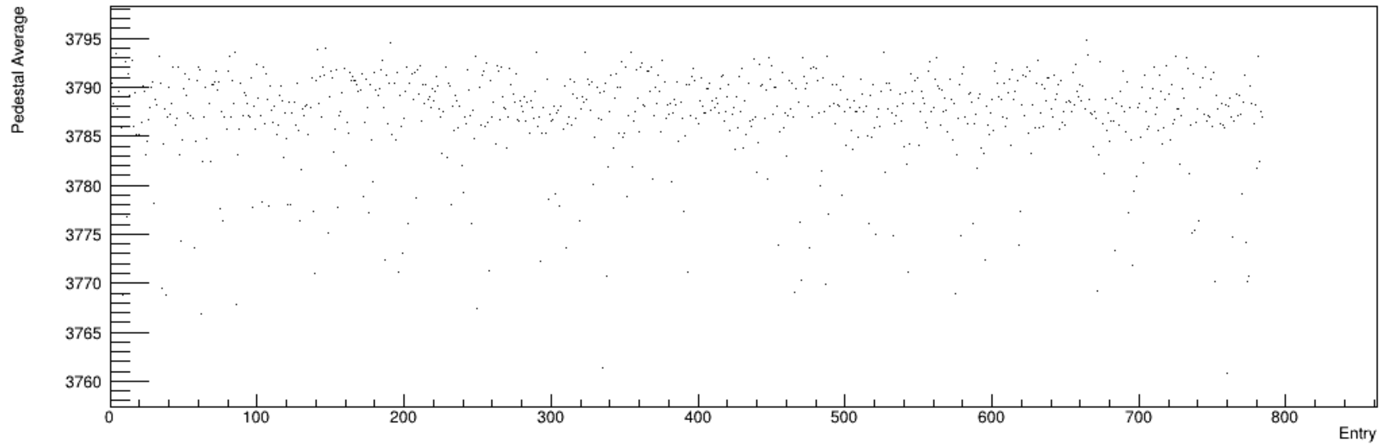
Run 5026, snapshots: Pedestal vs. Time
