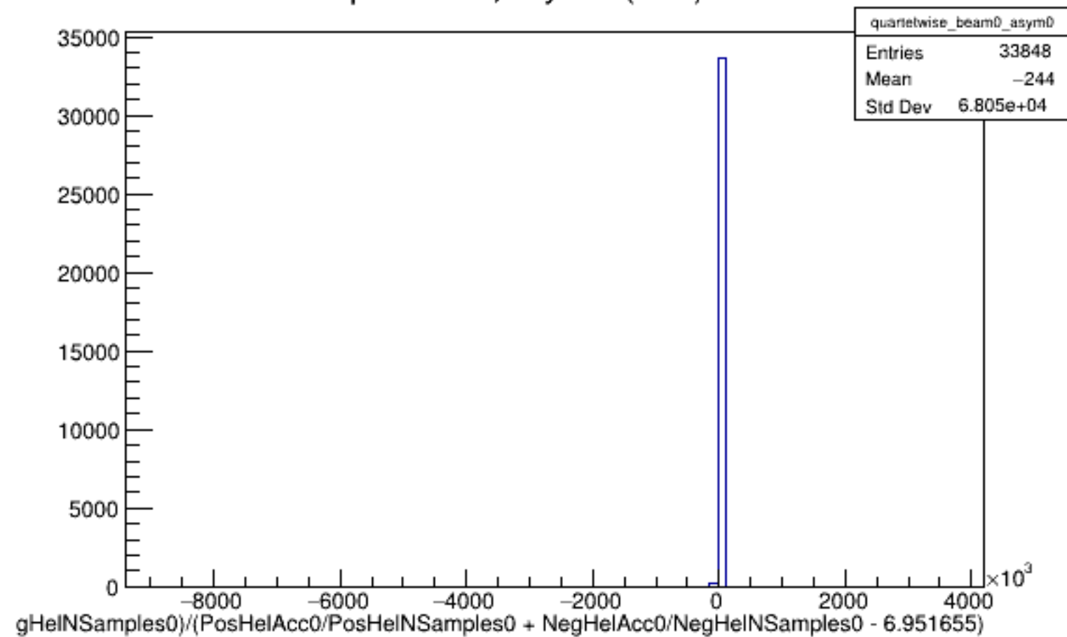
Run 5030 quartetwise, Asyms0 (Raw): Beam OFF
