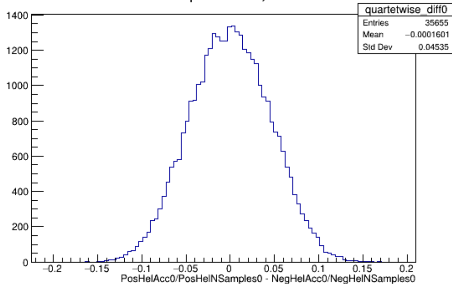
Run 5030 quartetwise, Diffs0: All
