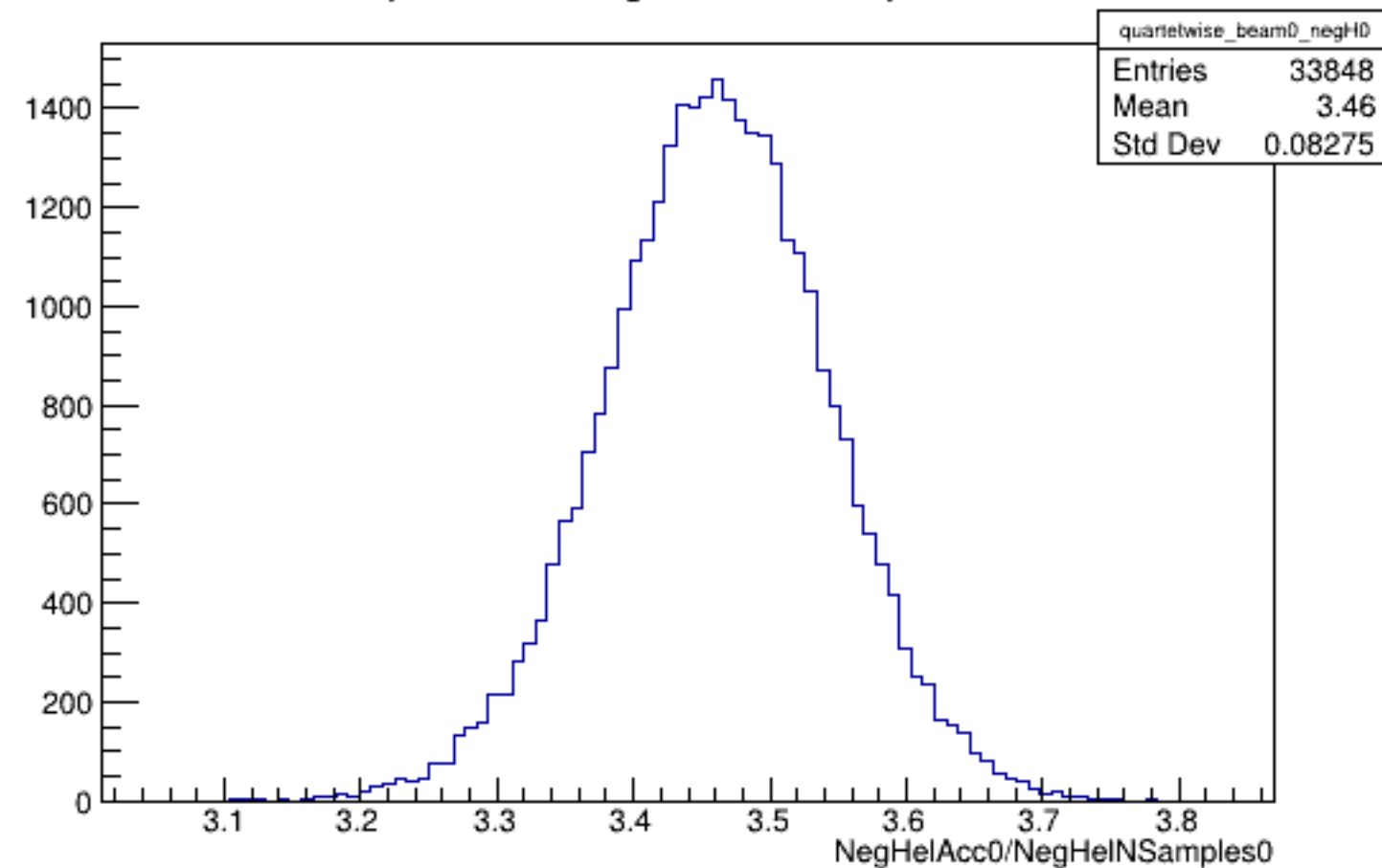
Run 5030 quartetwise, NegHelAcc0/NSamples0: Beam OFF
