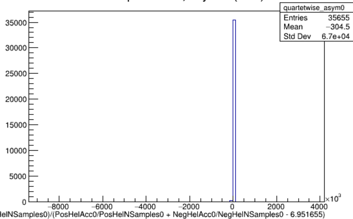
Run 5030 quartetwise, Asyms0 (Raw): All
