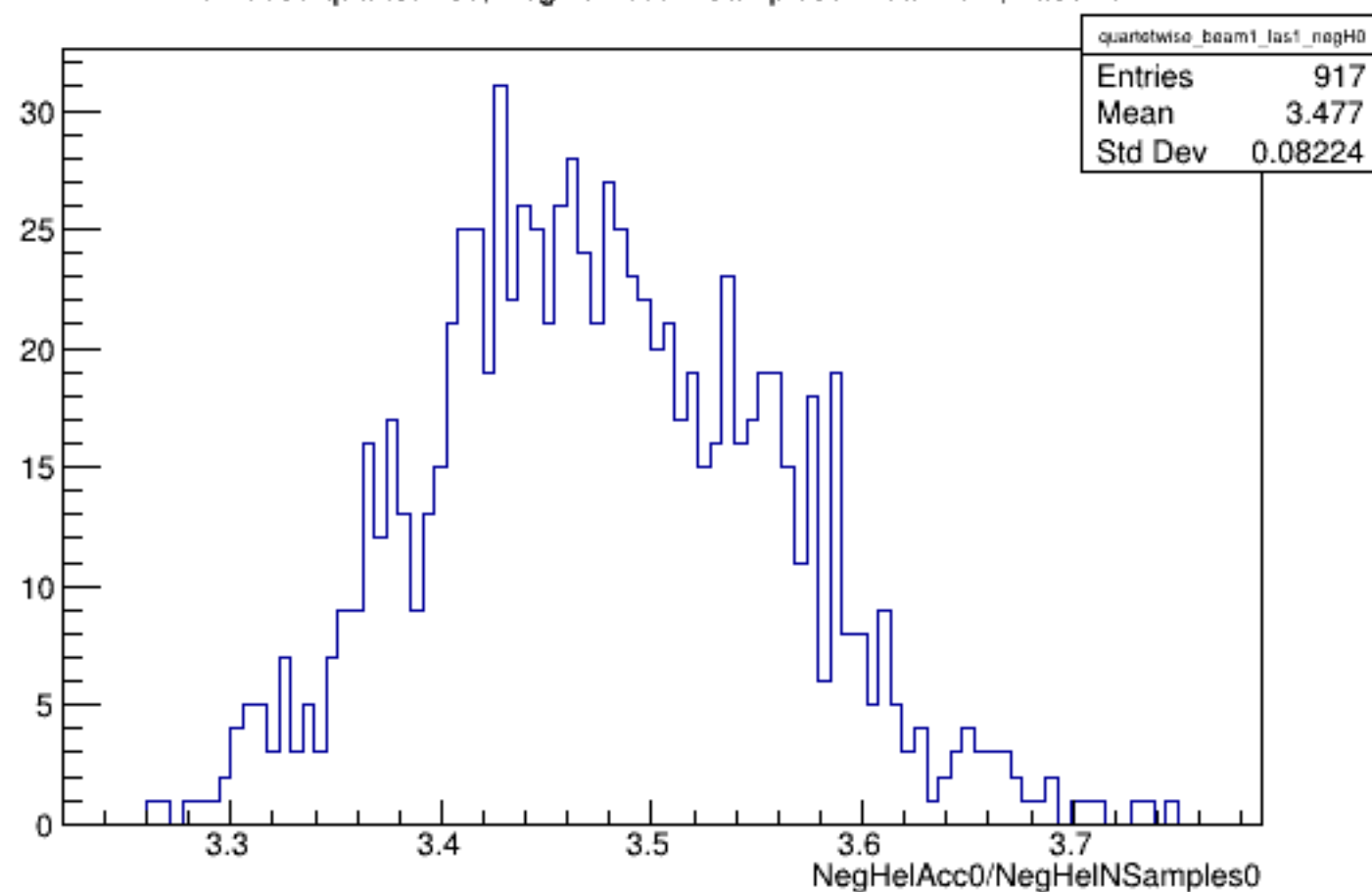
Run 5030 quartetwise, NegHelAcc0/NSamples0: Beam ON, Laser ON
