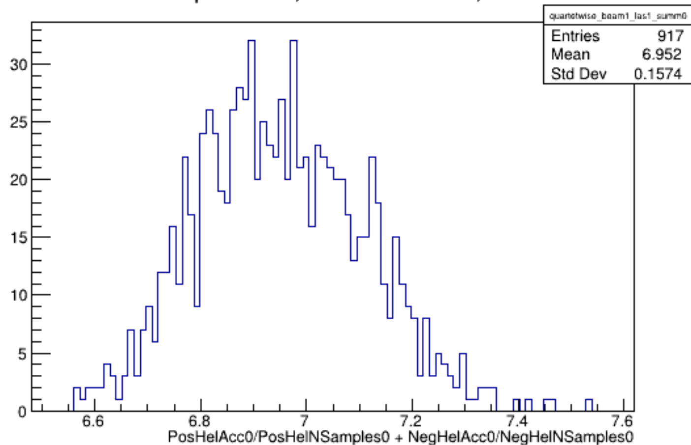
Run 5030 quartetwise, Sums0: Beam ON, Laser ON
