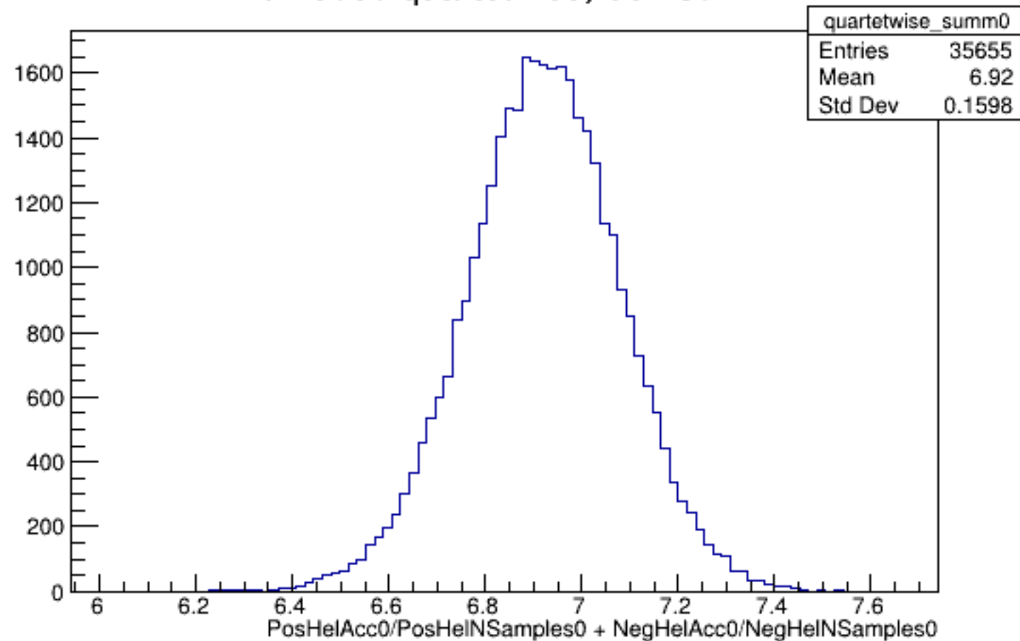
Run 5030 quartetwise, Sums0: All
