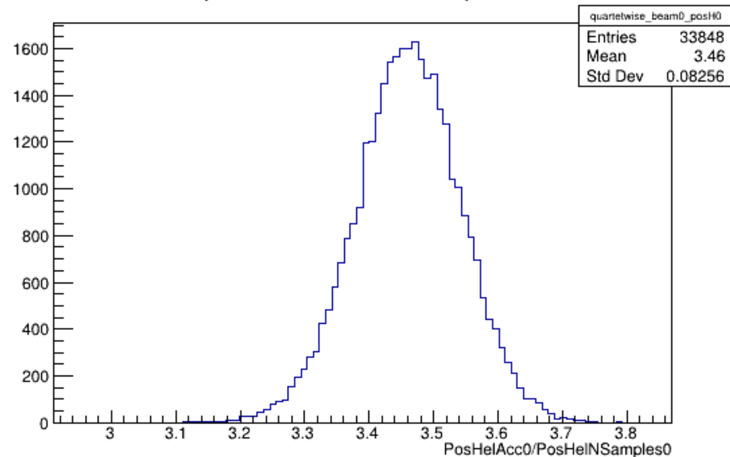
Run 5030 quartetwise, PosHelAcc0/NSamples0: Beam OFF
