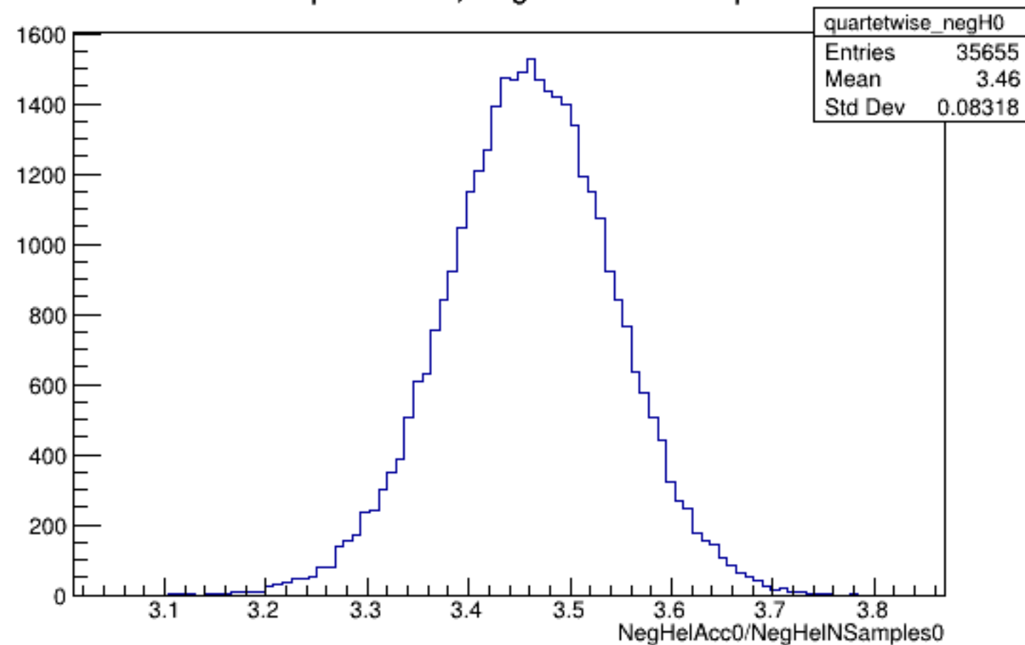
Run 5030 quartetwise, NegHelAcc0/NSamples0: All
