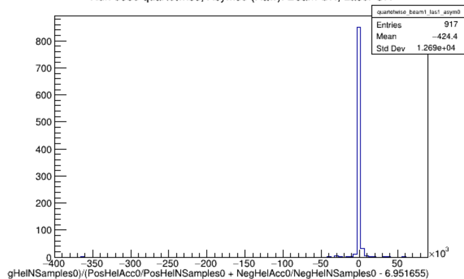
Run 5030 quartetwise, Asyms0 (Raw): Beam ON, Laser ON
