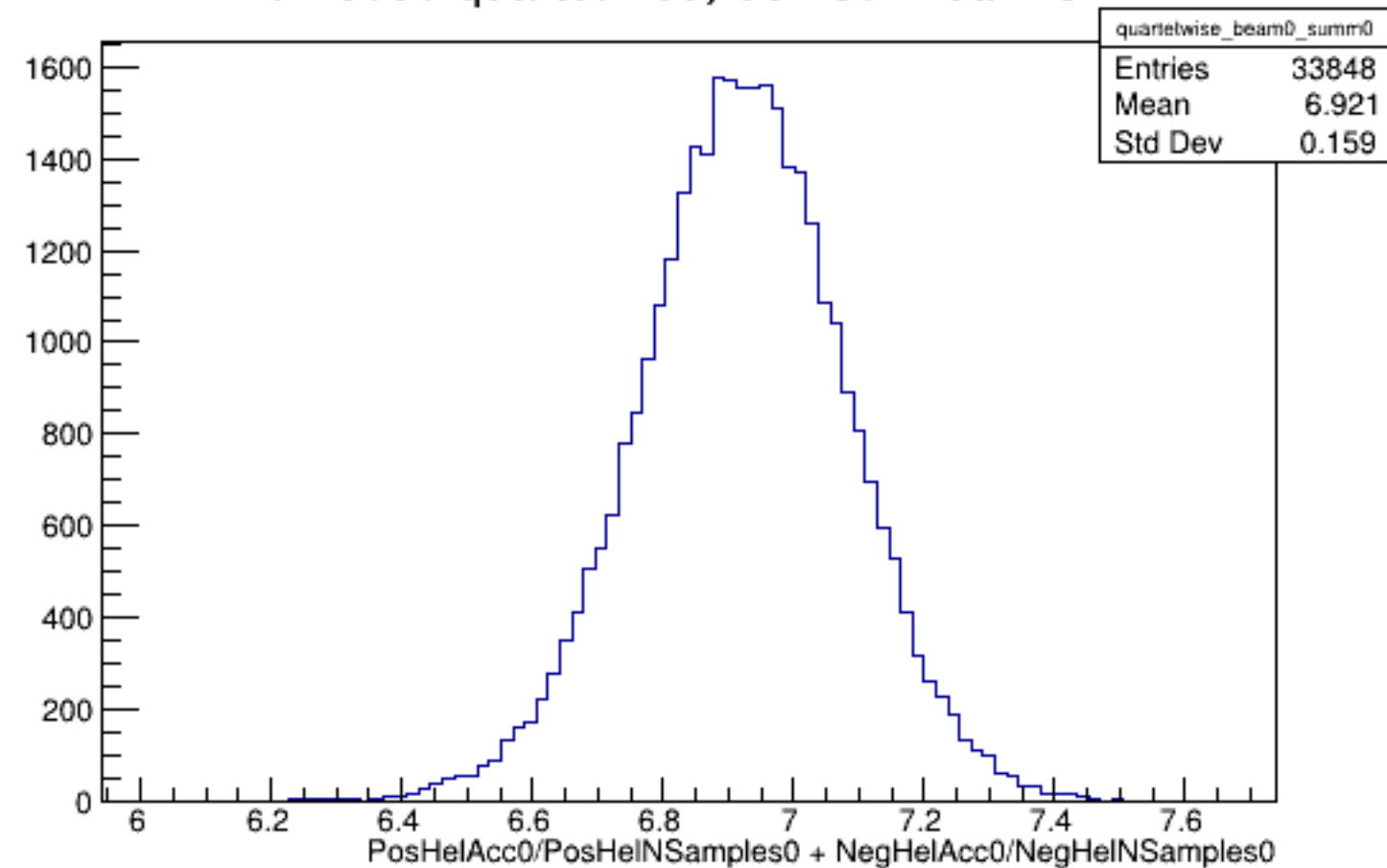
Run 5030 quartetwise, Sums0: Beam OFF
