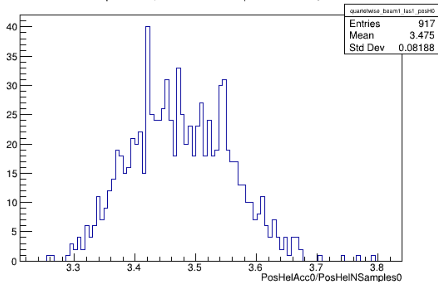
Run 5030 quartetwise, PosHelAcc0/NSamples0: Beam ON, Laser ON
