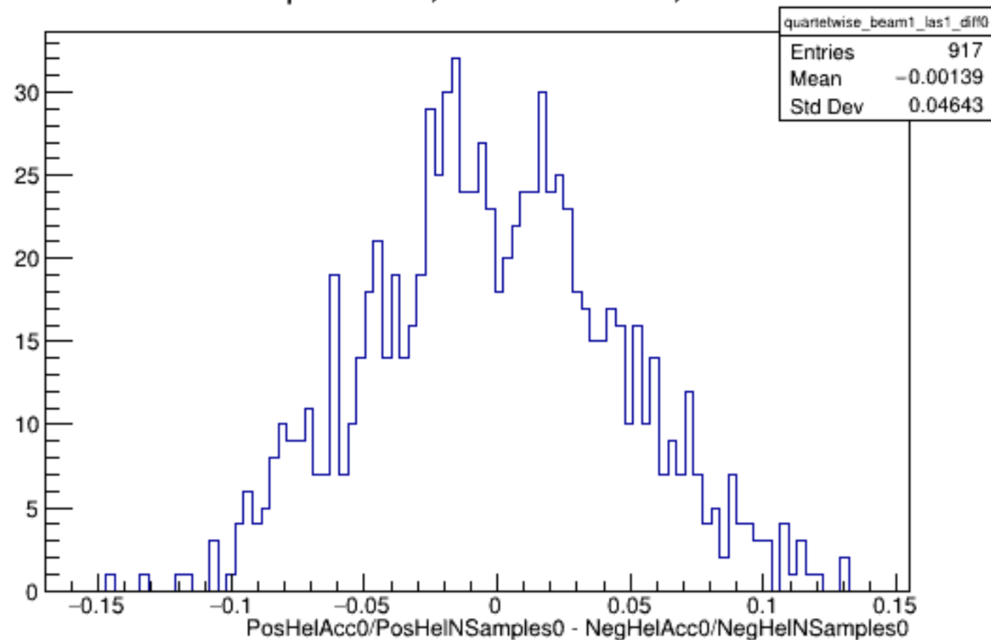
Run 5030 quartetwise, Diffs0: Beam ON, Laser ON
