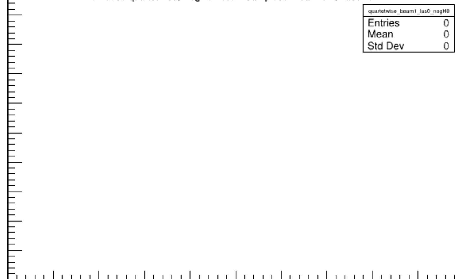
Run 5030 quartetwise, NegHelAcc0/NSamples0: Beam ON, Laser OFF
