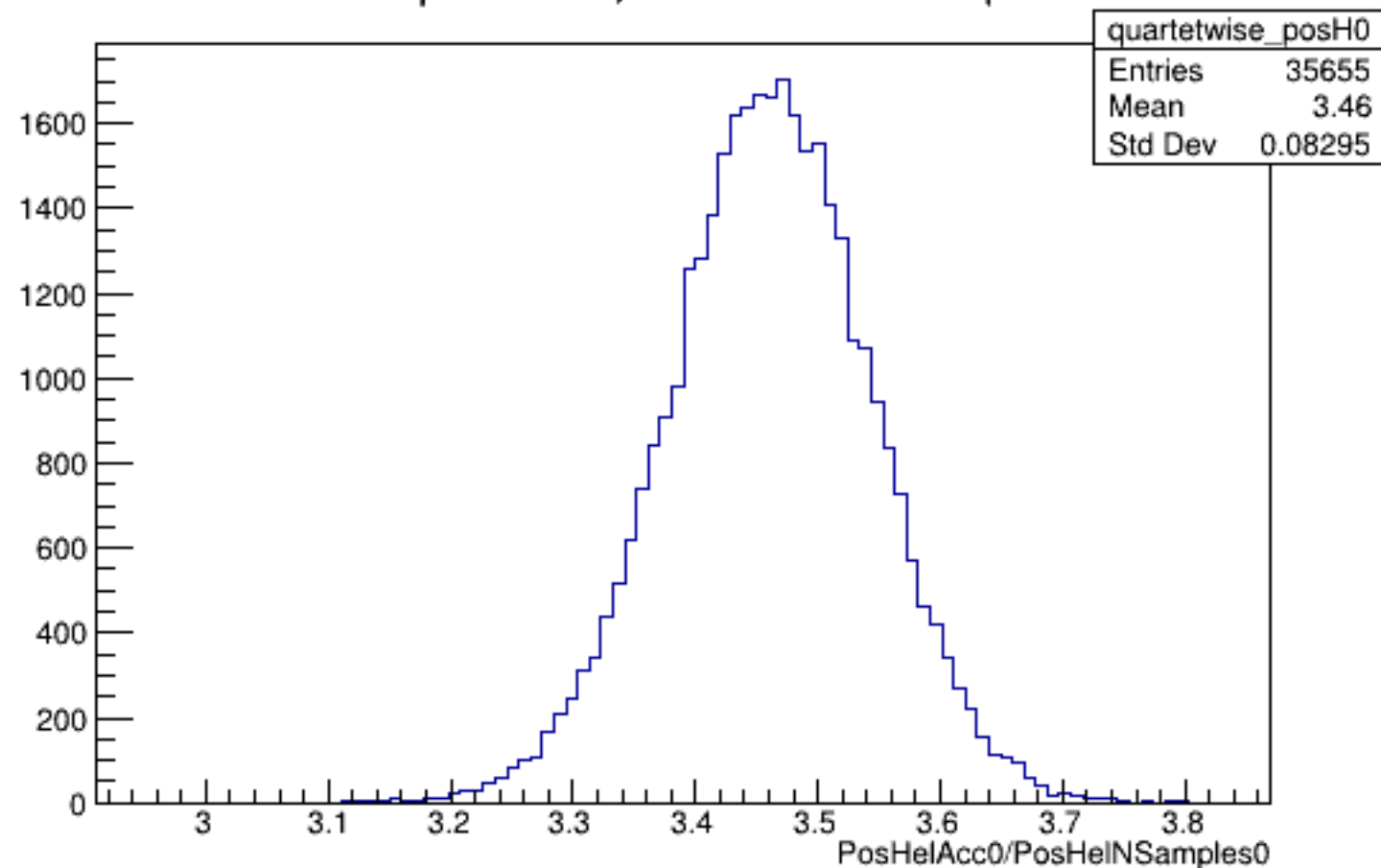
Run 5030 quartetwise, PosHelAcc0/NSamples0: All
