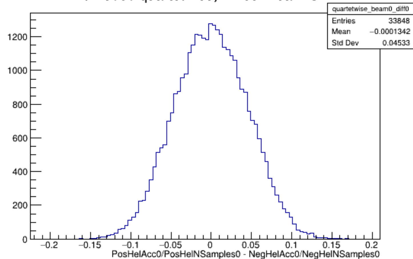
Run 5030 quartetwise, Diffs0: Beam OFF
