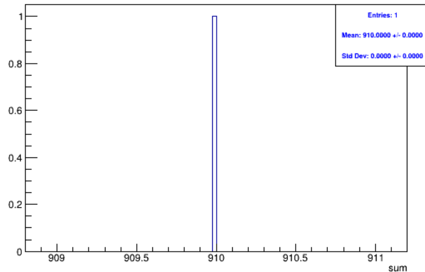
Run 5030 triggerwise, sums: Beam OFF
