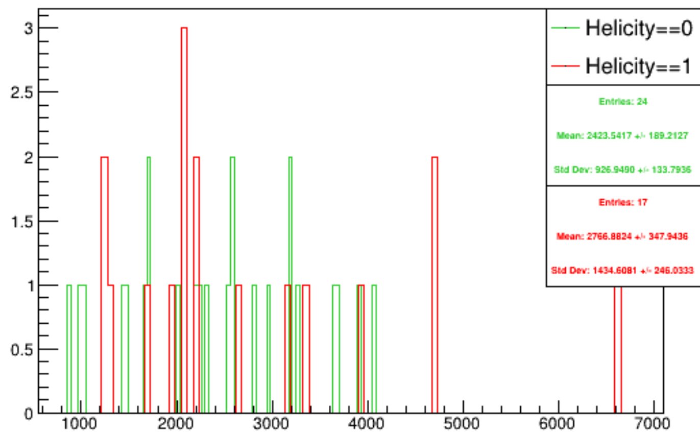
Run 5030 triggerwise, sums: Beam ON, Laser ON
