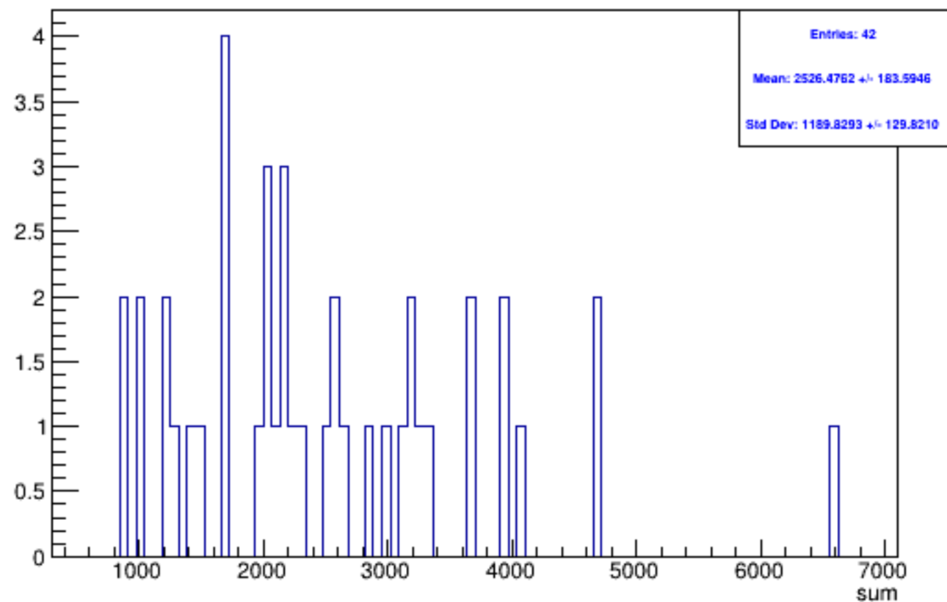
Run 5030 triggerwise, sums: All
