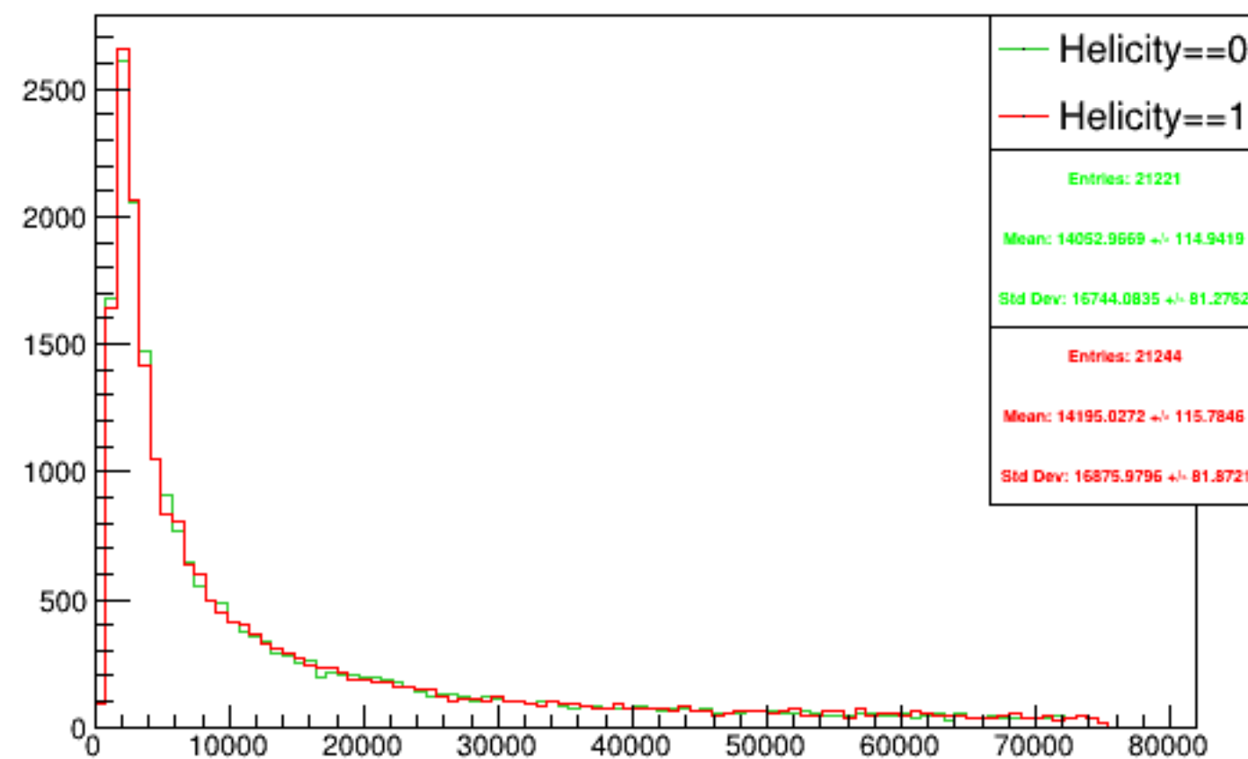
Run 5032 triggerwise, sums: Beam ON, Laser OFF
