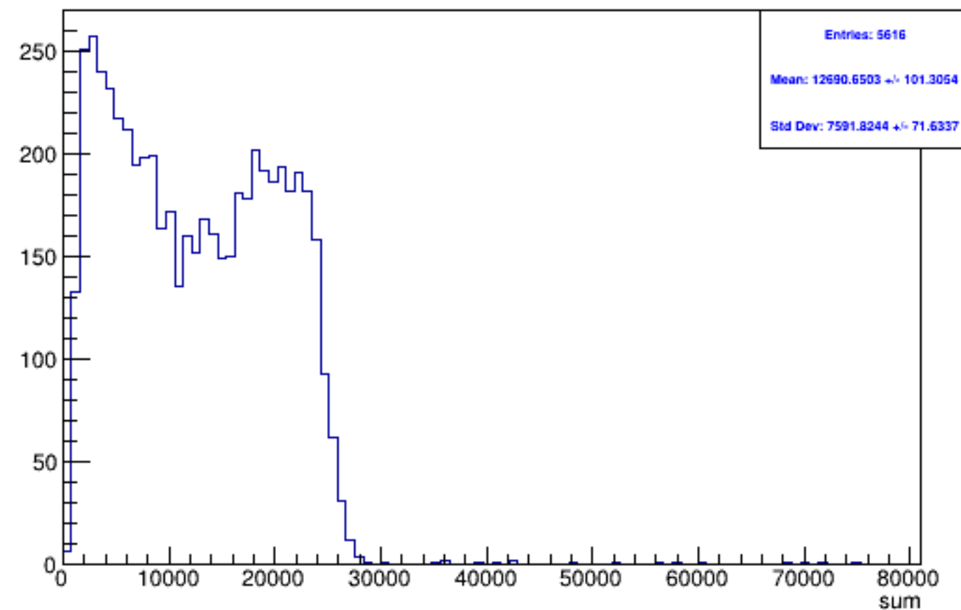
Run 5032 triggerwise, sums: Beam OFF
