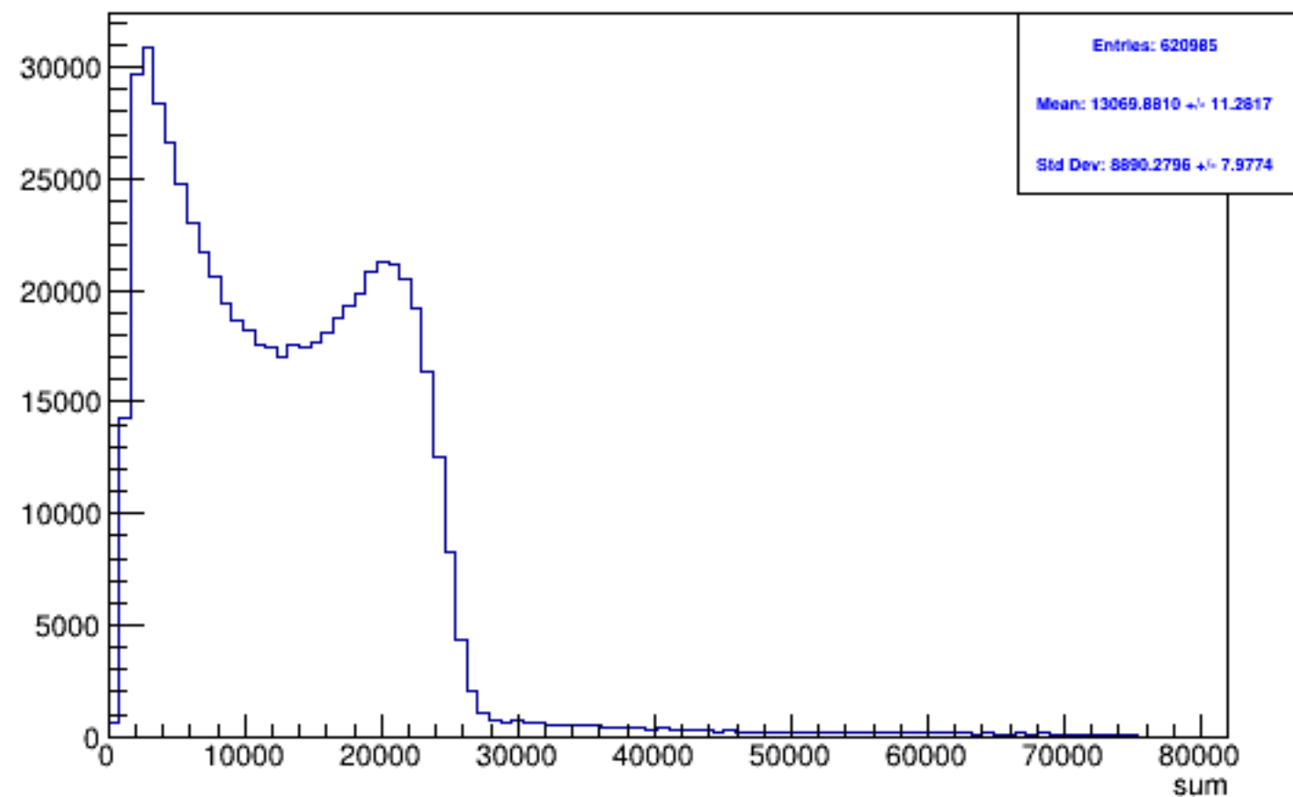
Run 5032 triggerwise, sums: All
