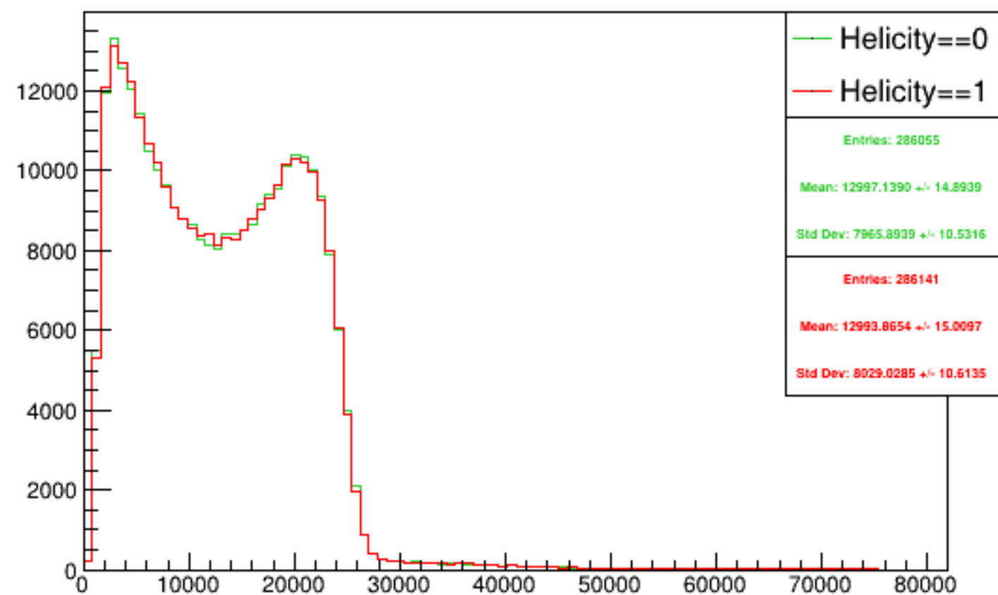
Run 5032 triggerwise, sums: Beam ON, Laser ON
