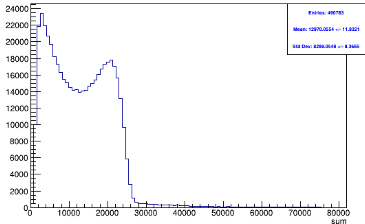
Run 5034 triggerwise, sums: All
