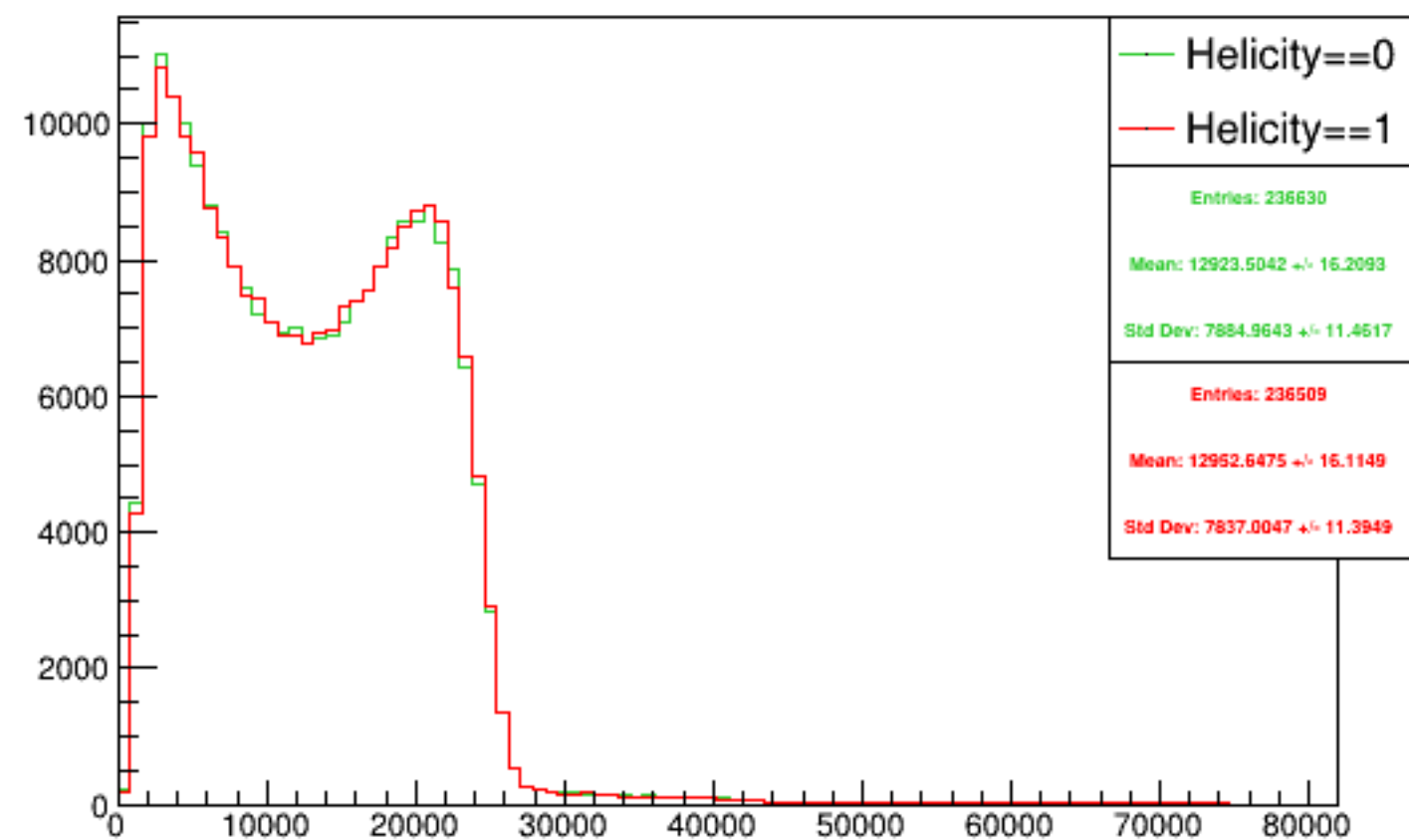
Run 5034 triggerwise, sums: Beam ON, Laser ON
