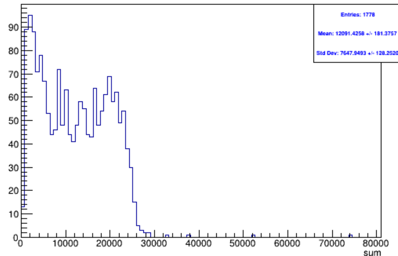
Run 5034 triggerwise, sums: Beam OFF
