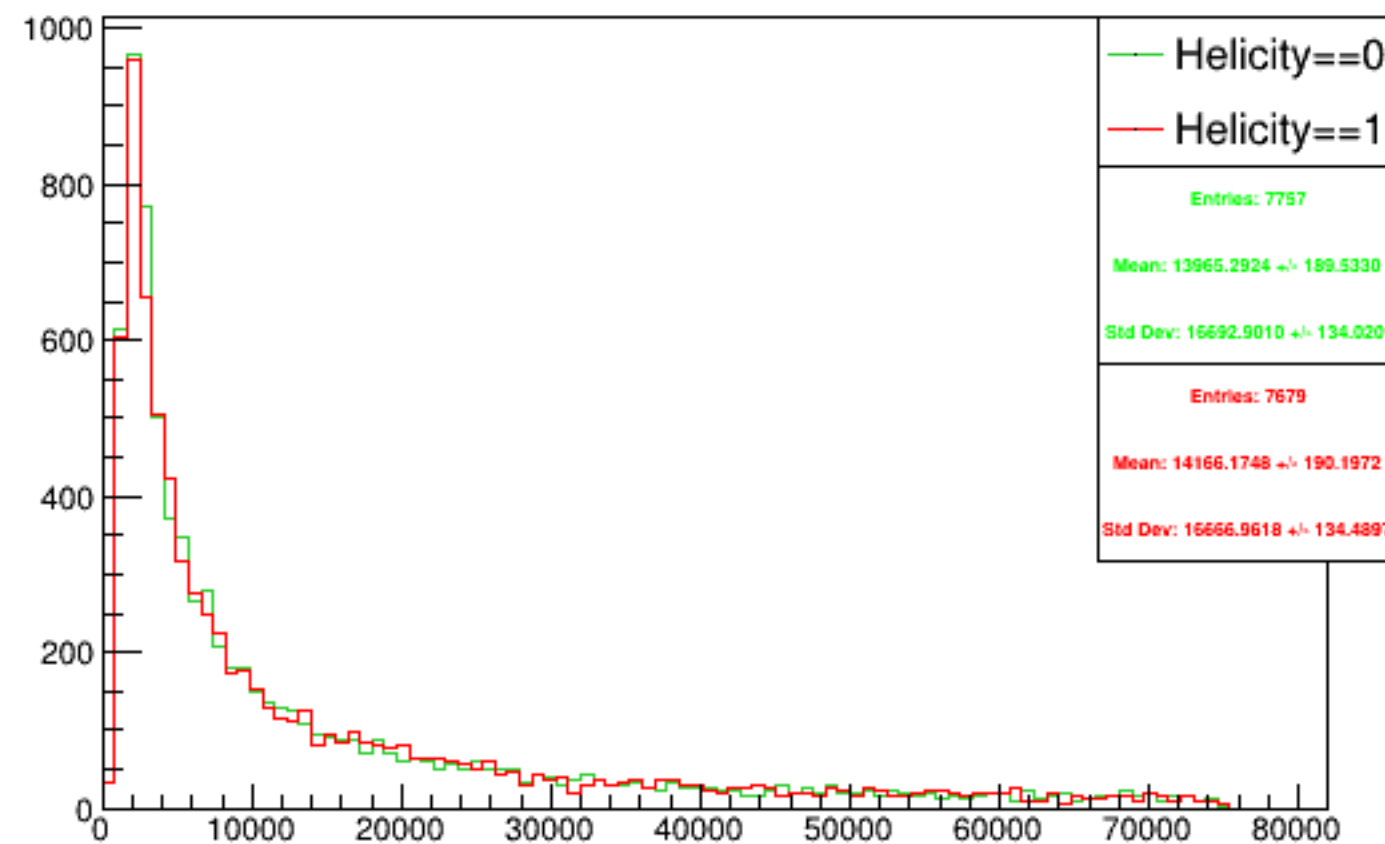
Run 5034 triggerwise, sums: Beam ON, Laser OFF
