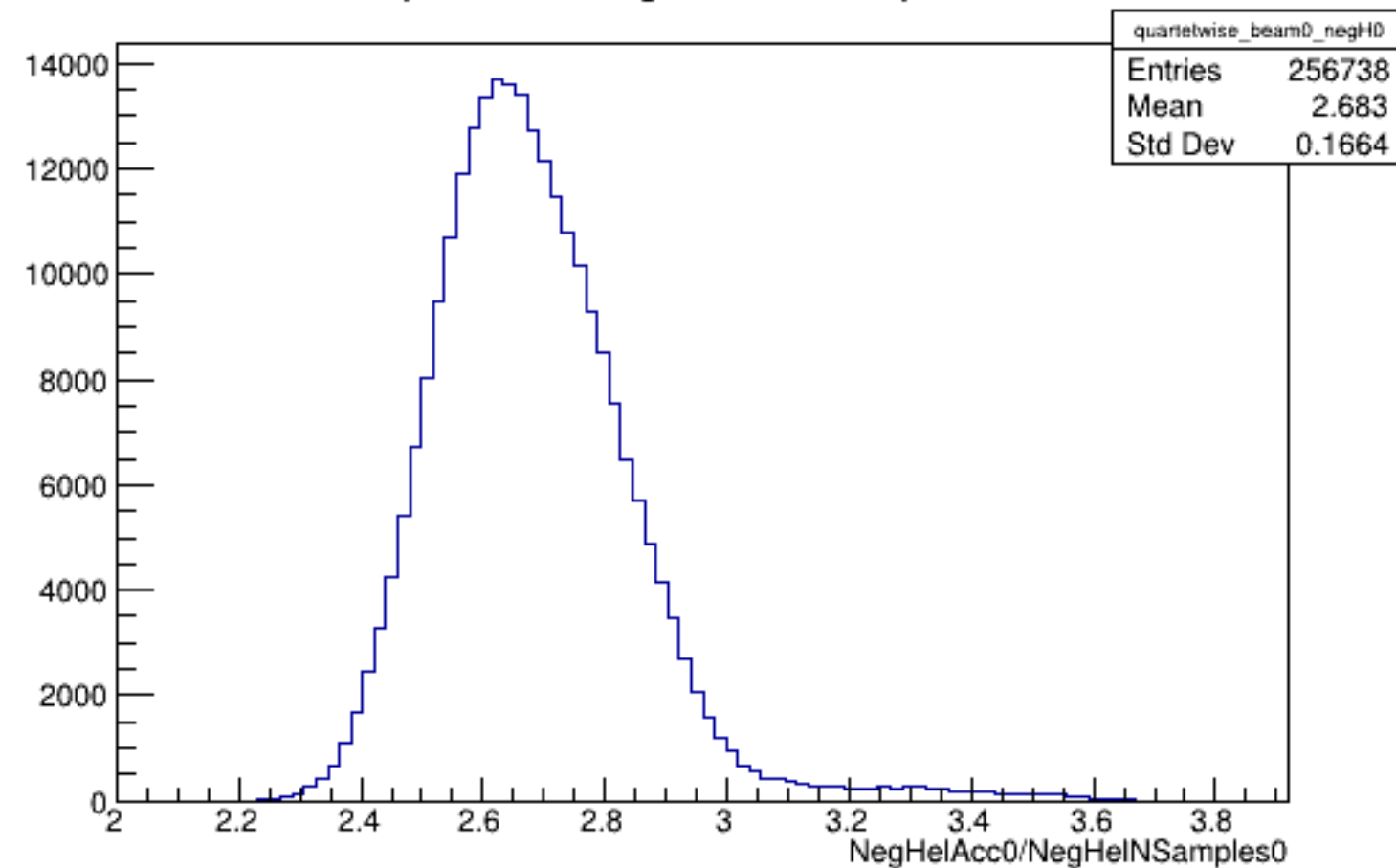
Run 5038 quartetwise, NegHelAcc0/NSamples0: Beam OFF
