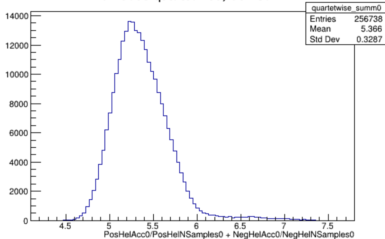
Run 5038 quartetwise, Sums0: All
