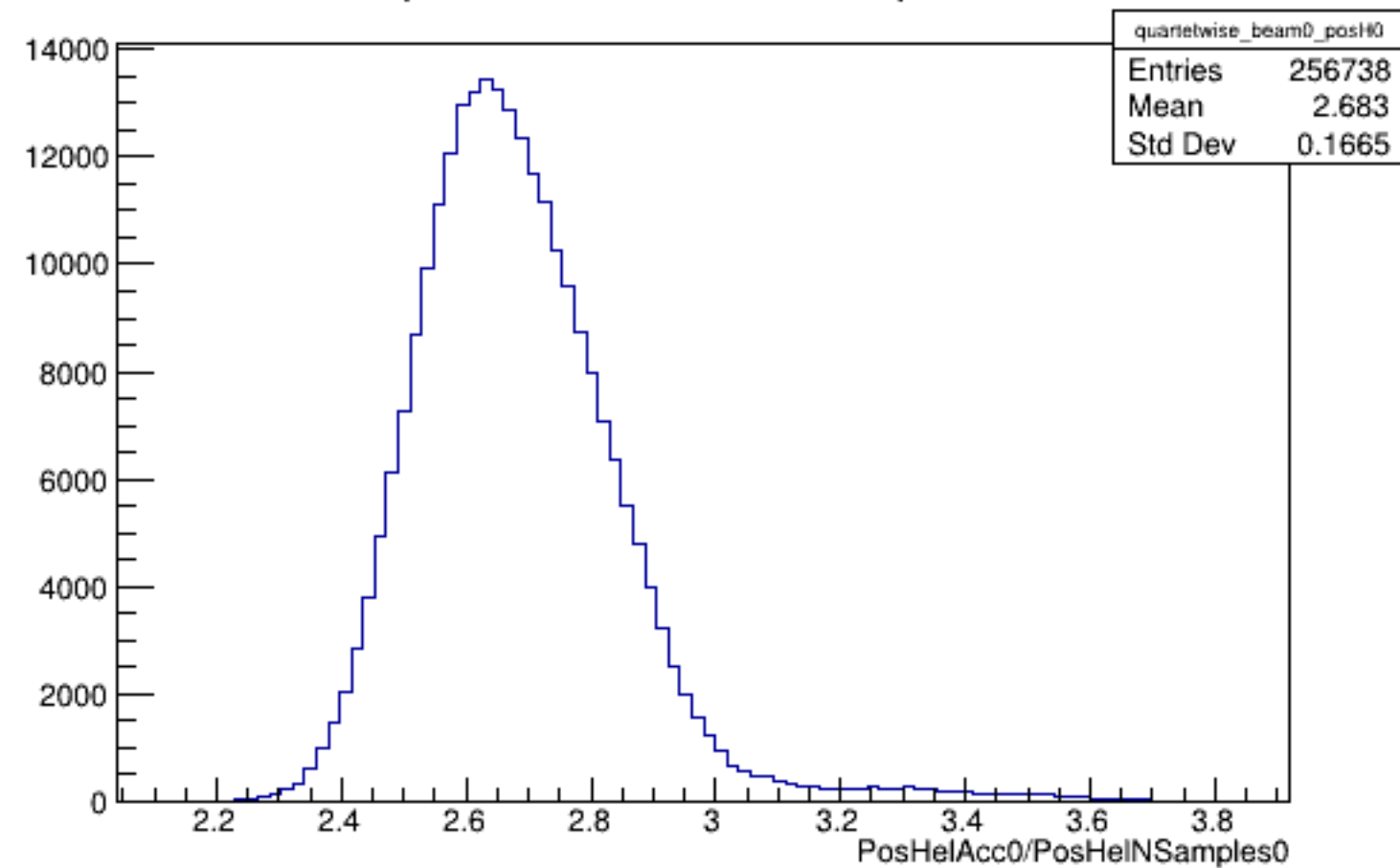
Run 5038 quartetwise, PosHelAcc0/NSamples0: Beam OFF
