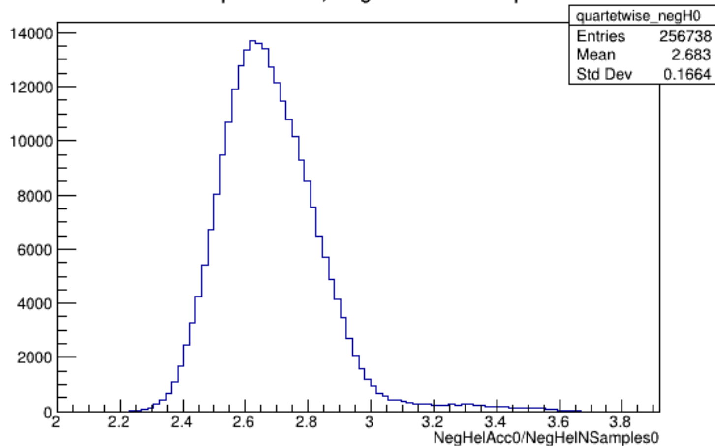
Run 5038 quartetwise, NegHelAcc0/NSamples0: All
