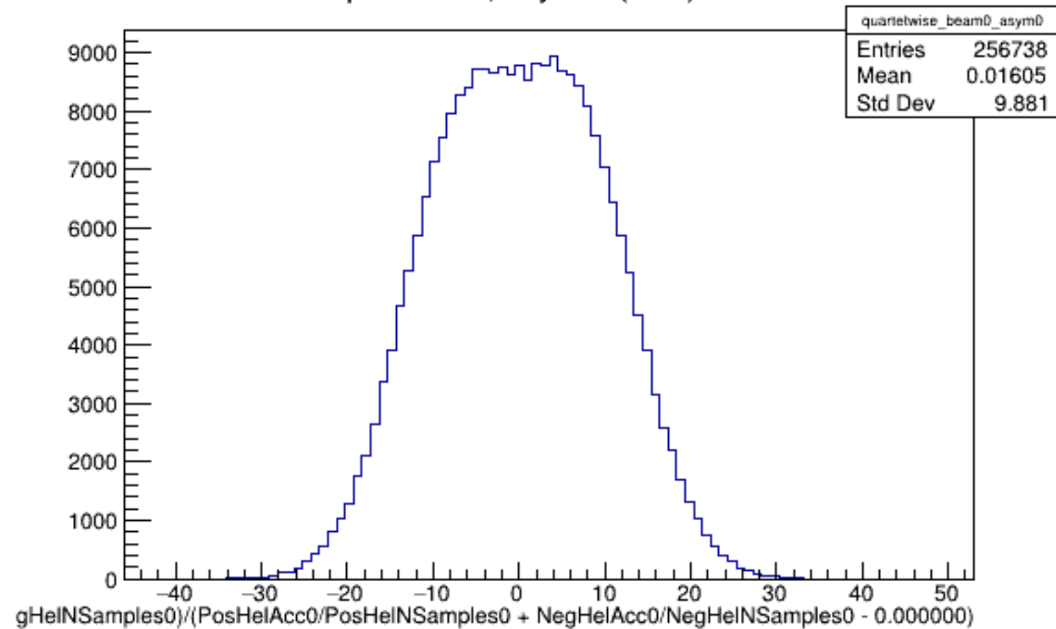
Run 5038 quartetwise, Asyms0 (Raw): Beam OFF
