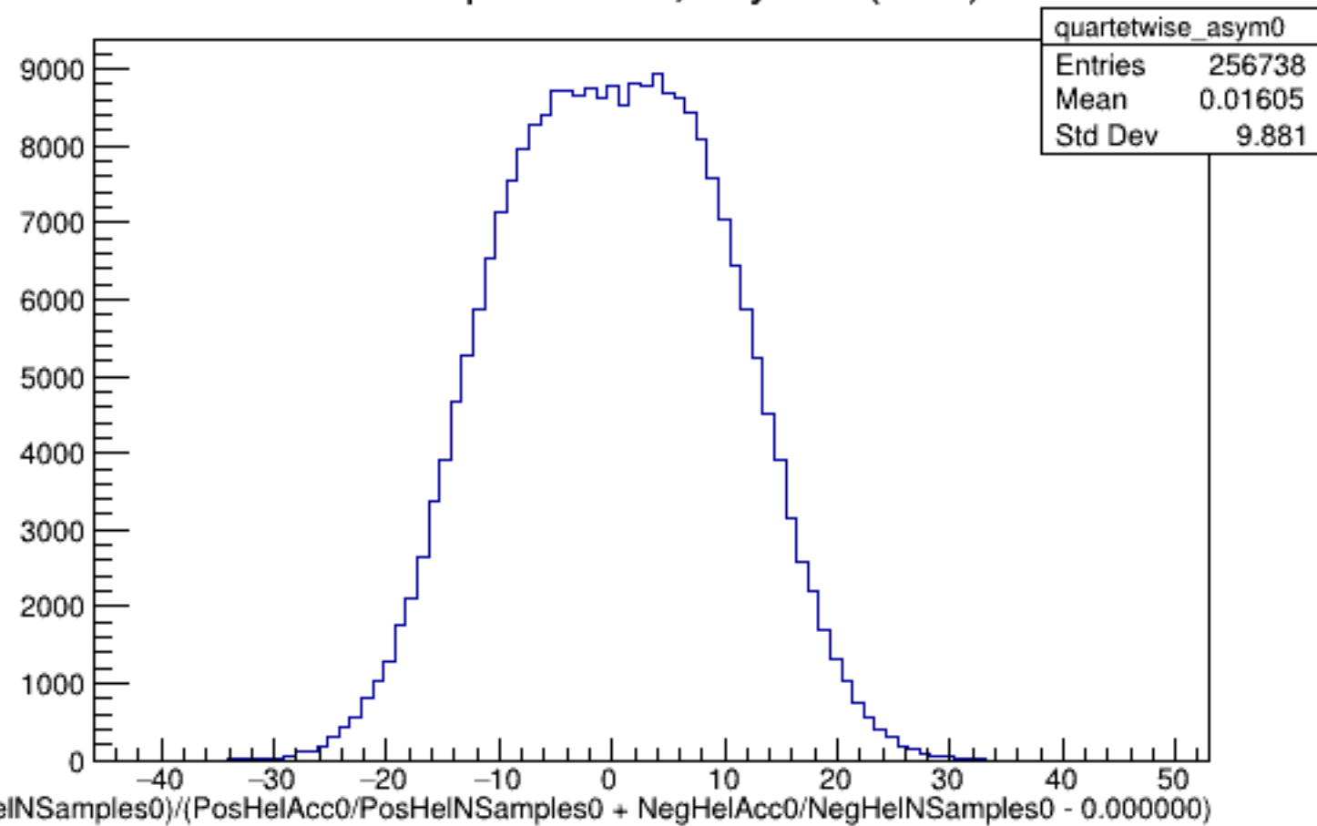
Run 5038 quartetwise, Asyms0 (Raw): All
