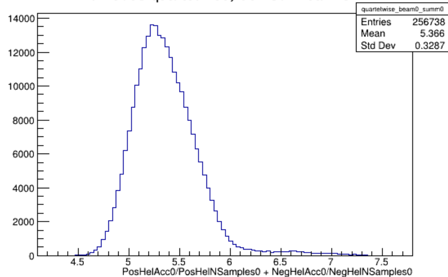
Run 5038 quartetwise, Sums0: Beam OFF
