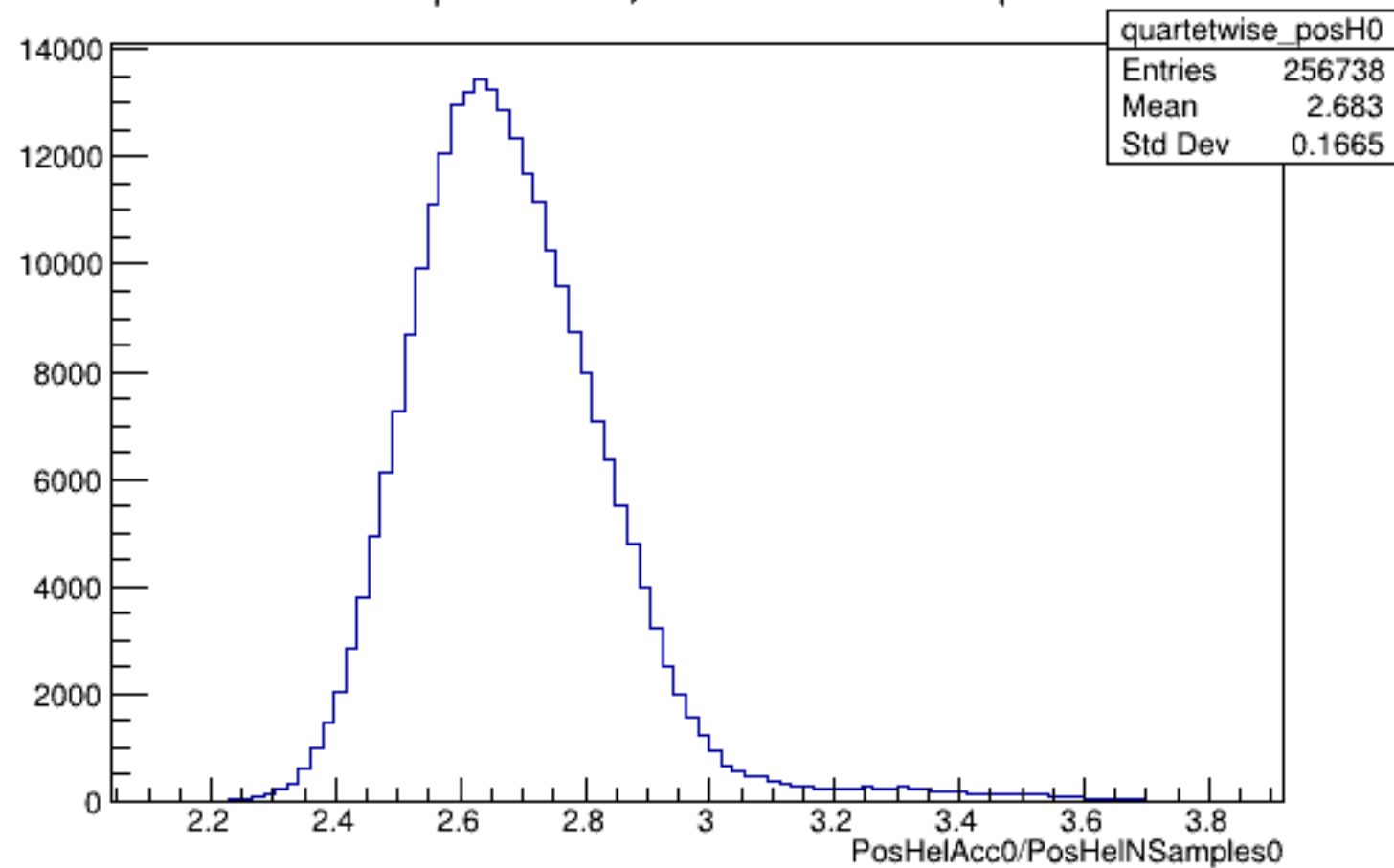
Run 5038 quartetwise, PosHelAcc0/NSamples0: All
