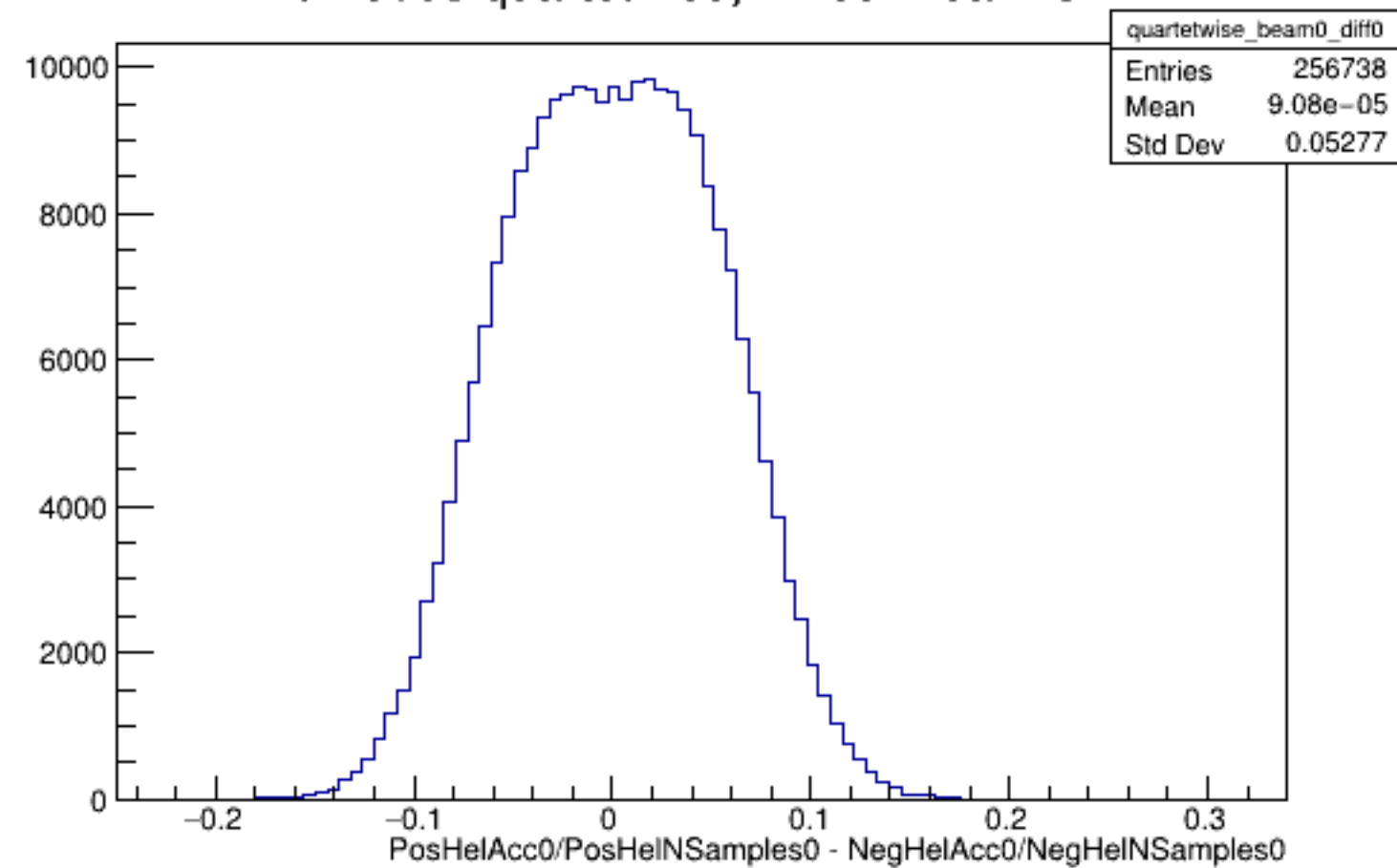
Run 5038 quartetwise, Diffs0: Beam OFF
