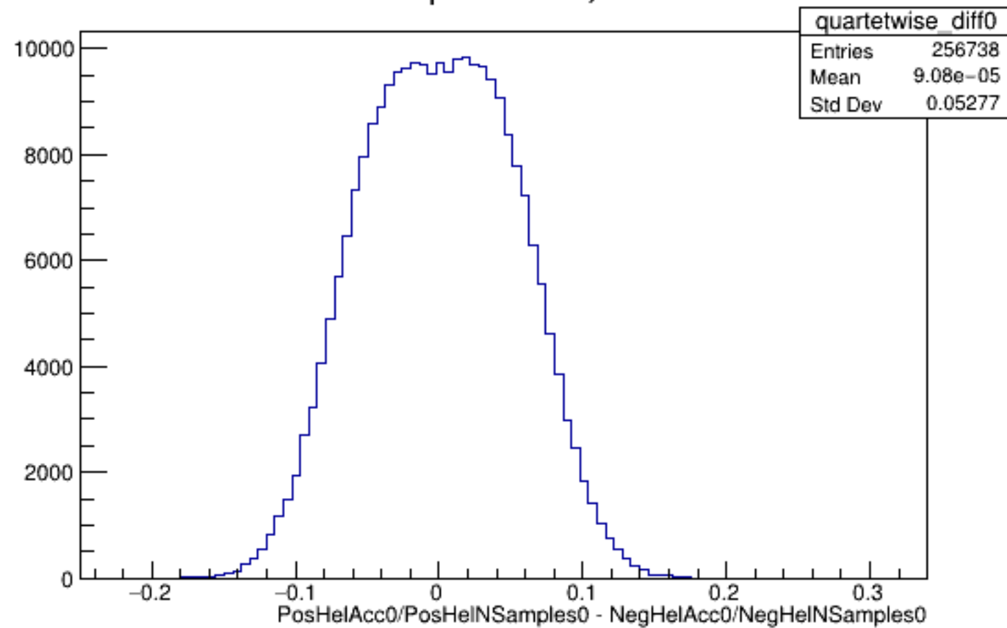
Run 5038 quartetwise, Diffs0: All
