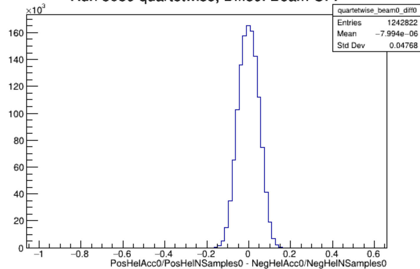
Run 5039 quartetwise, Diffs0: Beam OFF
