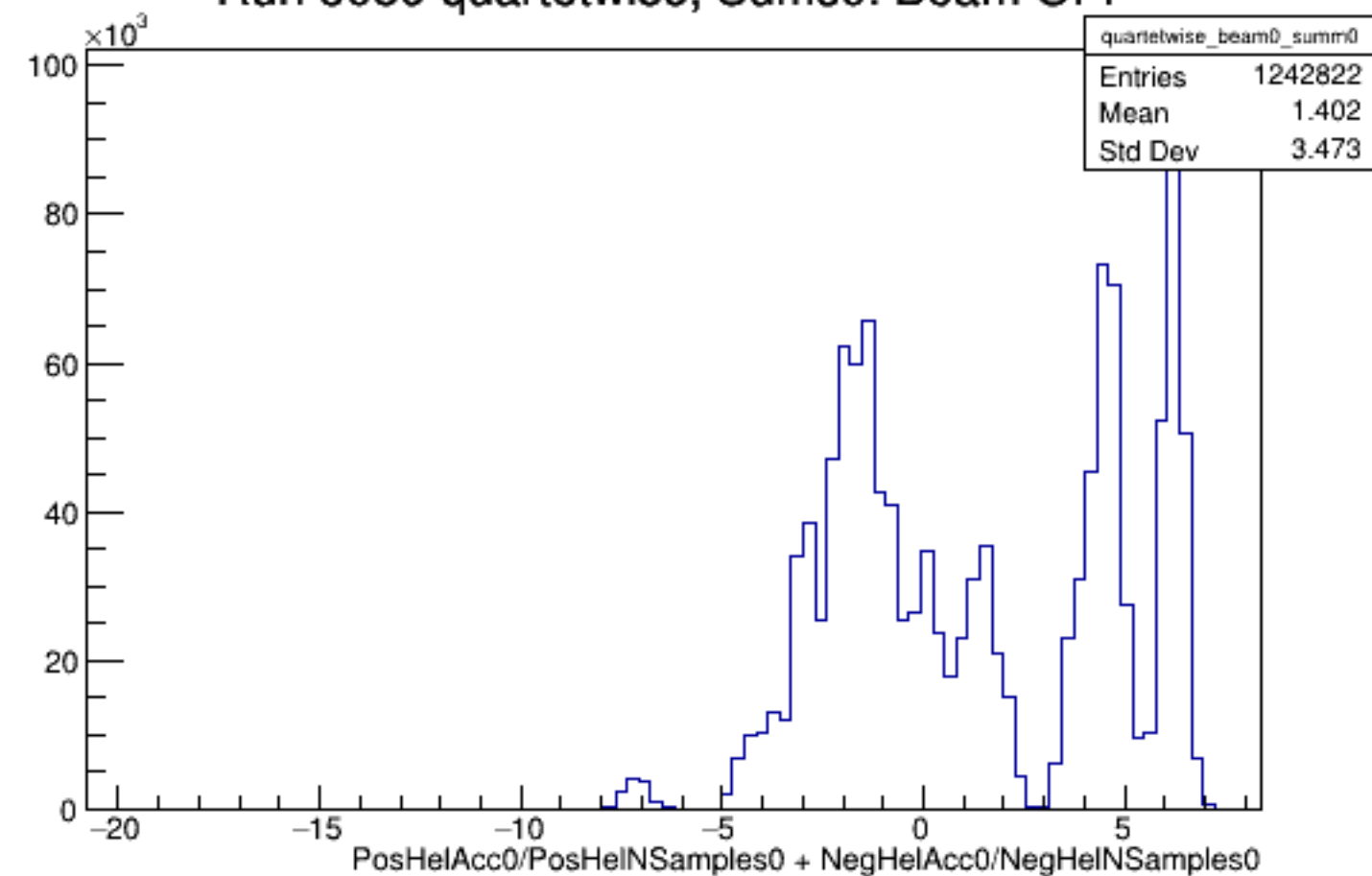
Run 5039 quartetwise, Sums0: Beam OFF
