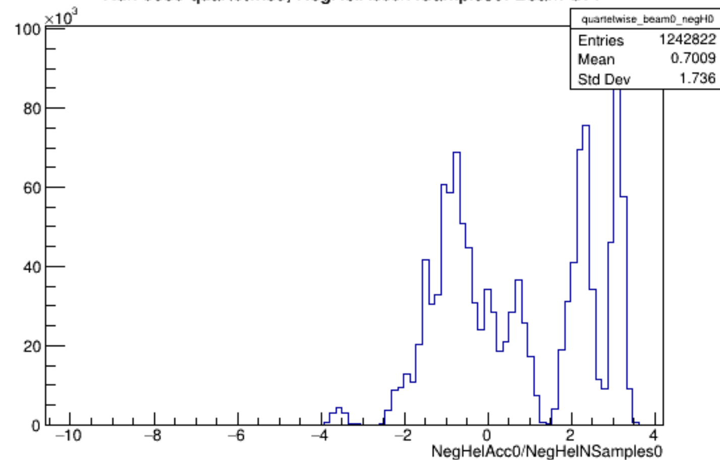
Run 5039 quartetwise, NegHelAcc0/NSamples0: Beam OFF
