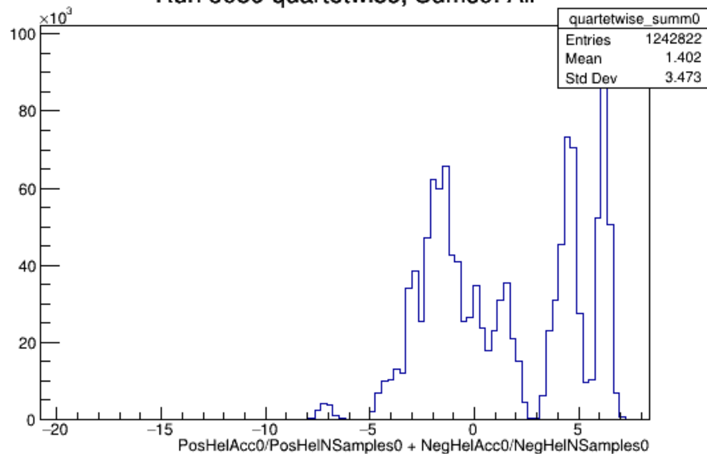
Run 5039 quartetwise, Sums0: All
