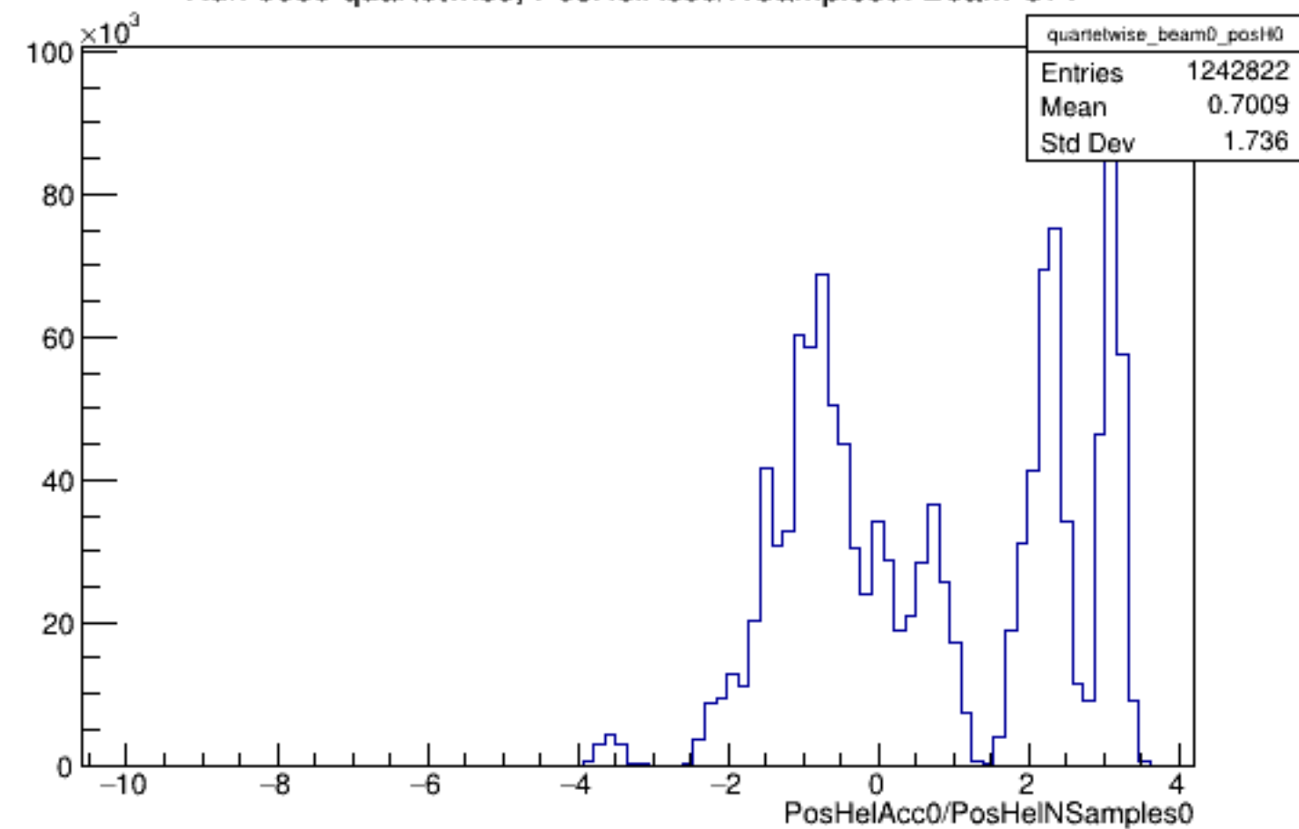
Run 5039 quartetwise, PosHelAcc0/NSamples0: Beam OFF
