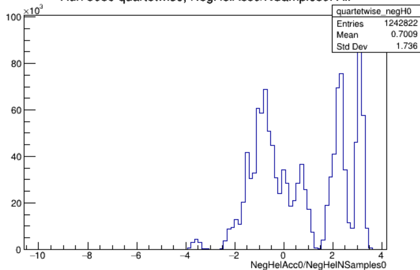
Run 5039 quartetwise, NegHelAcc0/NSamples0: All
