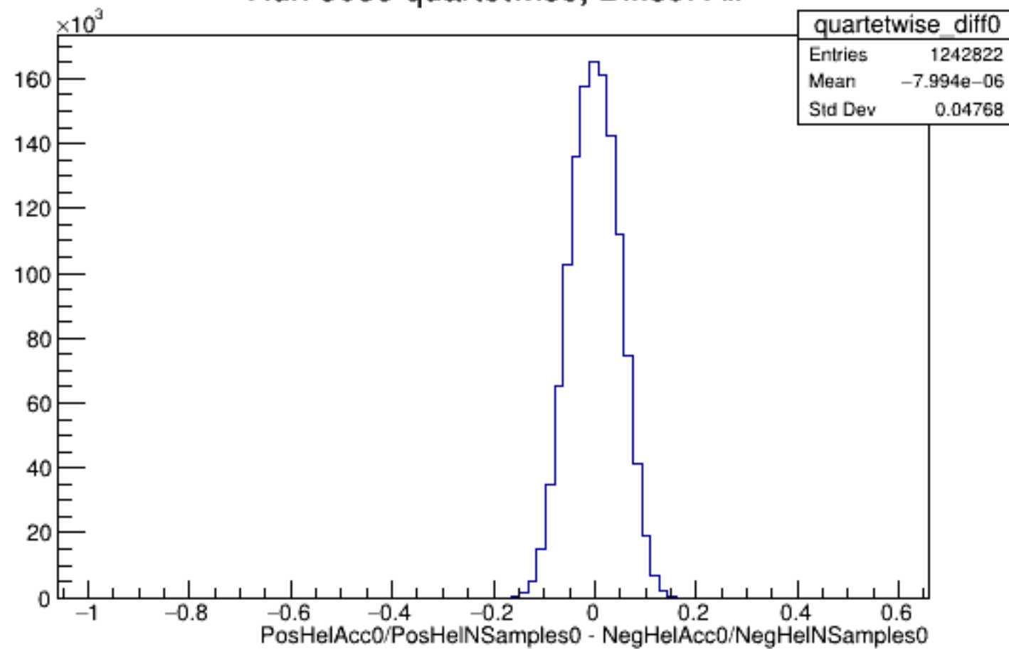
Run 5039 quartetwise, Diffs0: All
