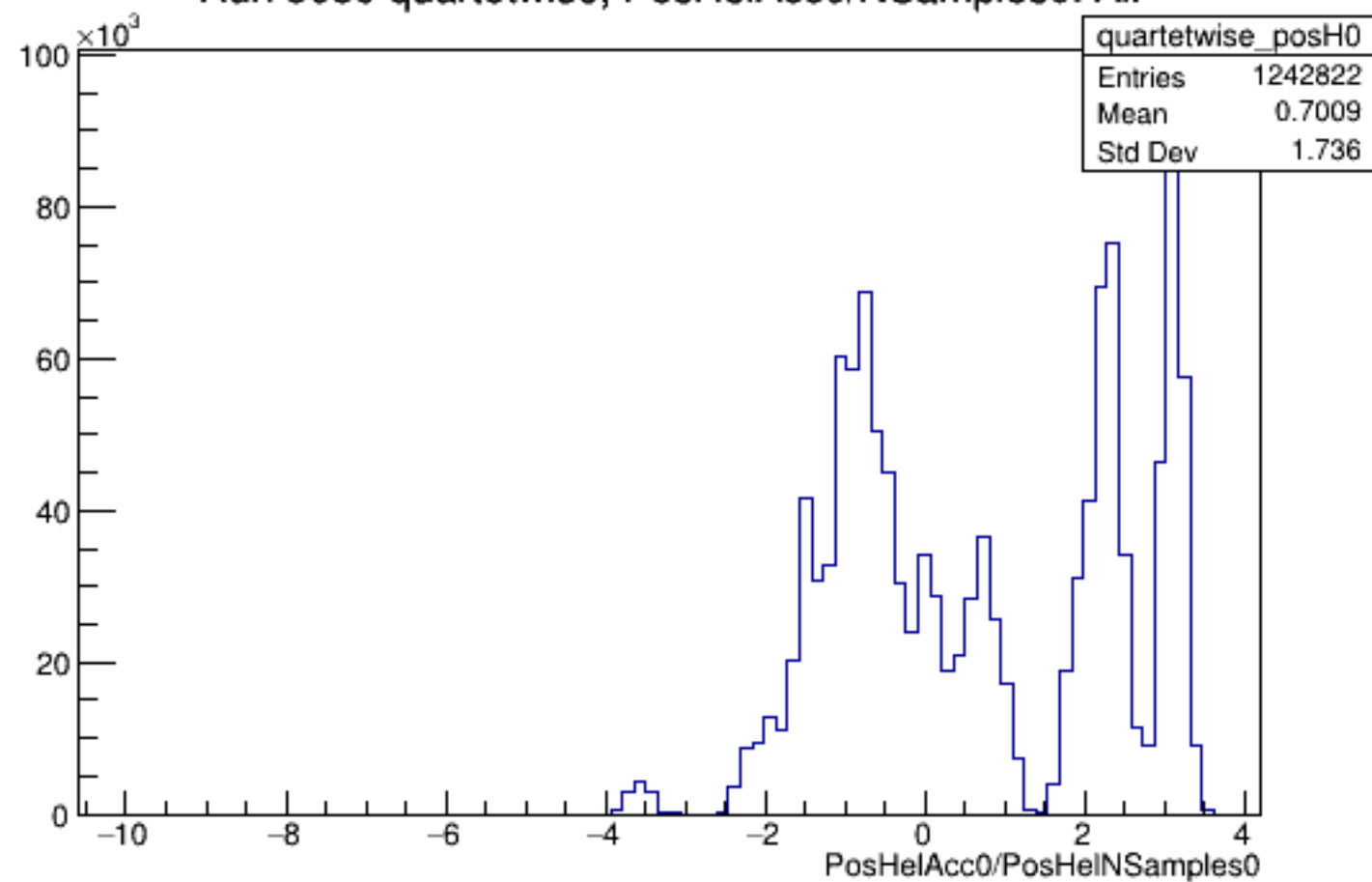
Run 5039 quartetwise, PosHelAcc0/NSamples0: All
