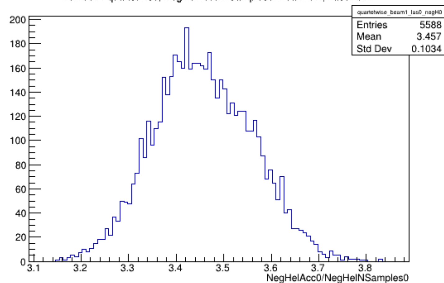
Run 5044 quartetwise, NegHelAcc0/NSamples0: Beam ON, Laser OFF
