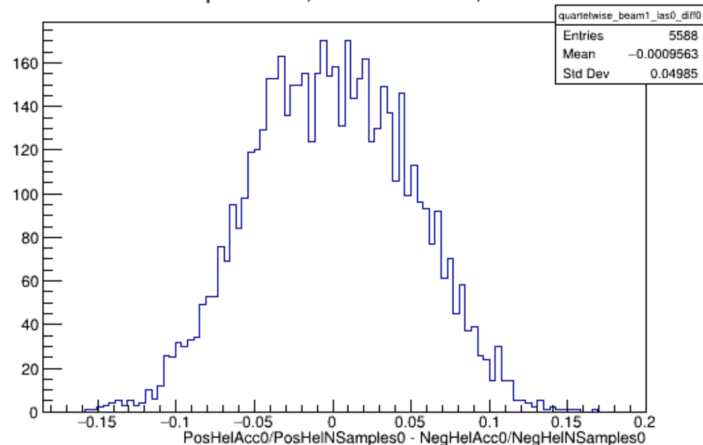
Run 5044 quartetwise, Diffs0: Beam ON, Laser OFF
