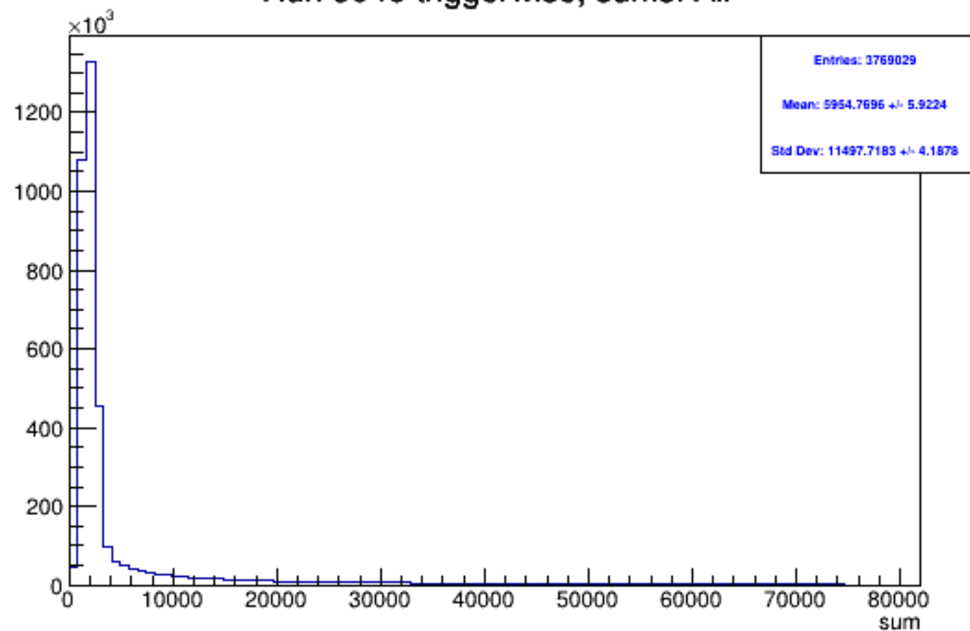
Run 5046 triggerwise, sums: All
