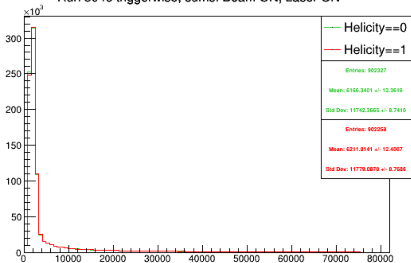
Run 5046 triggerwise, sums: Beam ON, Laser ON
