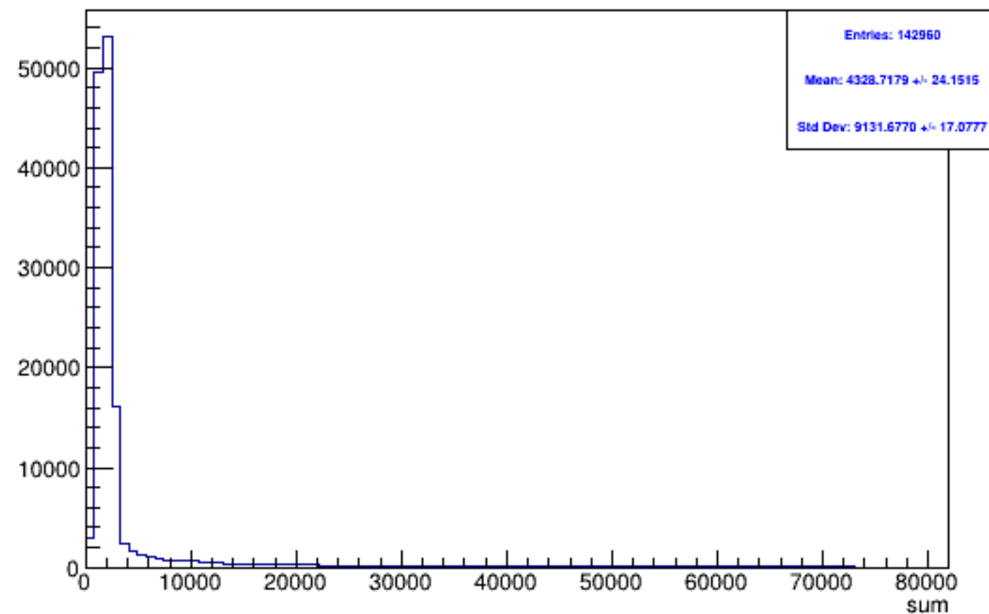
Run 5046 triggerwise, sums: Beam OFF
