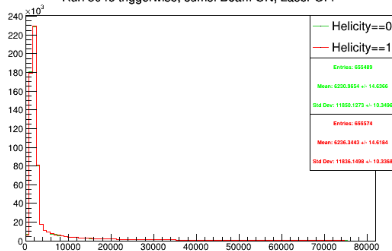
Run 5046 triggerwise, sums: Beam ON, Laser OFF
