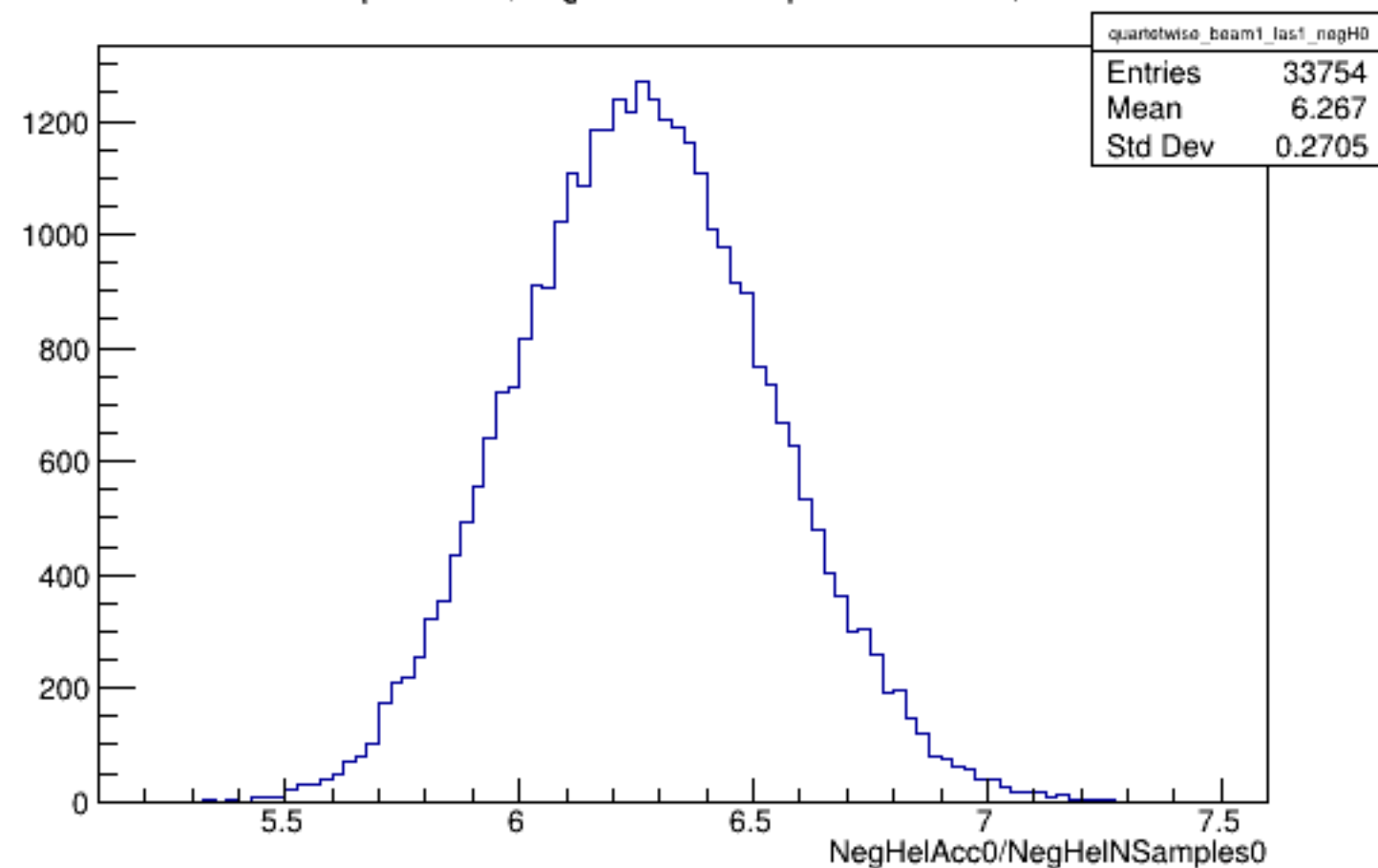
Run 5047 quartetwise, NegHelAcc0/NSamples0: Beam ON, Laser ON
