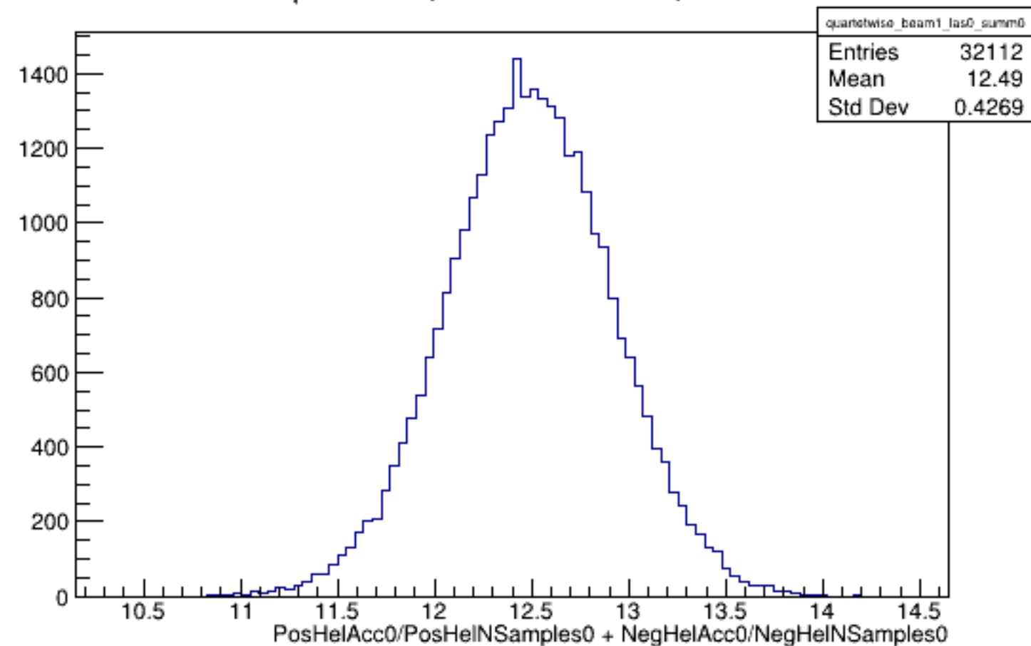
Run 5047 quartetwise, Sums0: Beam ON, Laser OFF
