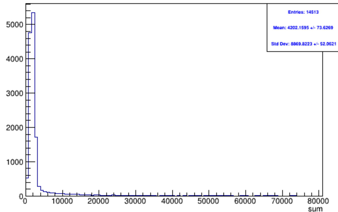
Run 5052 triggerwise, sums: Beam OFF
