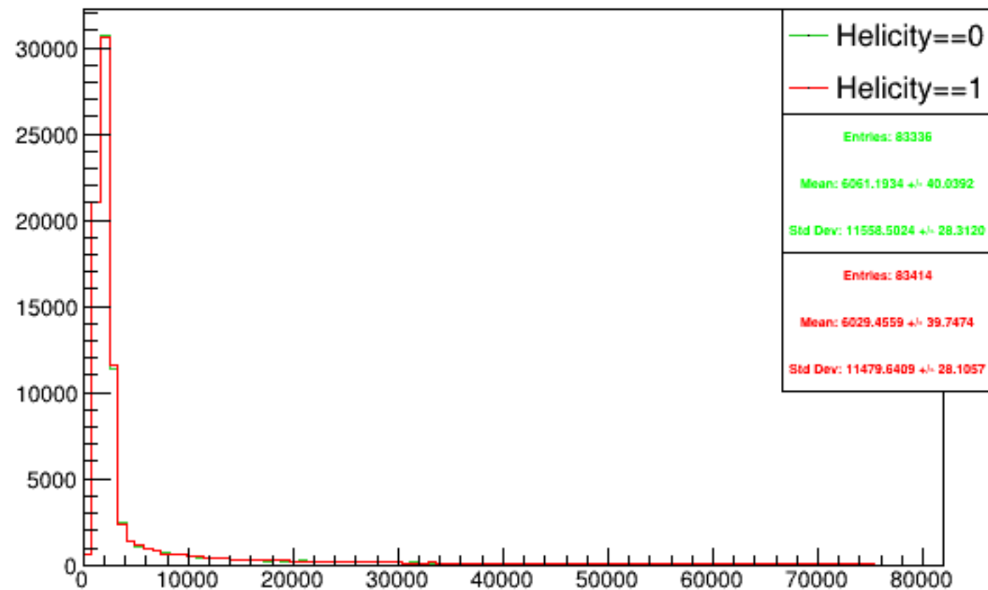
Run 5052 triggerwise, sums: Beam ON, Laser OFF
