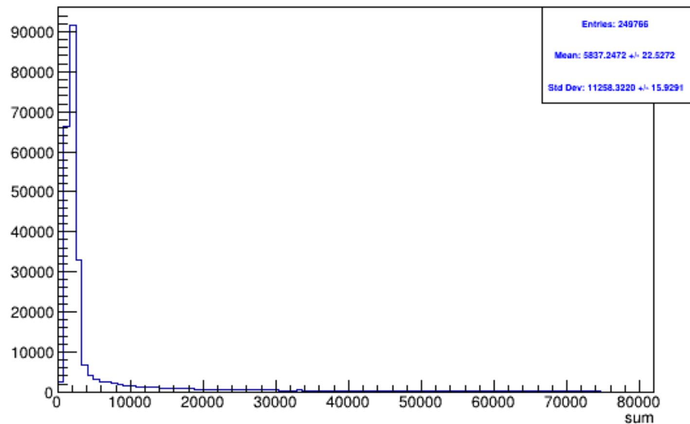
Run 5052 triggerwise, sums: All
