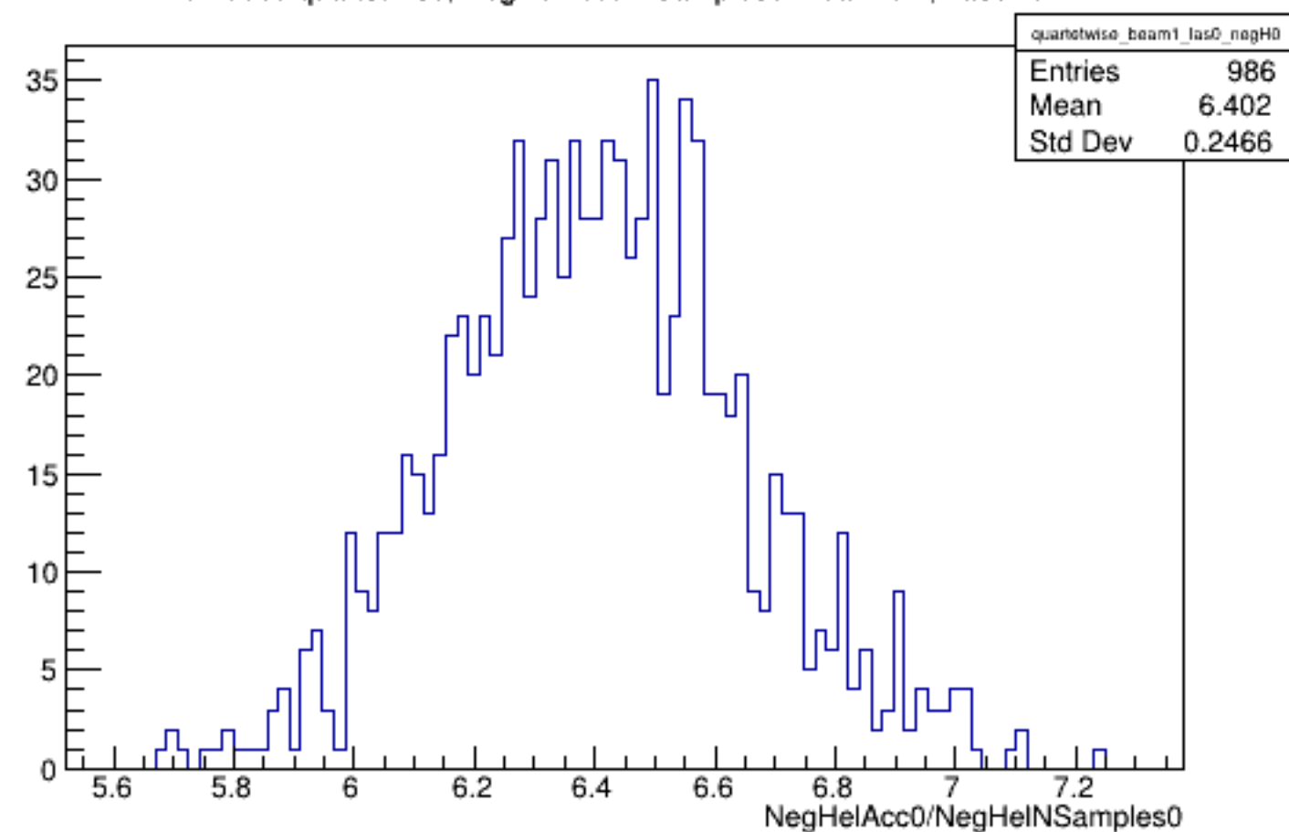
Run 5066 quartetwise, NegHelAcc0/NSamples0: Beam ON, Laser OFF
