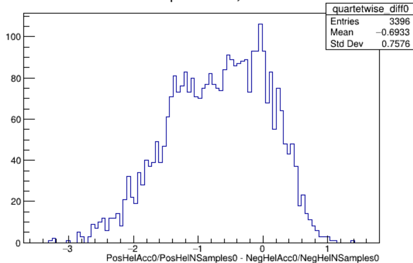
Run 5066 quartetwise, Diffs0: All
