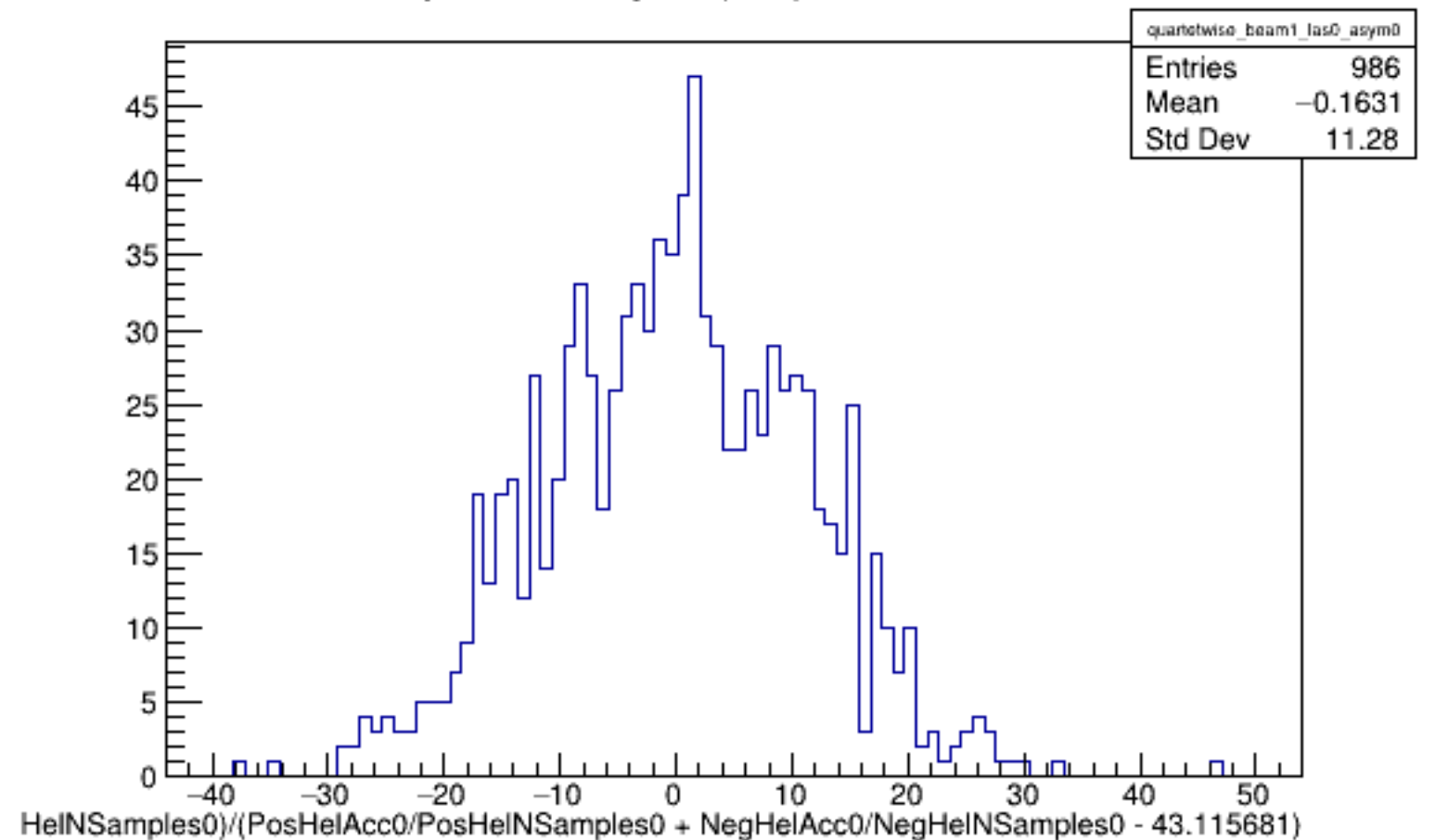
Run 5066 quartetwise, Asyms0 (Raw): Beam ON, Laser OFF
