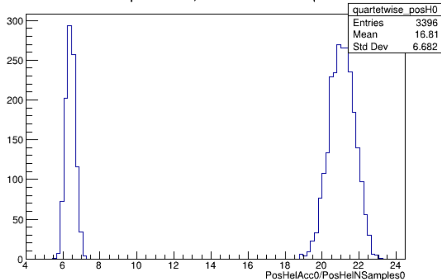
Run 5066 quartetwise, PosHelAcc0/NSamples0: All
