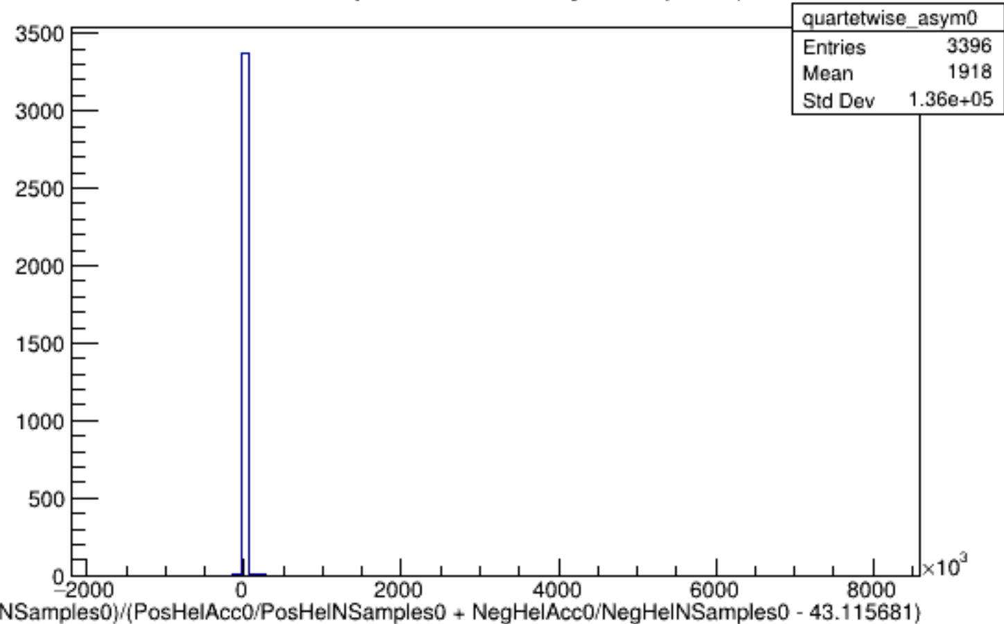
Run 5066 quartetwise, Asyms0 (Raw): All
