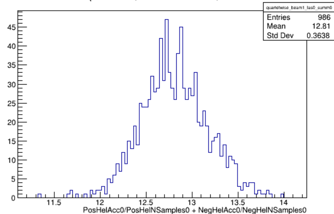
Run 5066 quartetwise, Sums0: Beam ON, Laser OFF
