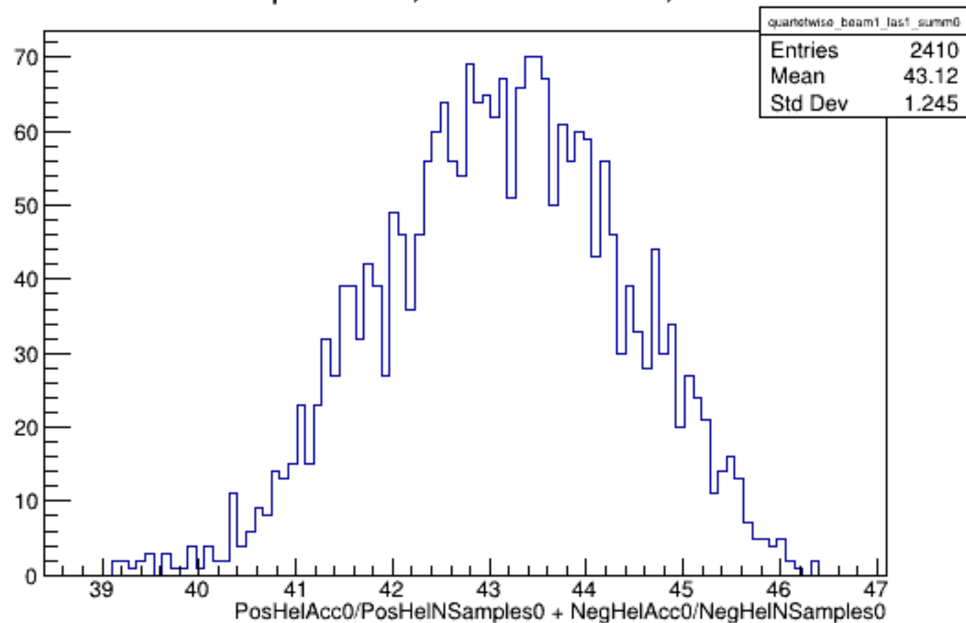
Run 5066 quartetwise, Sums0: Beam ON, Laser ON
