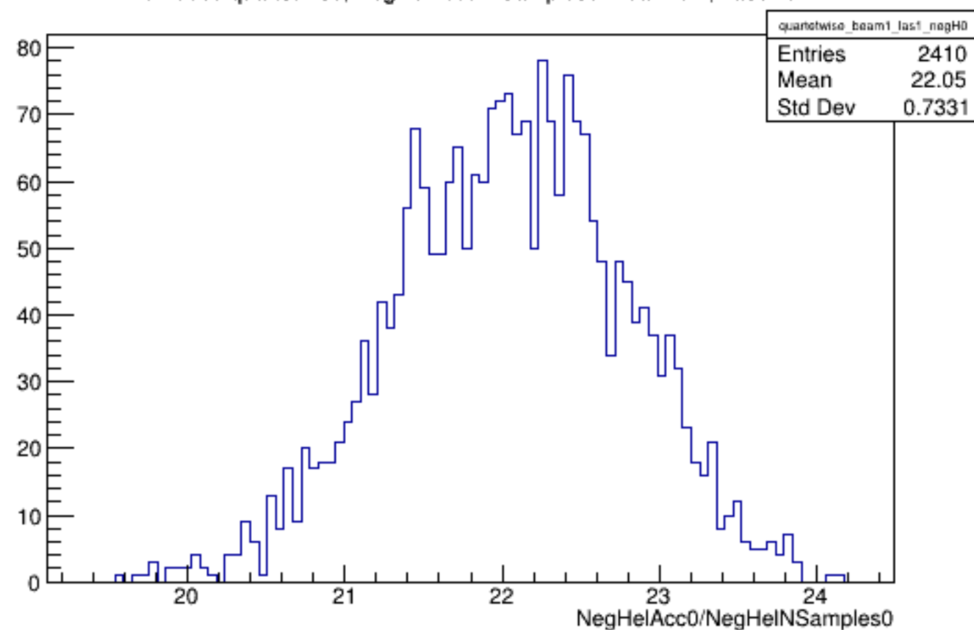
Run 5066 quartetwise, NegHelAcc0/NSamples0: Beam ON, Laser ON
