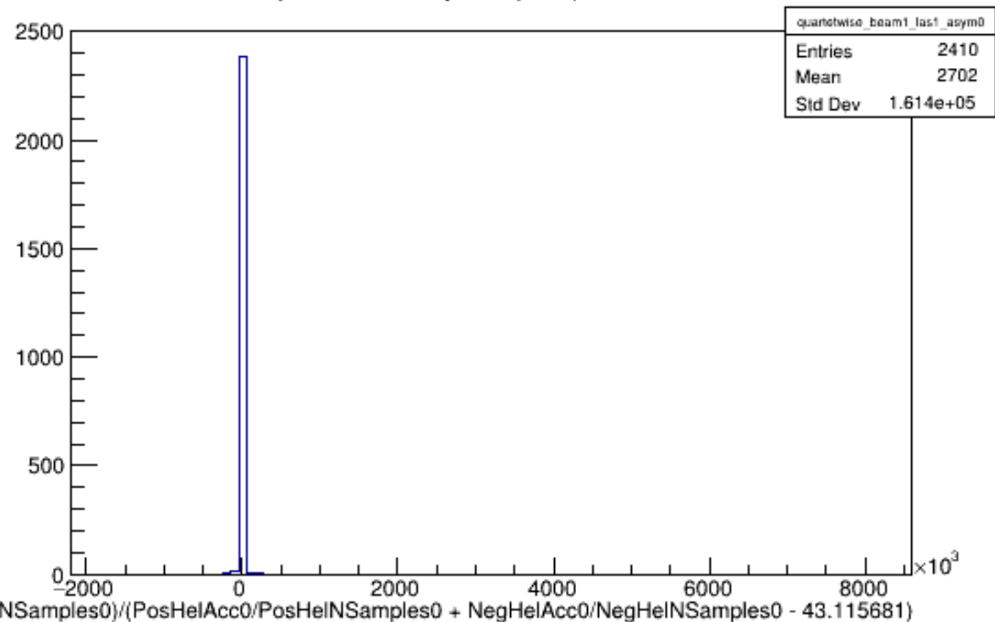
Run 5066 quartetwise, Asyms0 (Raw): Beam ON, Laser ON
