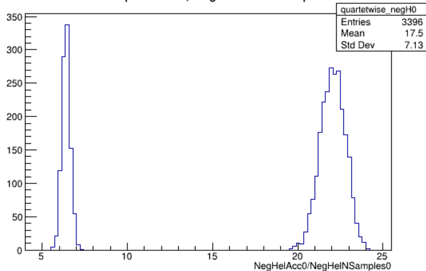
Run 5066 quartetwise, NegHelAcc0/NSamples0: All
