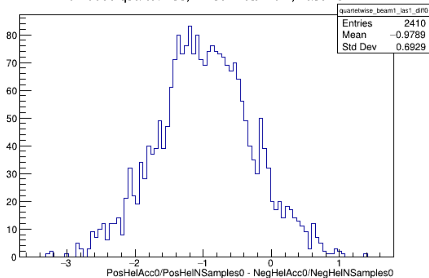
Run 5066 quartetwise, Diffs0: Beam ON, Laser ON
