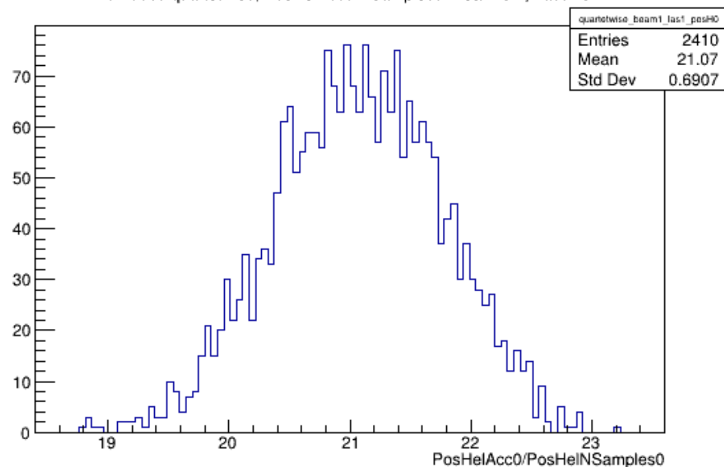
Run 5066 quartetwise, PosHelAcc0/NSamples0: Beam ON, Laser ON
