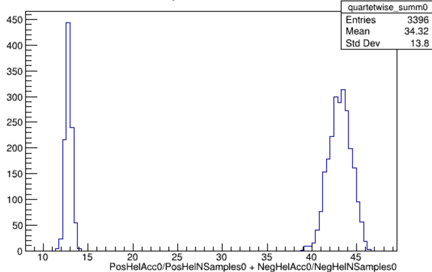
Run 5066 quartetwise, Sums0: All
