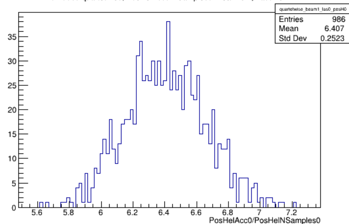
Run 5066 quartetwise, PosHelAcc0/NSamples0: Beam ON, Laser OFF
