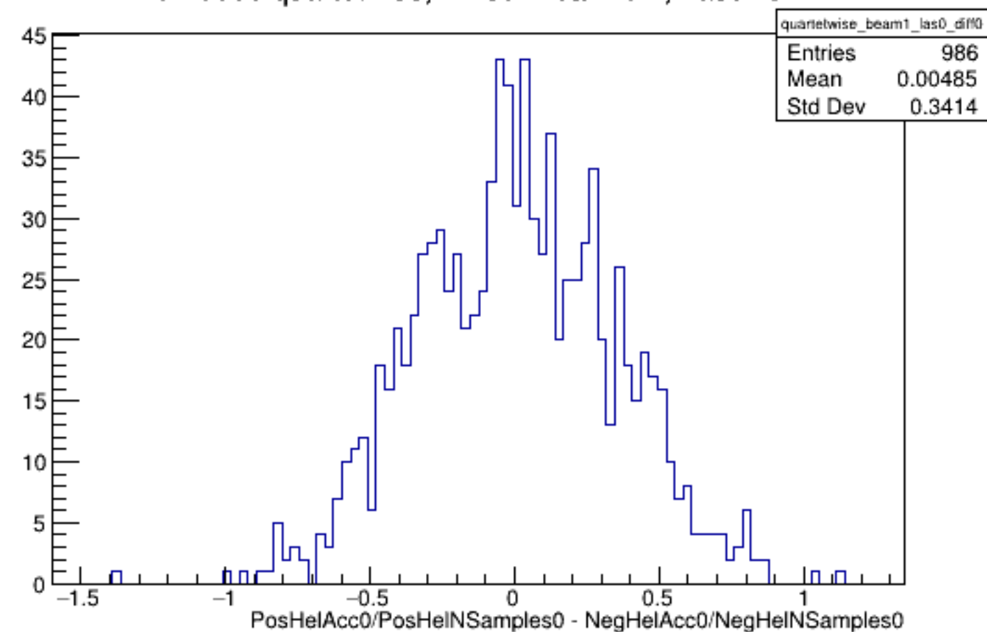
Run 5066 quartetwise, Diffs0: Beam ON, Laser OFF
