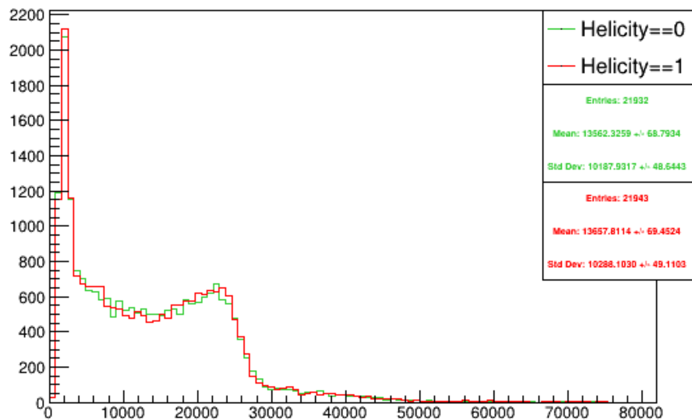
Run 5066 triggerwise, sums: Beam ON, Laser ON
