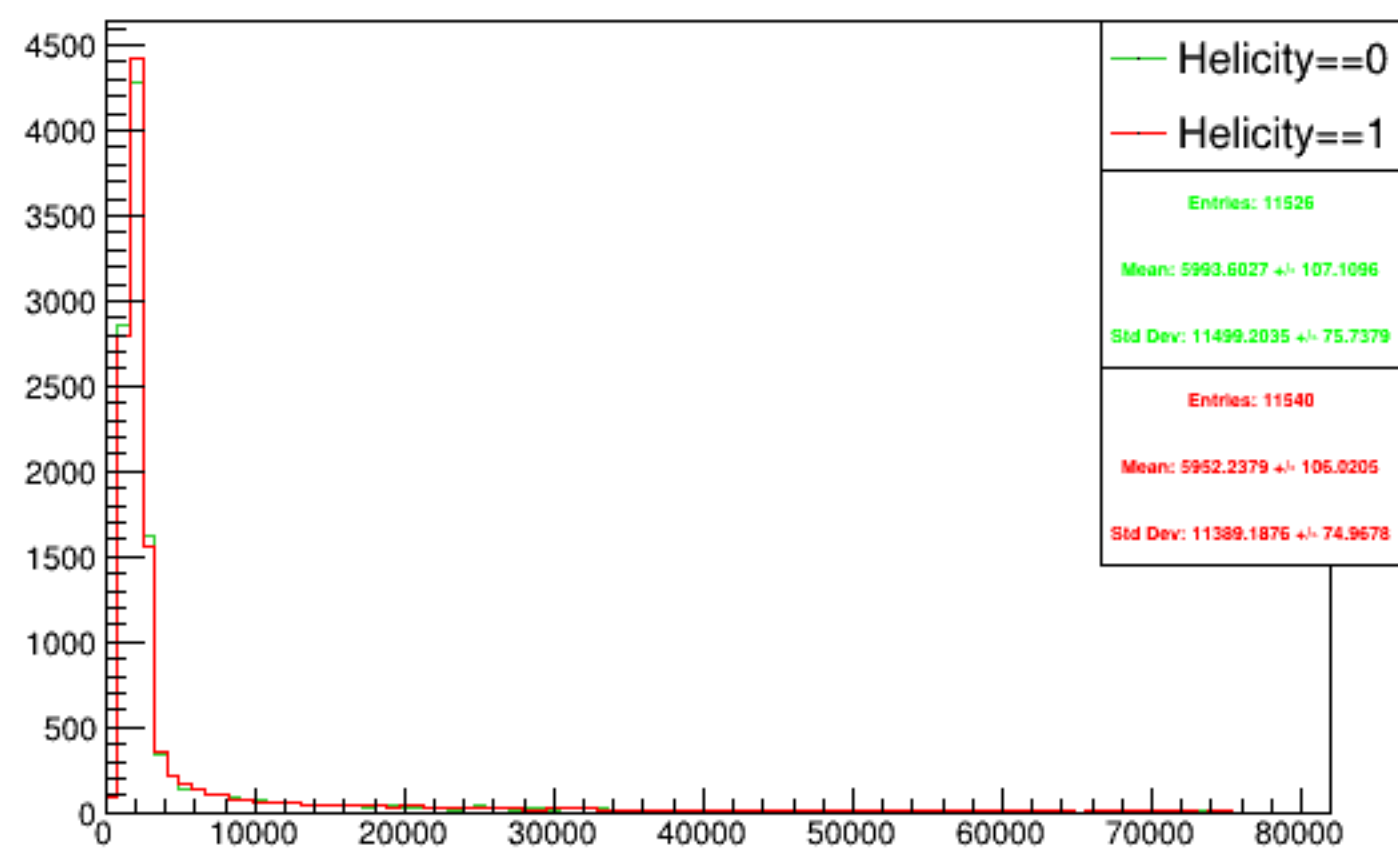
Run 5066 triggerwise, sums: Beam ON, Laser OFF
