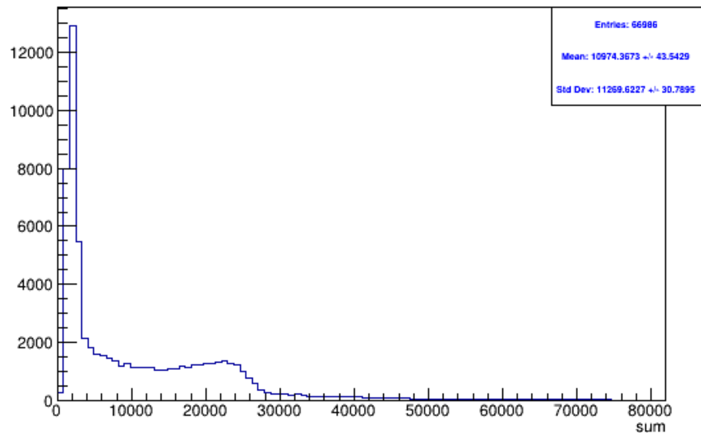
Run 5066 triggerwise, sums: All
