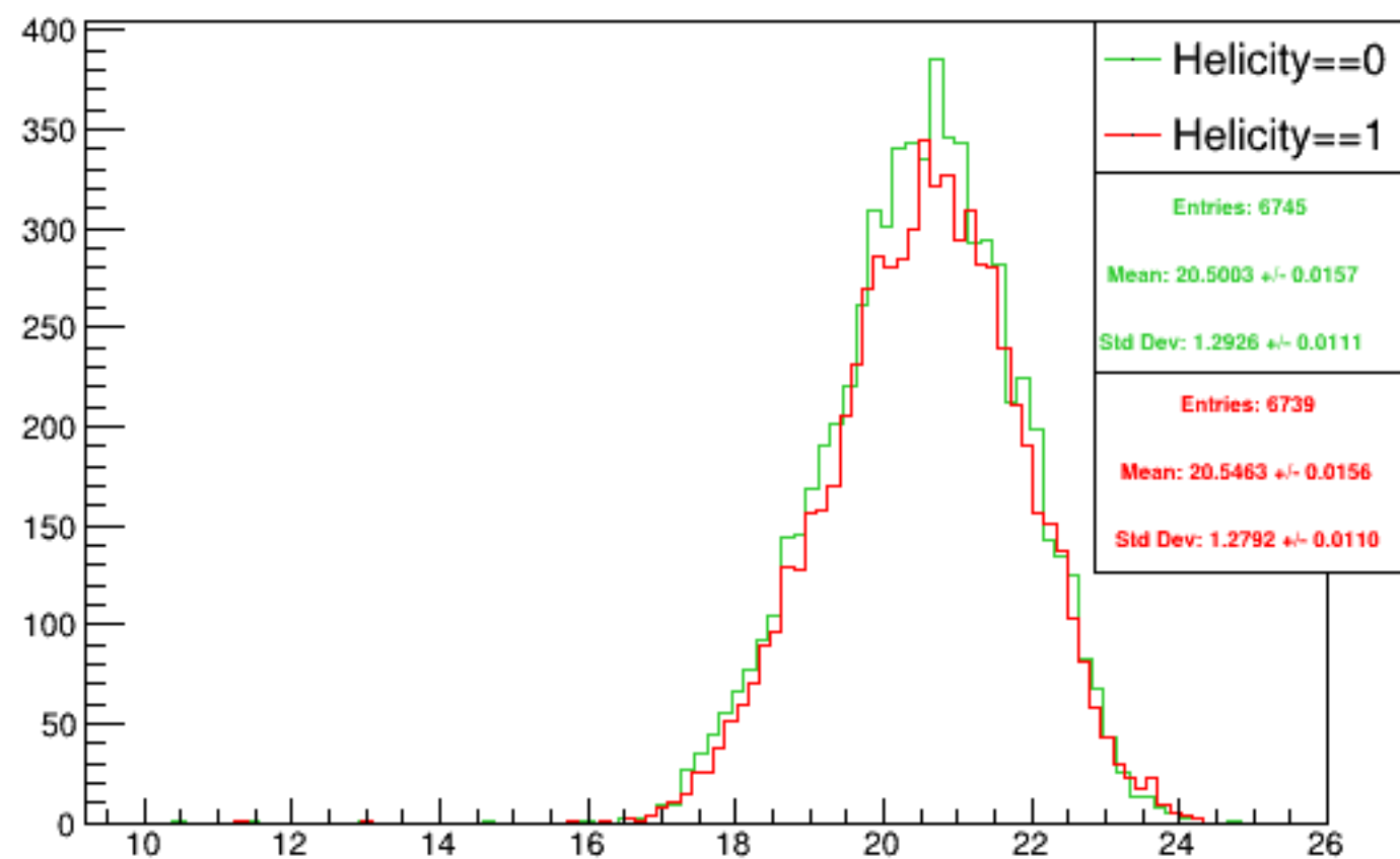
Run 5067 mpwise, acc0: Beam ON, Laser ON
