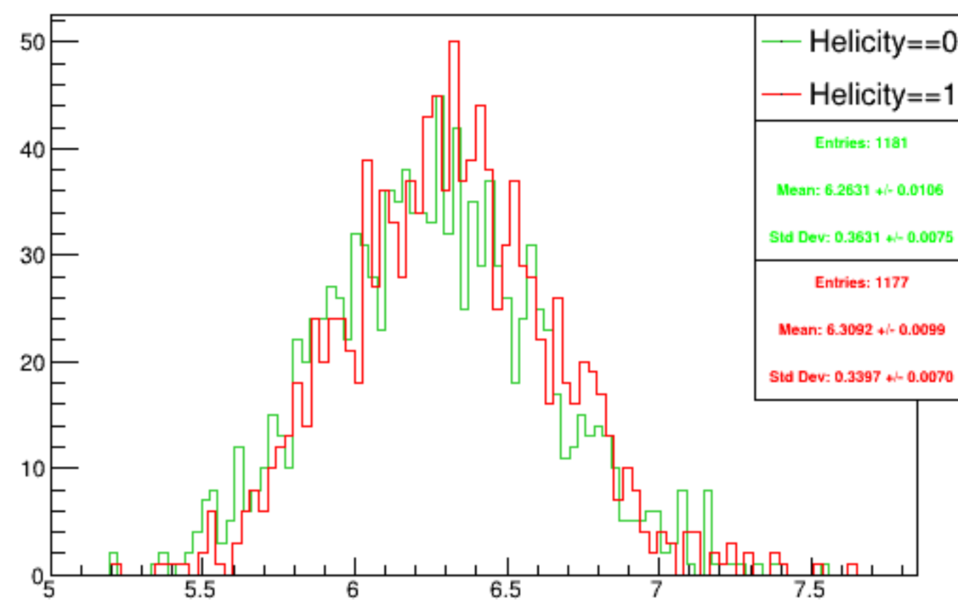
Run 5067 mpwise, acc0: Beam ON, Laser OFF
