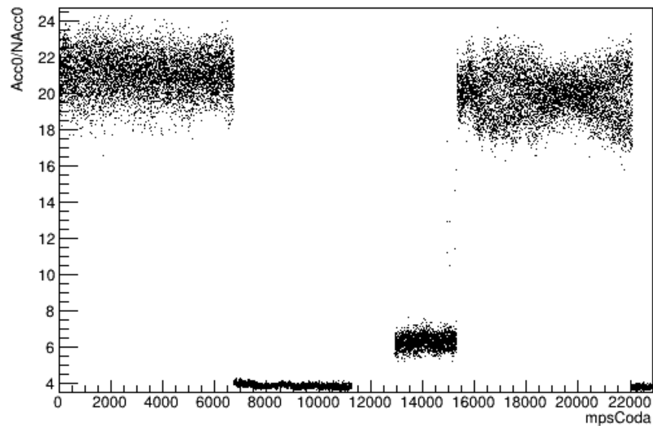
Run 5067 mpwise, Acc0 vs Time: All
