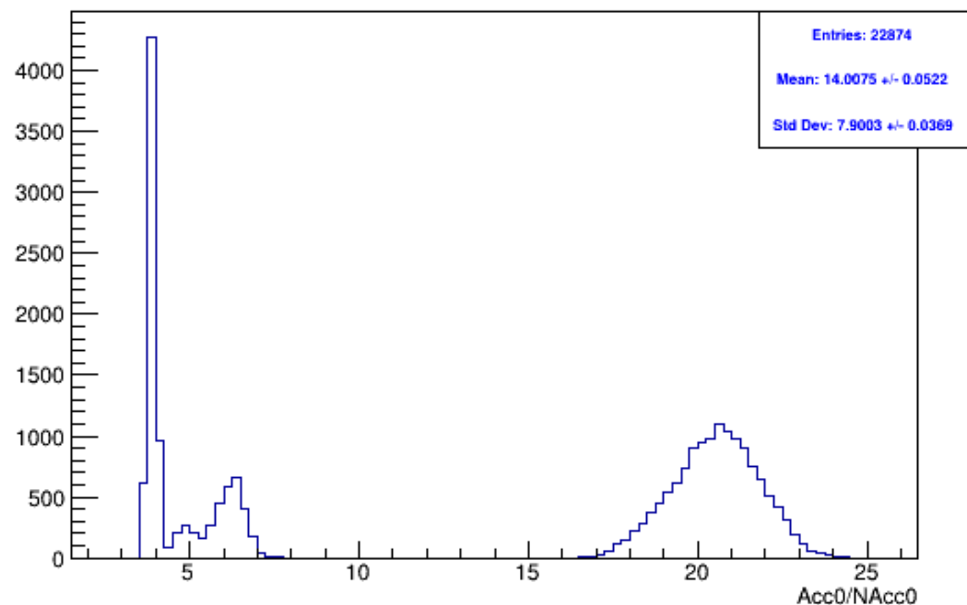
Run 5067 mpwise, acc0: All
