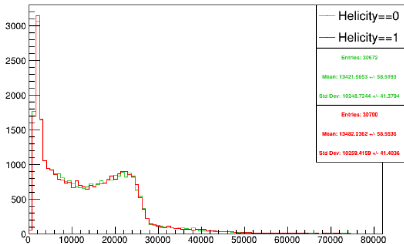
Run 5067 triggerwise, sums: Beam ON, Laser ON
