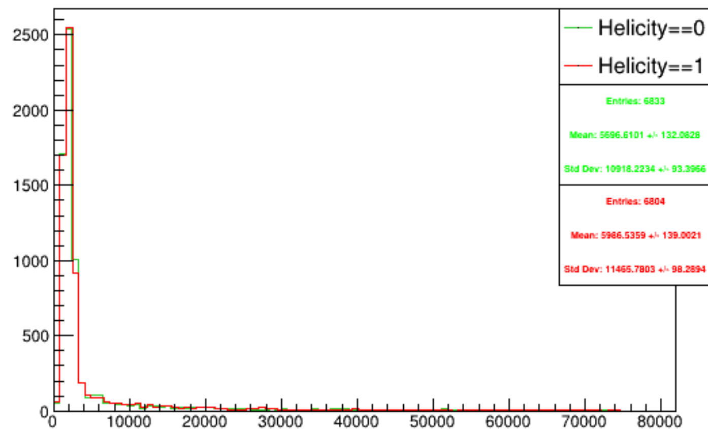
Run 5067 triggerwise, sums: Beam ON, Laser OFF
