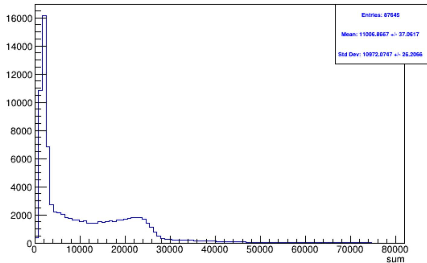
Run 5067 triggerwise, sums: All
