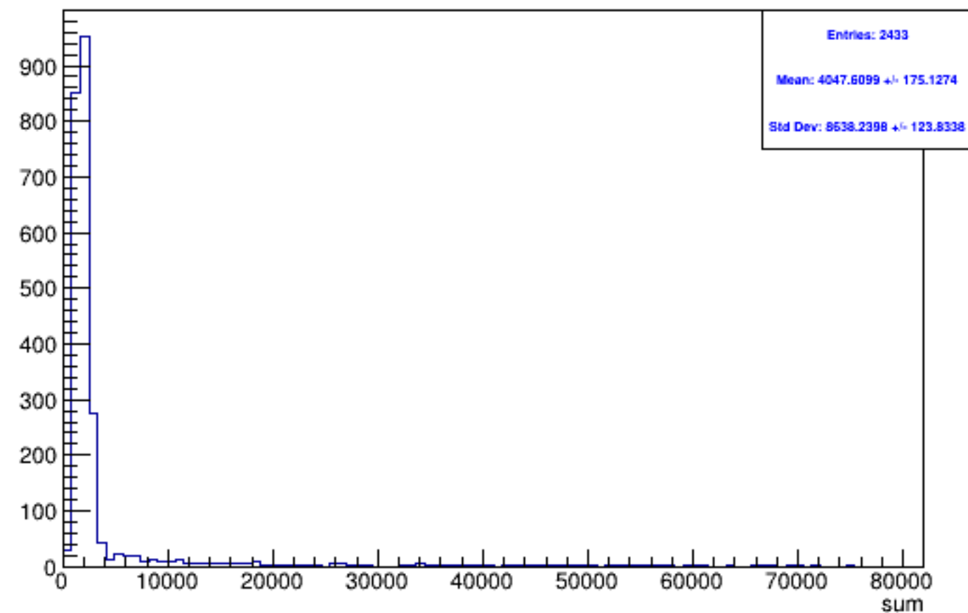
Run 5067 triggerwise, sums: Beam OFF
