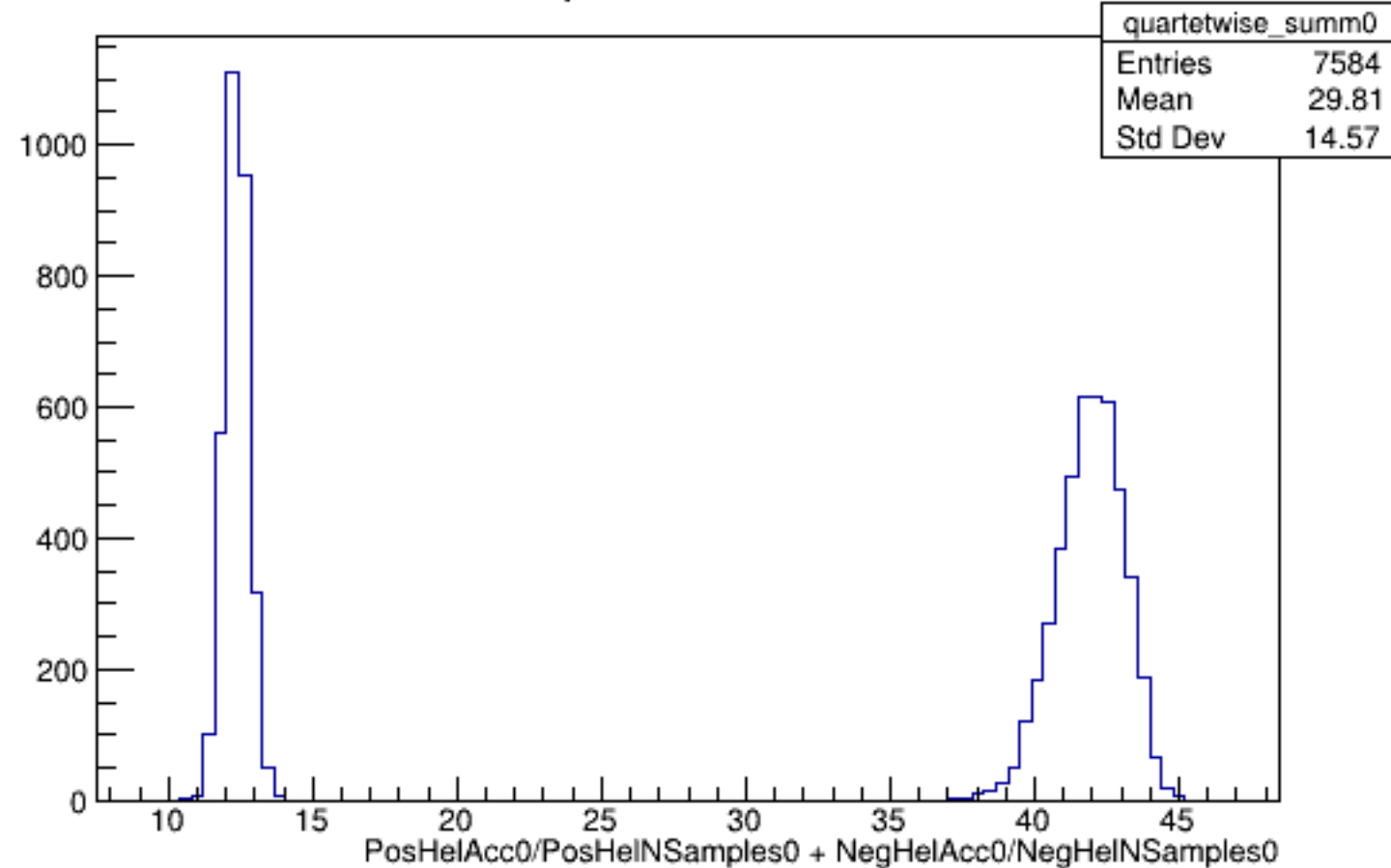
Run 5068 quartetwise, Sums0: All
