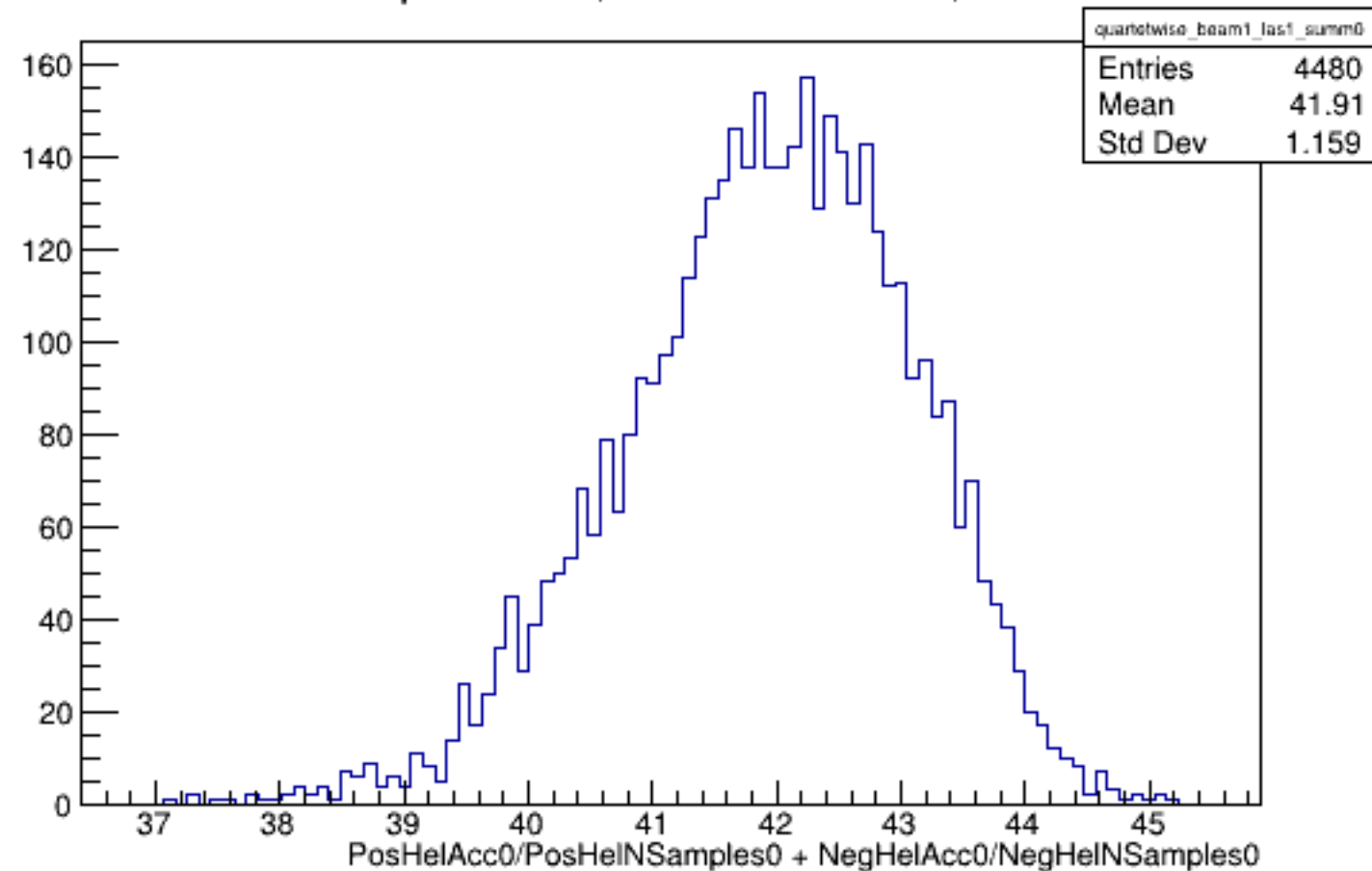
Run 5068 quartetwise, Sums0: Beam ON, Laser ON
