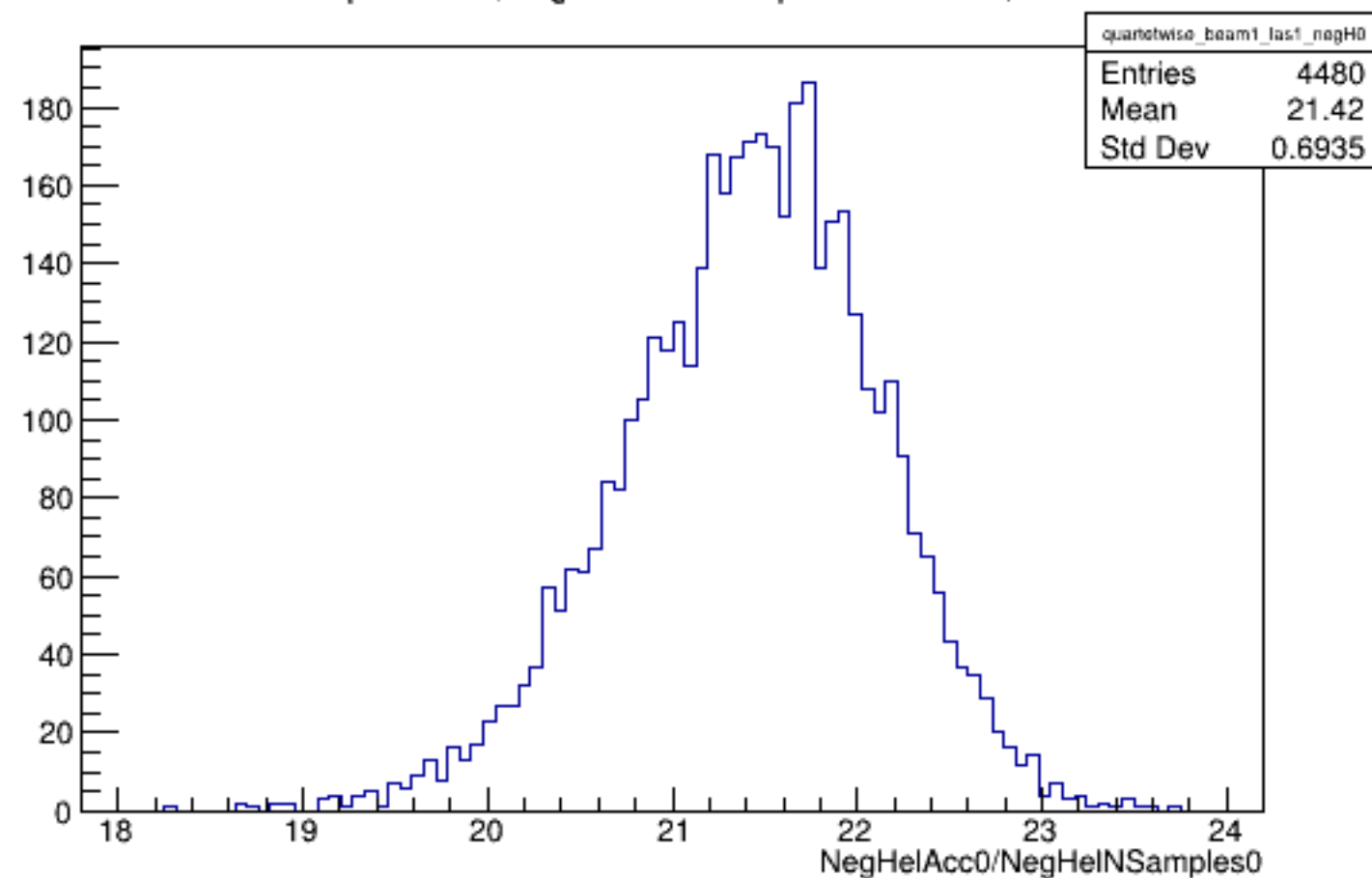
Run 5068 quartetwise, NegHelAcc0/NSamples0: Beam ON, Laser ON
