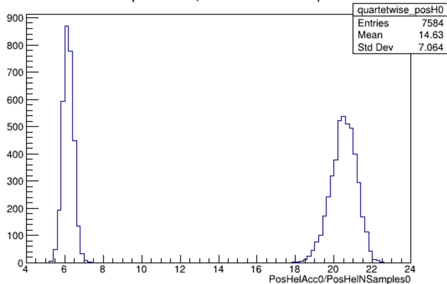
Run 5068 quartetwise, PosHelAcc0/NSamples0: All
