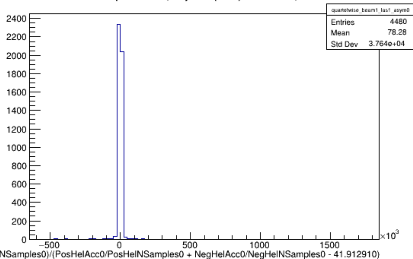
Run 5068 quartetwise, Asyms0 (Raw): Beam ON, Laser ON
