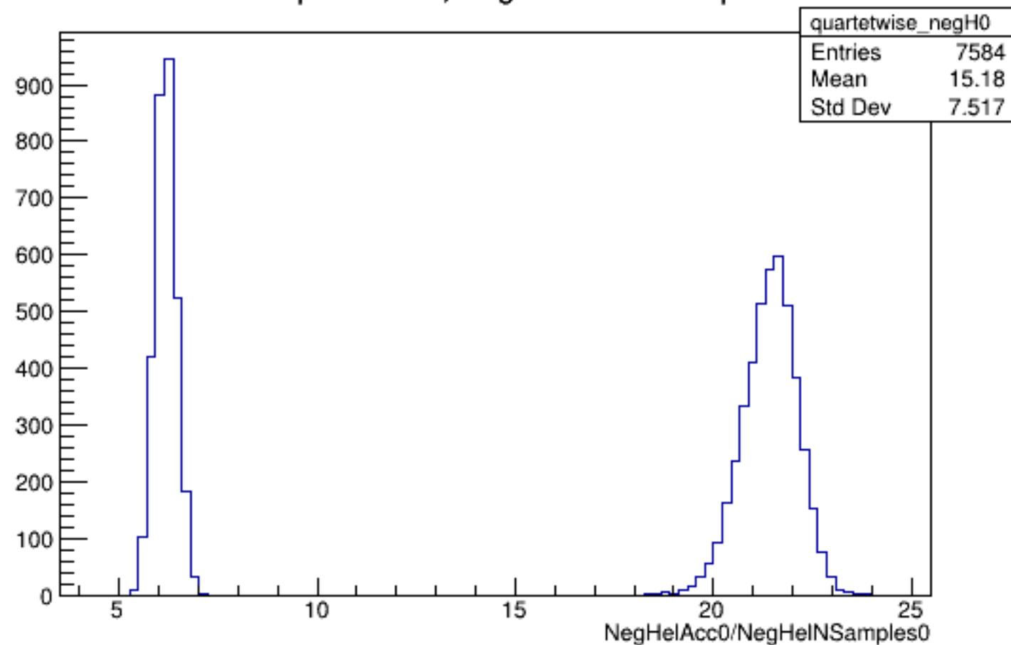
Run 5068 quartetwise, NegHelAcc0/NSamples0: All
