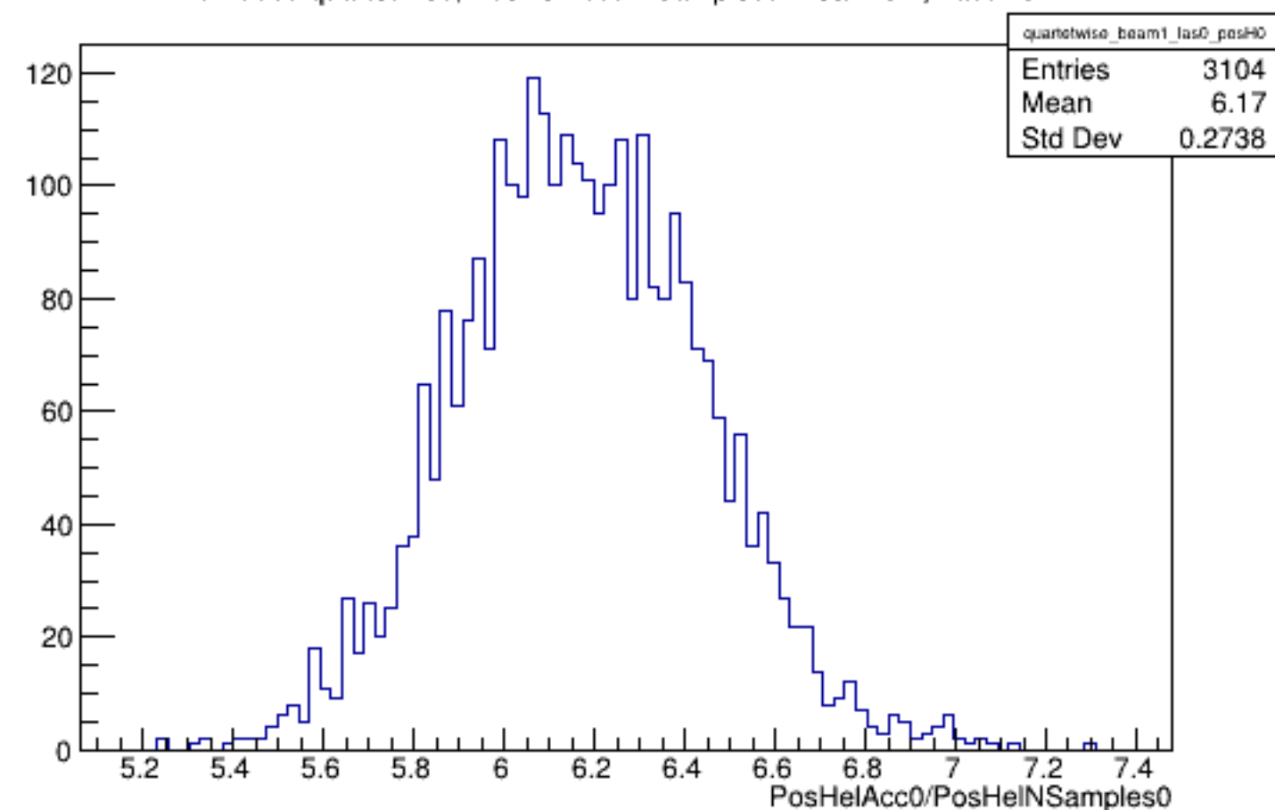
Run 5068 quartetwise, PosHelAcc0/NSamples0: Beam ON, Laser OFF
