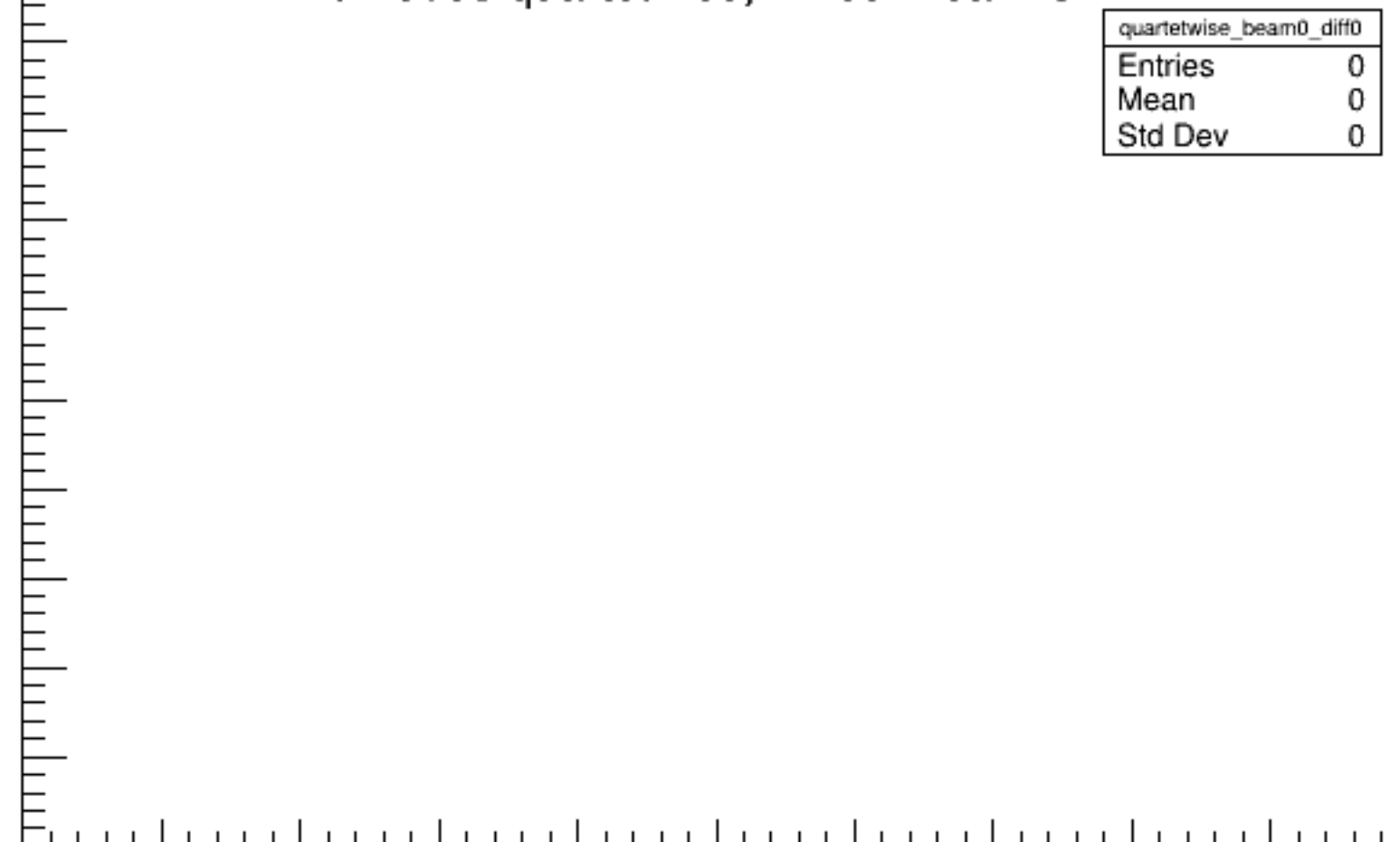
Run 5068 quartetwise, Diffs0: Beam OFF
