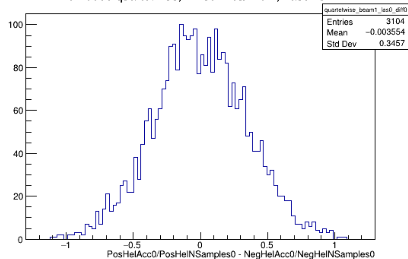
Run 5068 quartetwise, Diffs0: Beam ON, Laser OFF
