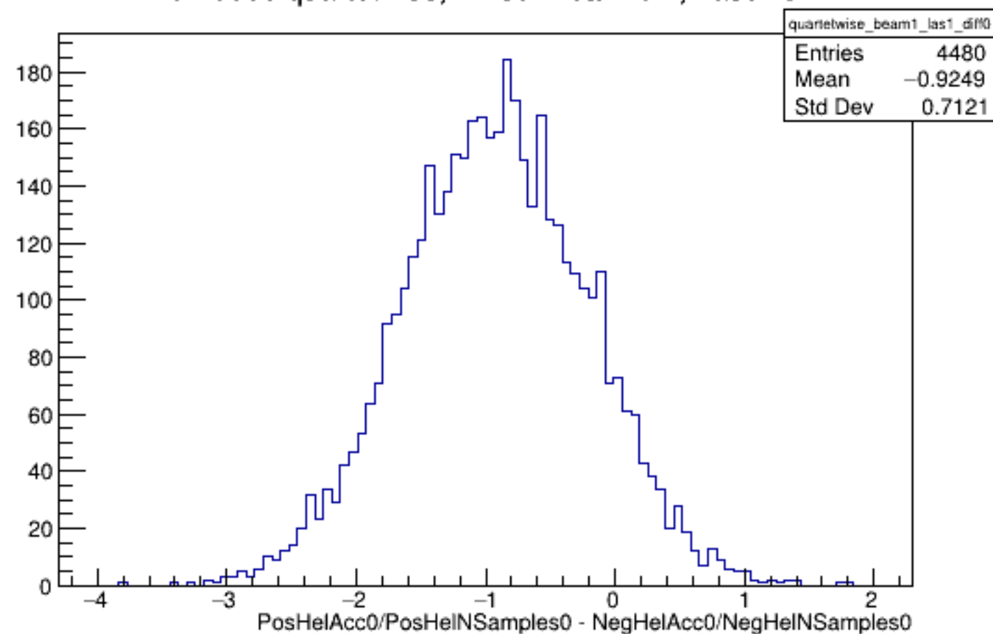
Run 5068 quartetwise, Diffs0: Beam ON, Laser ON
