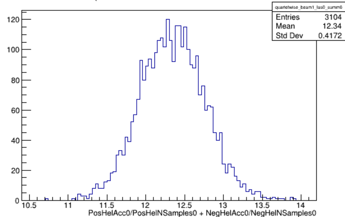
Run 5068 quartetwise, Sums0: Beam ON, Laser OFF
