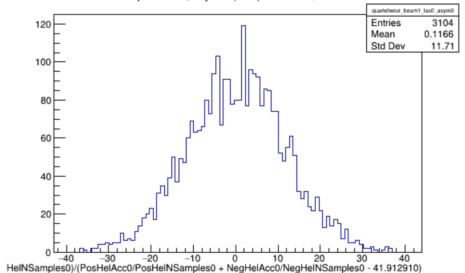
Run 5068 quartetwise, Asyms0 (Raw): Beam ON, Laser OFF
