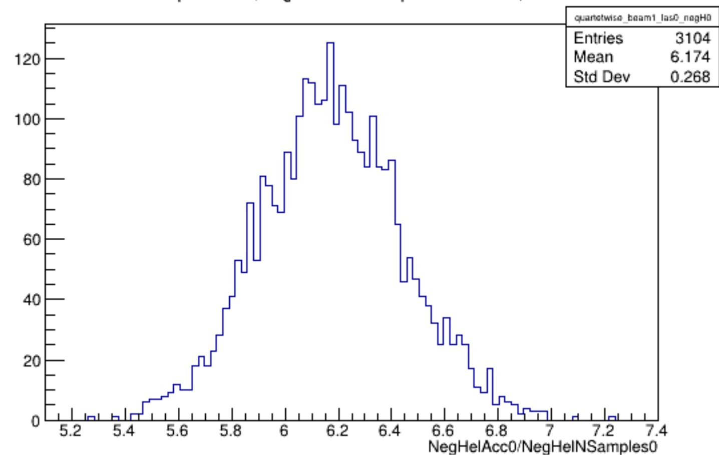
Run 5068 quartetwise, NegHelAcc0/NSamples0: Beam ON, Laser OFF
