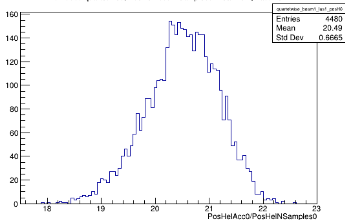
Run 5068 quartetwise, PosHelAcc0/NSamples0: Beam ON, Laser ON
