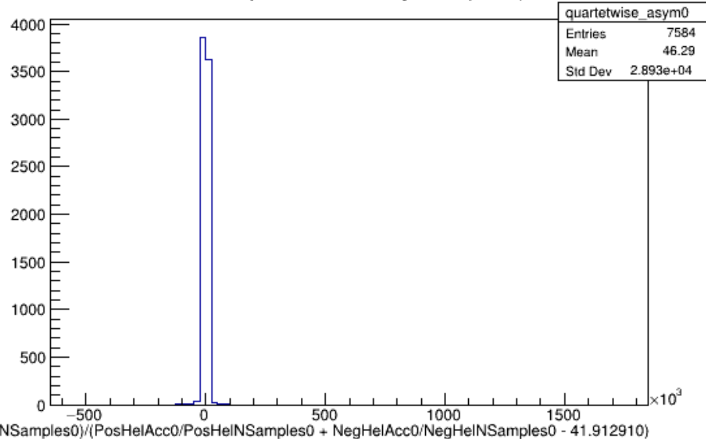
Run 5068 quartetwise, Asyms0 (Raw): All
