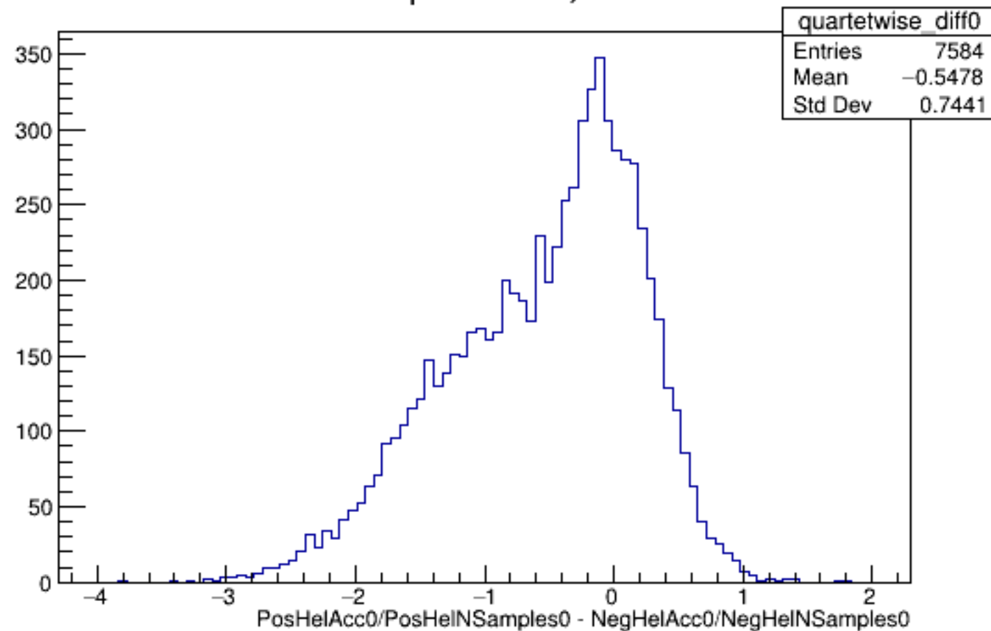
Run 5068 quartetwise, Diffs0: All
