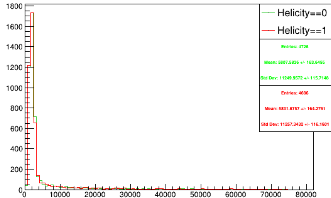
Run 5071 triggerwise, sums: Beam ON, Laser OFF
