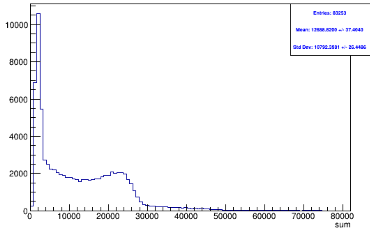
Run 5071 triggerwise, sums: All
