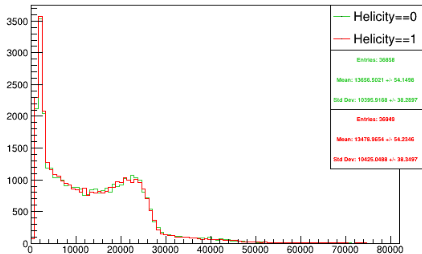
Run 5071 triggerwise, sums: Beam ON, Laser ON
