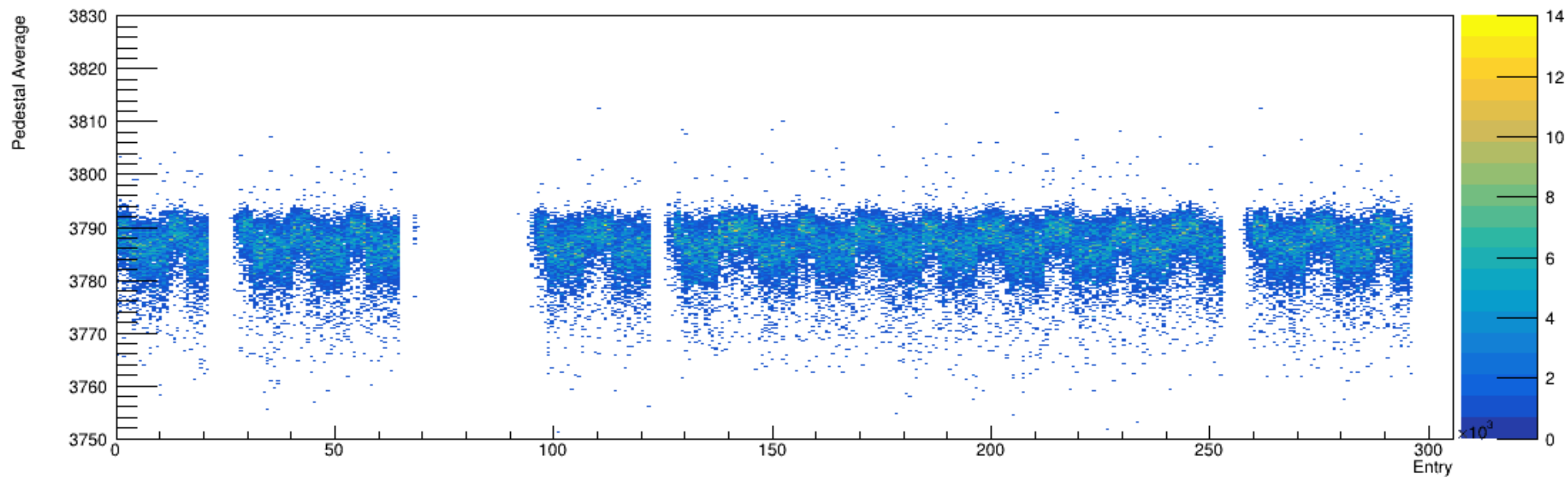
Run 5072, snapshots: Pedestal vs. Time
