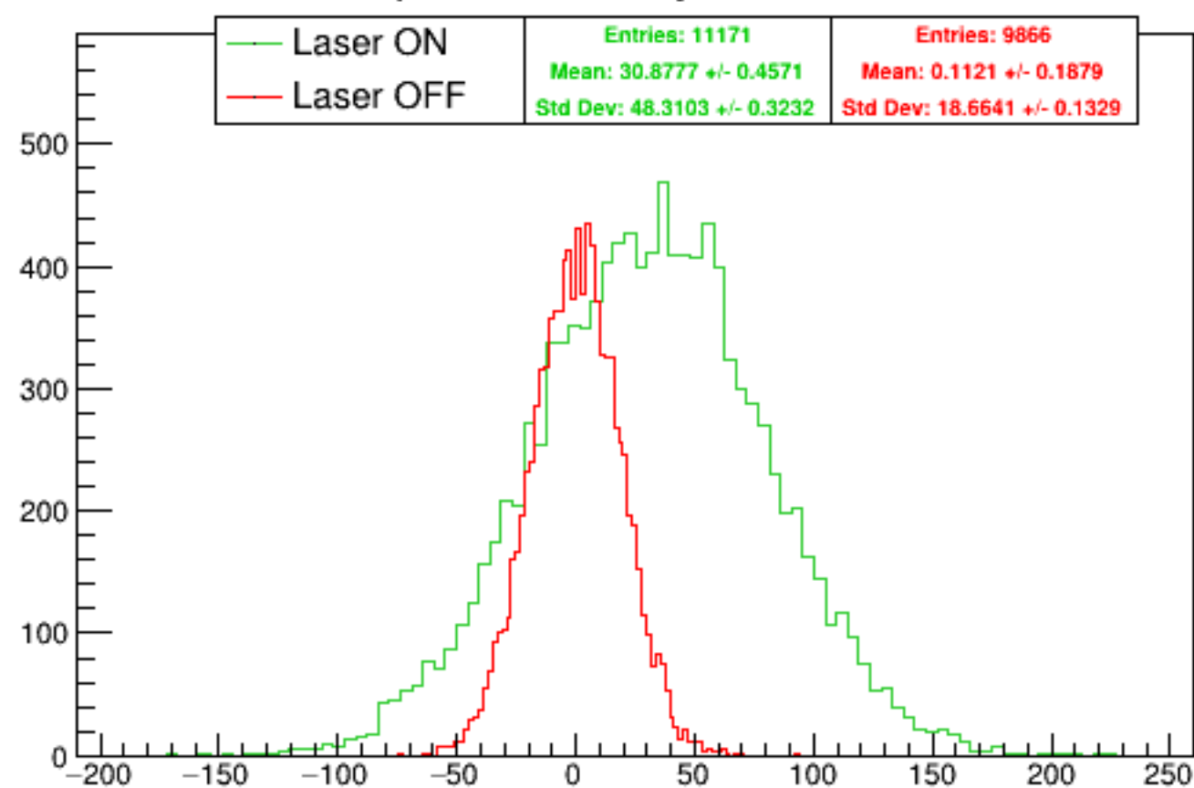
Run 5080 quartetwise, asym0sub: Beam ON
